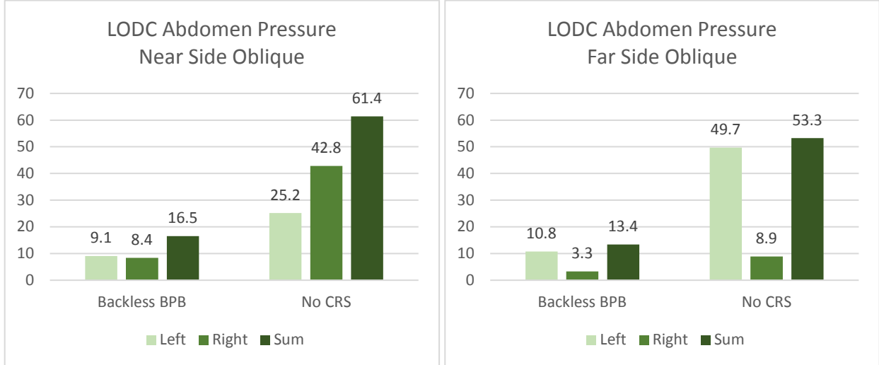
Figure 39. Near side occupant (left) and far side occupant (right) abdomen pressure results from the oblique Malibu buck sled tests for the LODC Rev4
