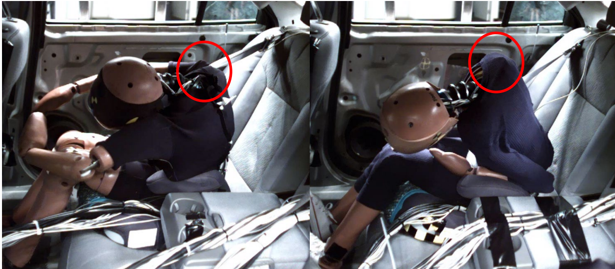
Figure 37. Far side oblique tests with the backless BPB showing shoulder belt engagement with the LODC Rev4 (left) and lack of belt engagement and torso roll out of the HIII-10C (right)
