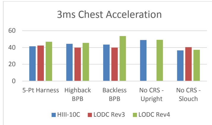
Figure 25. FMVSS No. 213 3 ms chest acceleration results for the HIII-10C (blue), LODC Rev3 (red), and LODC Rev4 (green)
