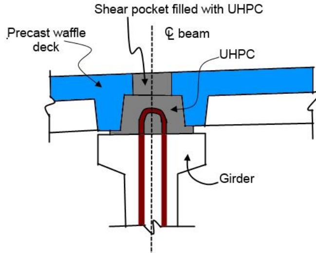
Figure 20. Connection detail between girder and waffle deck
