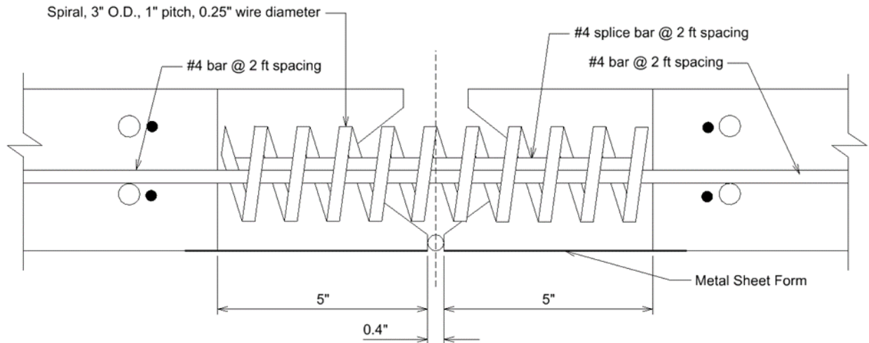
Figure 11. NU continuous precast prestressed panel reinforced pocket detail
