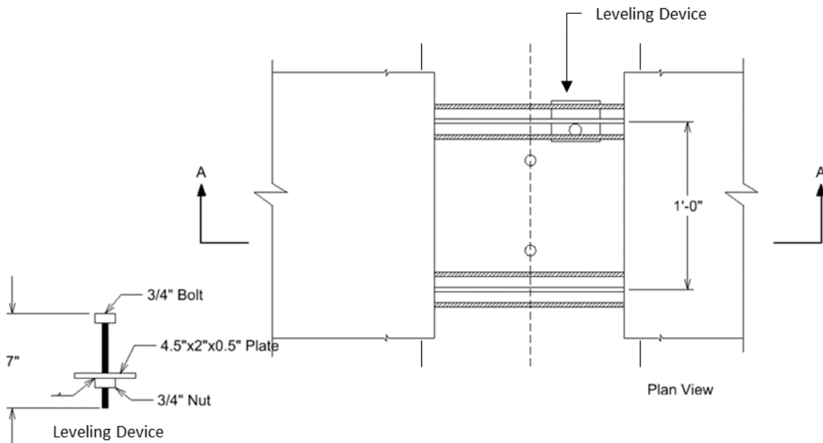
Figure 12. NU continuous precast prestressed panel leveling device
