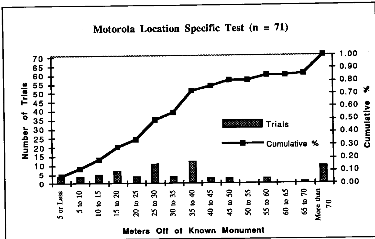
Figure 2.50 - Location Specific Test Results - Motorola Histogram
