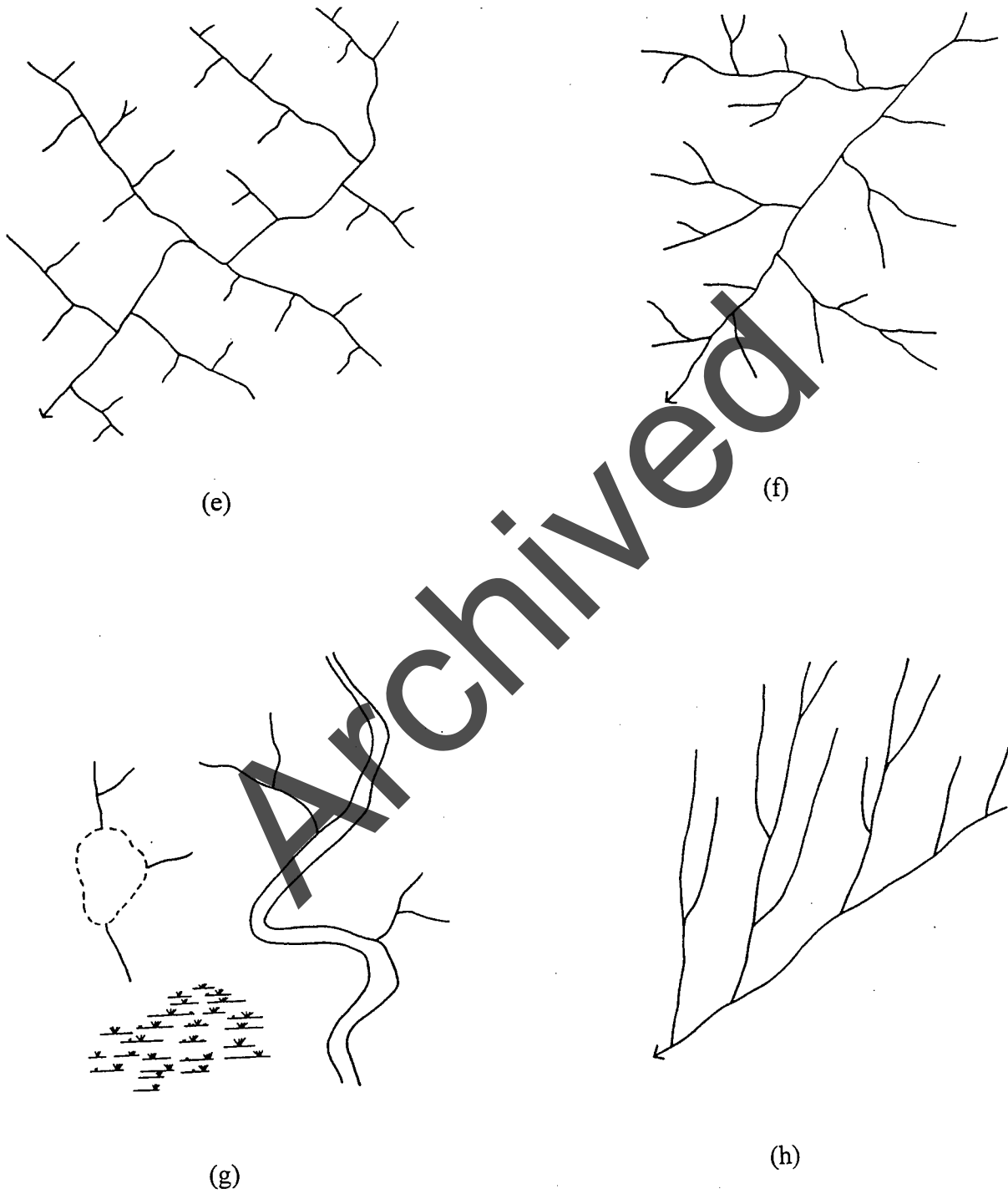
Figure 5-25b: Drainage Types. (e) Trellis Drainage Pattern, (f) Barbed Drainage Patten, (g) Deranged Drainage Pattern, (h) Parallel Drainage Pattern. (Way, 1973)
