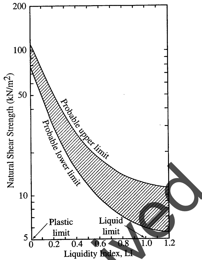
Figure 9-9: Relationship Between the Natural Shear Strength of Undisturbed Clays and LI. (Carter and Bentley, 1991)
