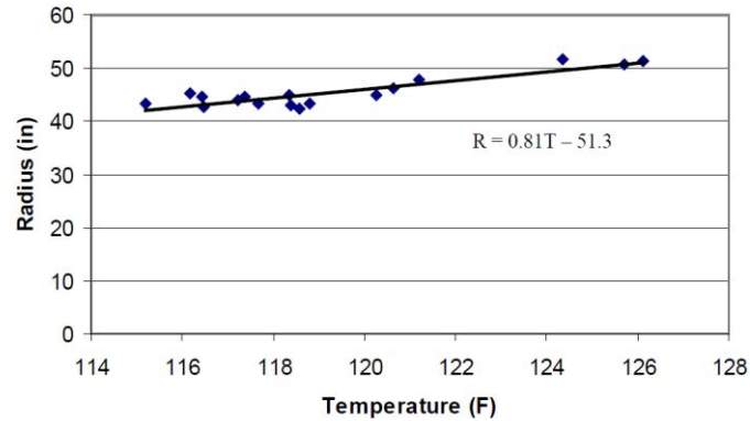
Figure 8: Example Level 2 temperature-radius model from Mullins and Winters (2011). Model is based on the data from Figure 7.
