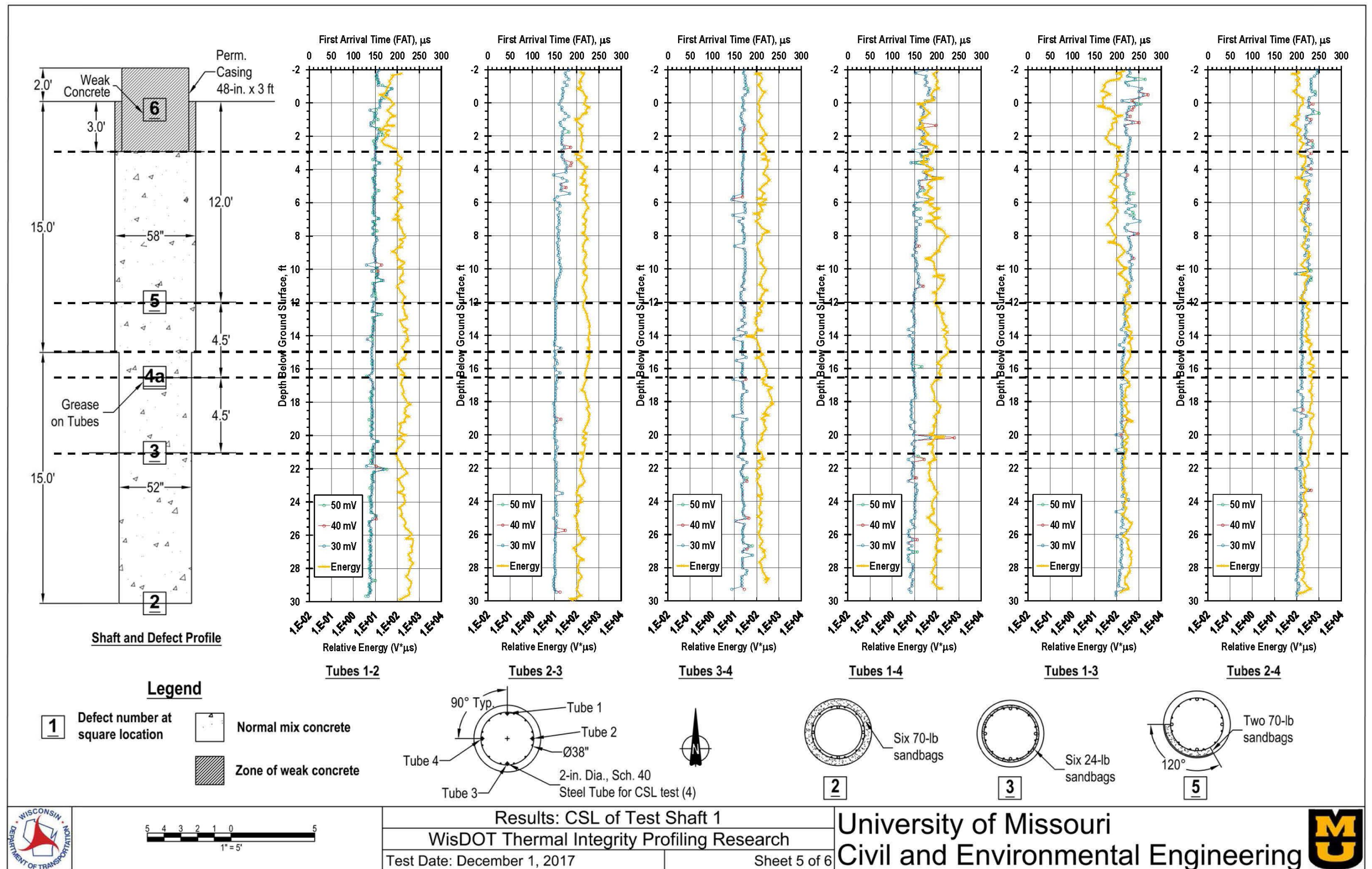
Figure 50: Results of CSL testing of Test Shaft 1.
