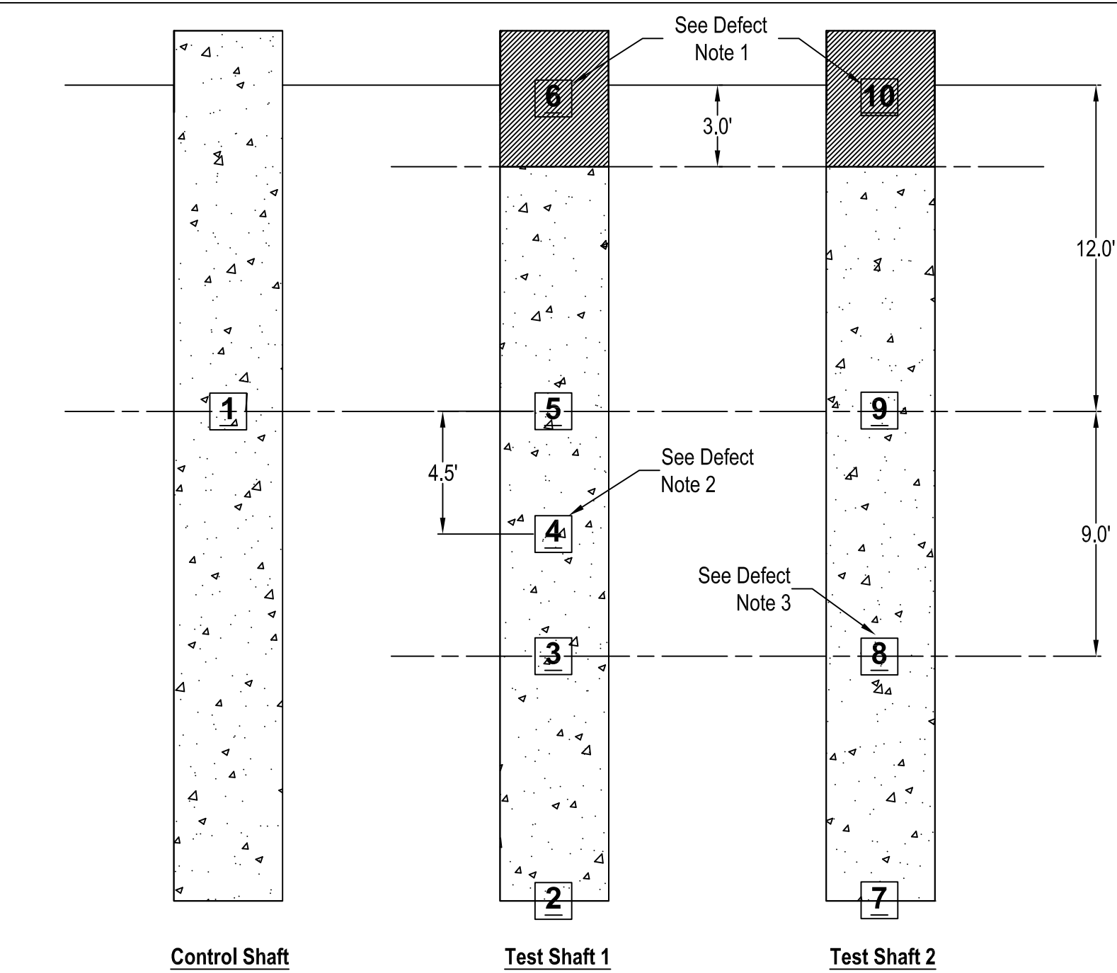
Shaft Profiles with Defect Locations
