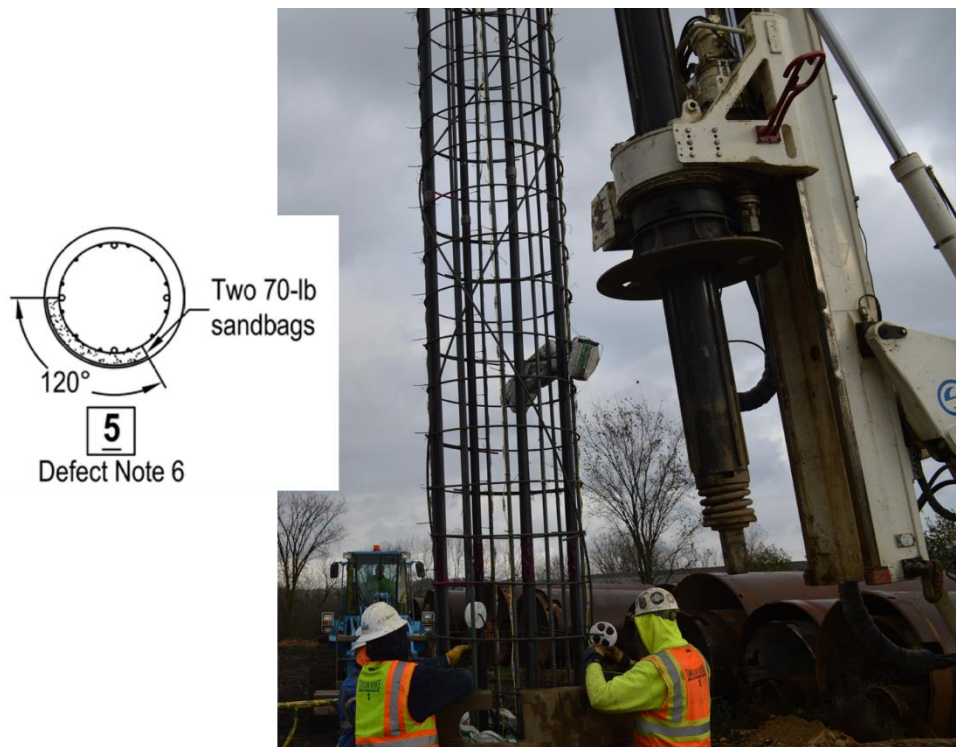
Figure 26: Defect 5 consisted of two 70 lb sandbags outside one side of the reinforcing cage for Test Shaft 1 at a depth of 12 ft.
