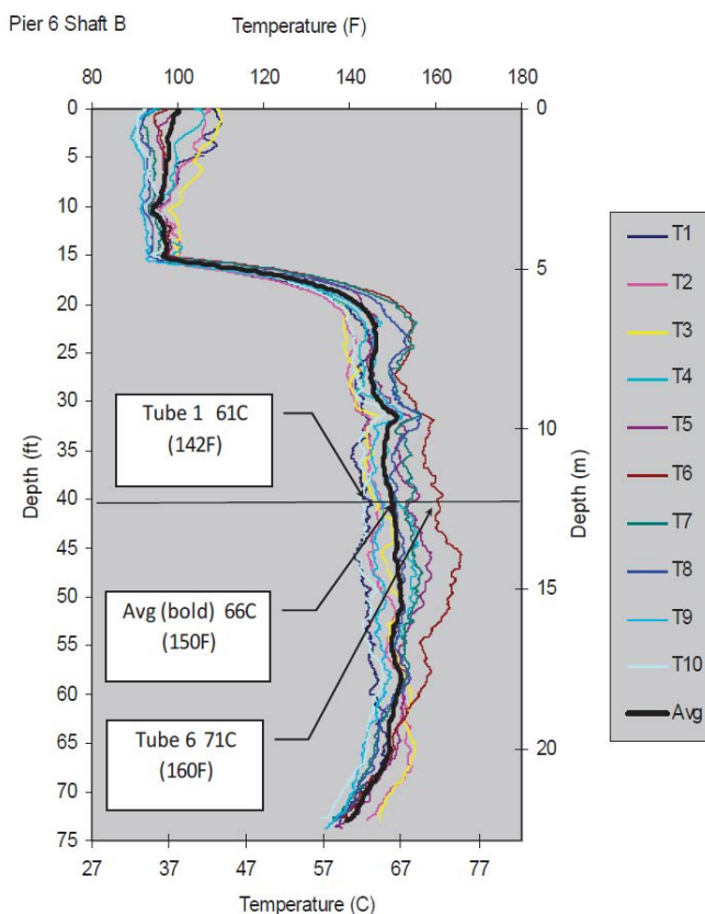
Figure 3: Example TIP result from Mullins (2010).
