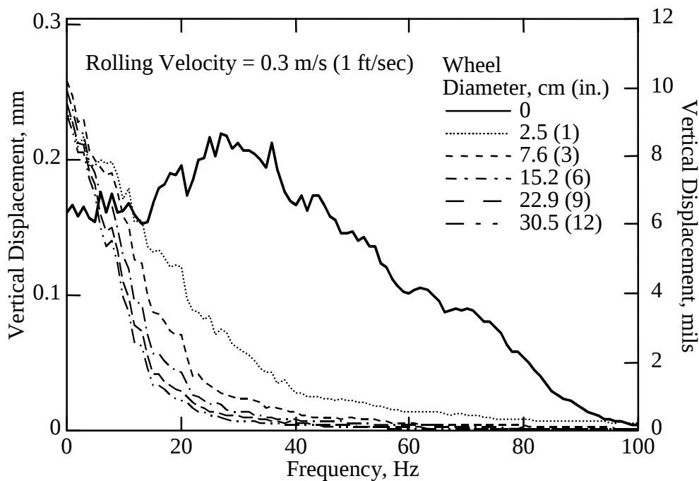
Figure 5.3 Vertical Displacement Spectra for Wheels with Various Diameters Rolling over the Synthesized Pavement Surface from Figure 5.1
