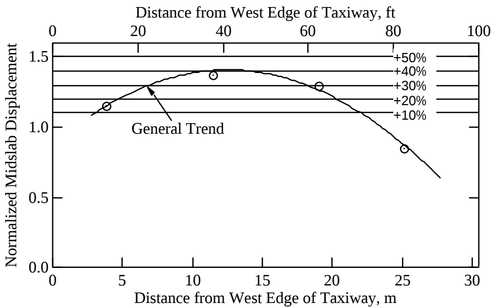
Figure 10.16 Normalized Midslab Displacements Measured at Taxiway L at the DFW International Airport
