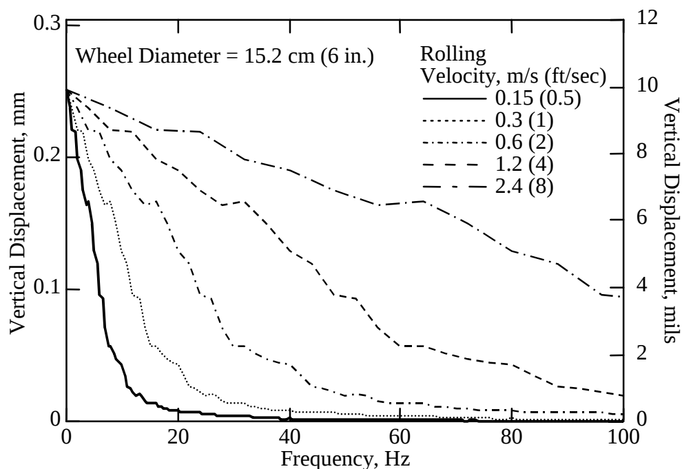
Figure 5.4 Vertical Displacement Spectra for 6-Inch Diameter Wheels Rolling over the Synthesized Pavement Surface from Figure 5.1 at Various Rolling Velocities
