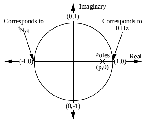
Figure 8.10 Plot of Unit Circle in the Z-Domain Showing Location of Poles for 0-Hz IIR Digital Notch-Pass Filter
