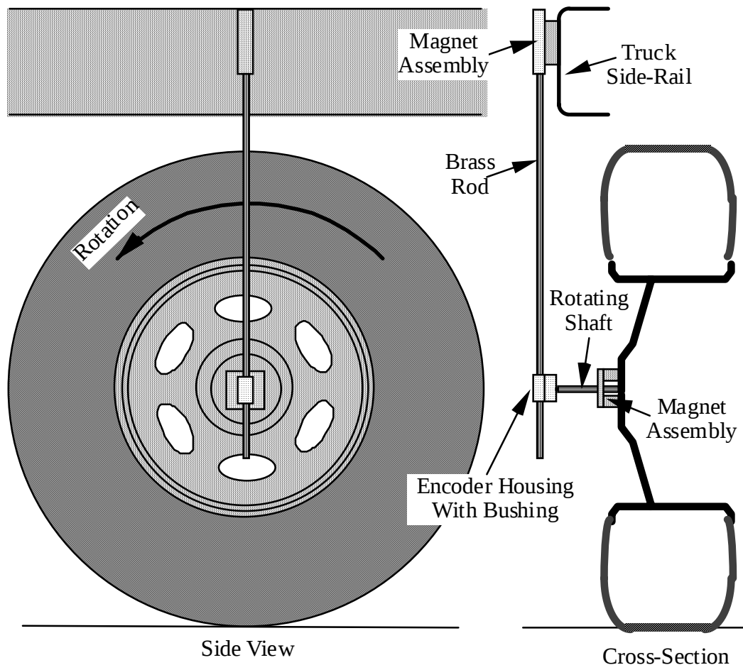
Figure 6.2 Side and Cross-Sectional Views Showing How the Rotary Encoder Mounts on a Truck Wheel
