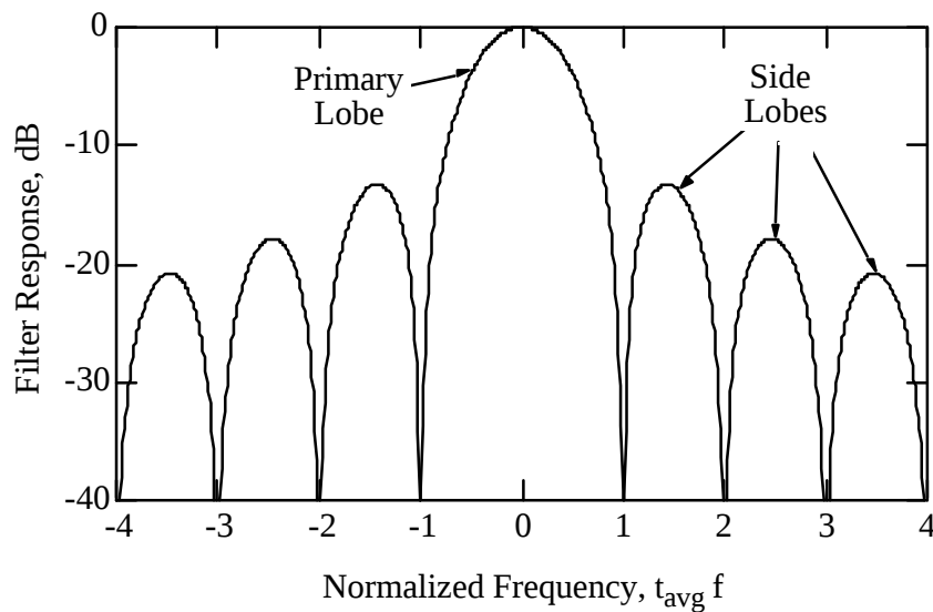
Figure 8.17 Response of FIR Digital Filter That Averages Data over a Time Interval of t_{avg}
