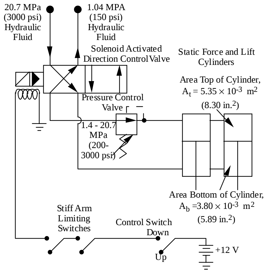
Figure 3.20 Schematic of Vibroseis Static Force and Lift System with Simplified Electrical Controls
