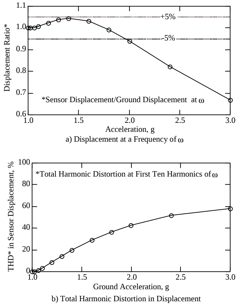
Figure 7.5 Amplitude and Distortion of Uncoupled Sensor at Acceleration Levels above 1 g
