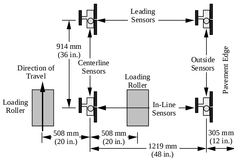
Figure 9.2 Rolling Sensor Configuration Used for RDD Testing on IH-10 near Orange, Texas
