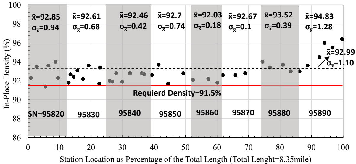
Figure 4-40 Construction information of In-Place Density (Gmm %) based on station locations (project STH 75) (12.5 mm Lift)
