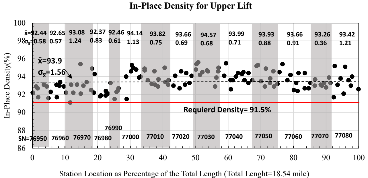
Figure 4-66 Construction information of in-place density (Gmm %) based on station locations (project STH 55)
