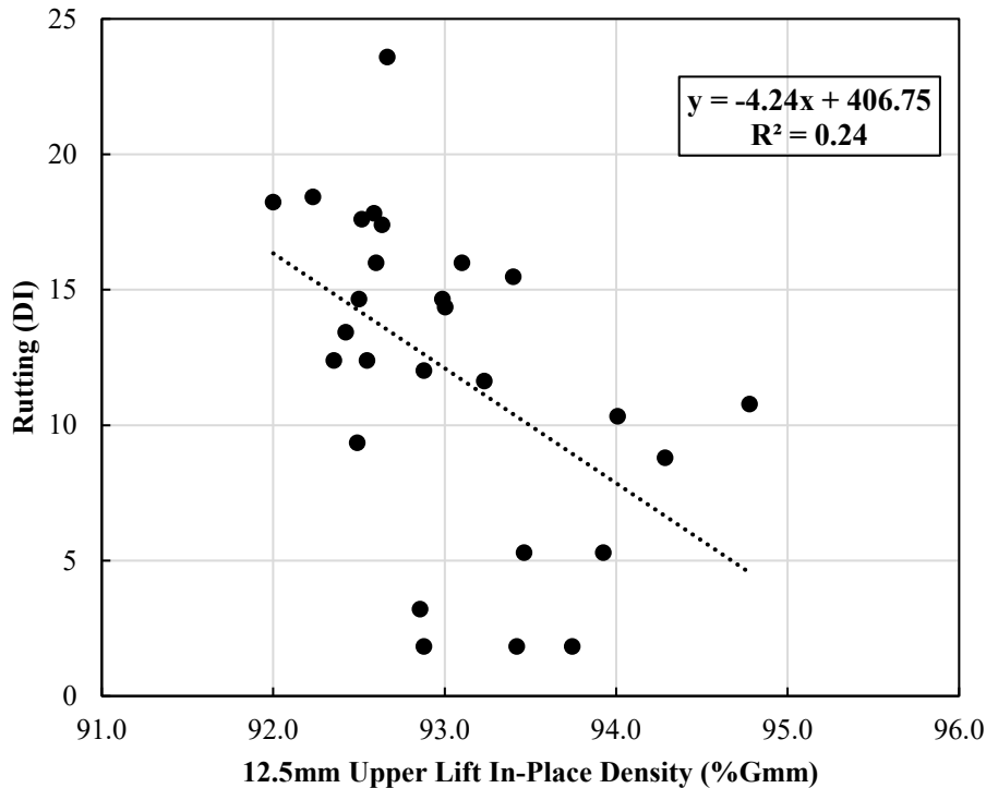
Figure 3-19 Rutting Against the In-Place Density of the 12.5mm Mixes
