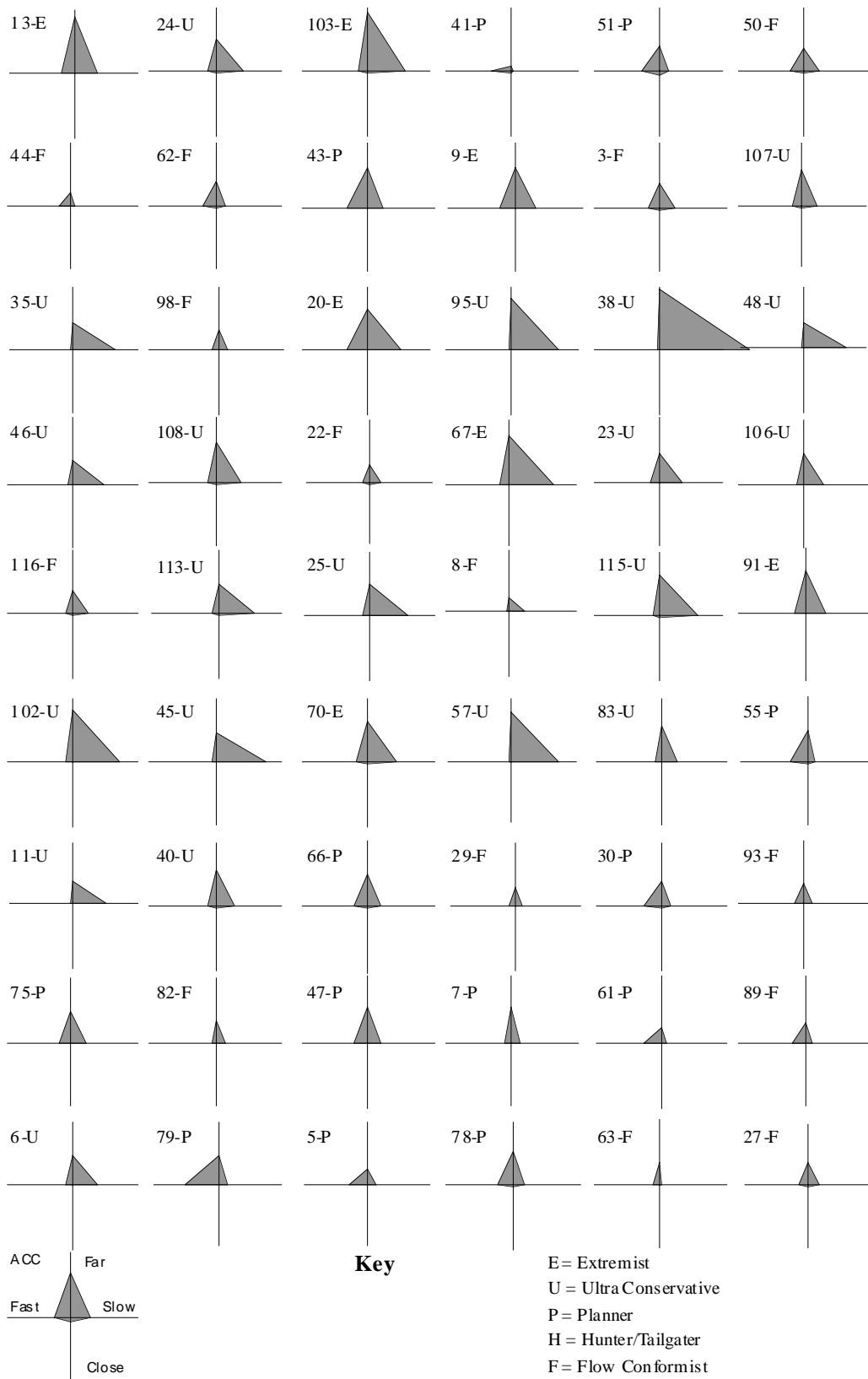
Figure 102. ACC driving behavior for individual drivers ( V > 55 mph)
