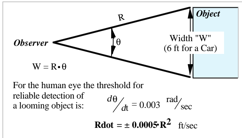
Figure 77. The visual angle, \theta
