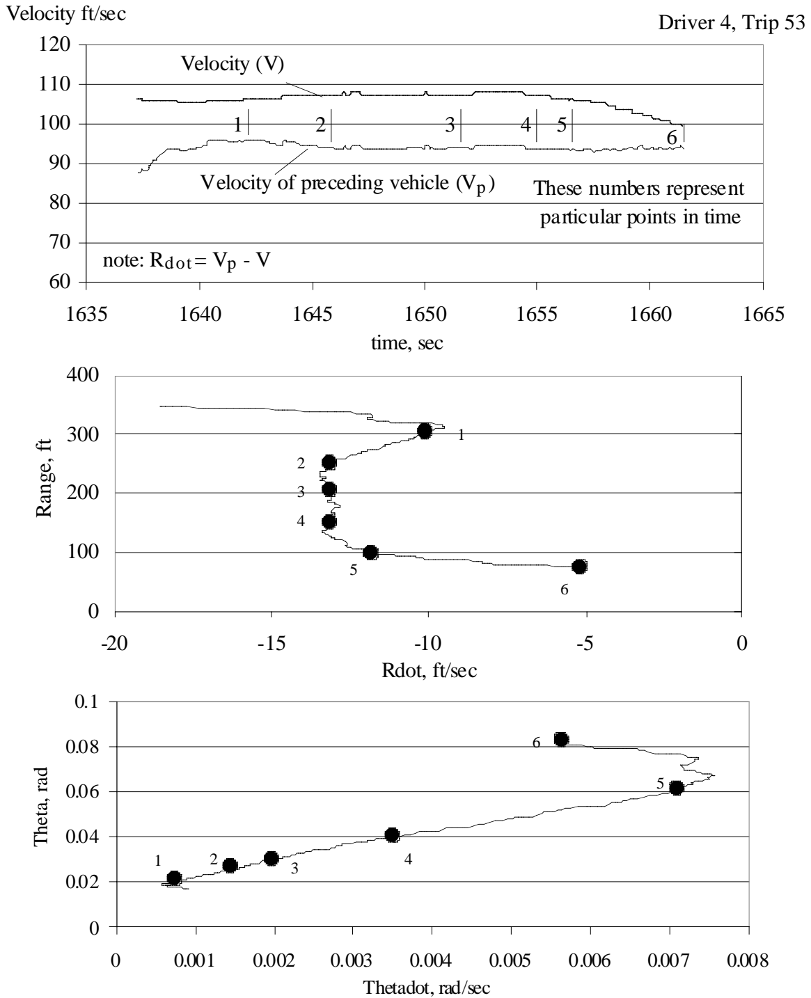
Figure 78. Example points in time displayed in R-vs.- R_{dot} and \theta -vs.- \theta_{dot} spaces
