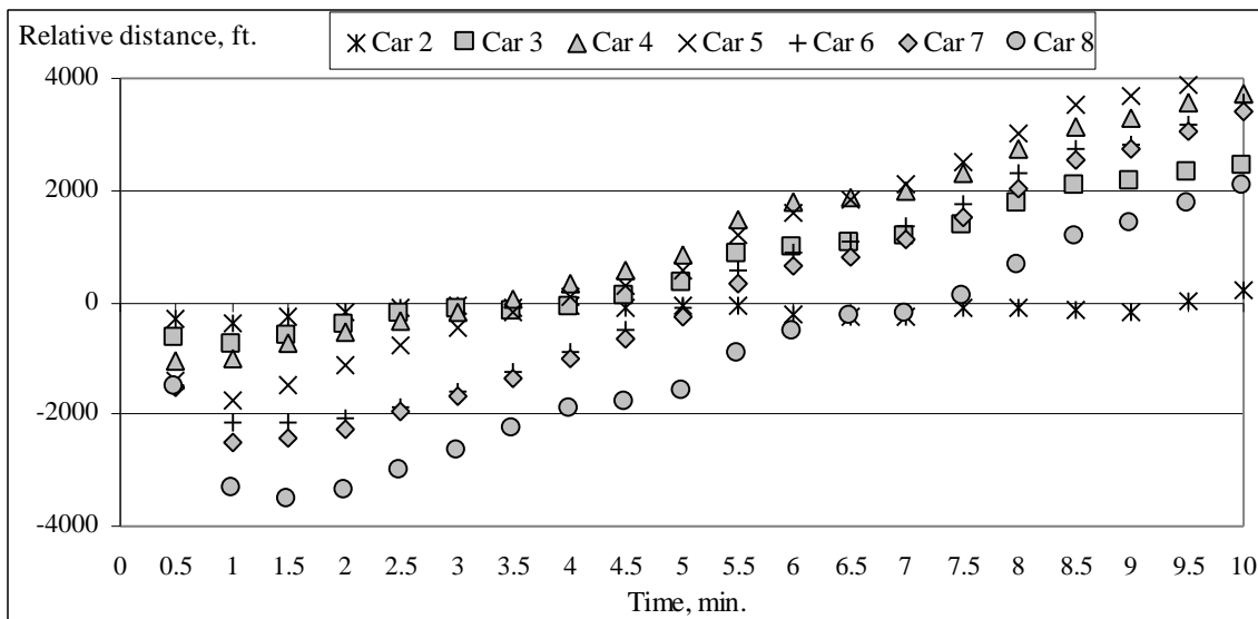
Figure 6. Relative distance during cluster test (Car 1 is baseline)
