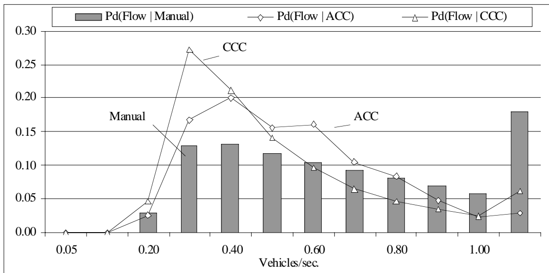
Figure 180. Frequency distribution of Flow in manual and ACC driving
