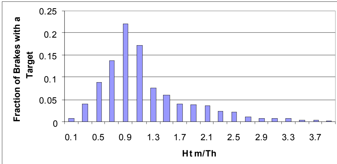
Figure 157. Normalized prevailing headway time during braking ( V > 55 mph)
