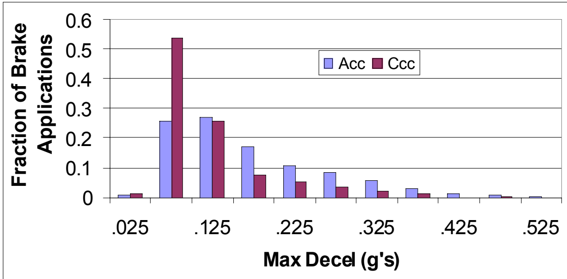
Figure 148. Maximum deceleration during braking (V>55mph)
