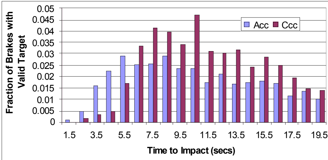
Figure 153. Time to Impact during braking ( V > 55 mph)
