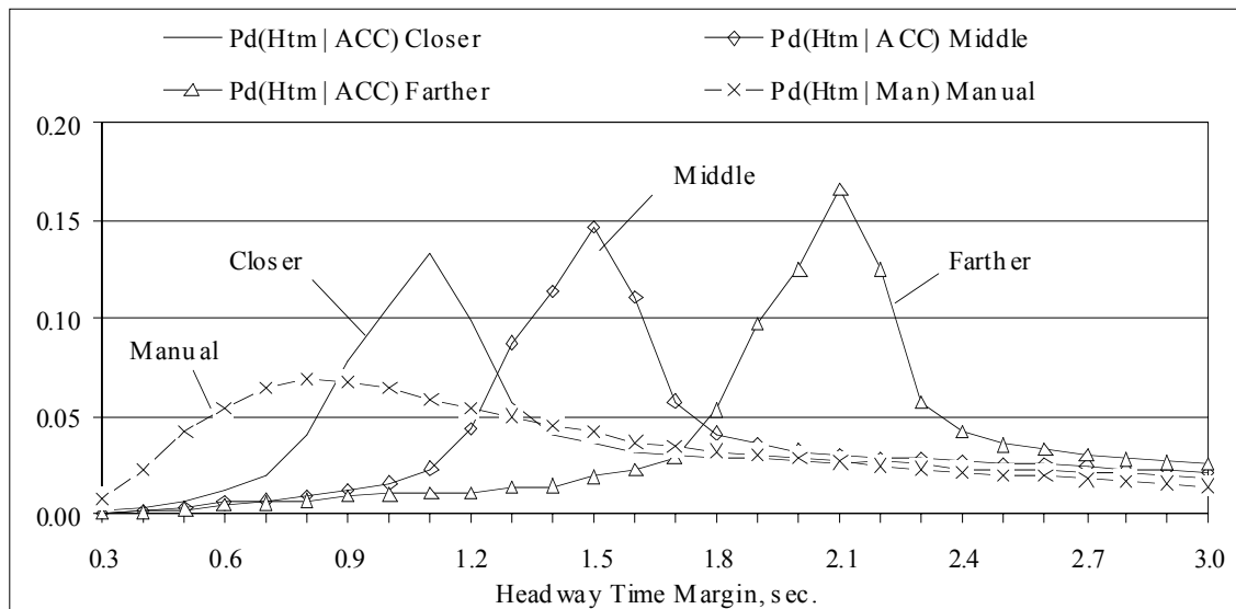
Figure 108. Comparison of ACC to manual driving using headway time margin, V > 55 mph
