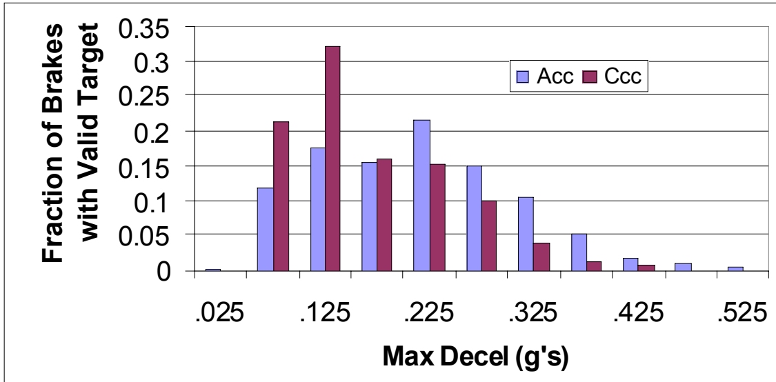
Figure 151. Maximum deceleration during braking, target present (V<55mph)
