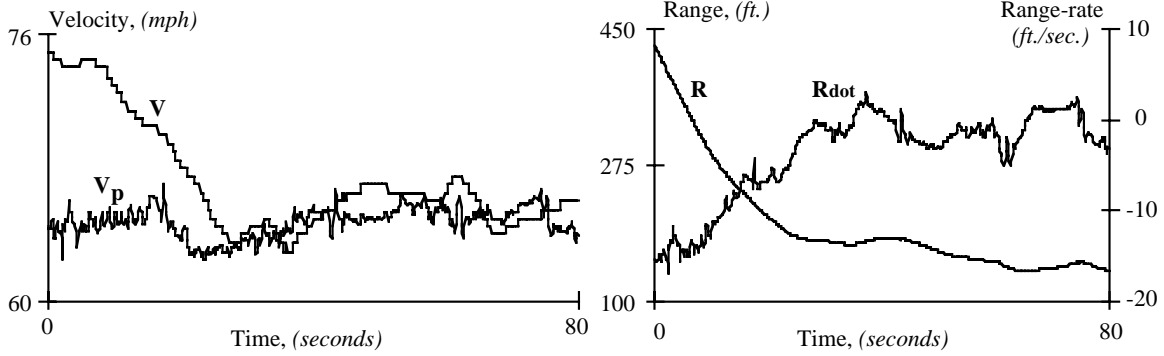
Figure 118. An example target stream illustrating closing and following operation during manual driving
