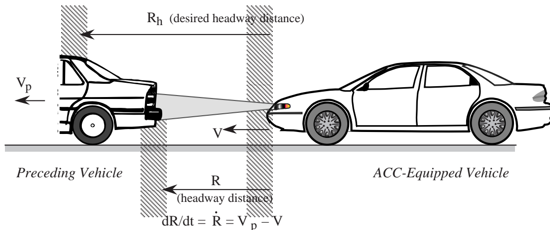
Figure 7. Headway control
