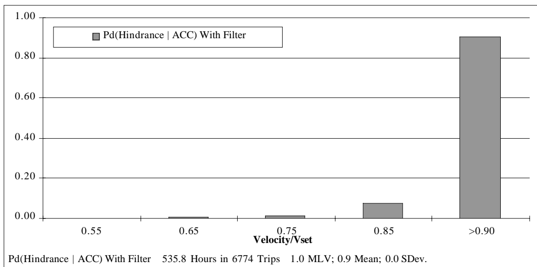
Figure 183. Frequency distribution of Hindrance in CCC and ACC driving
