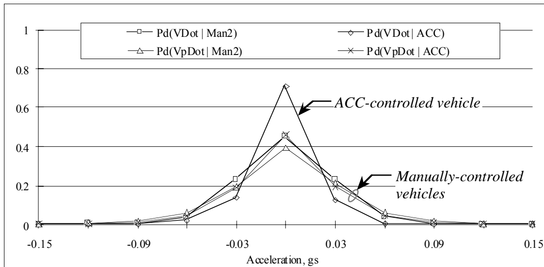
Figure 184. Frequency distribution of acceleration in manual and ACC driving
