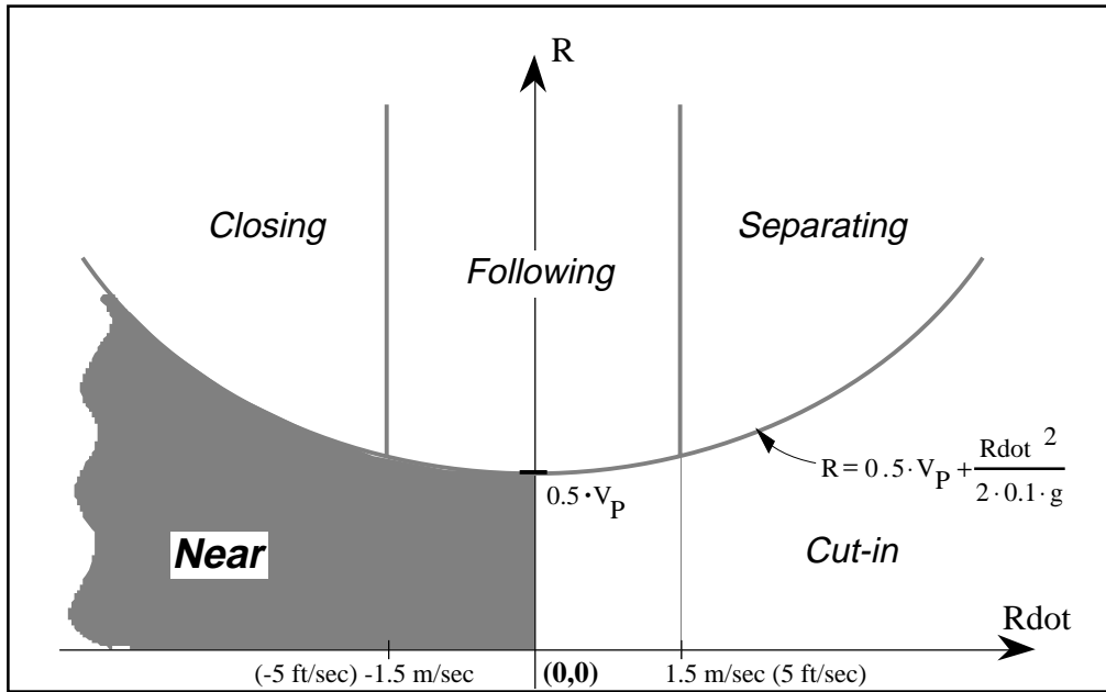
Figure 44. Near region in the range-versus-range-rate space
