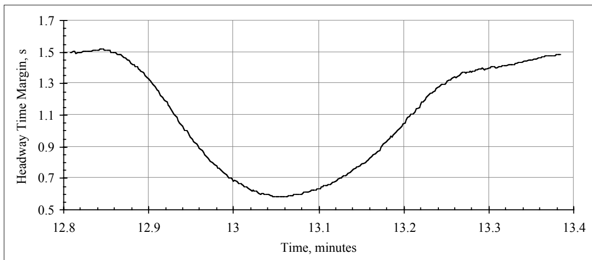
Figure E-8. Headway Time Margin versus time, manually accelerating
