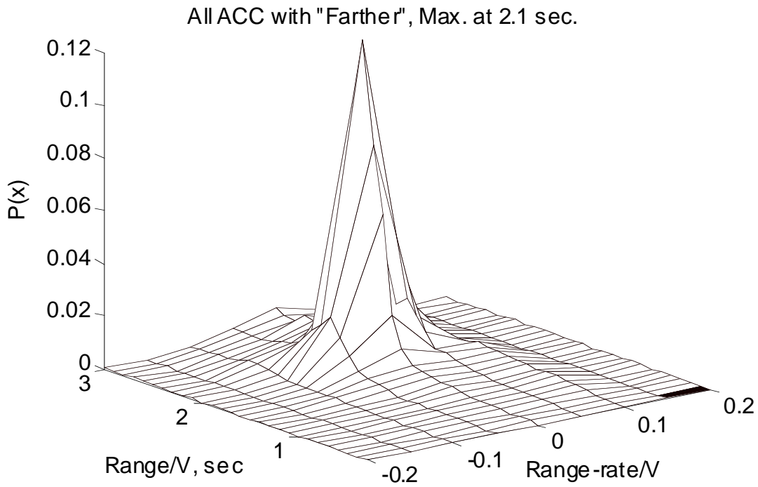
Figure 114. R/V versus Rdot/V for ACC driving with T_h = 2.1 sec. ( V > 55 mph)
