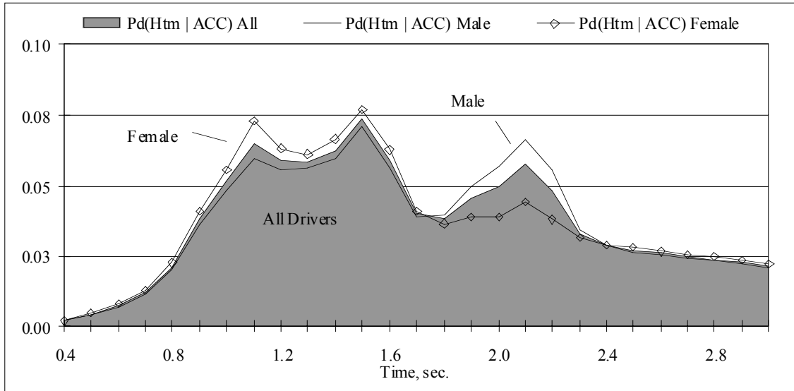
Figure 101. Distribution of headway time margin under ACC by driver gender
