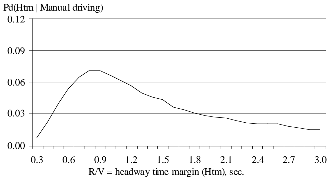
Figure 72. Htm for manual driving with V > 55 mph
