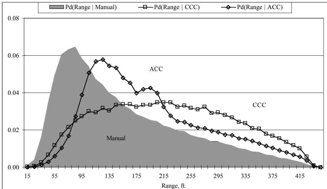
Figure 182. Frequency distribution of Range in manual and ACC driving
