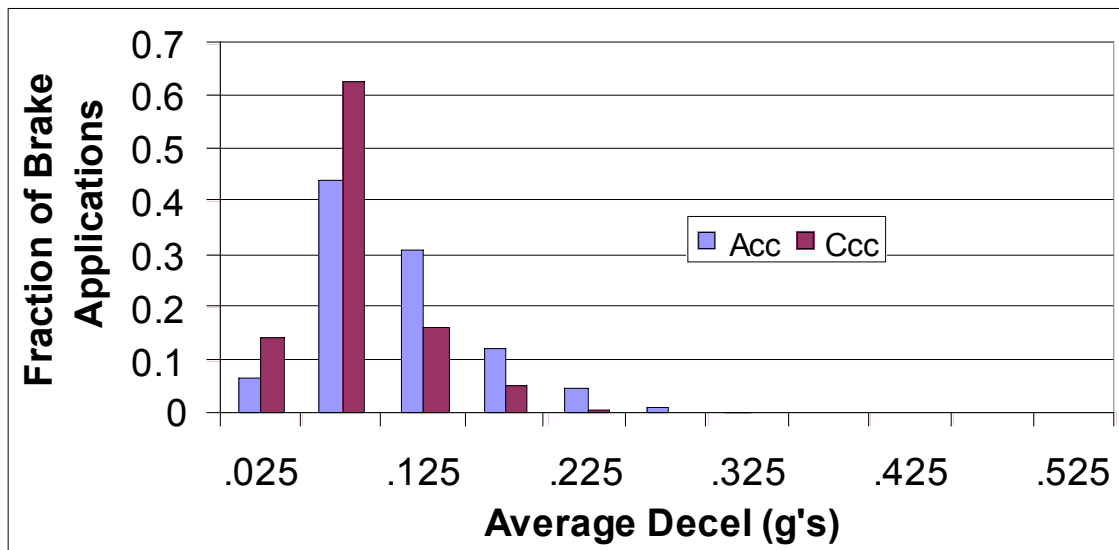
Figure 147. Average deceleration during braking (V>55mph)
