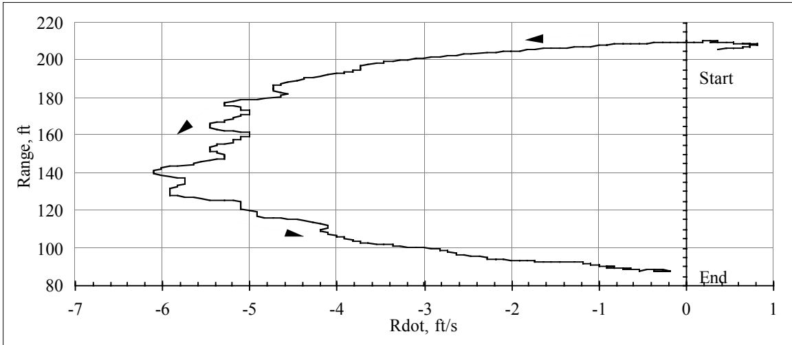
Figure E-3. Range versus Range-Rate, changing from T_h = 2.0 to 1.0 s
