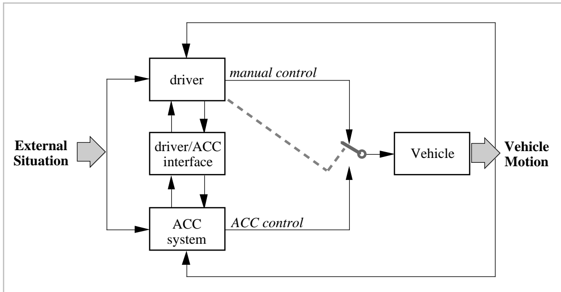
Figure 98. Overview of control supervision in ACC driving
