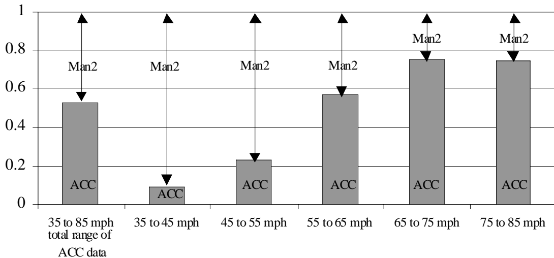
Figure 79. ACC and manual (MAN2) utilization vs. velocity
