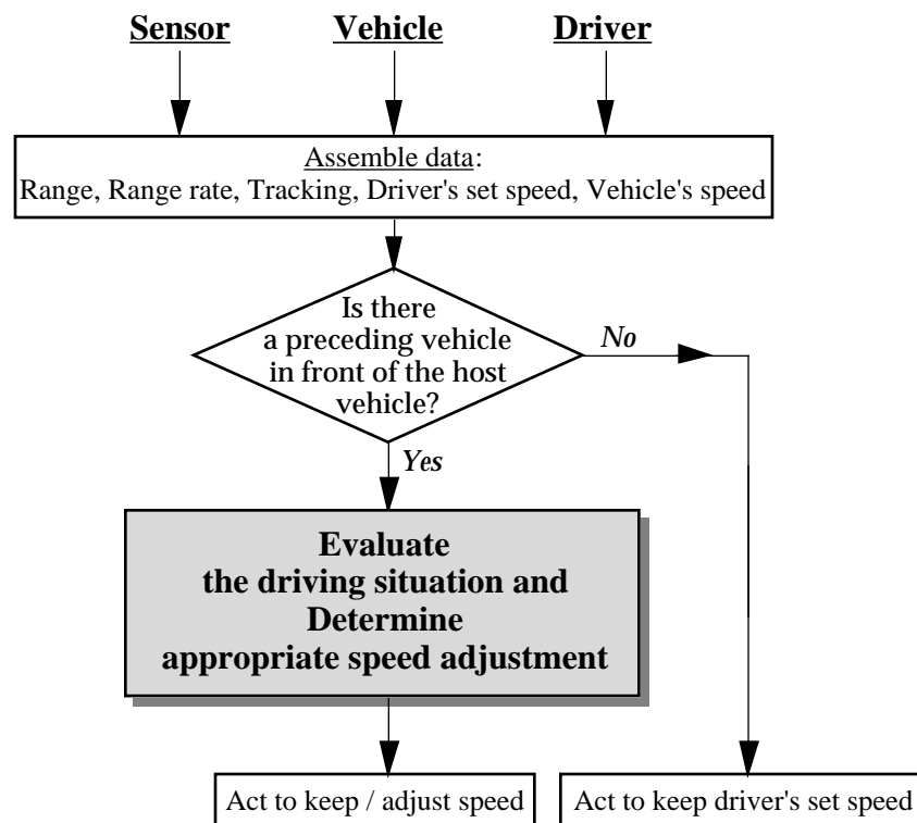
Figure 6. Employing speed to control headway
