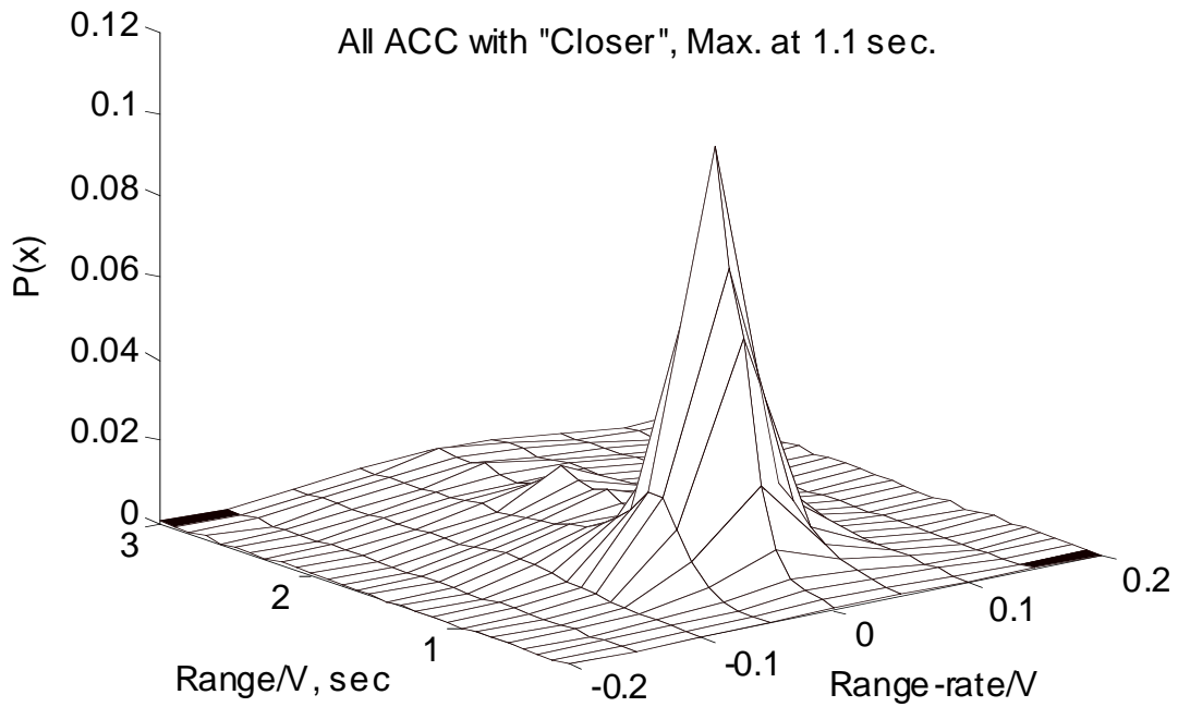
Figure 112. R/V versus Rdot/V for ACC driving with T_h = 1.1 sec. ( V > 55 mph)
