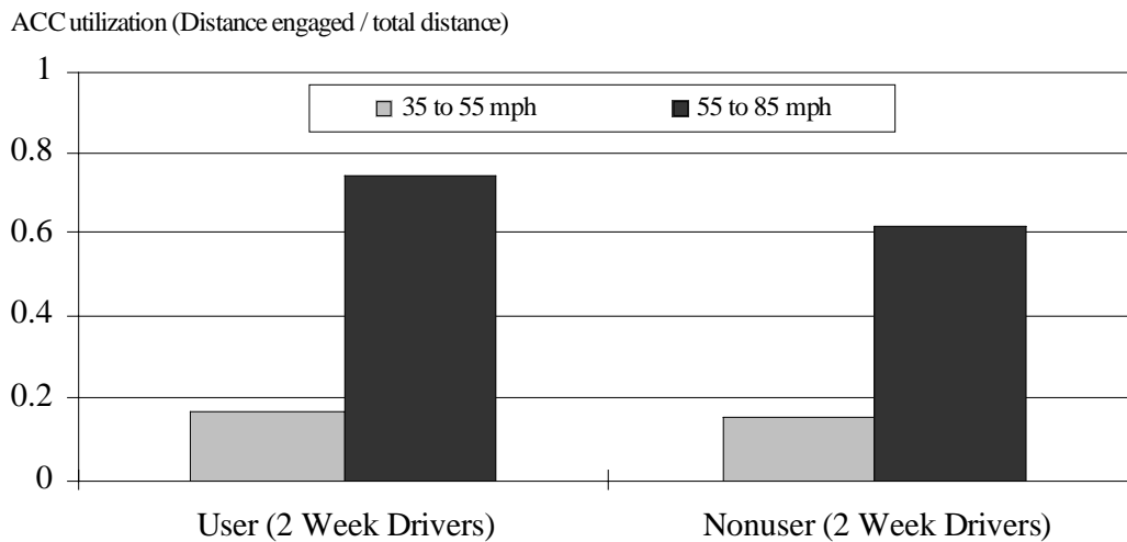
Figure 132. ACC utilization for users and nonusers
