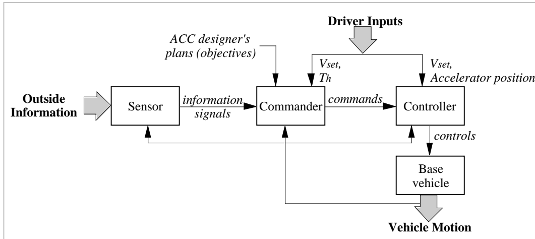
Figure 96. Diagram of the controlled system during ACC operation
