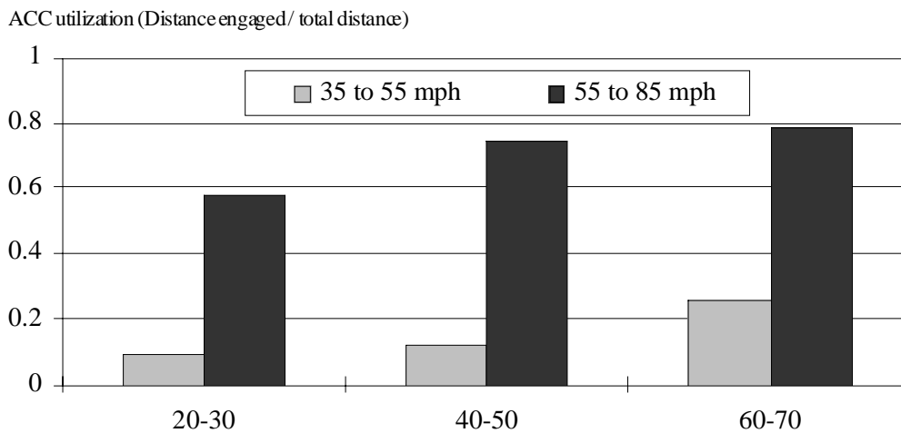
Figure 131. Influence of driver age on ACC utilization
