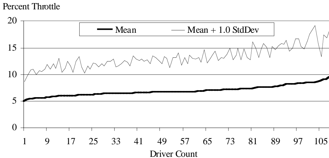
Figure 71. Mean and standard deviation of throttle setting by driver
