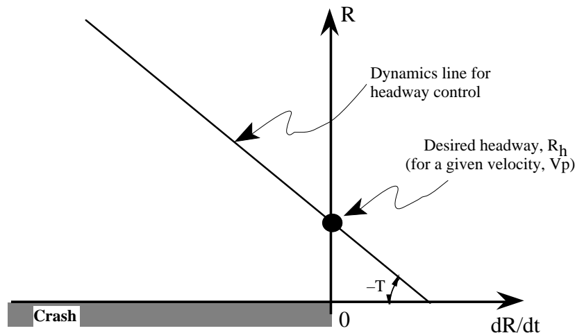
Figure 8. Range rate versus range
