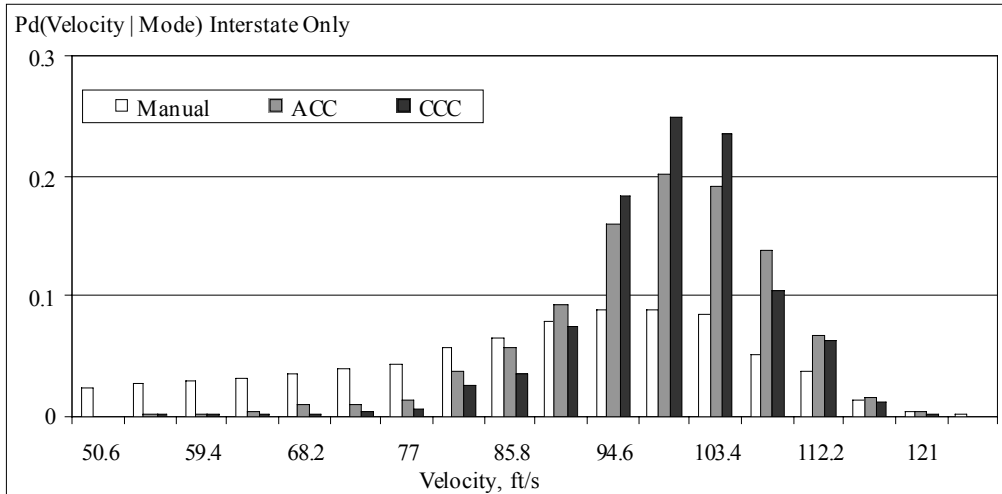
Figure 181. Frequency distribution of traffic speed ( V_p ) in manual and ACC driving
