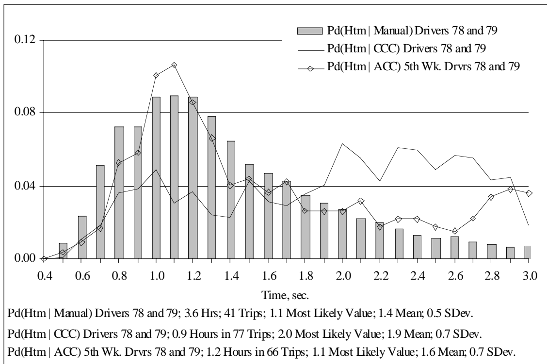
Figure 173. Headway time histograms for drivers 78 and 79 over all their fifth-week driving
