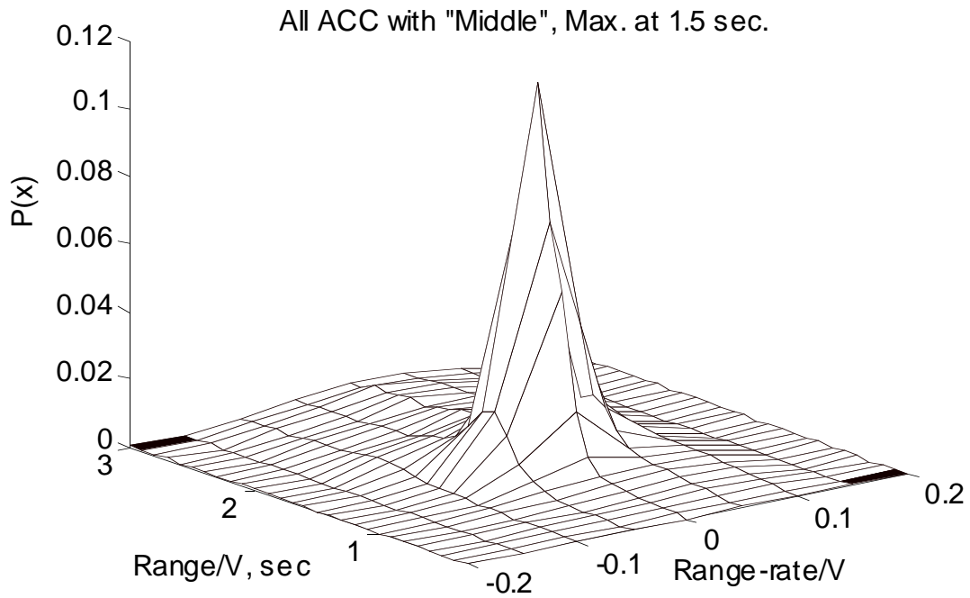
Figure 113. R/V versus Rdot/V for ACC driving with T_h = 1.5 sec. ( V > 55 mph)
