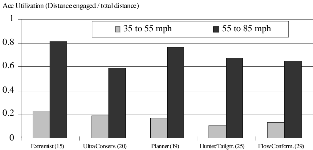
Figure 134. ACC utilization for different driving styles
