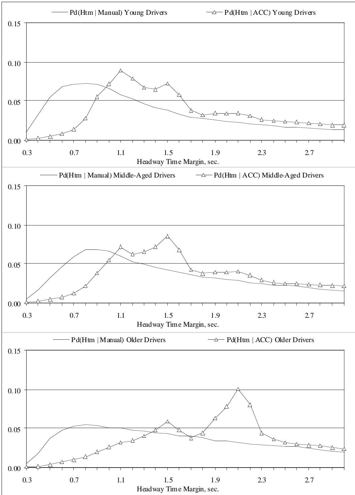
Figure 177. Htm shift between manual and ACC driving as a function of age
