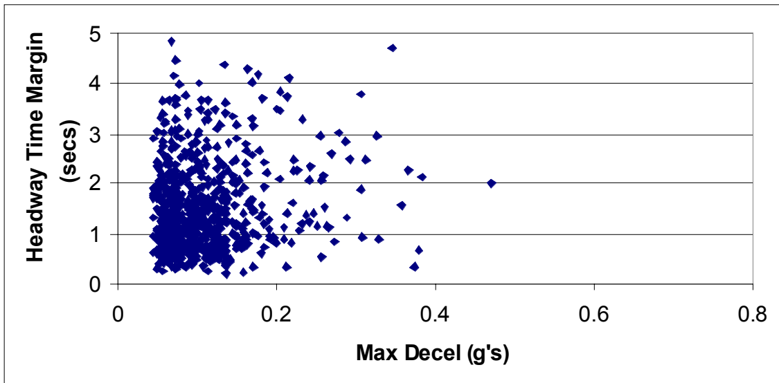
Figure 179. CCC disengagements via braking
