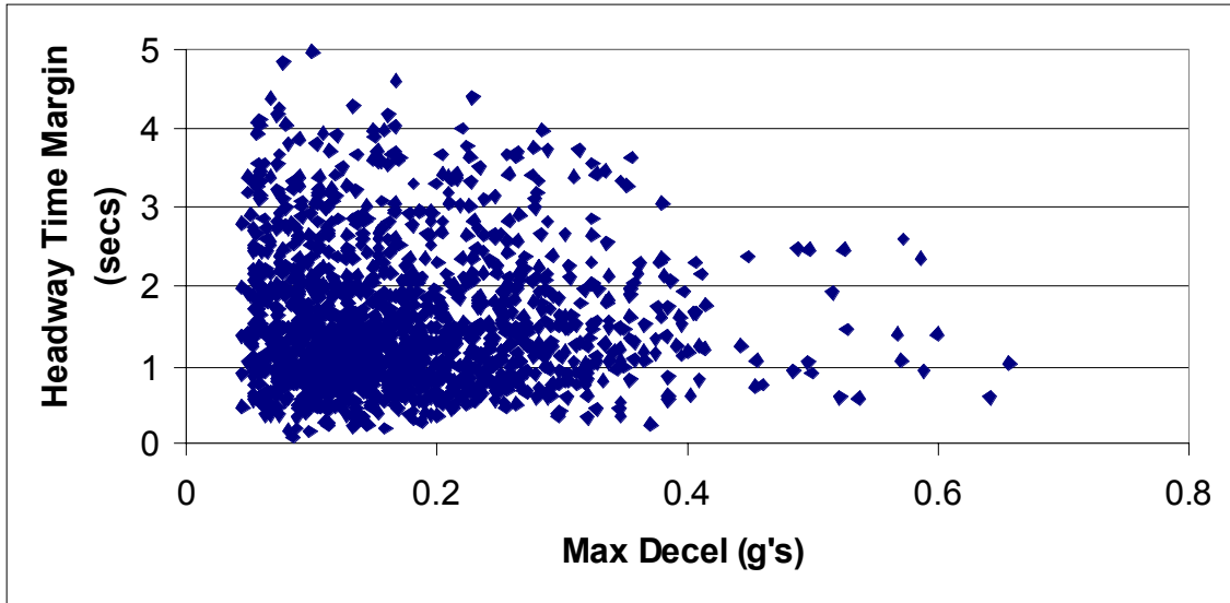
Figure 178. ACC disengagements via braking
