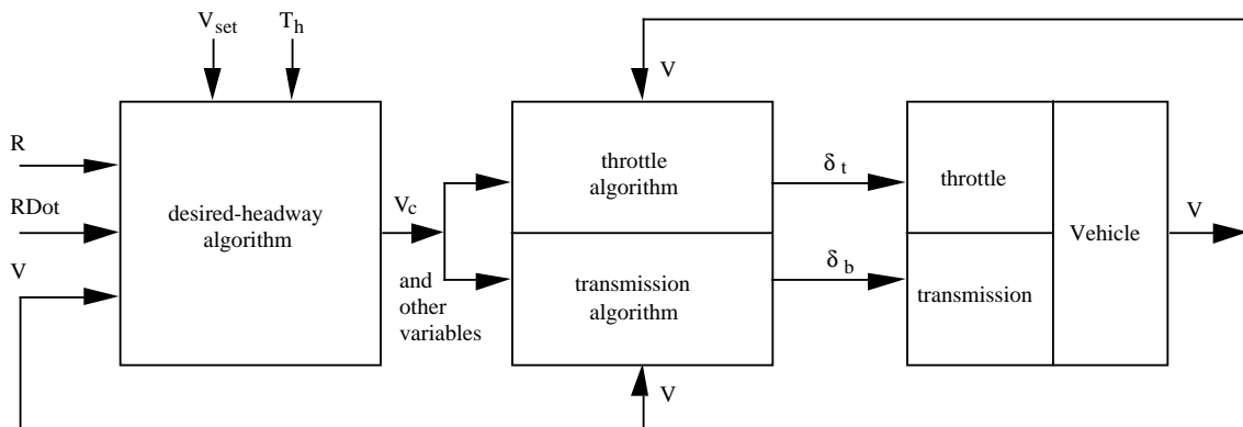
Figure 10. Control architecture for FOT ACC system
