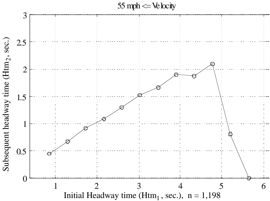
Figure 162. Average Htm 2 at cut-in vs. Htm 1 prior to cut-in, high speed
