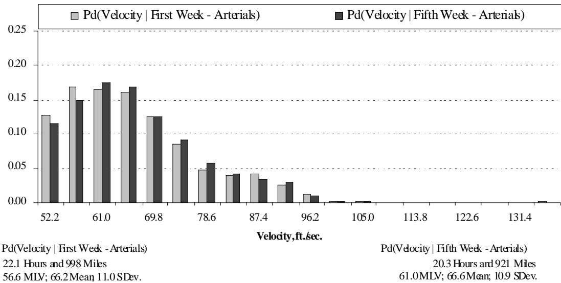
Figure 170. Velocity histogram for the first week and fifth week of five-week drivers on arterial roads
