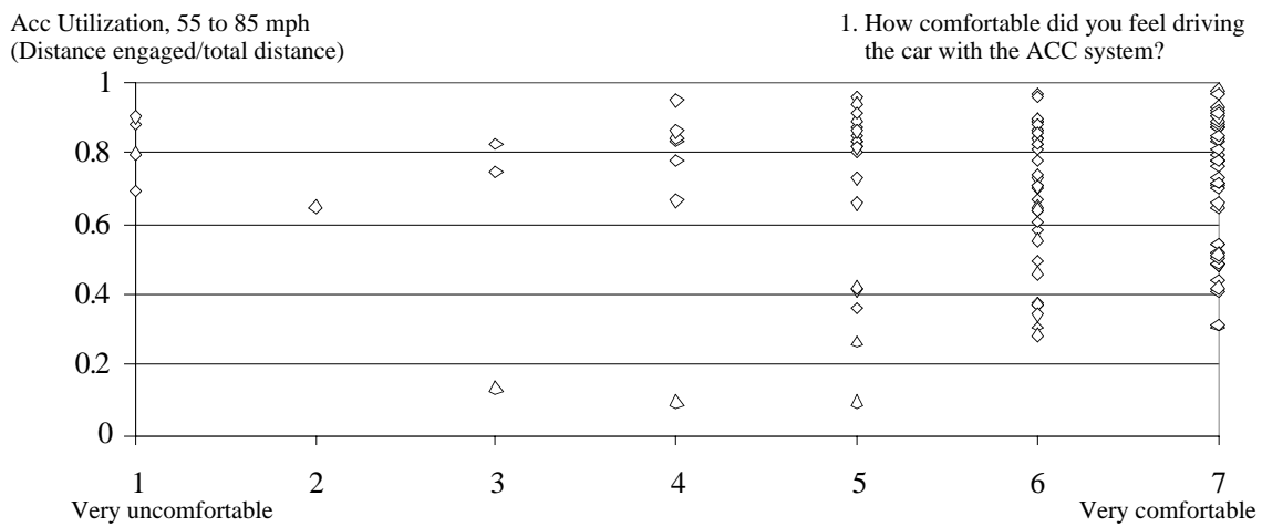
Figure 137. ACC utilization and driver comfort
