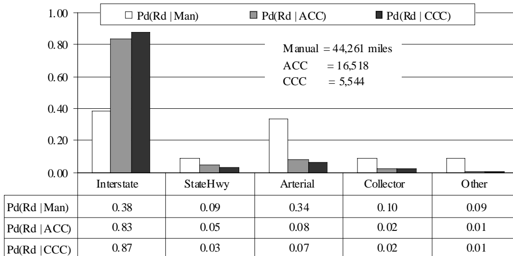
Figure 66. Frequency of road type for the three different driving modes
