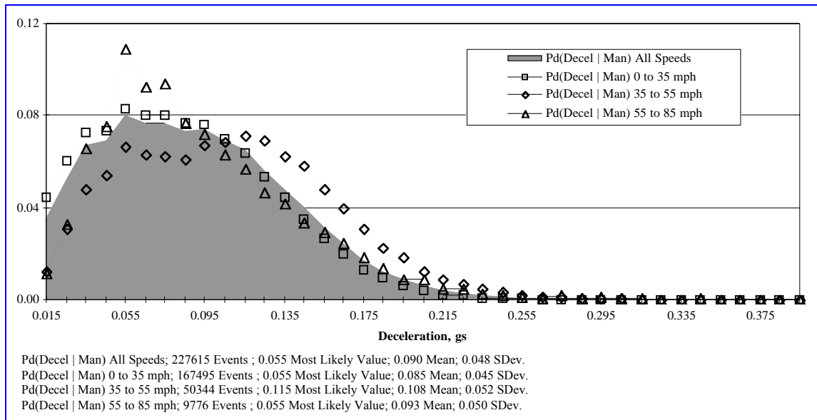
Figure 90. Average deceleration in manual braking events (duration > 0.3 seconds)
