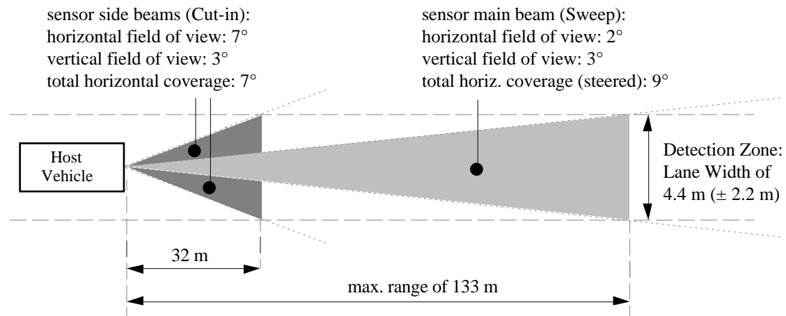
Figure 4. ODIN4 sensors coverage areas
