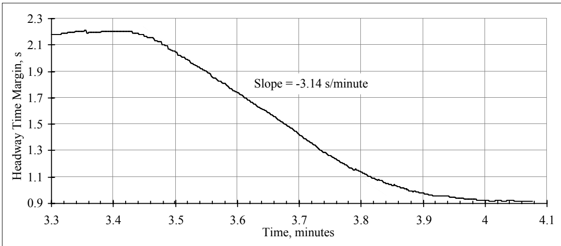
Figure E-4. Headway Time Margin ( H_{tm} ) versus time, changing from T_h = 2.0 to 1.0 s
