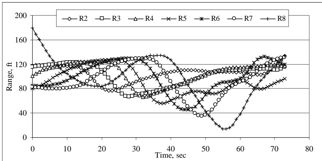
Figure 5. Range time history of seven FOT vehicles in a string, following a longitudinal disturbance
