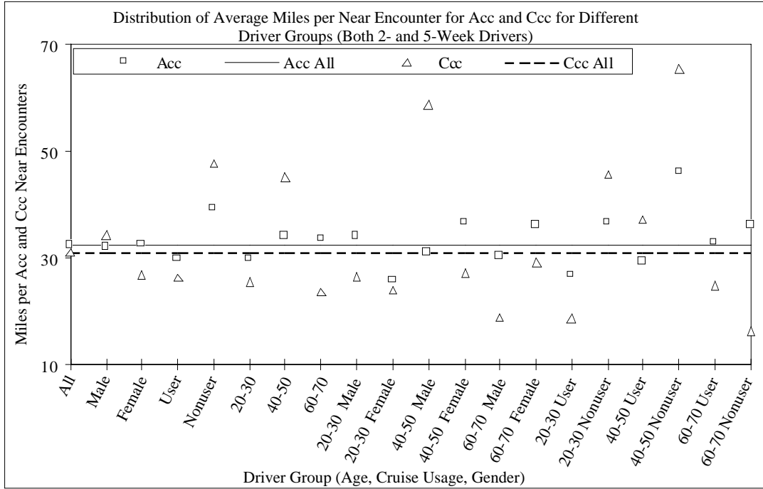
Figure 105. ACC near encounters per mile
