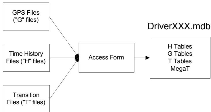
Figure 33. Driver Database Loading
