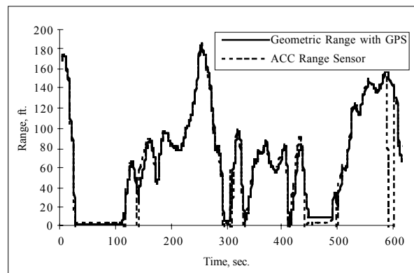
Figure 49. GPS Time history example
