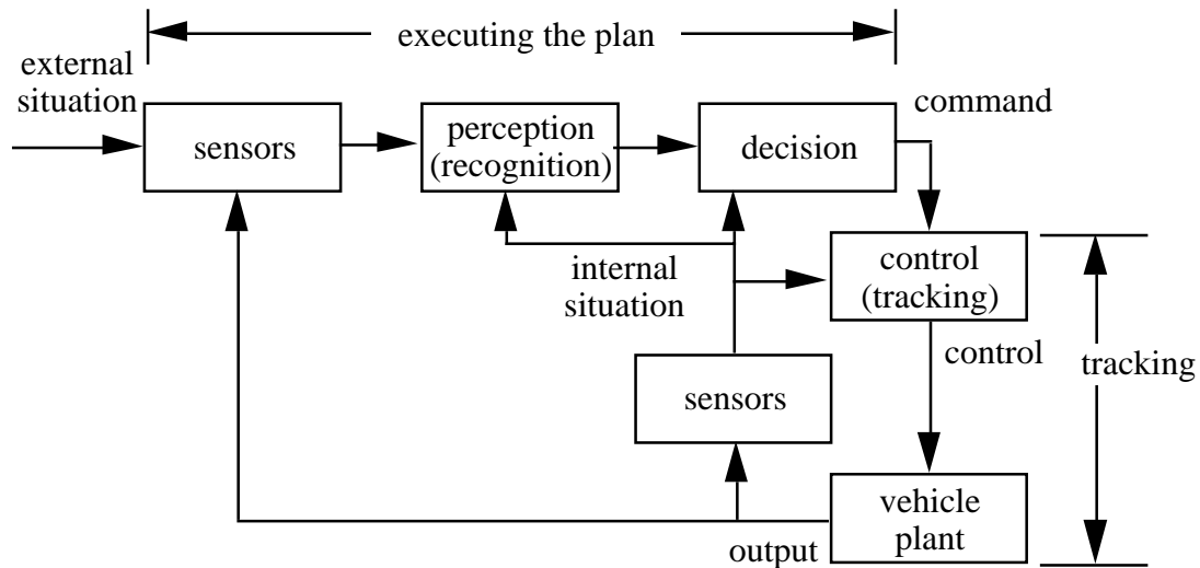
Figure 73. Conceptual portrayal of the elements of the driving process
