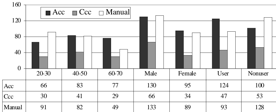
Time for 5 Week Drivers, hours (Velocity > 55 mph)
