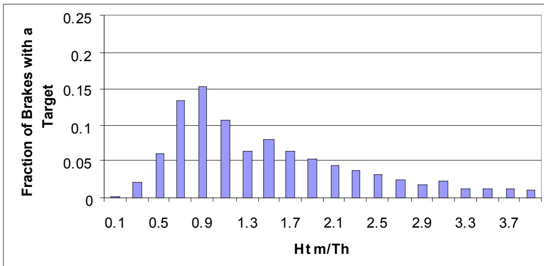
Figure 158. Normalized prevailing headway time during braking ( V < 55 mph)
