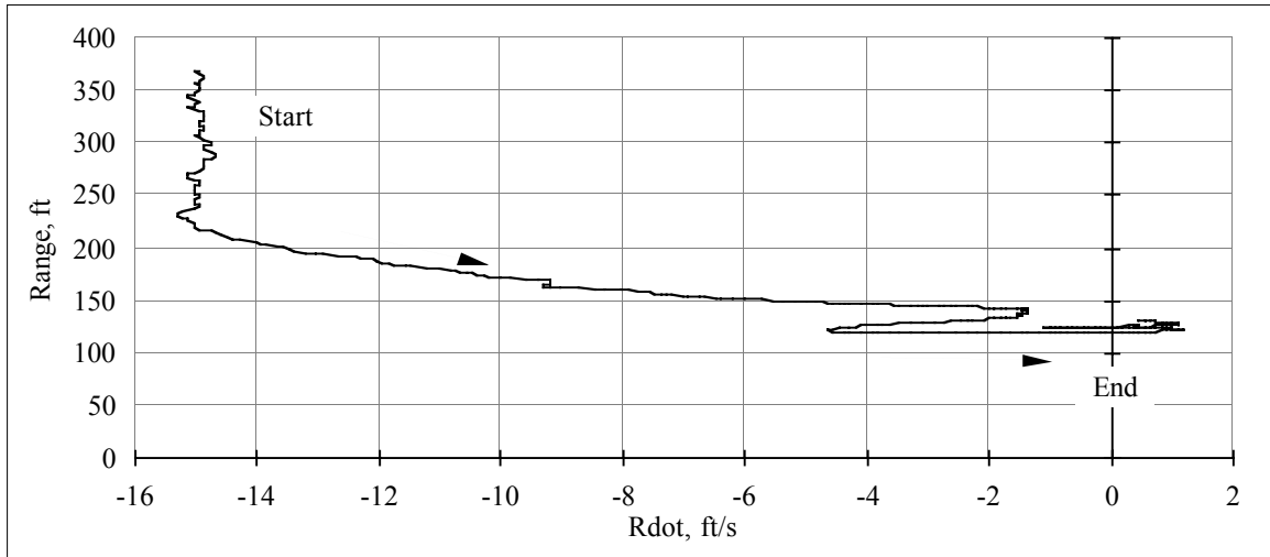
Figure E-1. Range versus Range-Rate, closing from long range
