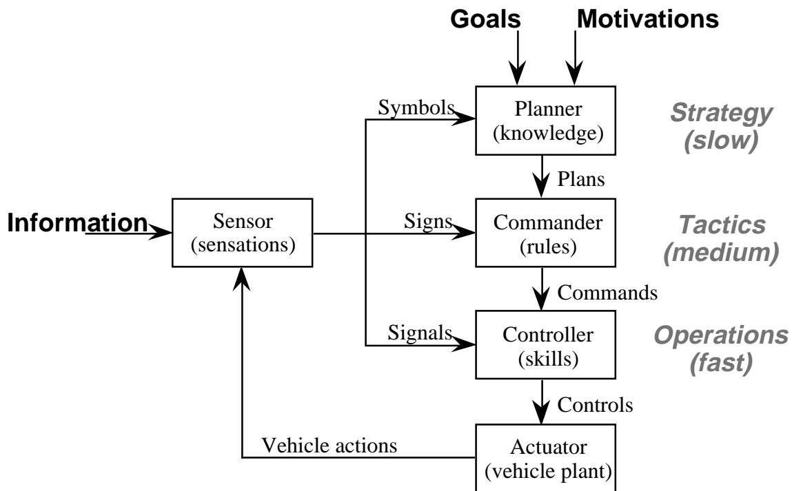
Figure 186. Simplified concept of driver-vehicle system
