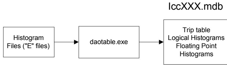
Figure 35. ICC Database Loading
