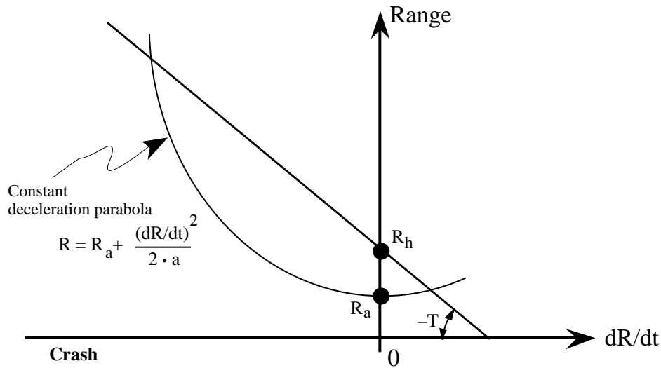
Figure 9. Constant deceleration parabola
