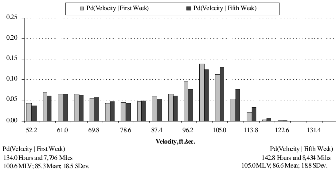
Figure 168. Velocity histogram for the first week and fifth week of five-week drivers
