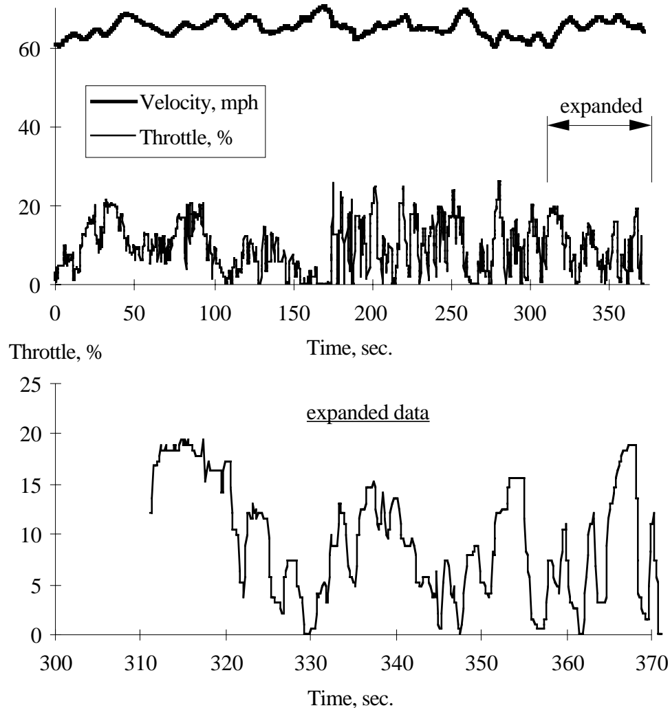
Figure 70. Typical throttle modulation in manual driving
