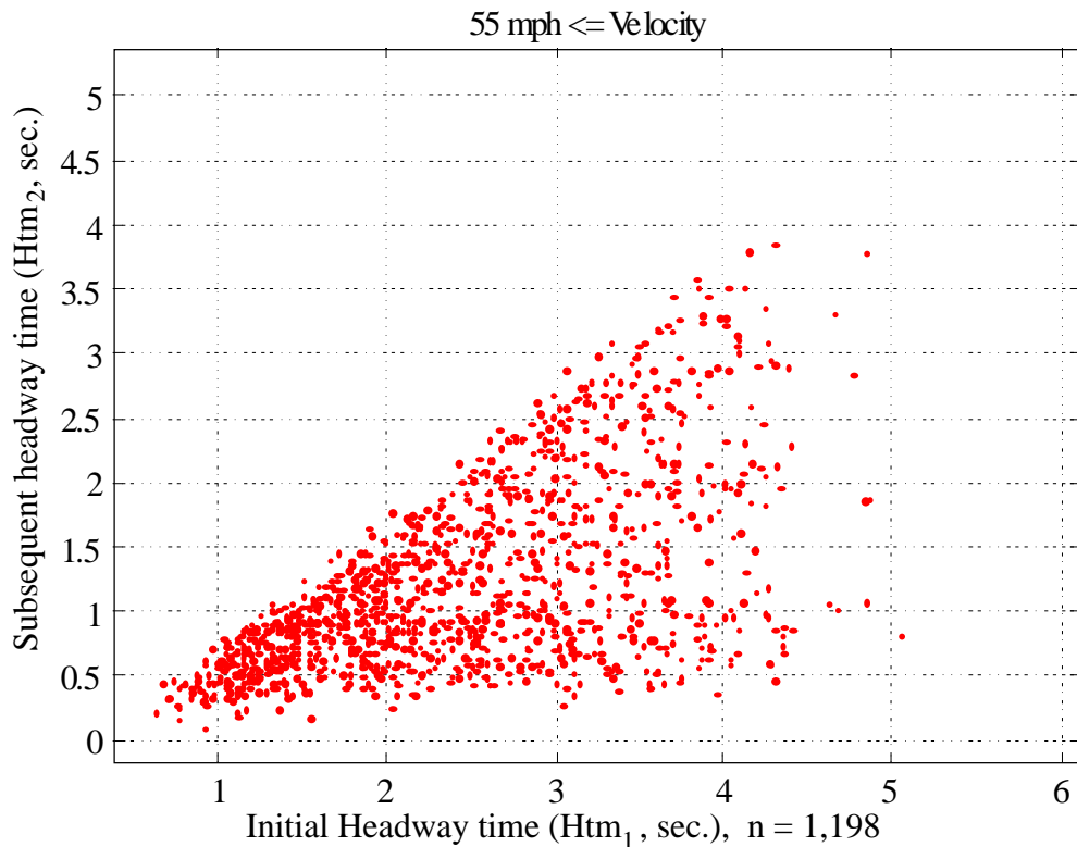
Figure 160. Htm_2 at cut-in vs. Htm_1 prior to cut-in, high speed
