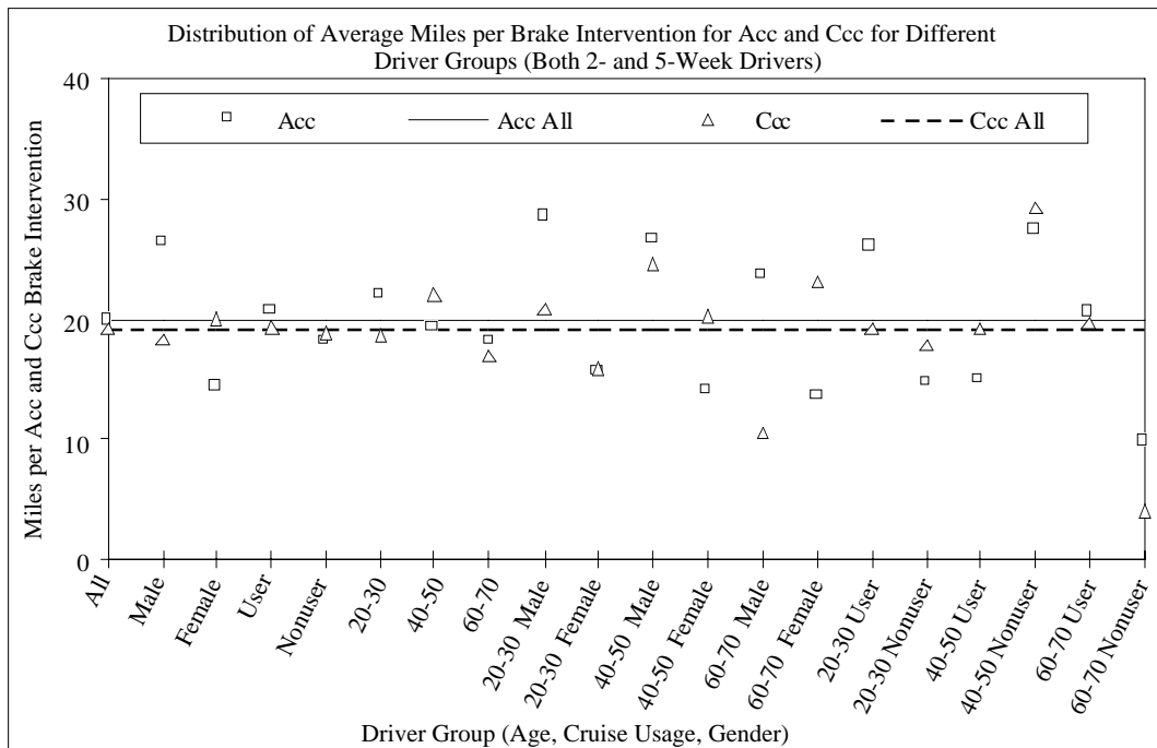
Figure 104. ACC braking per mile
