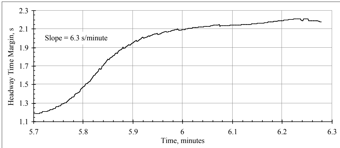
Figure E-6. Headway Time Margin ( H_{tm} ) versus time, changing from T_h = 1.0 to 2.0 s
