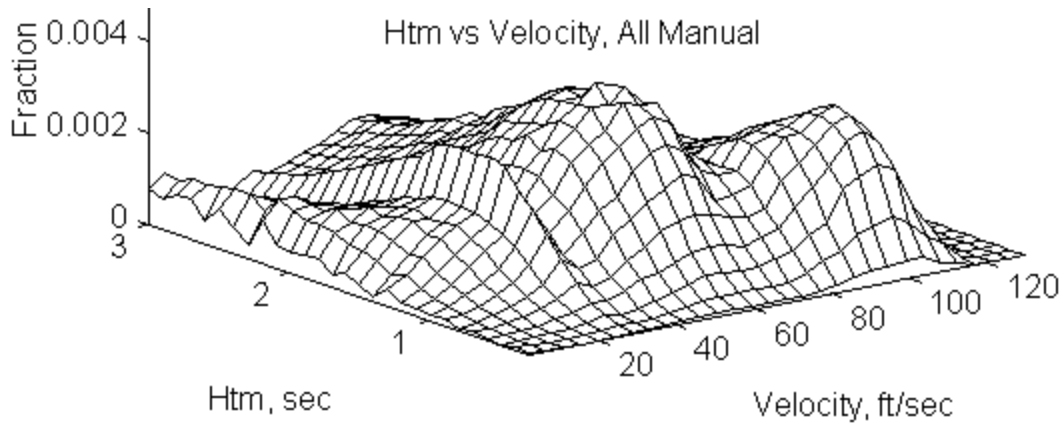
Figure 106. Observed frequencies of headway time margin versus velocity, manual driving
