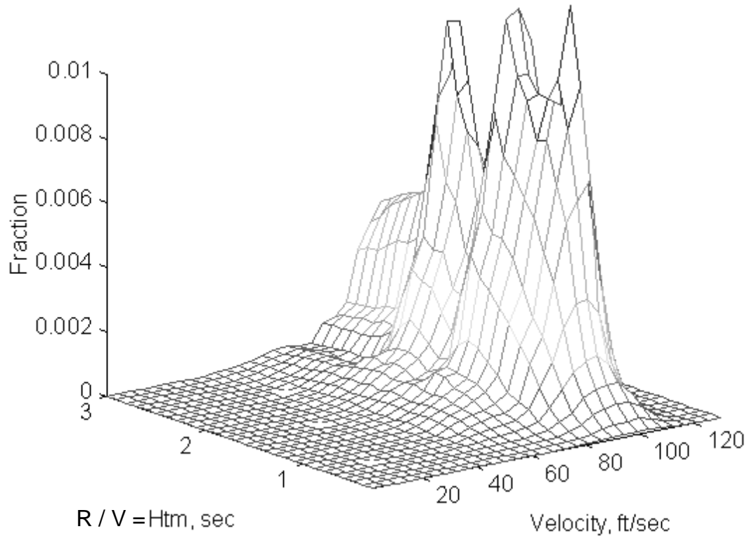
Figure 41. Two-dimensional histogram of velocity and Htm for ACC driving mode
