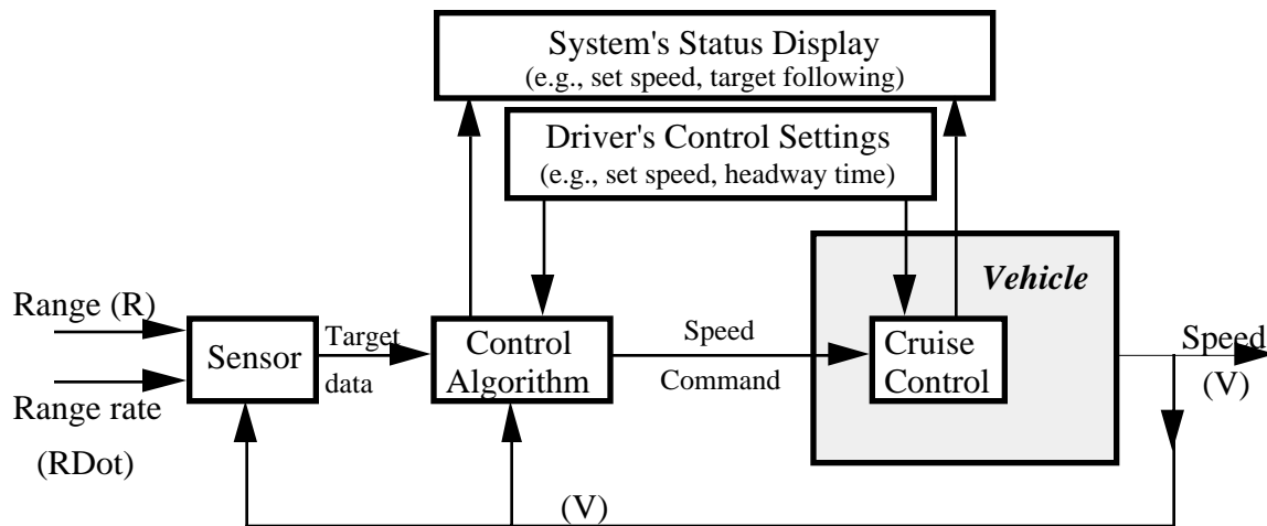
Figure 12. ACC System structure
