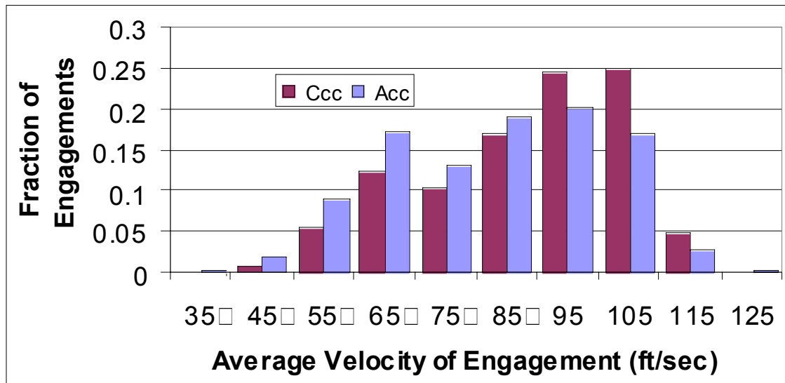
Figure 140. Average engaged velocities
