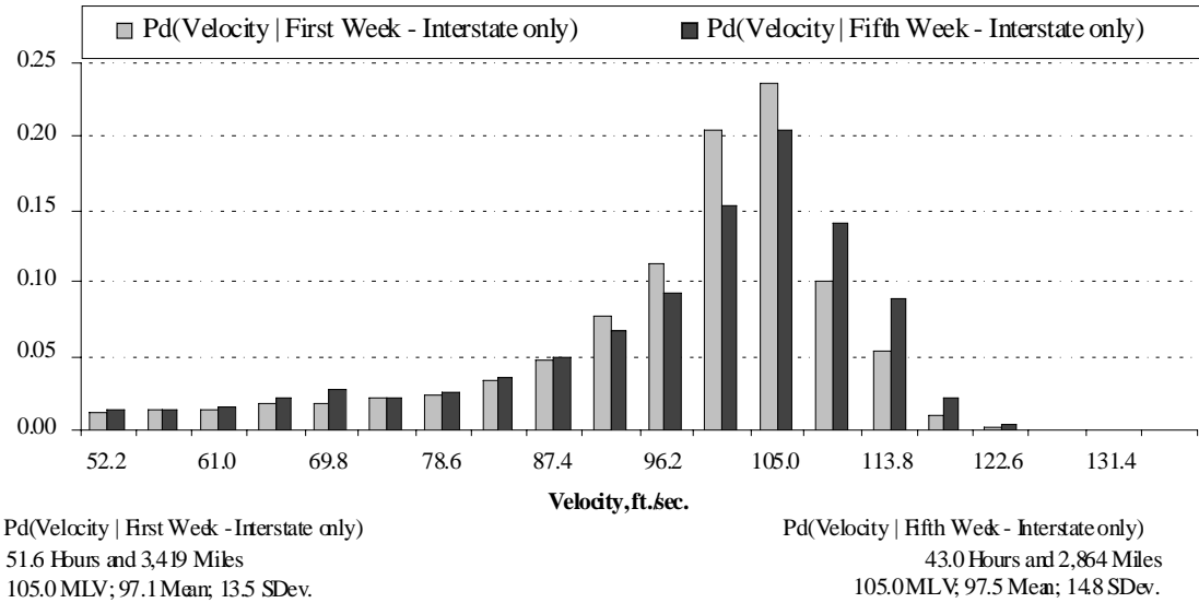
Figure 169. Velocity histogram for the first week and fifth week of five-week drivers on interstate roads
