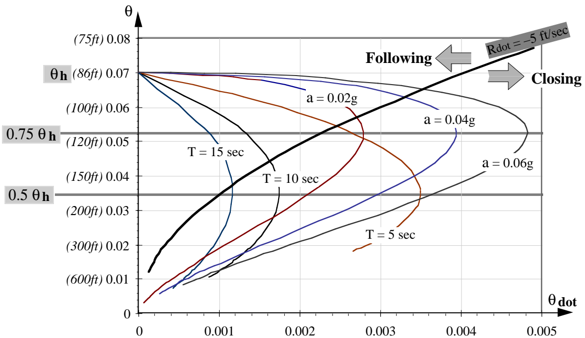
Figure 82. Idealized closing trajectories in \theta vs. \dot{\theta} space
