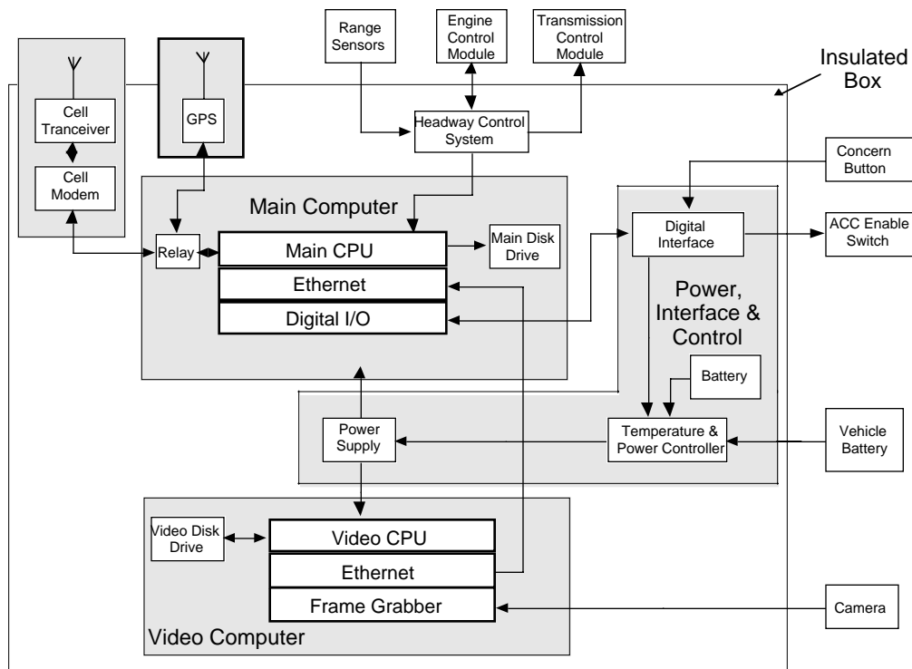
Figure 22. Data-acquisition system hardware
