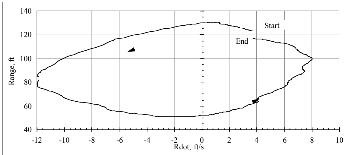
Figure E-7. Range versus Range-Rate, manually accelerating
