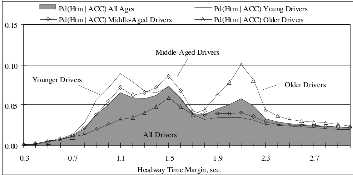
Figure 100. Distribution of headway time margin under ACC by driver age group
