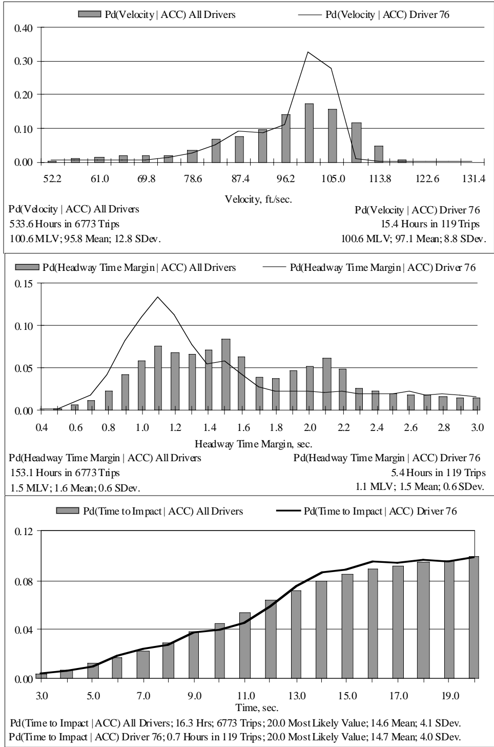
Figure 171. Velocity, Htm, and TTI histograms under ACC for driver 76
