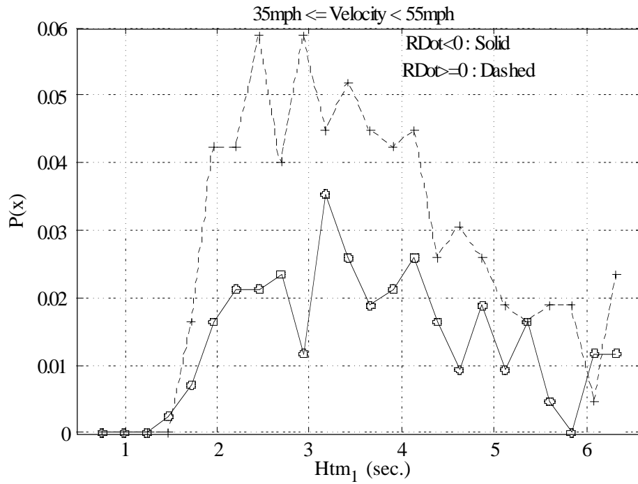
Figure 163. Frequency of cut-in, low speed
