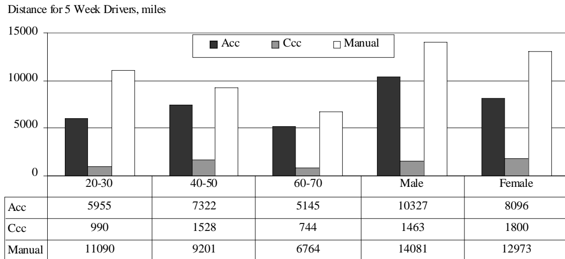
Figure 57. Exposure distance for all velocities
