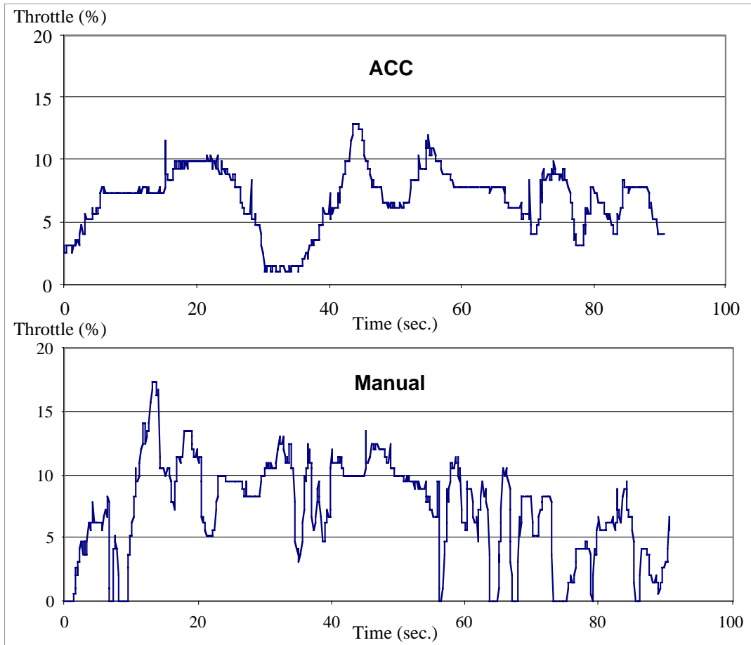
Figure 185. Throttle modulation under ACC and under manual control
