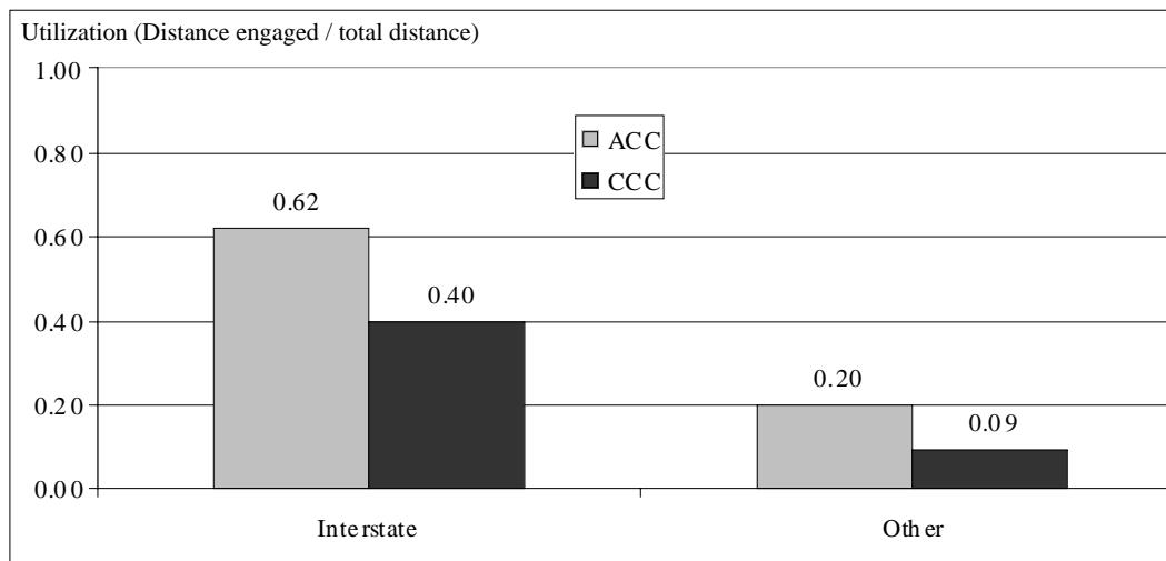
Figure 129. ACC and CCC utilization influenced by road type
