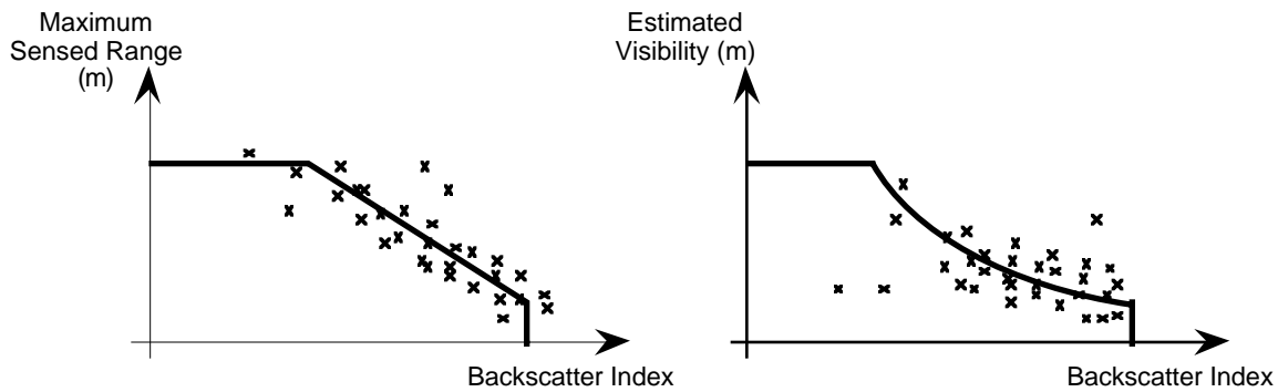
Figure 5. Empirical relationships based on backscatter index
