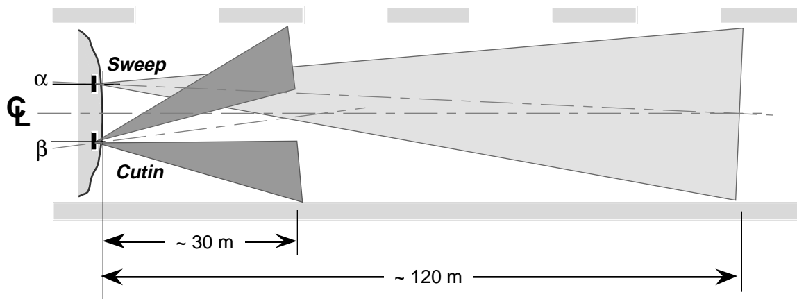
Figure 13. Top view of aligned sensor beams
