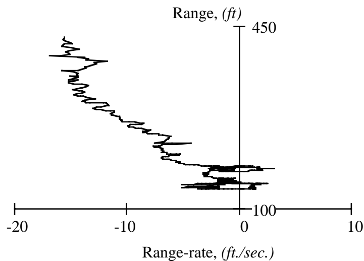
Figure 119. Range vs. range rate during the closing and following sequence of Figure 118
