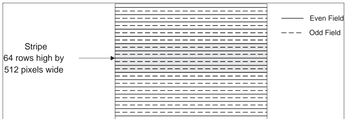
Figure 24. Video image frame structure
