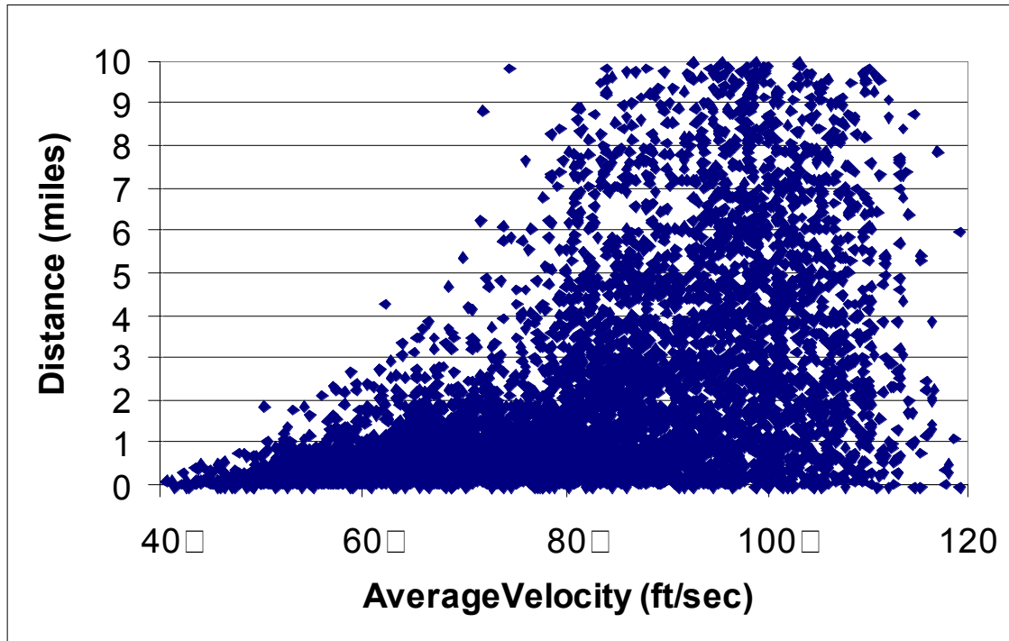
Figure 141. ACC Distance engaged vs. average velocity over the engagement
