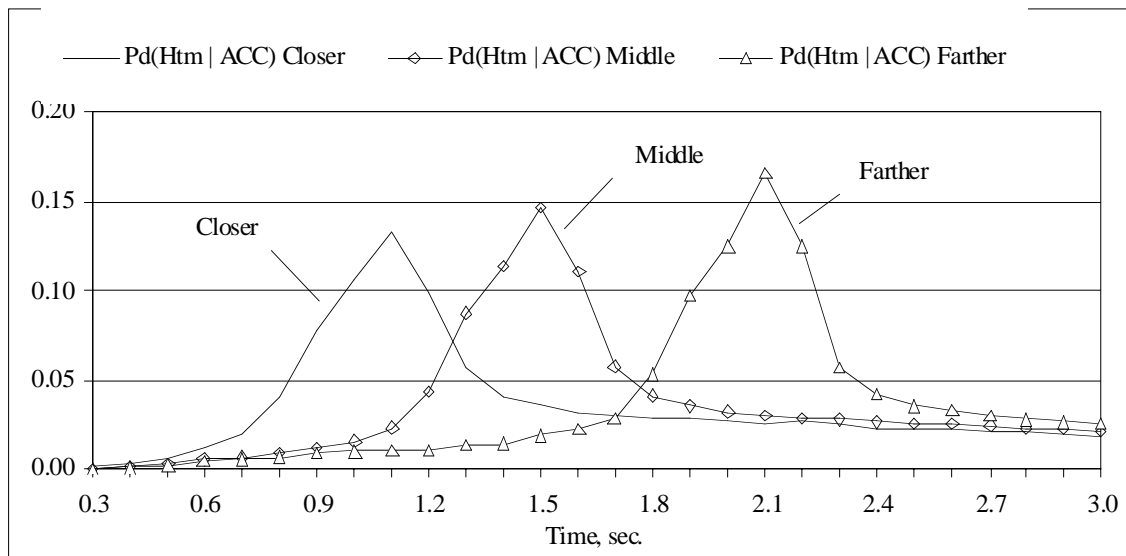
Figure 99. H_{tm} for ACC driving with V > 55 mph
