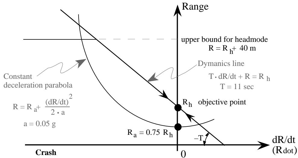
Figure 97. ACC rules built into the commander
