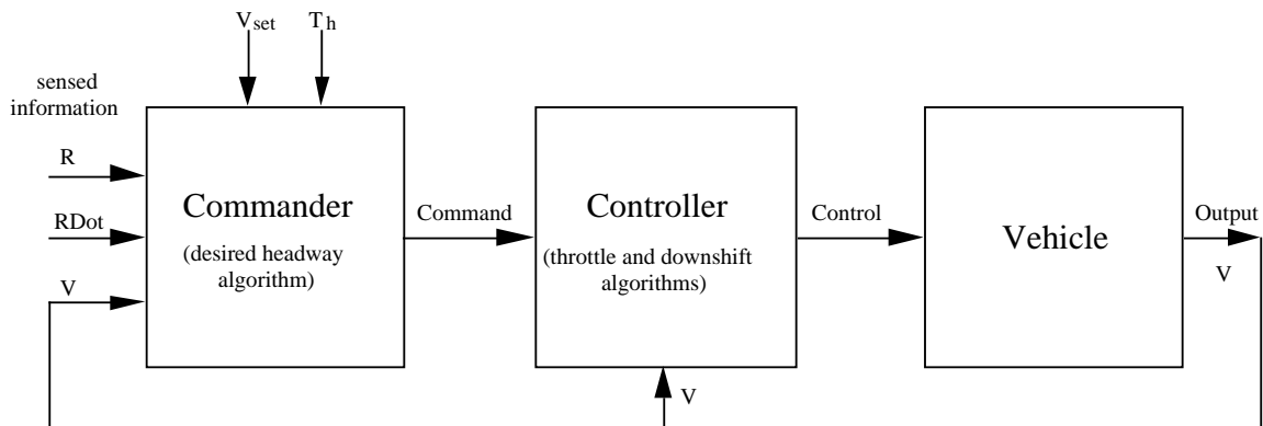
Figure 11. Control architecture with a commander
