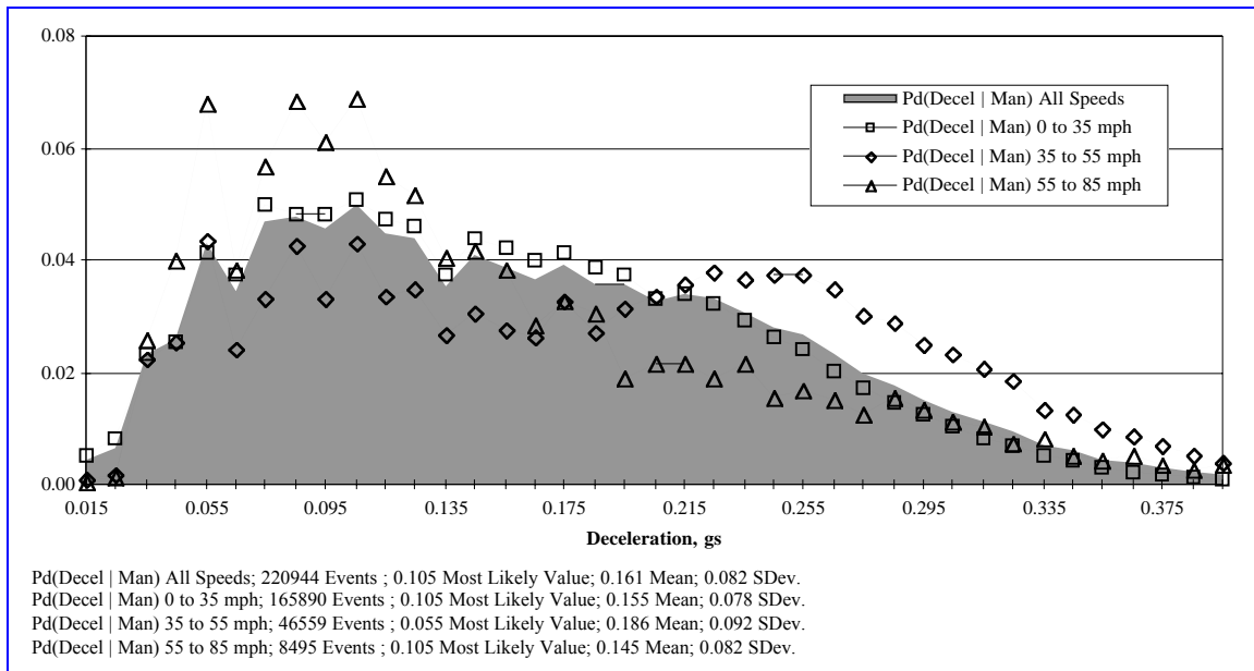
Figure 91. Maximum deceleration in manual braking events (duration > 1.0 seconds)
