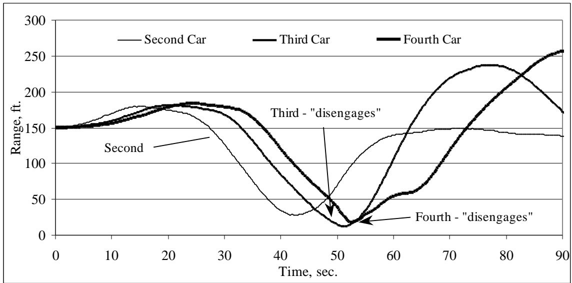
Figure 2. Range time history of three FOT vehicles in a string with a longitudinal disturbance
