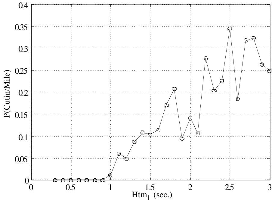
Figure 165. Frequency of cut-in rate per mile, low speed
