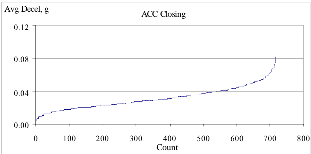
Figure 126. Average deceleration during the last 50ft of ACC closing
