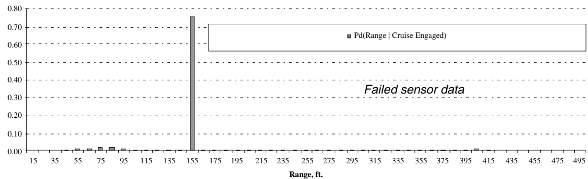
Pd(Range | Cruise Engaged); 0.9 Hrs; 1 Trips; 155.0 Most Likely Value; 168.7 Mean; 64.0 SDev.
