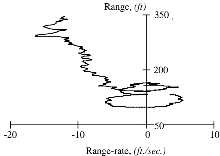
Figure 121. Range vs. range rate during the closing and following sequence of Figure 120
