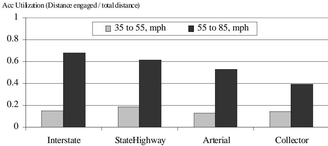
Figure 133. ACC utilization for different road type
