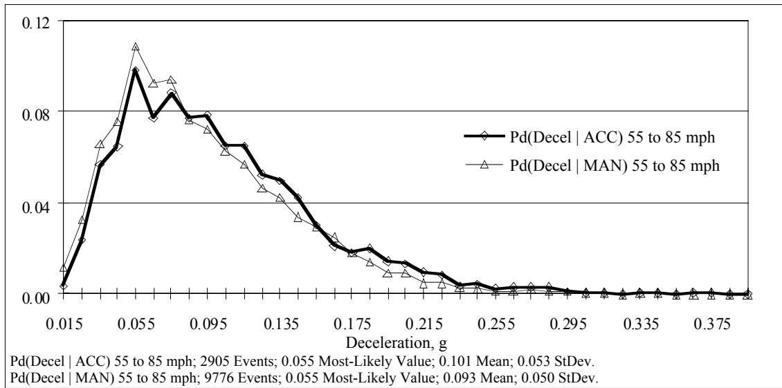
Figure 117. Distribution of average deceleration in braking events for ACC and manual driving (V > 55 mph)
