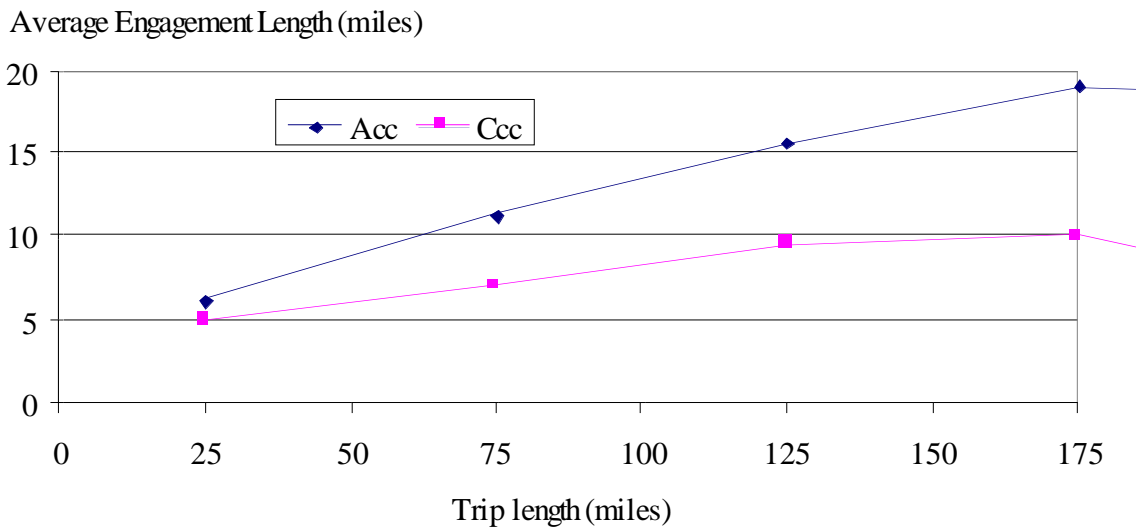
Figure 143. Average engaged length ( V_{ave}>55\text{mph} )
