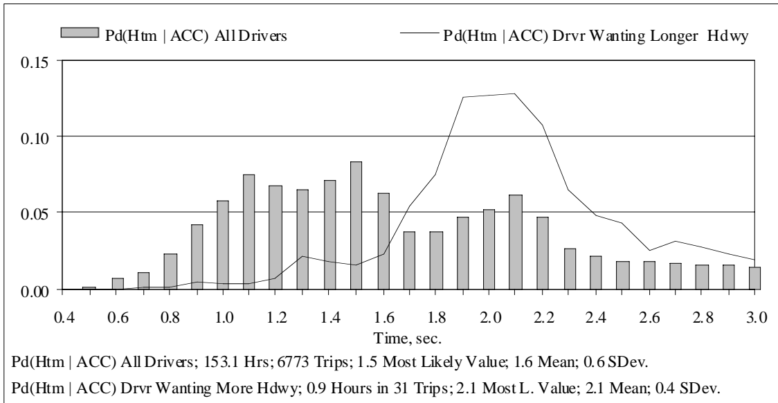
Figure 175. Headway time histogram for driver number 91
