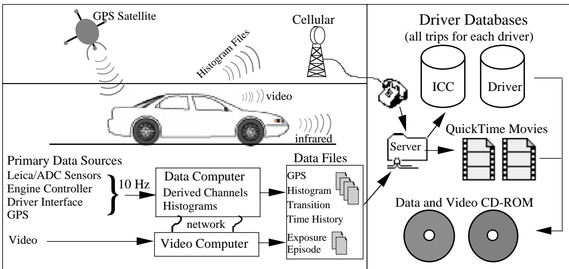
Figure 21. Data flow for the field operational test
