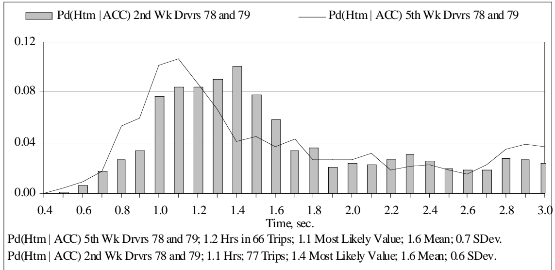
Figure 174. Headway time histograms for drivers 78 and 79 during their ACC driving
