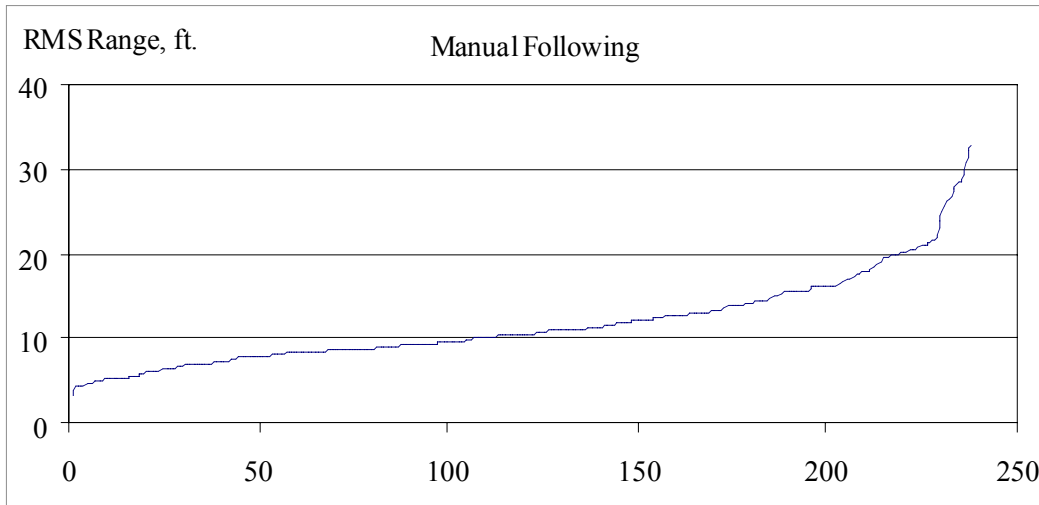
Figure 122. Root-mean-square deviation in range during manual following
