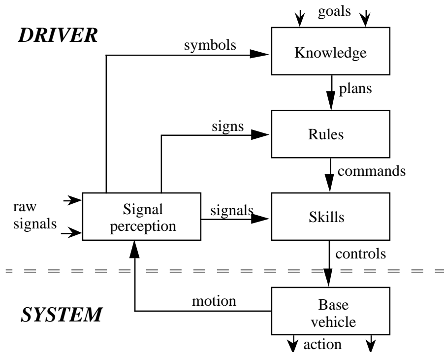
Figure 74. Skills, rules and knowledge associated with the driving process
