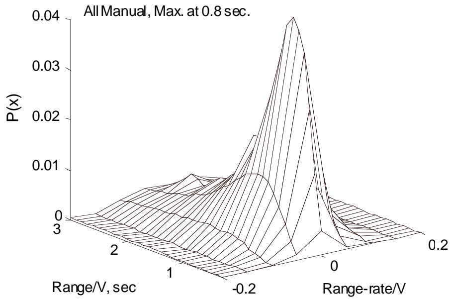
Figure 111. R/V versus Rdot/V for manual driving ( V > 55 mph)
