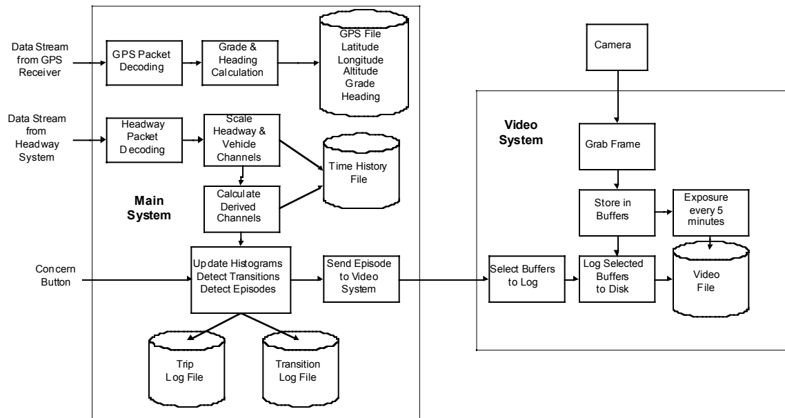
Figure 23. Data acquisition system operation
