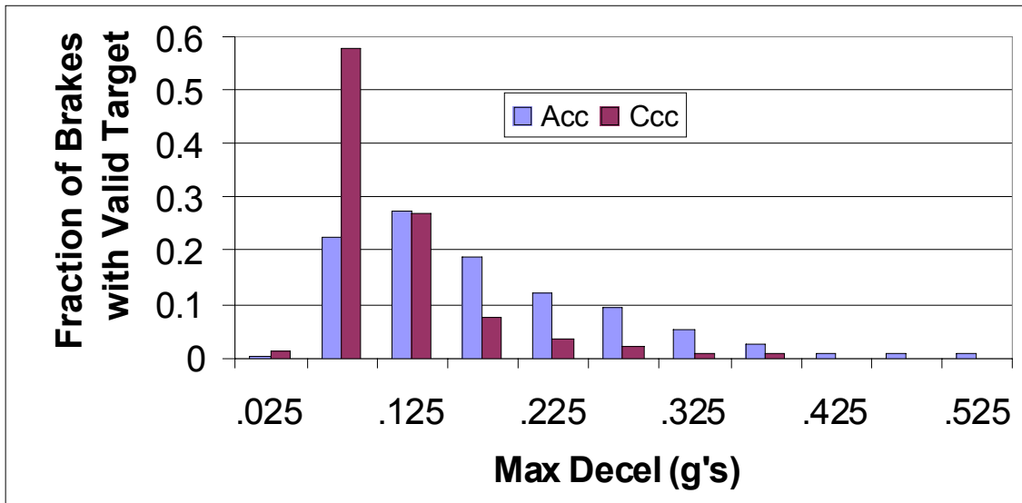
Figure 149. Maximum deceleration during braking, target present (V>55mph)
