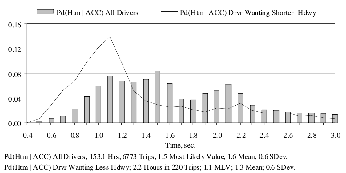
Figure 176. Headway time histogram for driver 85
