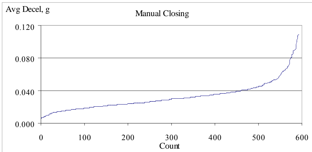
Figure 124. Average deceleration during the last 50ft of manual closing
