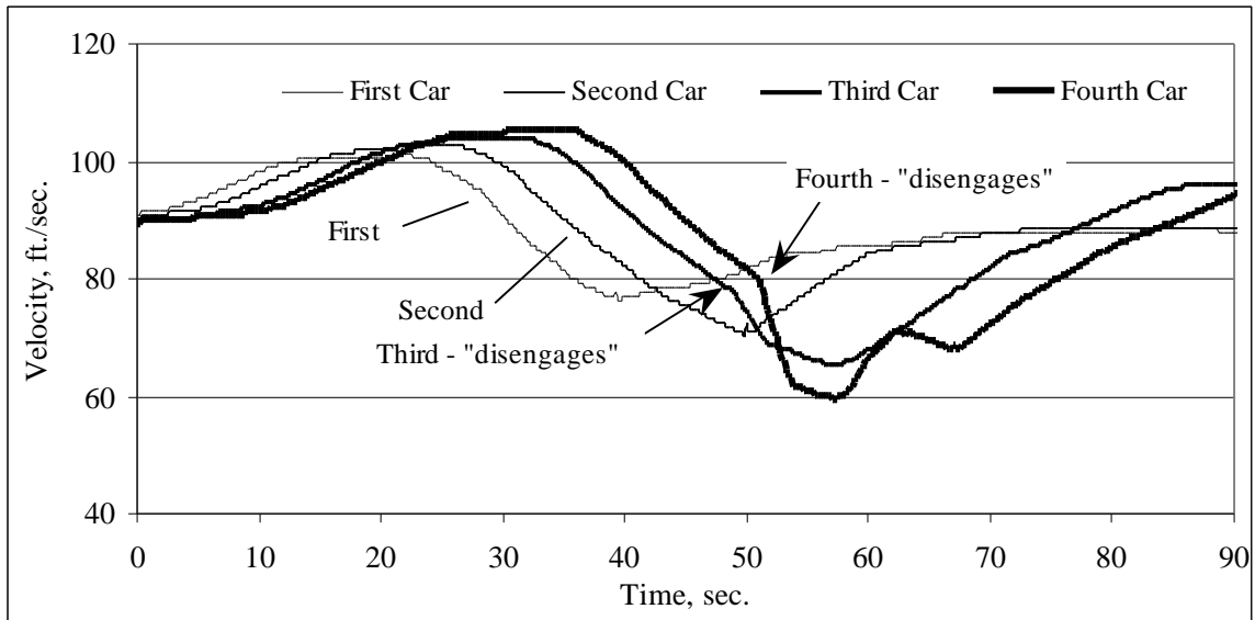
Figure 1. Velocity time history of four FOT vehicles in a string following a longitudinal disturbance
