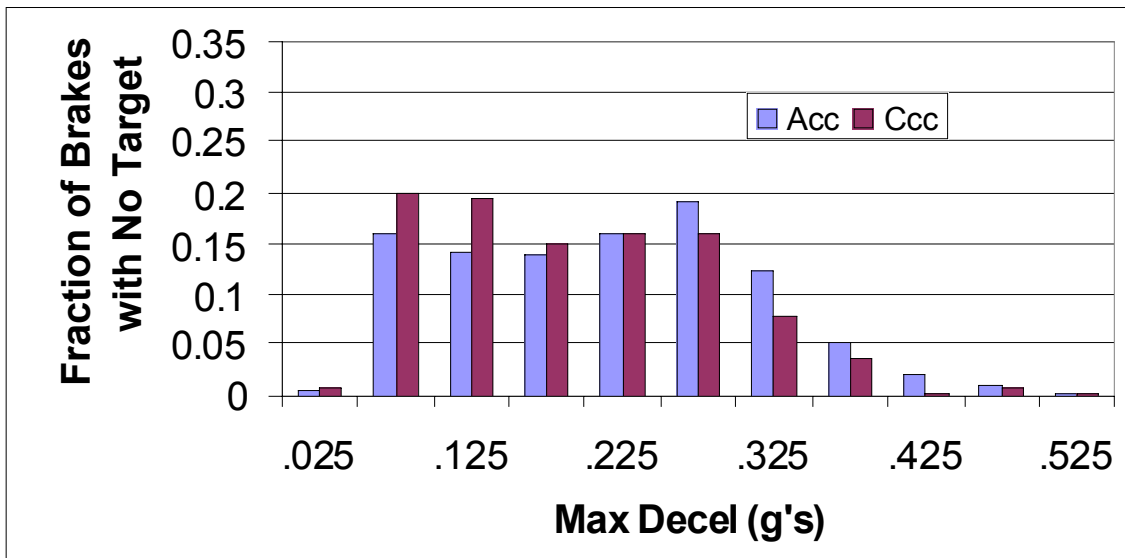
Figure 152. Maximum deceleration during braking, no target present (V<55mph)
