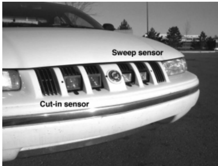
Figure 17. Sensors installed in the grill
