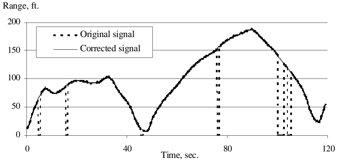
Figure 42. Original and corrected range signal
