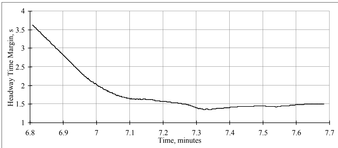
Figure E-2. Headway Time Margin ( H_{tm} ) versus time, closing from long range
