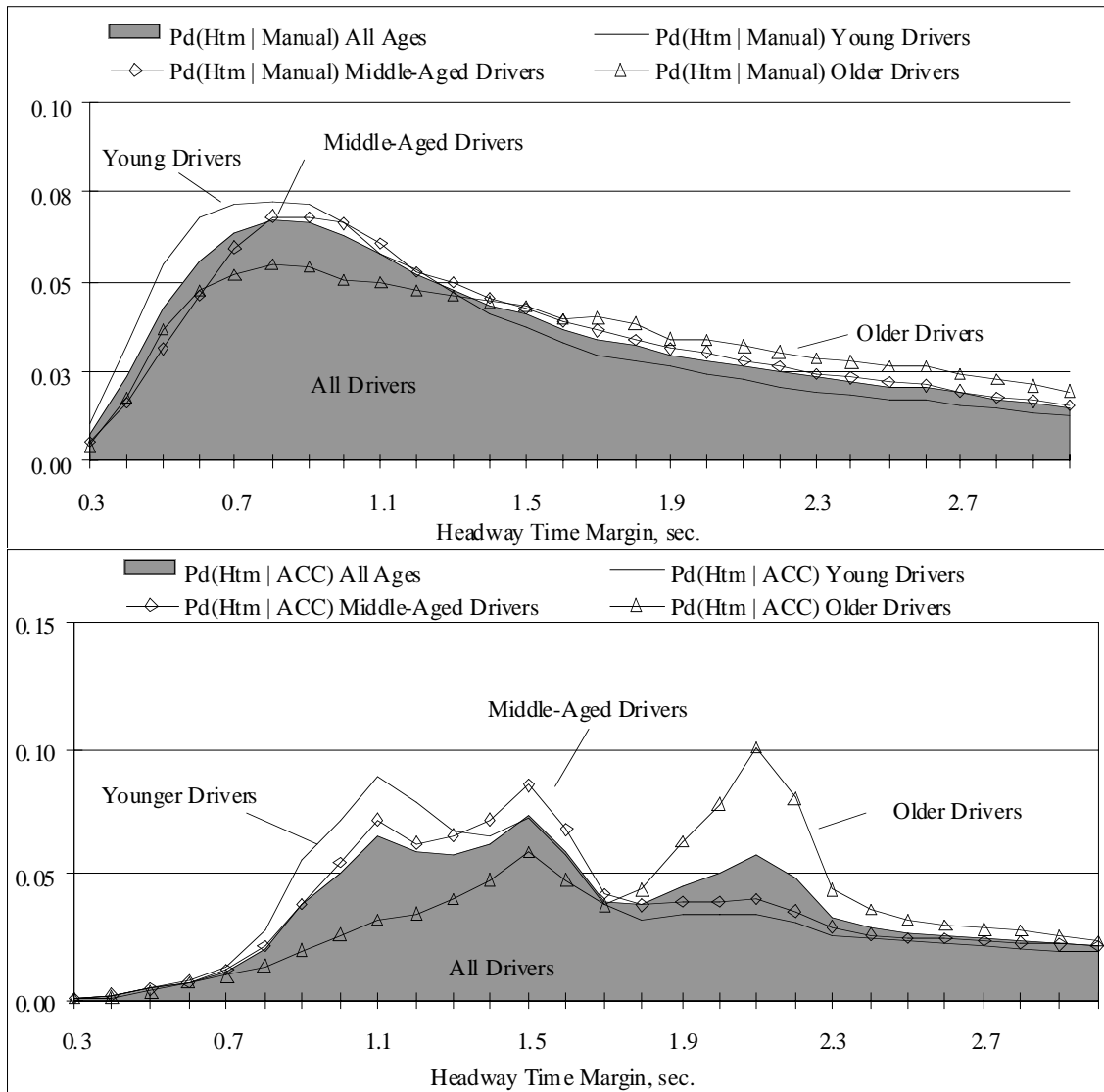
Figure 109. Influence of age on headway time margin under ACC and manual control
