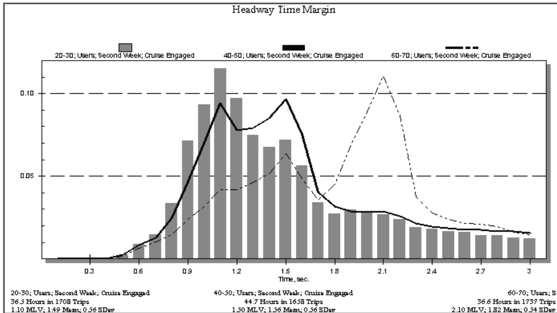
Figure 40. Example headway-time-margin histogram for cruise users
