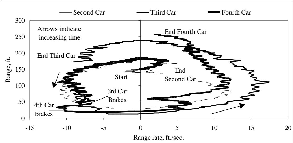
Figure 3. Range versus range-rate of three FOT vehicles in a string during a longitudinal disturbance
