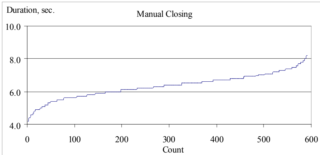
Figure 123. Duration of time for the last 50ft of manual closing
