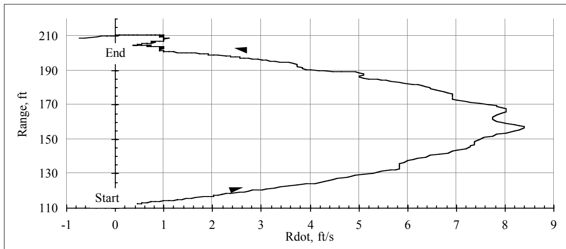
Figure E-5. Range versus Range-Rate, changing from T_h = 1.0 to 2.0 s
