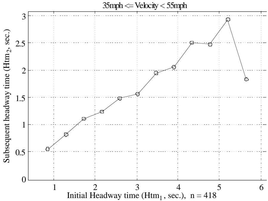
Figure 161. Average Htm 2 at cut-in vs. Htm 1 prior to cut-in, low speed
