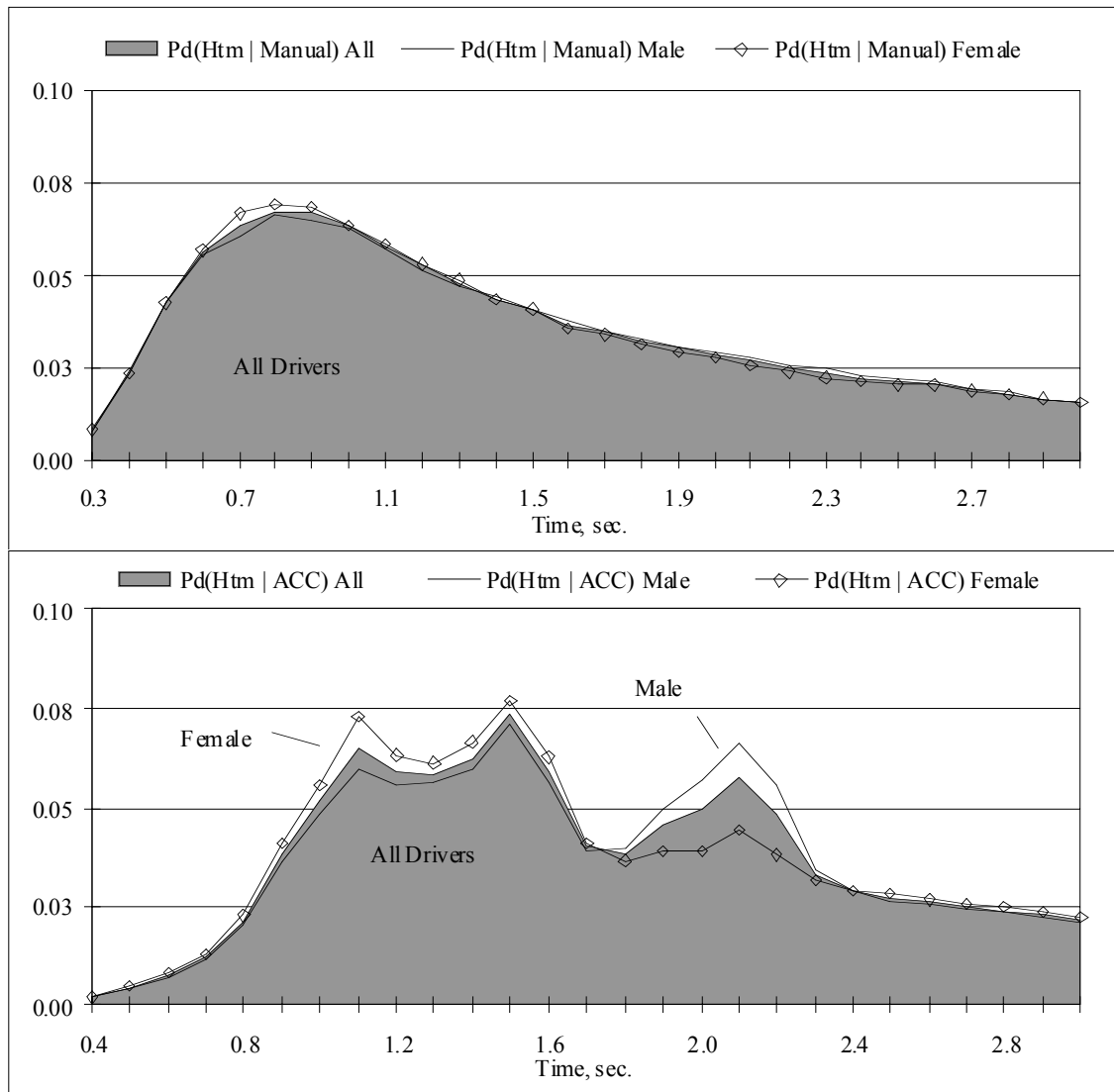
Figure 110. Influence of gender on headway time margin under ACC and manual control
