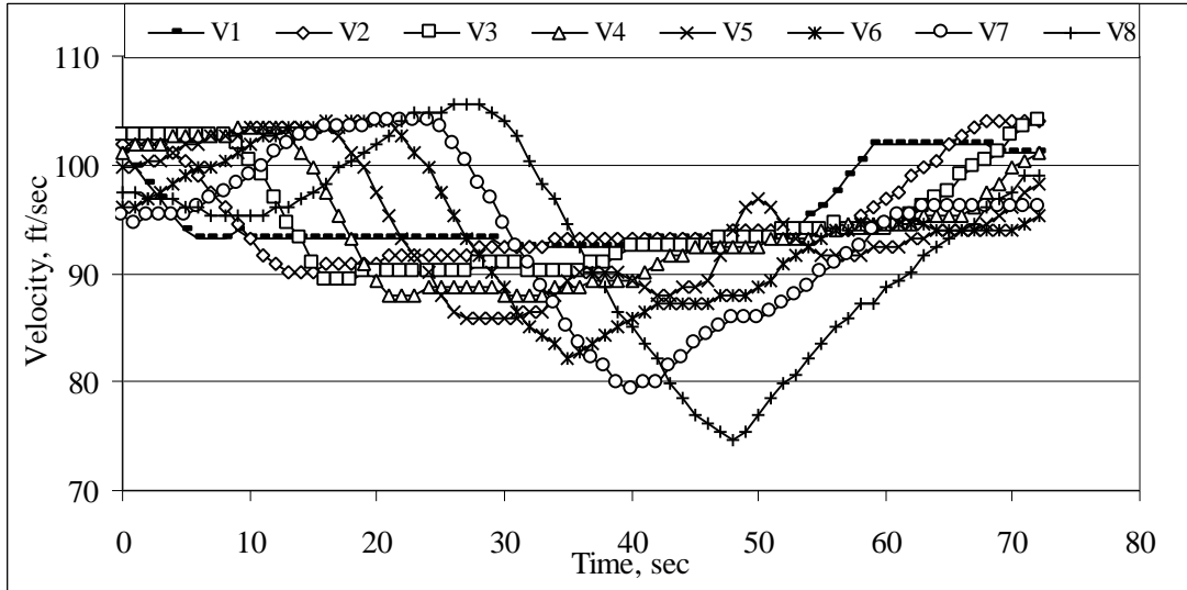
Figure 4. Velocity time history of eight FOT vehicles in a string with a longitudinal disturbance
