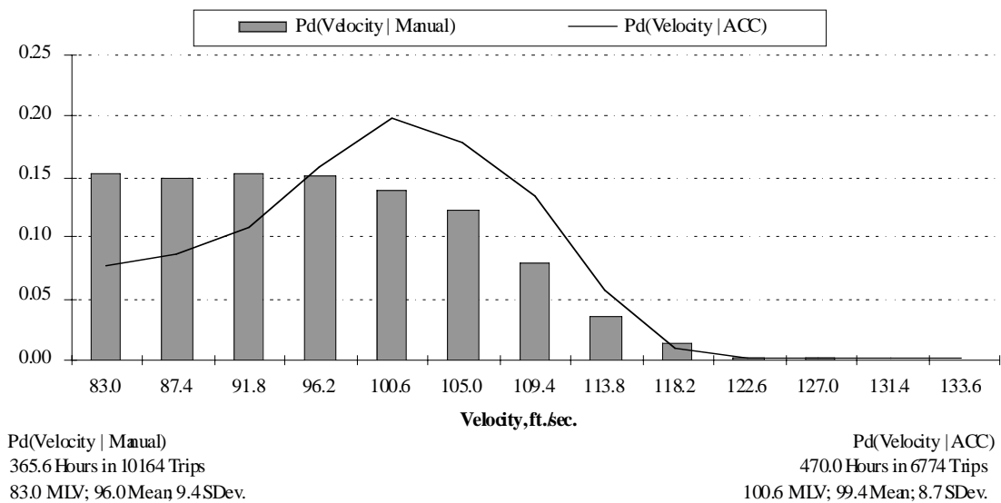
Figure 167. Velocity histogram of manual and ACC driving for all FOT drivers
