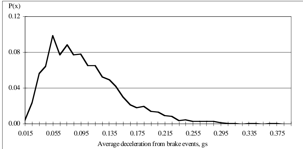
Figure 103. Average deceleration for all ACC braking events at V_{start} > 55 mph
