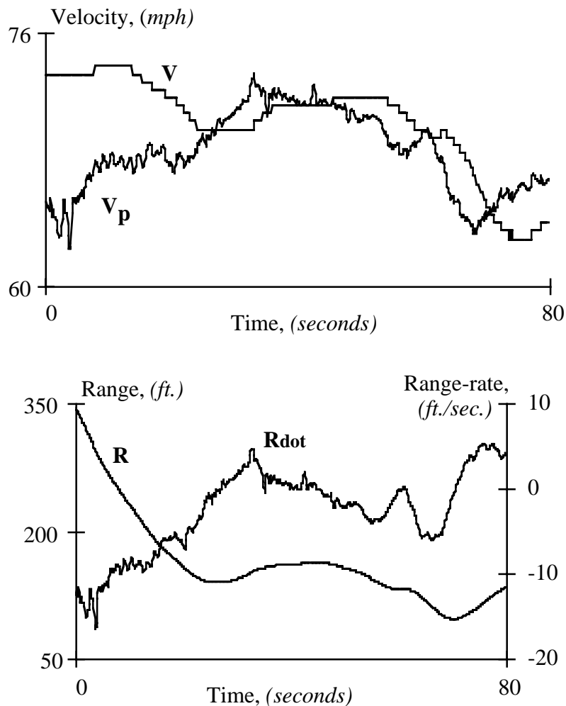
Figure 120. An example target stream illustrating closing and following operation during ACC driving
