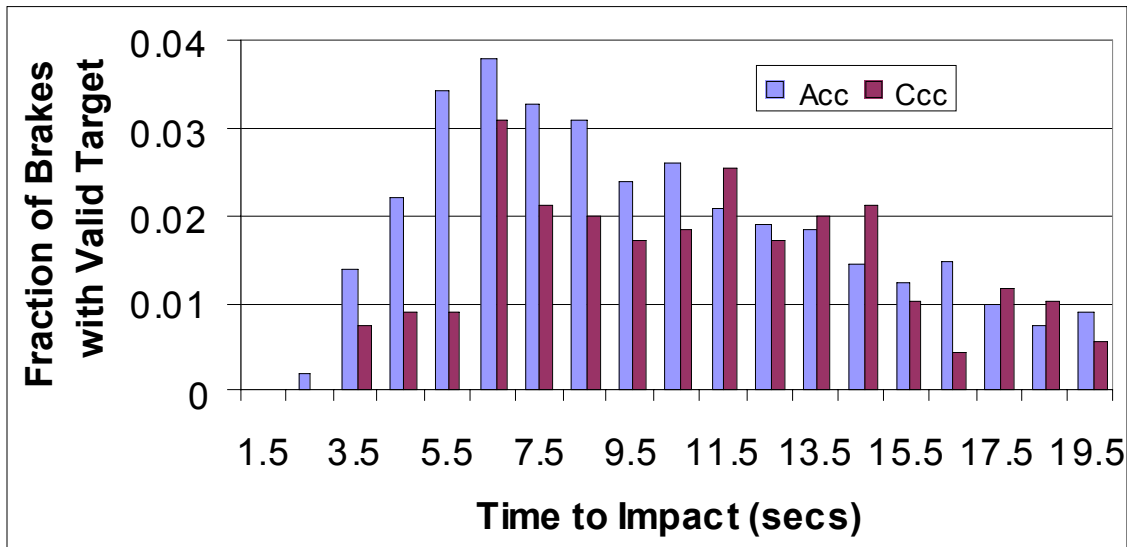
Figure 154. Time-To-Impact during braking ( V < 55 mph)
