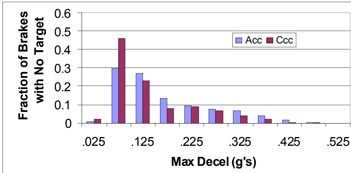
Figure 150. Maximum deceleration during braking, no target present ( V > 55 mph)
