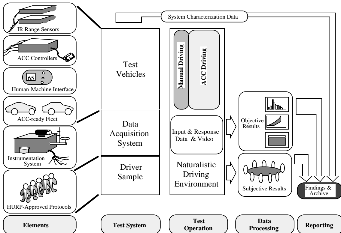
Figure 2. FOT Methodology overview
