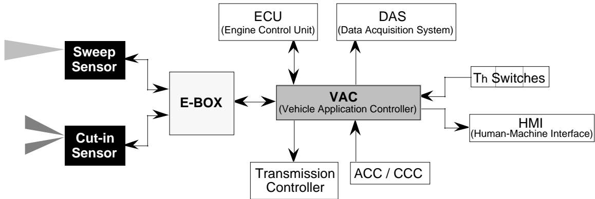
Figure 3. The ACC system layout and its connections
