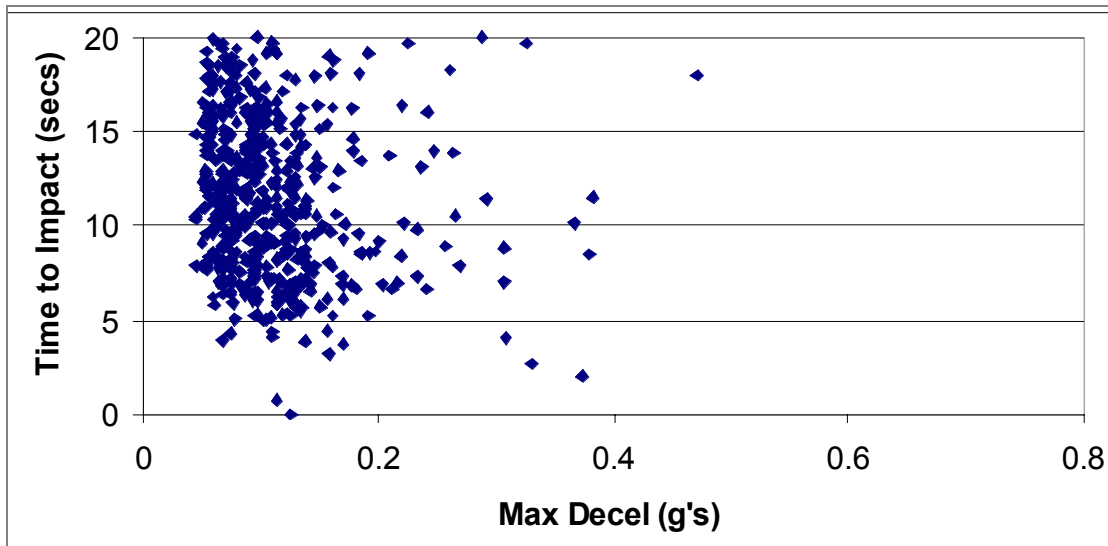
Figure 156. Time to Impact and maximum deceleration during CCC braking ( V > 55 mph)
