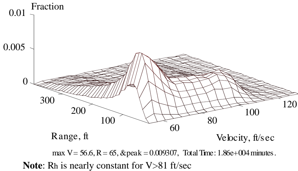
Figure 80. Observed frequency of range vs. velocity for manual driving
