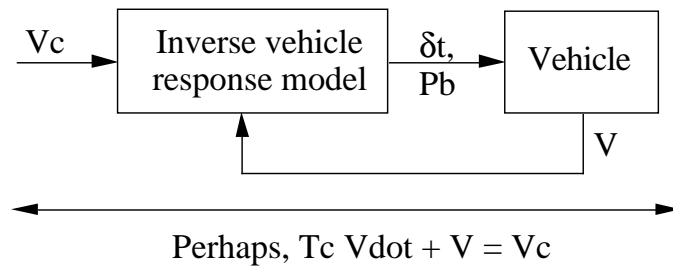
Figure 75. The operational elements of a tracking activity
