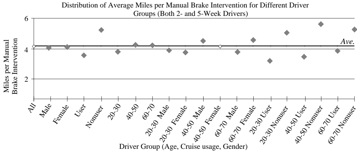
Figure 92. Manual braking per mile (V > 50mph)
