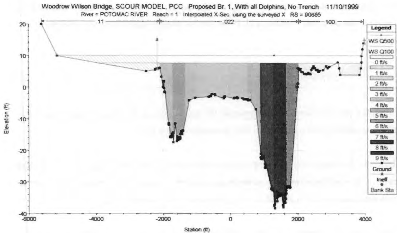
Figure 26. Velocity distribution from HEC-RAS model of Potomac River at cross-section approximately 5 mi upstream of the proposed bridges.
