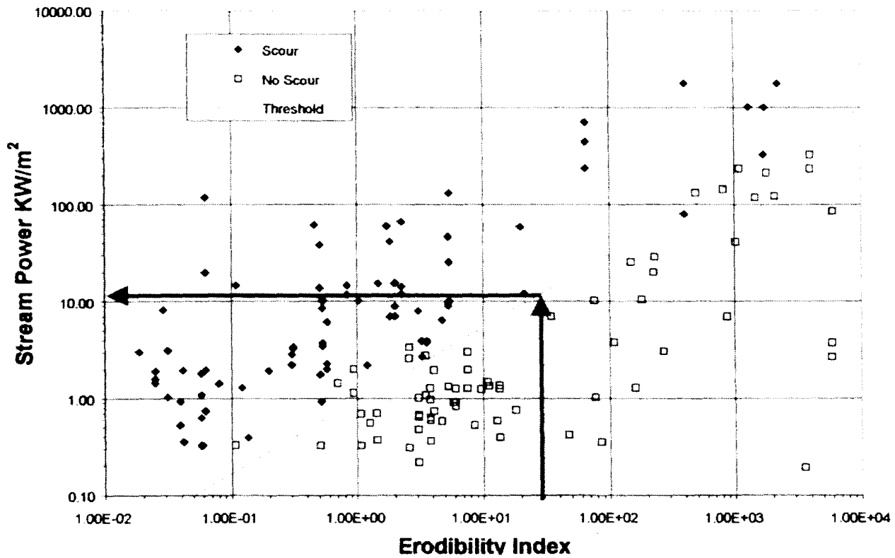
Figure 9. Determination of stream power that is required to scour earth material once the value of the Erodibility Index is known.
