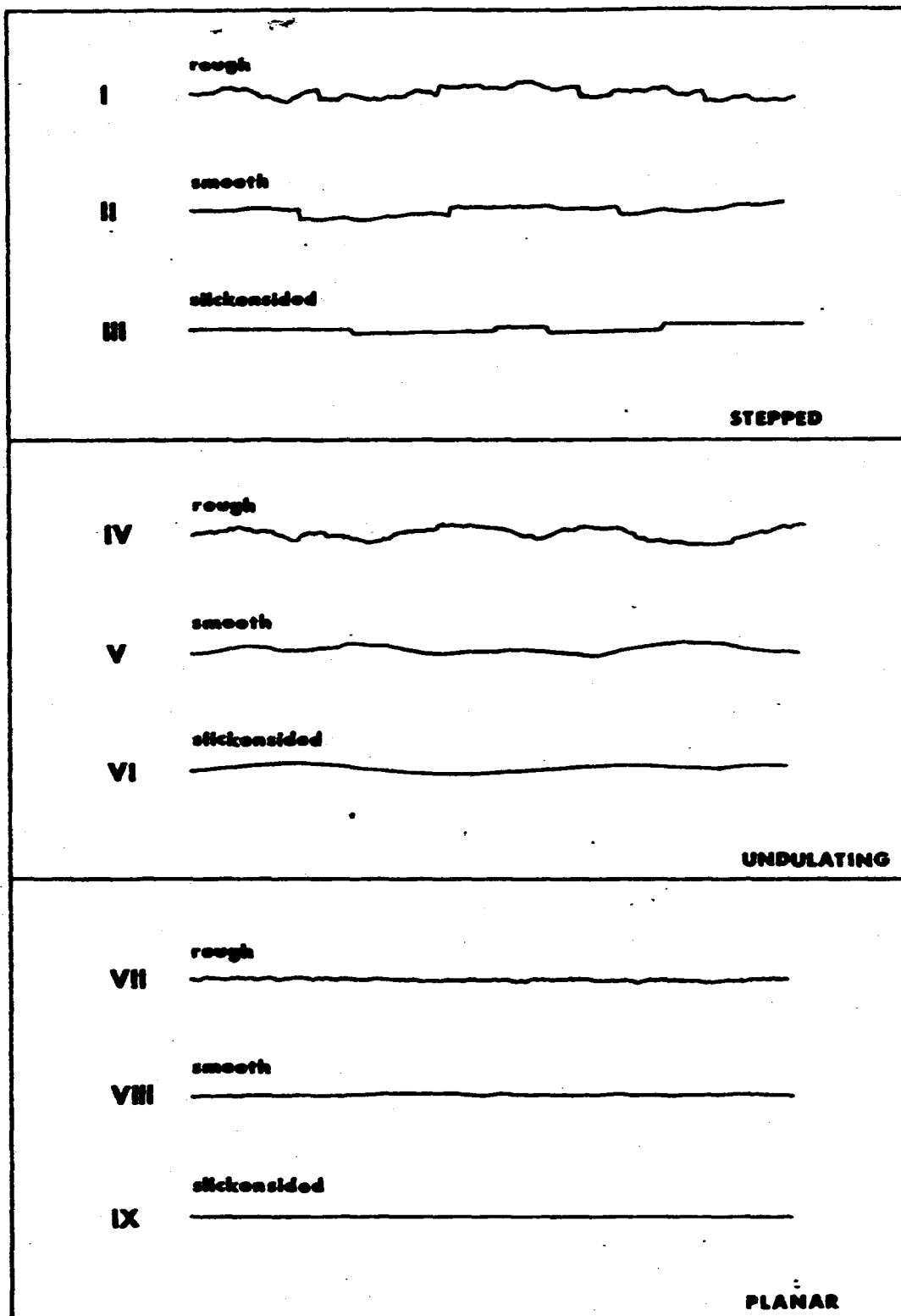
Figure 17. Schematic presentation of conventional descriptions of joint roughness.
