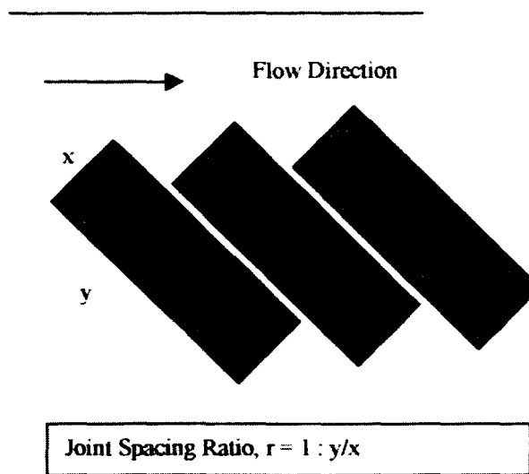
Figure 19. Determination of the joint spacing ratio, r .
