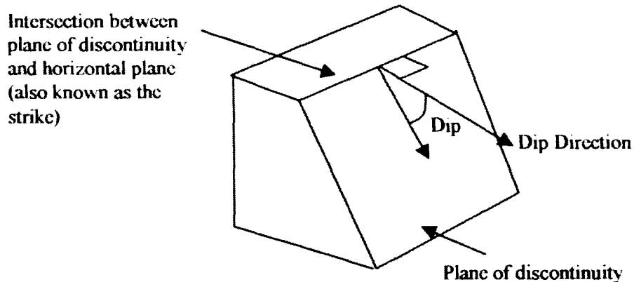
Figure 18. Definition sketch pertaining to dip and dip direction of rock.
