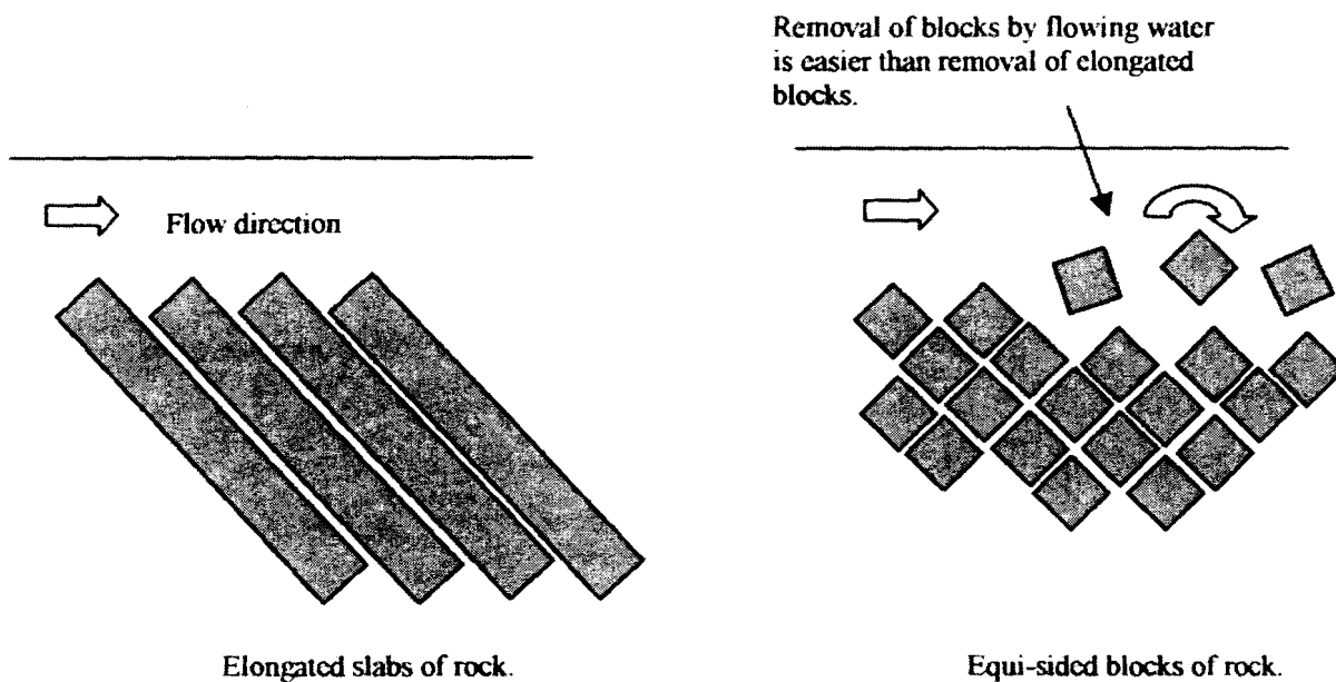
Figure 21. Influence of shape of rock blocks on scour resistance.
