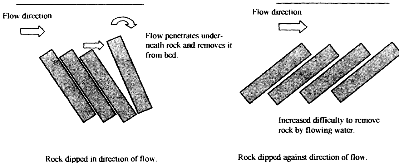
Figure 20. Influence of dip direction on scour resistance offered by rock.
