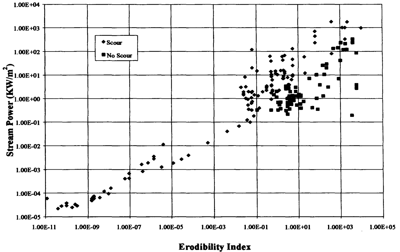
Figure 5. Erosion threshold for lower values of the Erodibility Index (Annandale 1995).
