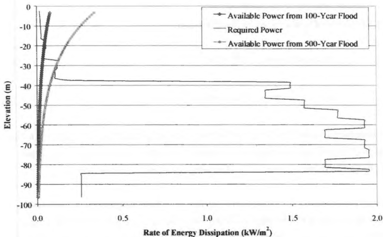
Figure 27. Available stream power and power required at pier M10.
