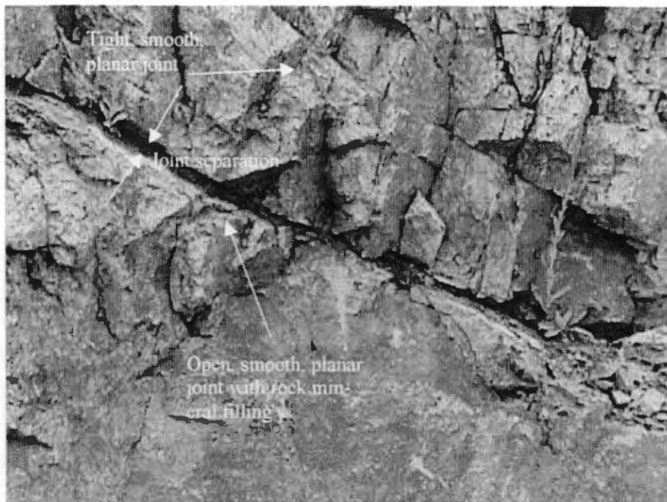
Figure 15. Planar joints.
