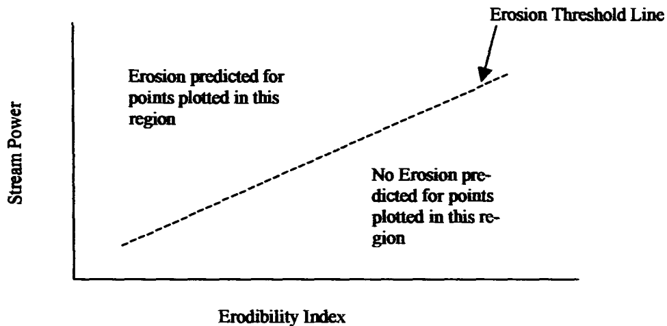
Figure 7. Determination of erodibility of earth materials.
