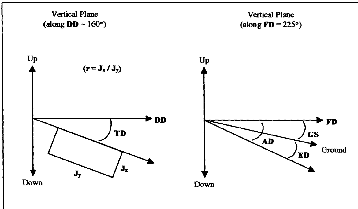
Figure 23. Vertical plane showing relationships between dip direction ( DD ), true dip ( TD ),
