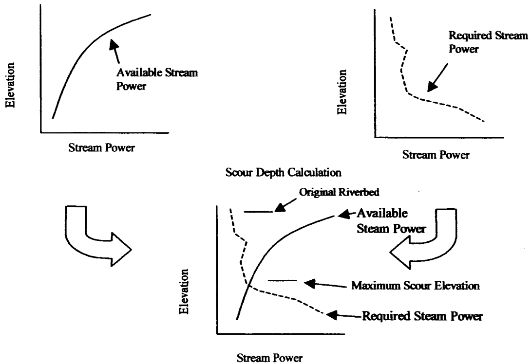
Figure 8. Determination of the extent of scour by comparing available and required stream power.
