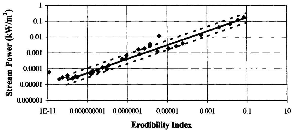
Figure 6. Erosion threshold for the entire range of earth materials, ranging from silt to intact, massive rock – combining figures 4 and 5 (Annandale 1995).
