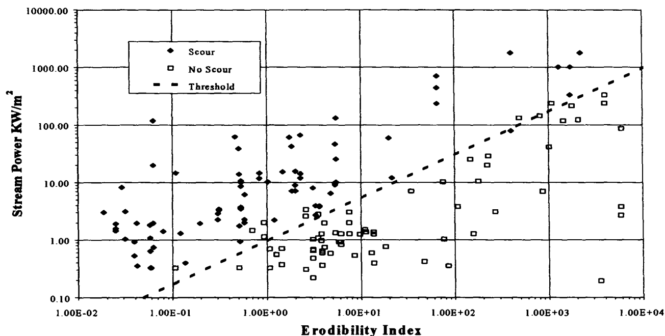
Figure 4. Erosion threshold for higher values of the Erodibility Index (Annandale 1995).
