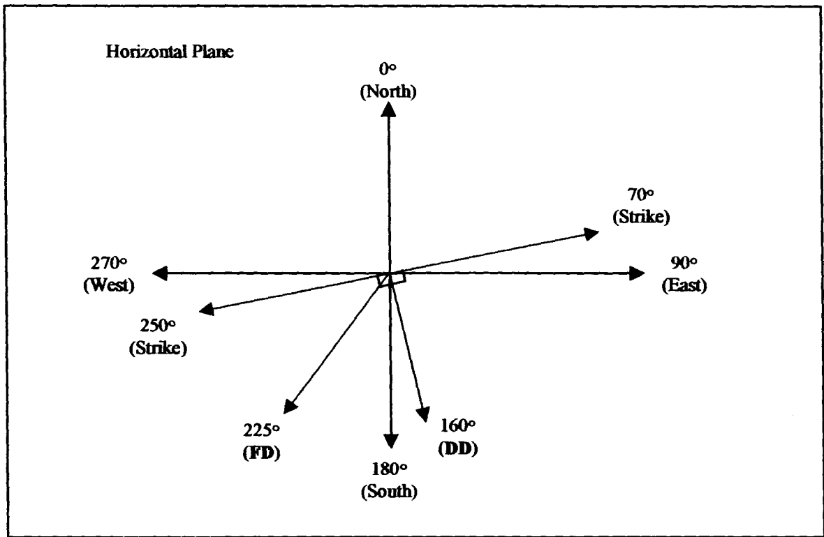
Figure 22. Horizontal plane showing relationships between flow direction ( FD ), dip direction ( DD ) and strike.
