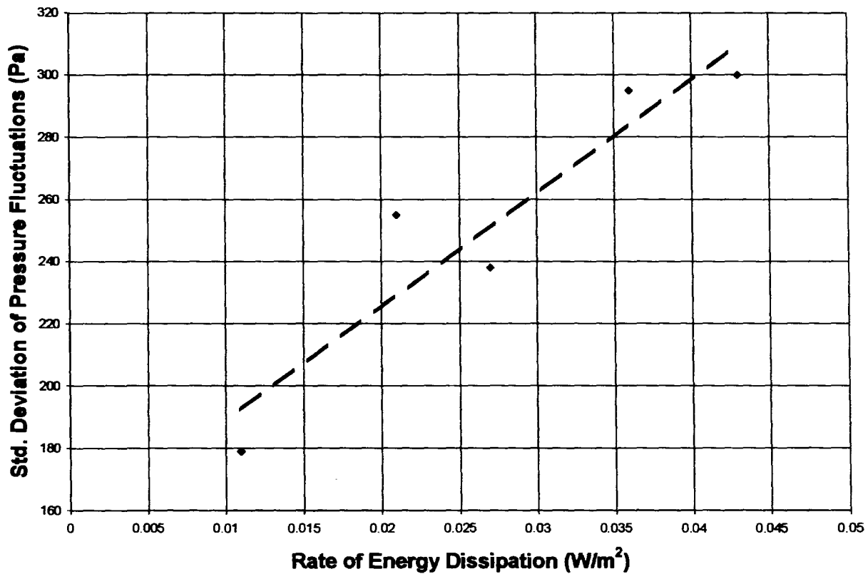
Figure 3. Relationship between the rate of energy dissipation and standard deviation of pressure fluctuations (Annandale 1995).
