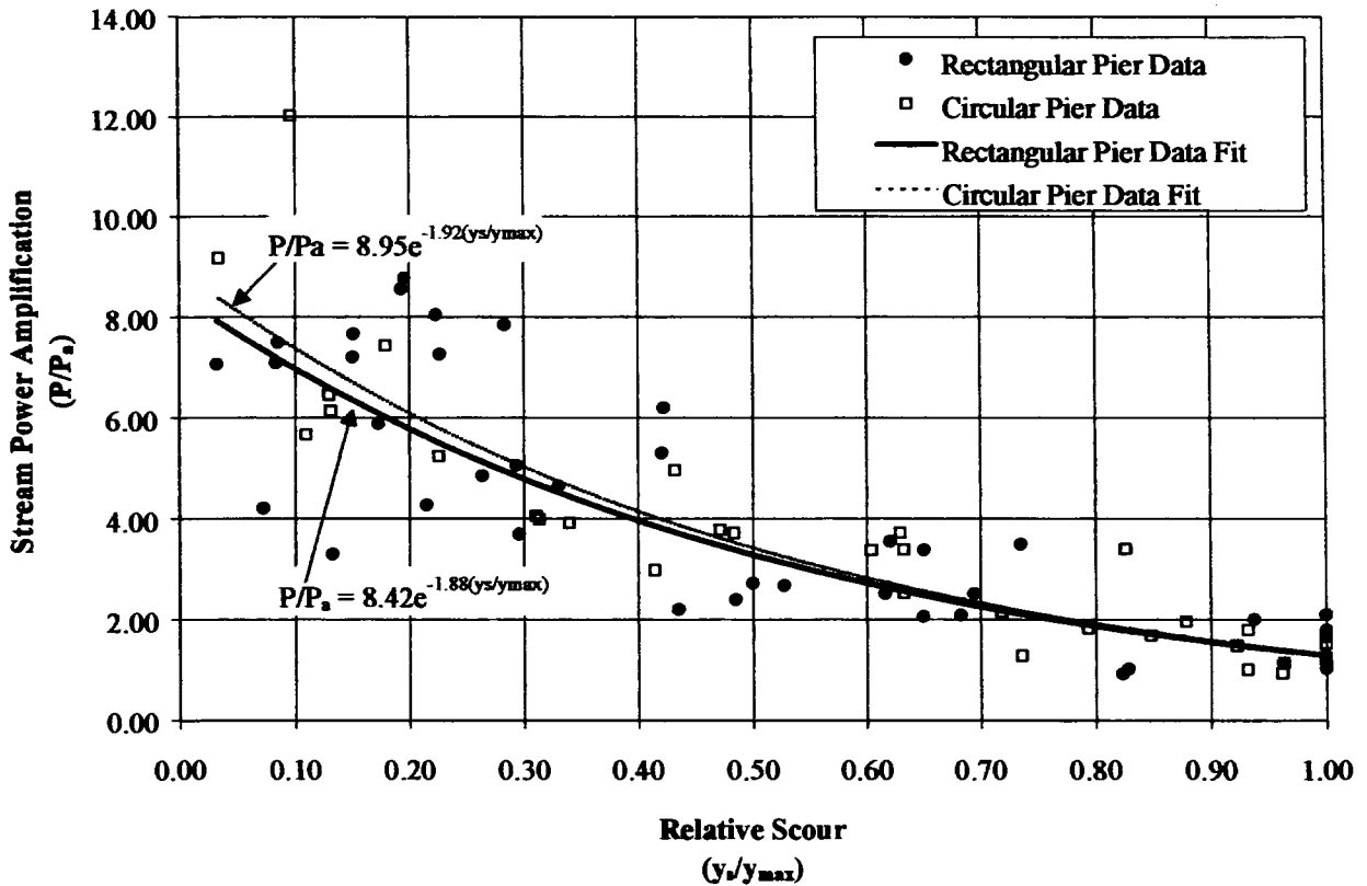
Figure 11. Dimensionless stream power at the base of a scour hole versus dimensionless scour hole depth from FHWA.
