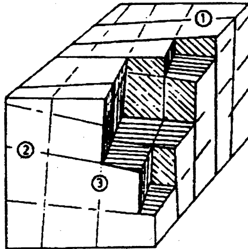
THREE JOINT SET
