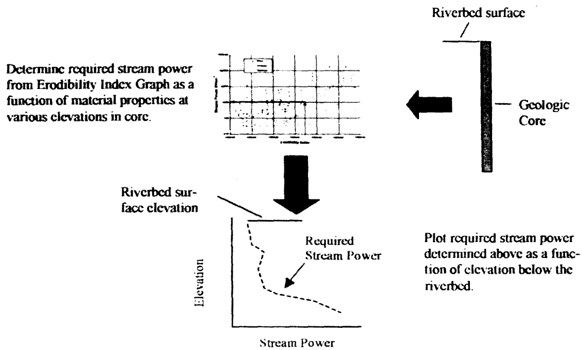
Figure 10. Development of a relationship between the required stream power and elevation below a riverbed.
