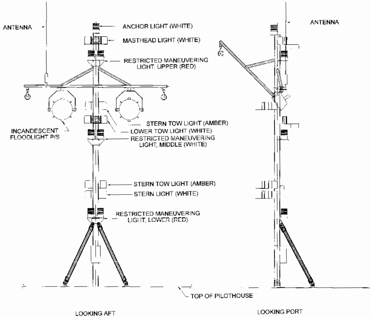
Figure 3-45 Navigation Lights, Searchlights, Floodlights, and Signal Devices (Elevation View)
