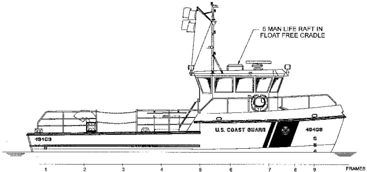
Figure 2-20 Life Raft
