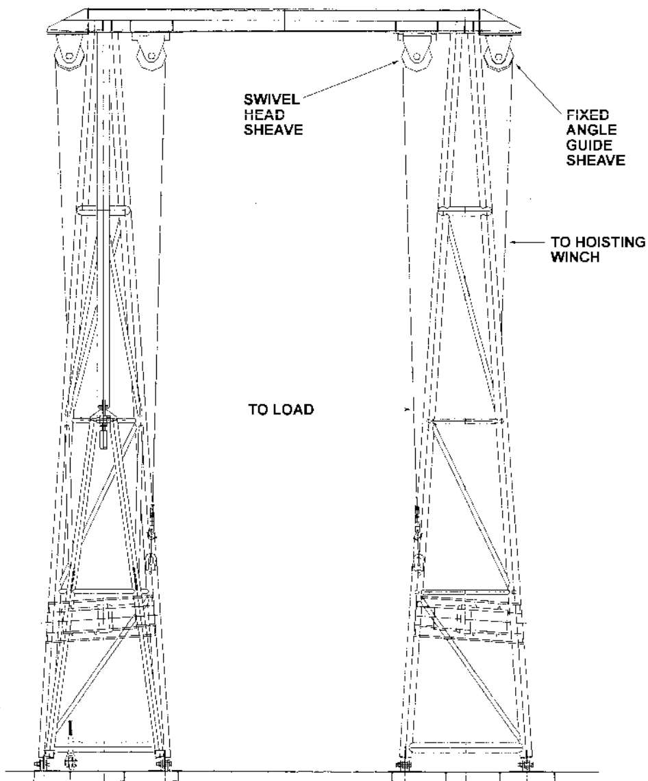
Figure 3-34 A-Frame Structure
