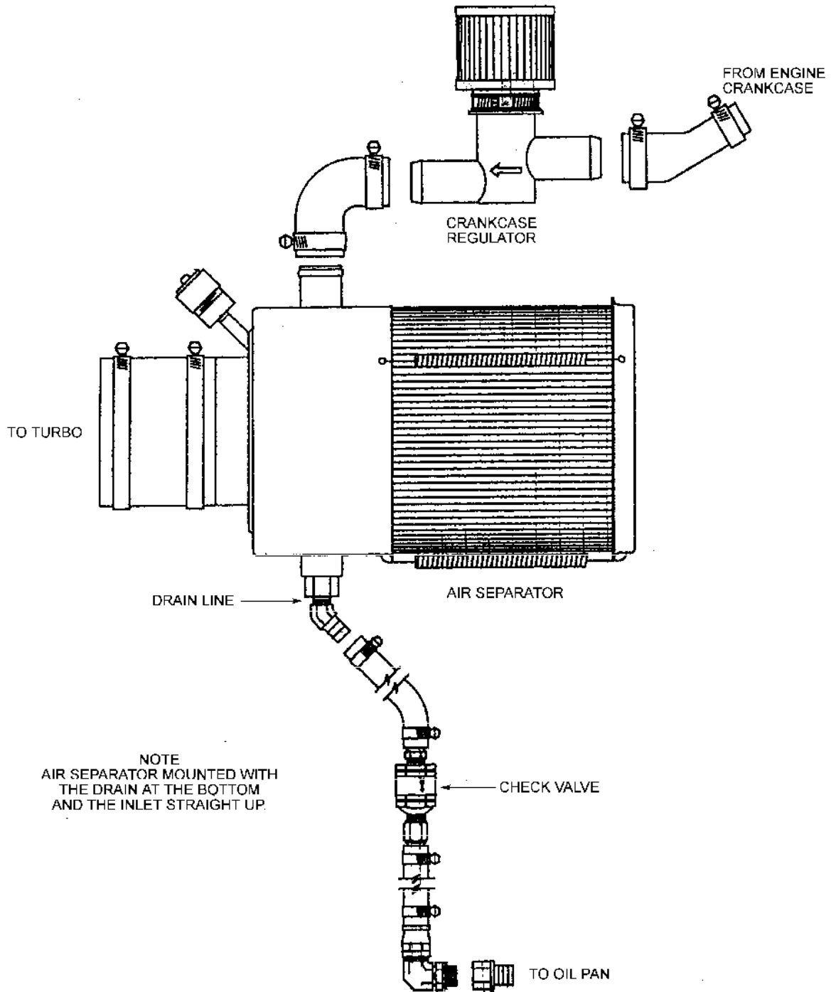
Figure 3-11 Engine Crankcase Ventilation System
