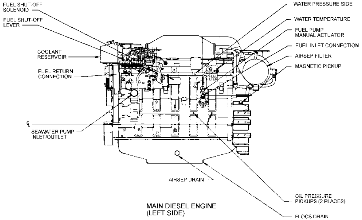
Figure 3-1 Propulsion System
