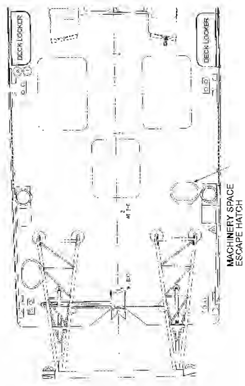
Figure 2-6 Machinery Space
