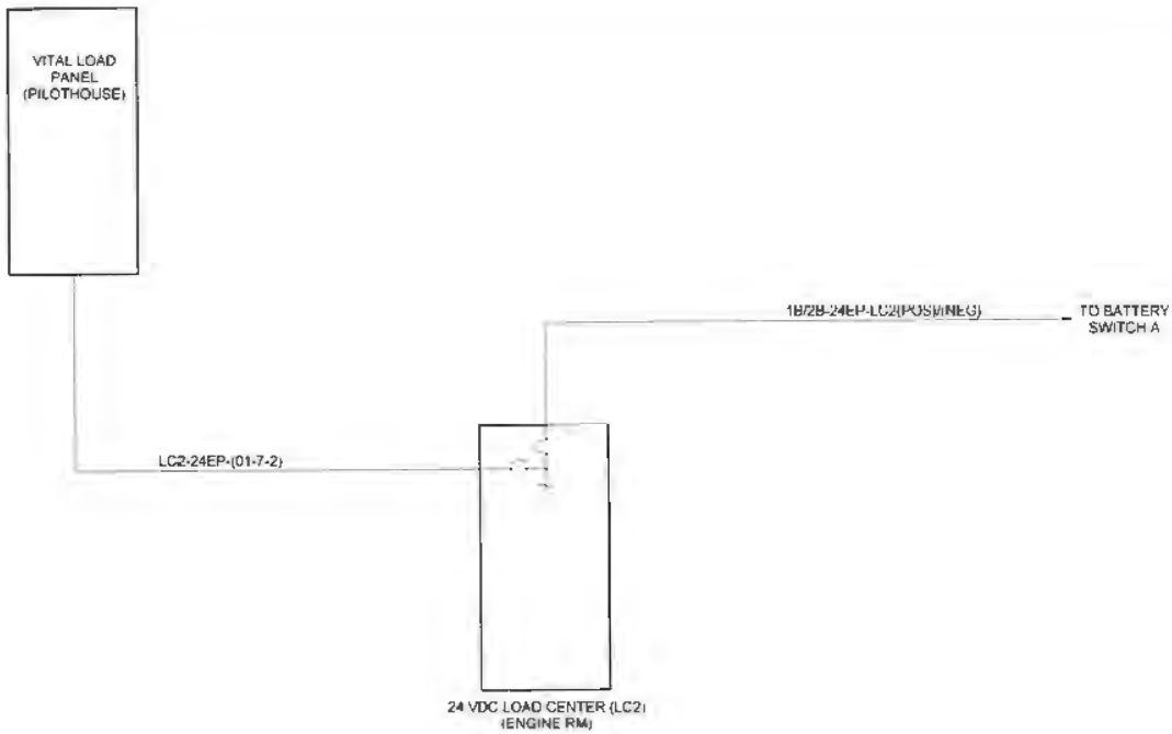
Figure 3-20 Power Panels
