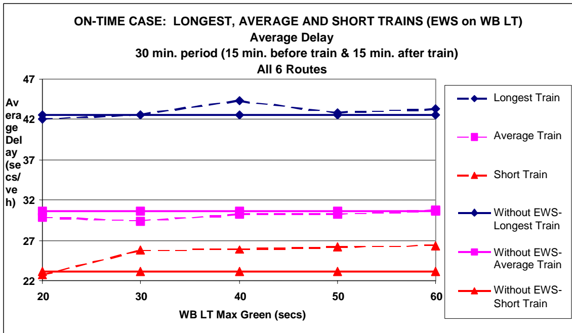
Figure 13: Delay for Different Gates Down Durations Using EWS on WB LT
