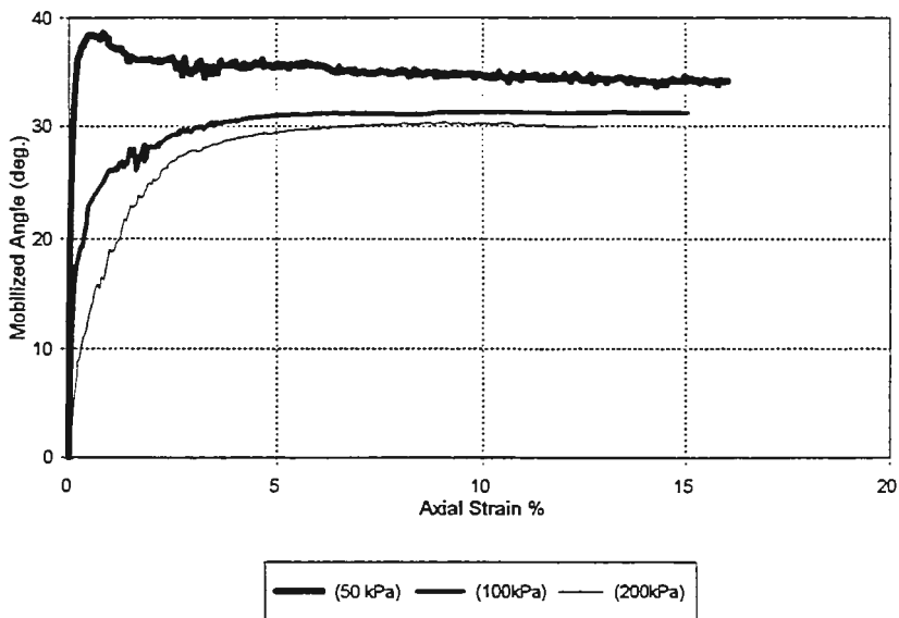
CID Triaxial, Fly/Bottom Ash Gibson Plant Ash, (F2=53%, R=90%)
