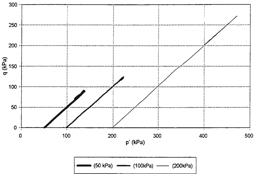
CID Triaxial, Fly/Bottom Ash Schahfer Plant Ash, (F1=75%, R=90%)
