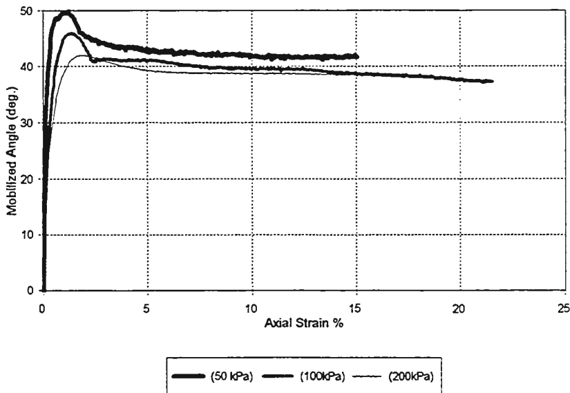
CID Triaxial, Fly/Bottom Ash Gibson Plant Ash, (F2=22%, R=95%)
