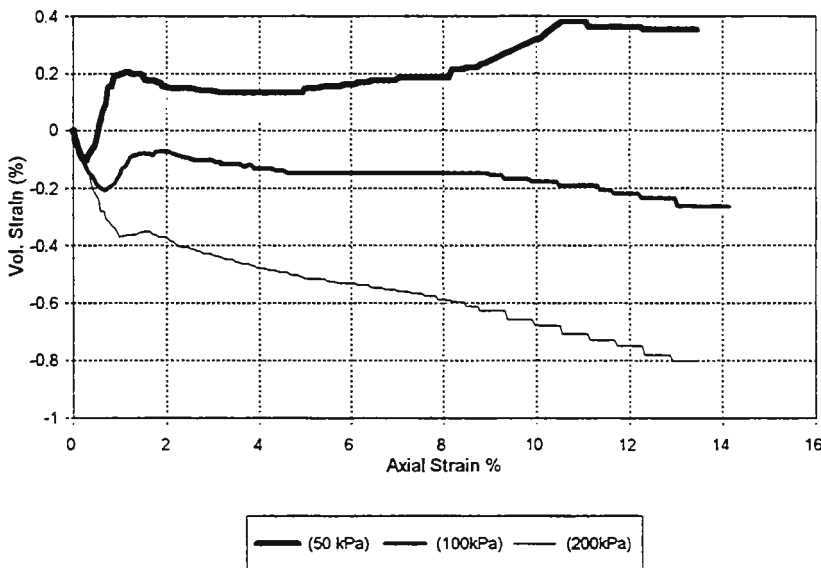
CID Triaxial, Fly/Bottom Ash Schahfer Plant Ash, (F 1 =75%, R=95%)
