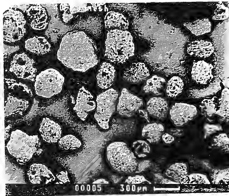
(b) Retained no.200 Sieve.
