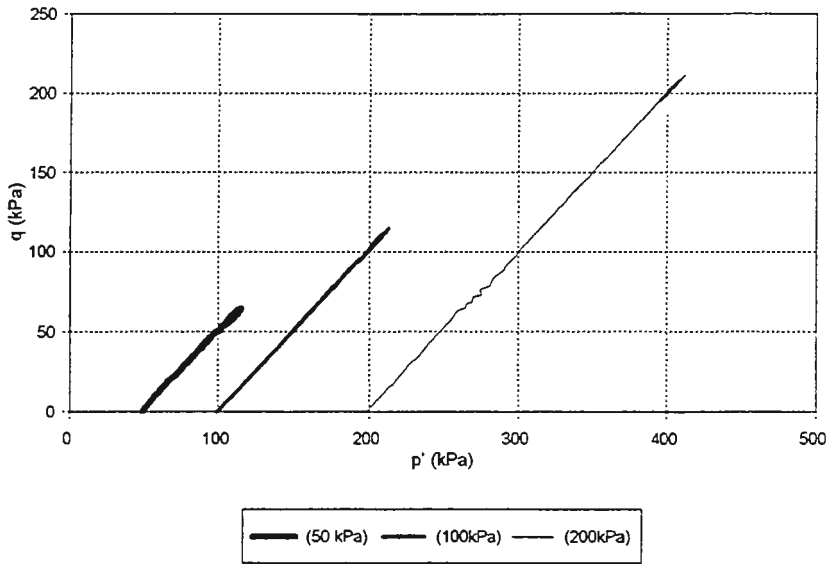
CID Triaxial, Fly/Bottom Ash Gibson Plant Ash, (F2=74%, R=90%)
