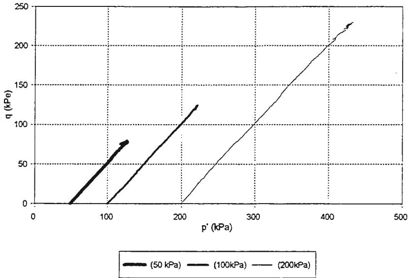
CID Triaxial, Fly/Bottom Ash Schahfer Plant Ash, (F1=50%, R=90%)
