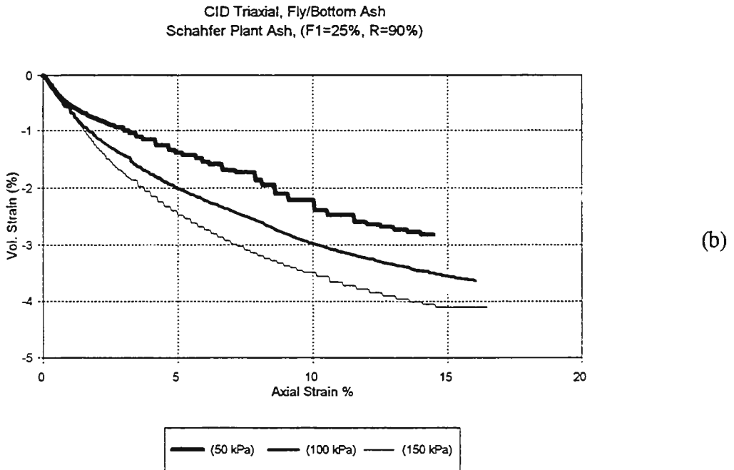
Figure 5.11 CID Triaxial Tests on Explicit Mixtures (F 1 = 25%) Compacted at R = 90% (a) Deviatoric Stress vs. Axial Strain (b) Volumetric Strain vs. Axial Strain (c) Effective Stress Path (d) Mobilized Angle of Shearing Resistance vs. Axial Strain. [Continued]
