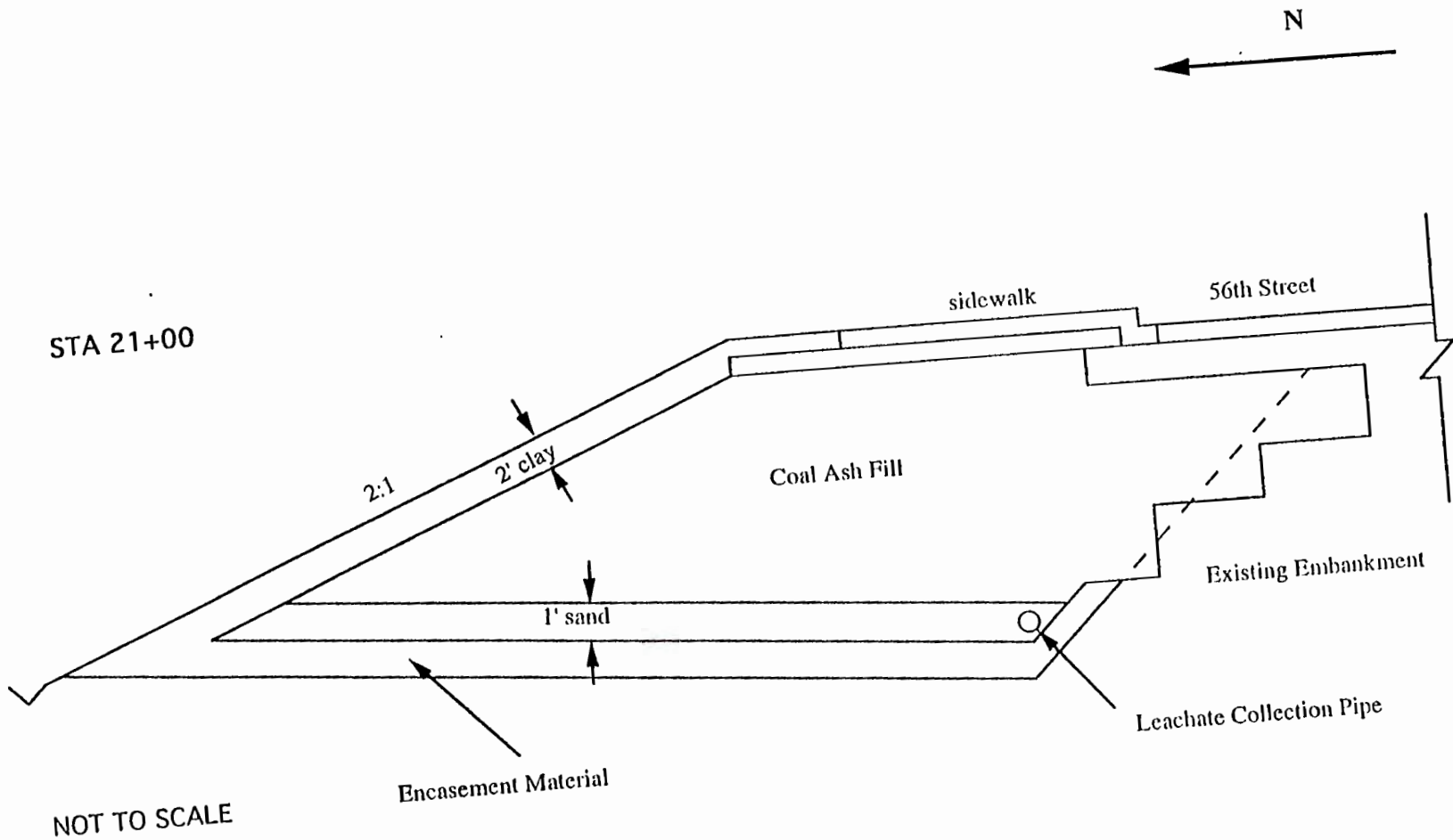
Figure 6.1 Cross Section of 56th Street-West, CCBP Embankments, Indianapolis (Alleman et al. 1996)
