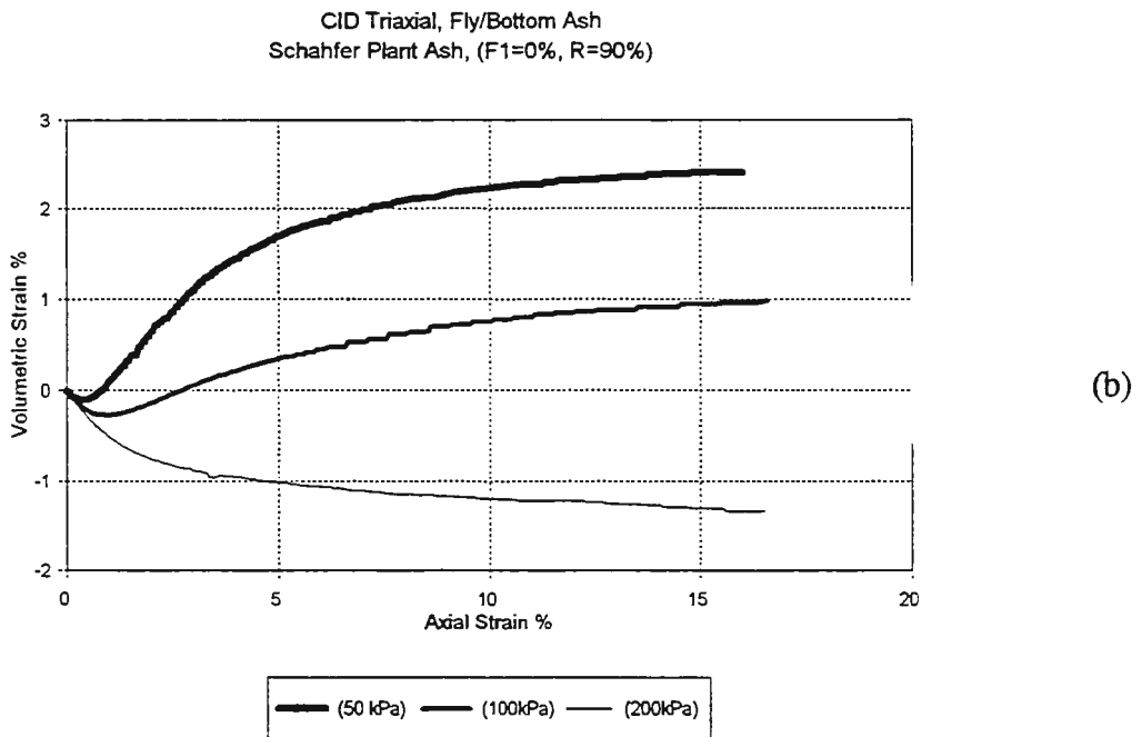
Figure 5.10 CID Triaxial Tests on Bottom Ash ( F_1 = 0.0\% ) Compacted at R = 90\% (a) Deviatoric Stress vs. Axial Strain (b) Volumetric Strain vs. Axial Strain (c) Effective Stress Path (d) Mobilized Angle of Shearing Resistance vs. Axial Strain. [Continued]
