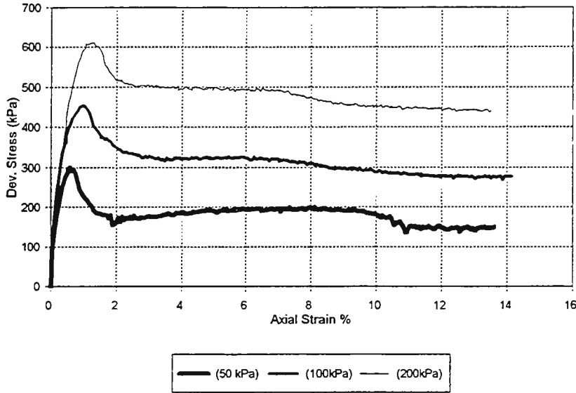
CID Triaxial, Fly/Bottom Ash Schahfer Plant Ash, (F 1 =75%, R=95%)
