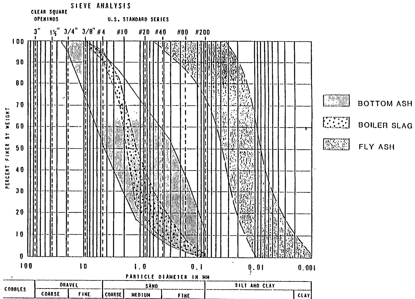
Figure 2.3 Typical Particle Size Distribution Ranges for Coal Ash. (McLaren and Digioia 1987), (Huang 1990), (USIFCA and GAI 1993).
