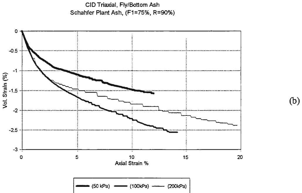
Figure 5.13 CID Triaxial Tests on Explicit Mixtures (F 1 = 75%) Compacted at R = 90% (a) Deviatoric Stress vs. Axial Strain (b) Volumetric Strain vs. Axial Strain (c) Effective Stress Path (d) Mobilized Angle of Shearing Resistance vs. Axial Strain. [Continued]
