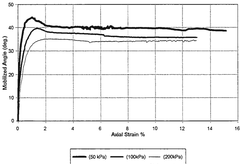
CID Triaxial, Fly/Bottom Ash Gibson Plant Ash, (F2=22%, R=90%)
