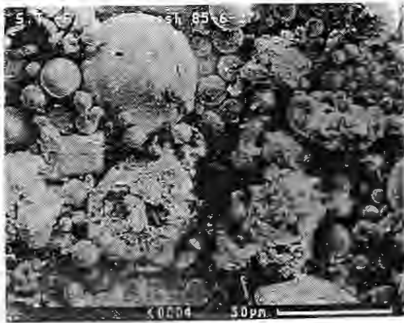
(a) Passing no.400 Sieve.
