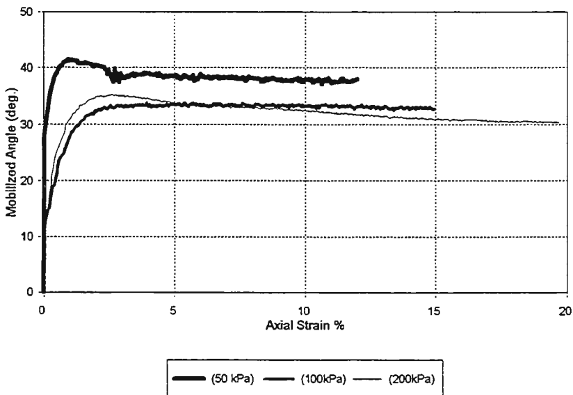
CID Triaxial, Fly/Bottom Ash Schahfer Plant Ash, (F1=75%, R=90%)
