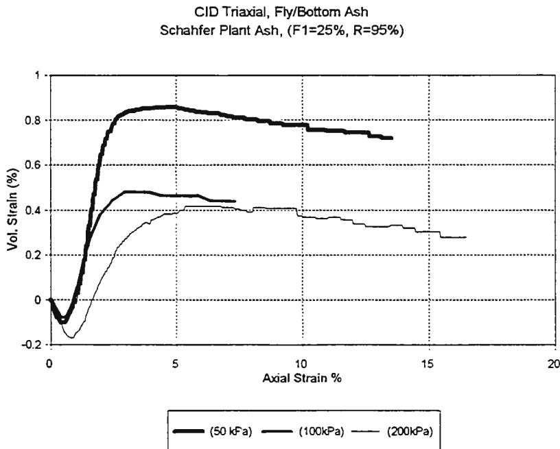
Figure 5.6 CID Triaxial Tests on Explicit Mixtures (F 1 = 25%) Compacted at R = 95 % (a) Deviatoric Stress vs. Axial Strain (b) Volumetric Strain vs. Axial Strain (c) Effective Stress Path (d) Mobilized Angle of Shearing Resistance vs. Axial Strain. [Continued]
