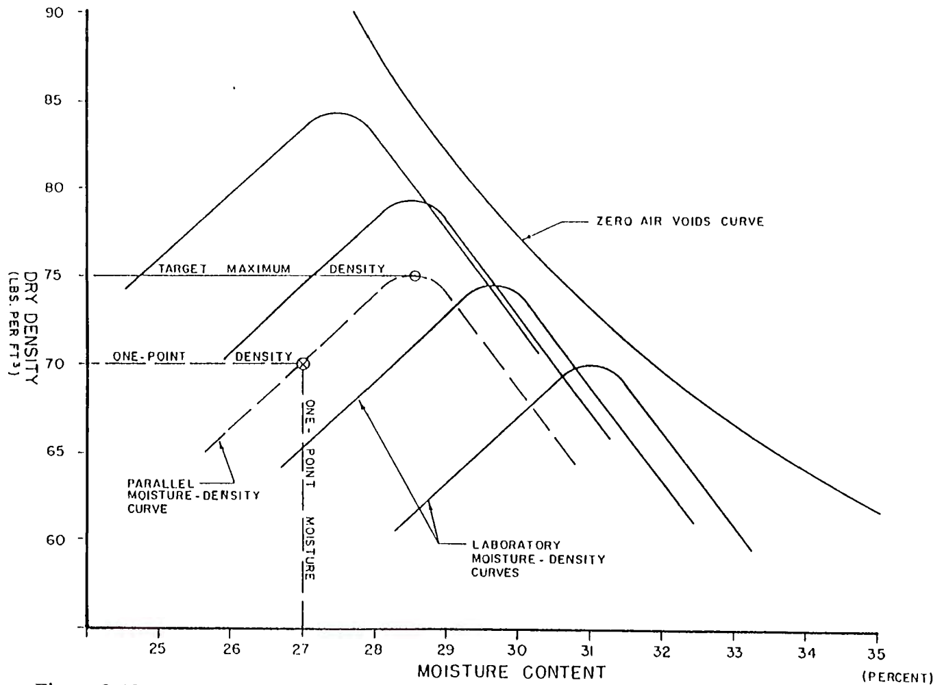
Figure 2.19 Determination of Maximum Dry Density Value from One-point Standard Compaction Test in the I-495 and Edgemoor Road Interchange, Delaware. (Srivastava and Collins 1989)
