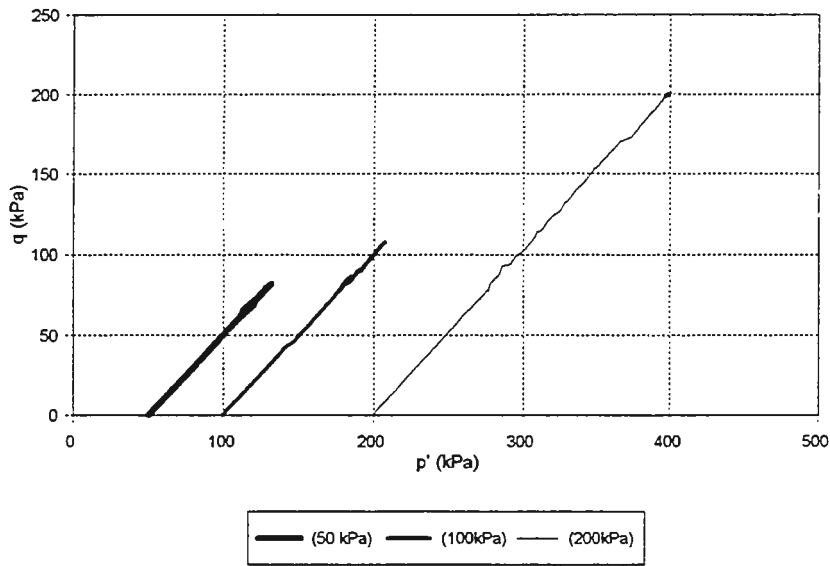
CID Triaxial, Fly/Bottom Ash Gibson Plant Ash, (F2=53%, R=90%)
