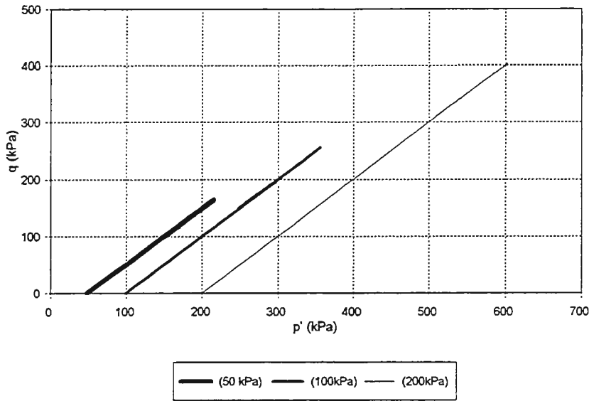
CID Triaxial, Fly/Bottom Ash Gibson Plant Ash, (F2=22%, R=95%)
