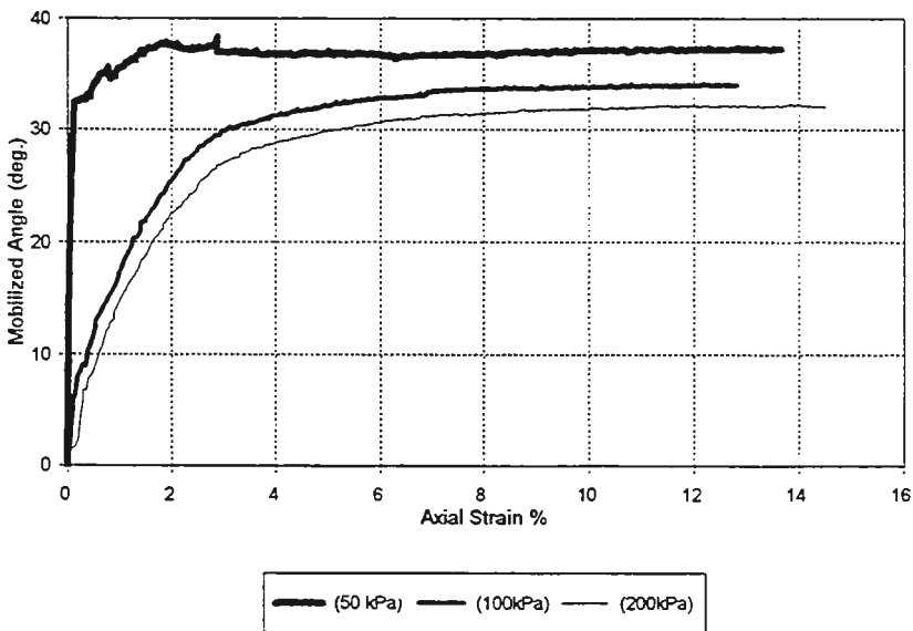
CID Triaxial, Fly/Bottom Ash Schahfer Plant Ash, (F1=50%, R=90%)
