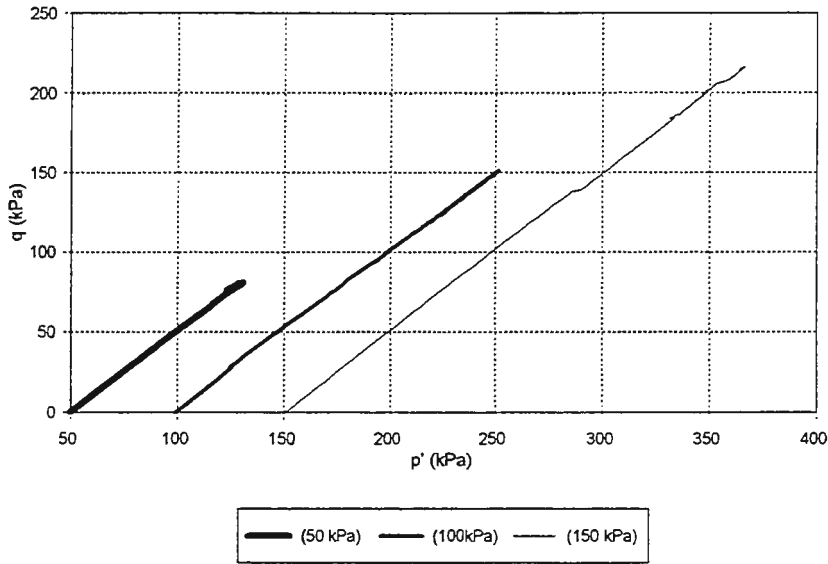
CID Triaxial, Fly/Bottom Ash Schahfer Plant Ash, (F1=25%, R=90%)
