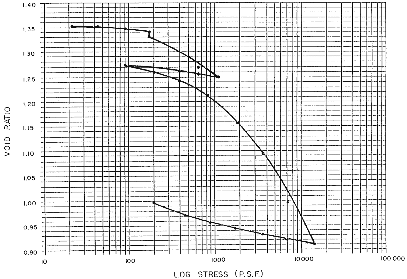
Figure 2.13 Consolidation Test Data on Delmarva Stockpiled Class F Fly Ash Utilized in the Delaware Demonstration Project. (Srivastava and Collins 1989)
