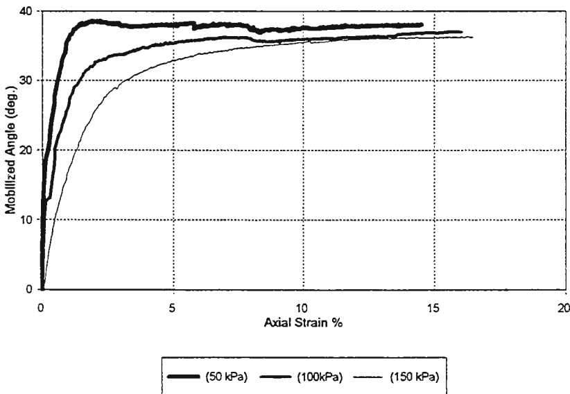
CID Triaxial, Fly/Bottom Ash Schahfer Plant Ash, (F1=25%, R=90%)
