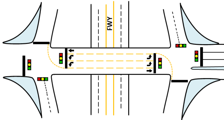
Figure 4. Illustration. DRLT-interchange design used in this experiment.
