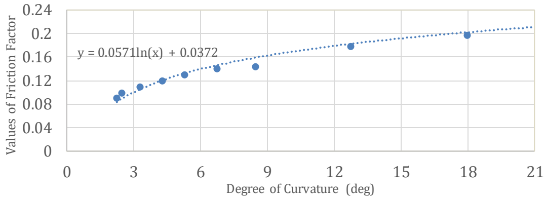
Figure 3.3 The friction factor vs. degree of curvature
