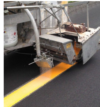
Figure 8: Thermoplastic markings applied with the push cart.
