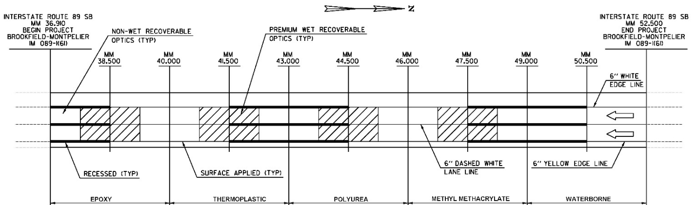
EXPERIMENTAL PAVEMENT MARKING LAYOUT
