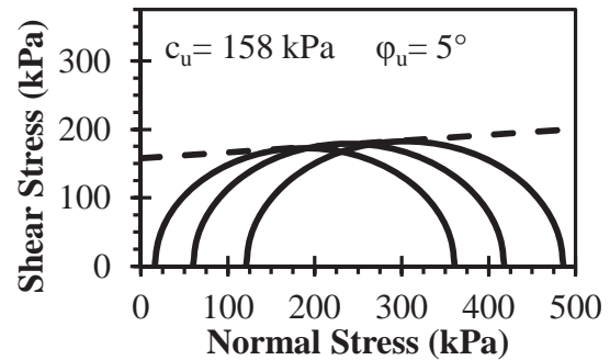
Figure 6.16. UU Triaxial Results: Memphis 10% C_{dry} LL% Initial w_c
