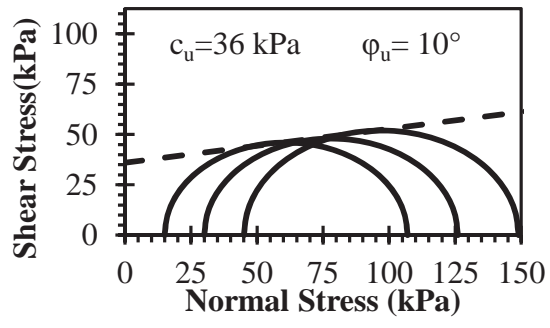
Figure 6.17. UU Triaxial Results: Memphis 5% C dry 100% Initial w c
