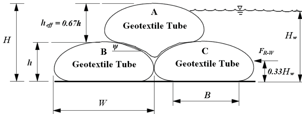
Figure 9.3. Dimensions for tubes filled with LC-VHMS (Howard et al., 2011)
