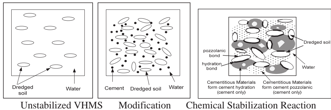
Figure 6.1. Schematic Diagram of VHMS Stabilization Process
