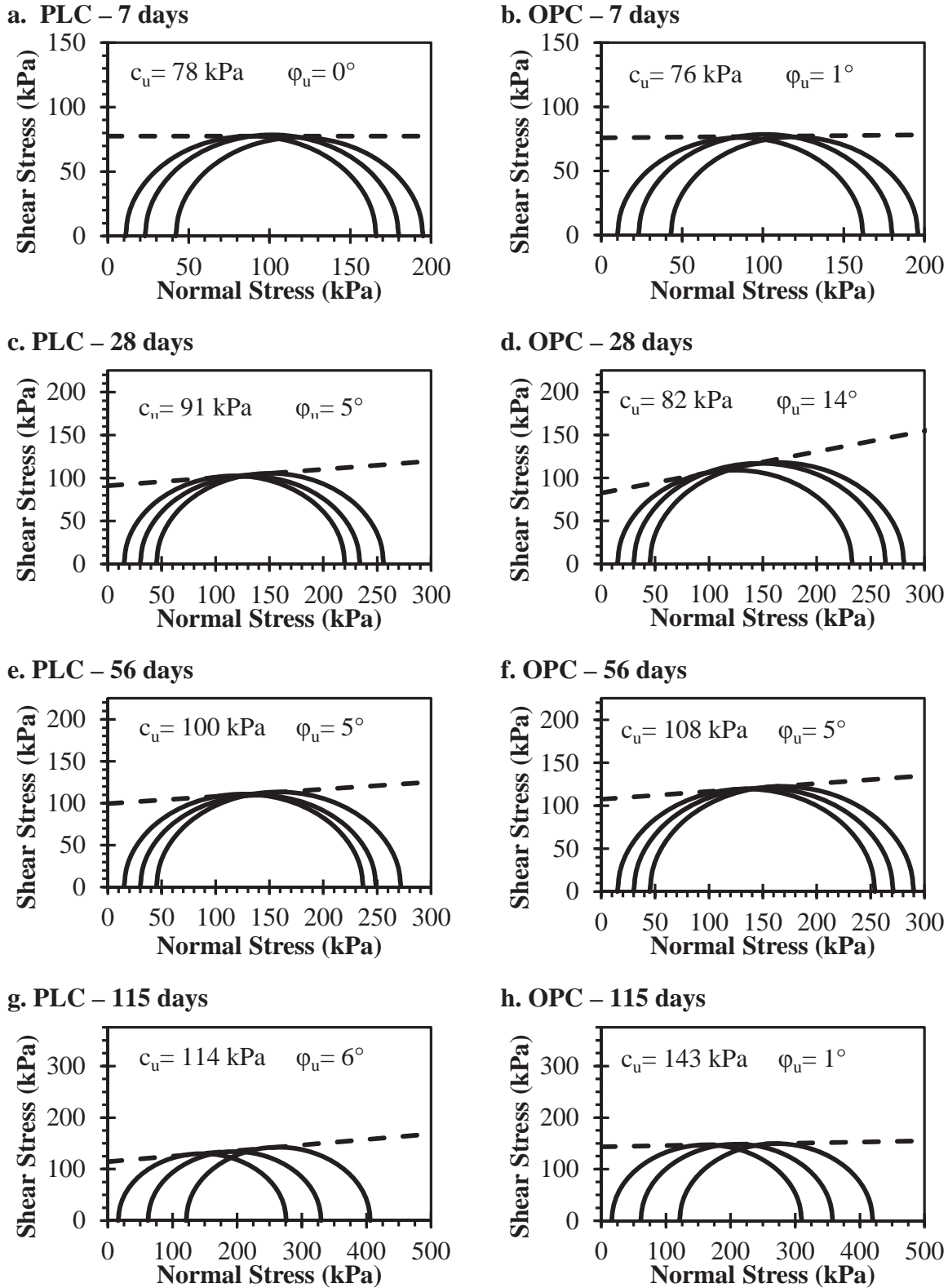
Figure 6.18. UU Triaxial Results: Memphis 10% C_{dry} 100% Initial w_c
