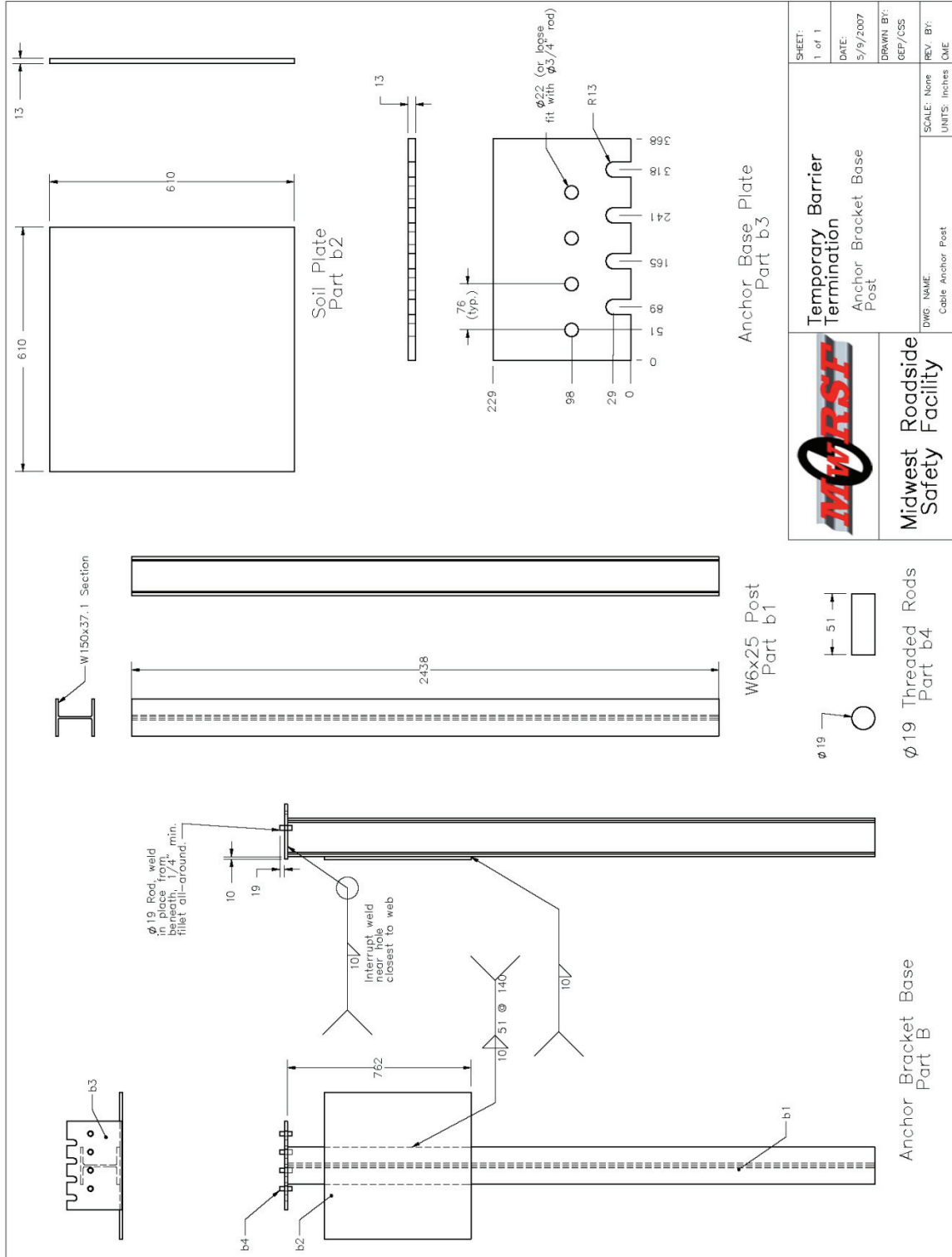
Figure A-12. Termination of Temporary Concrete Barrier, Test No. TTCB-1
