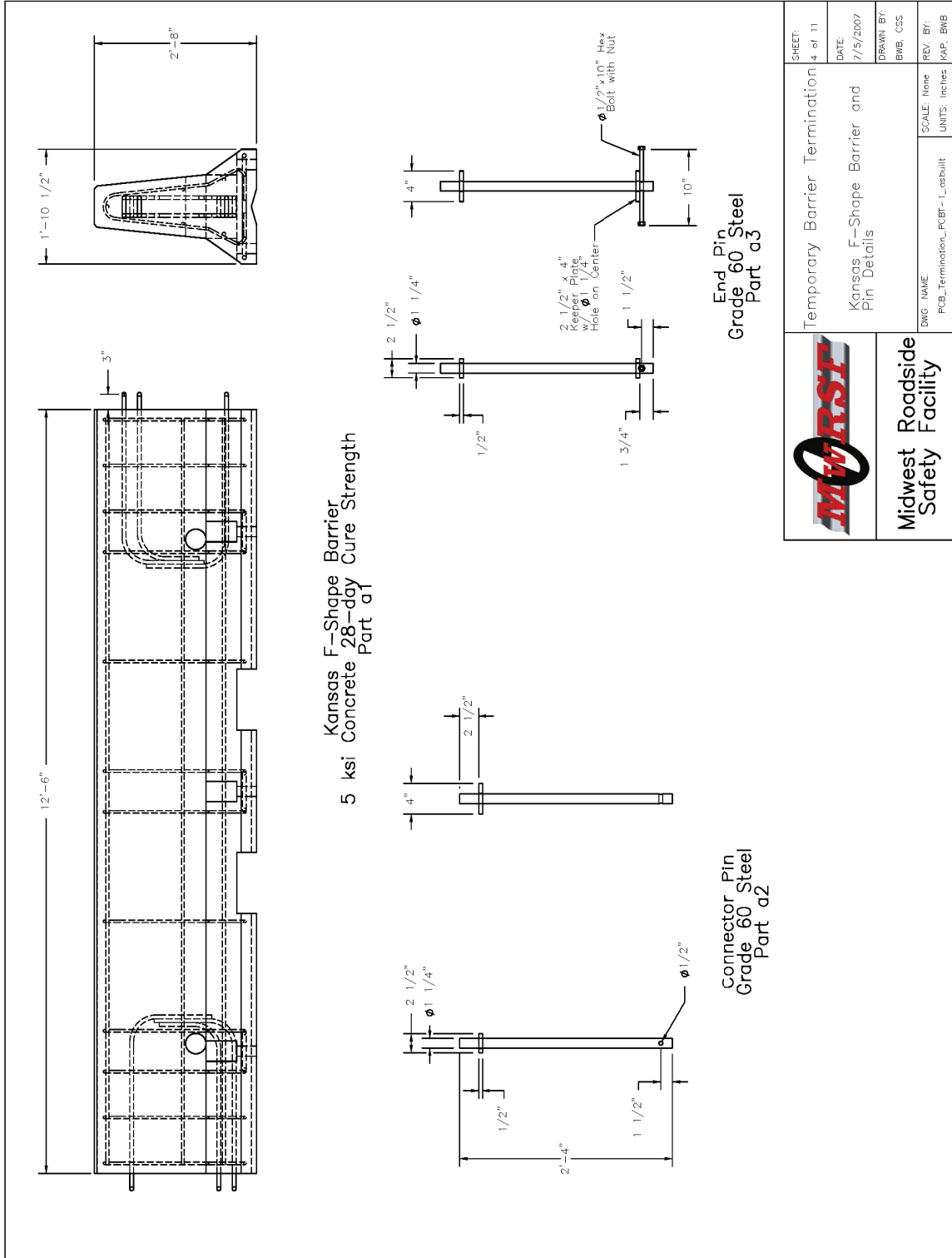
Figure 11. Temporary F-Shape Barrier and Pin Details, Test No. TTCB-1
