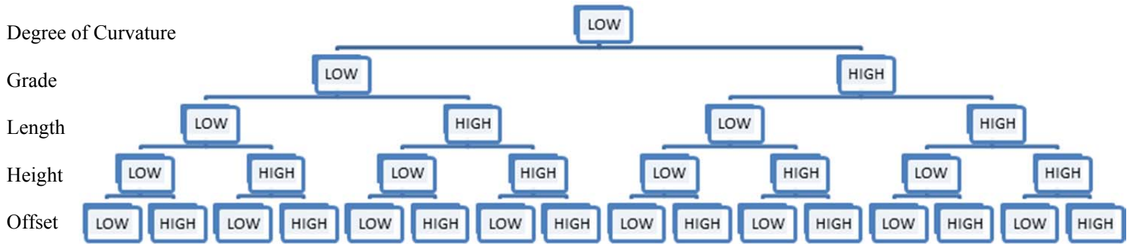
Figure 15. Interpolation Tree used in BCAF
