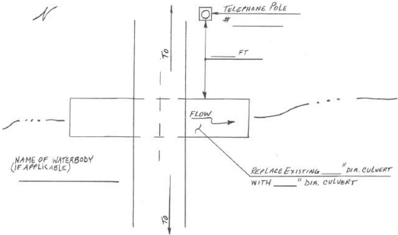
REPLACE CULVERT AT SAME LOCATION
