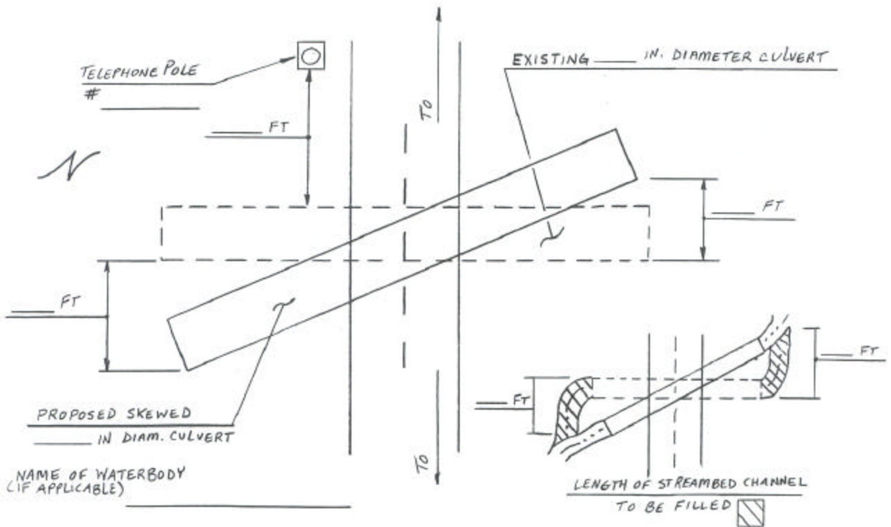
SKEWING AN EXISTING CULVERT
