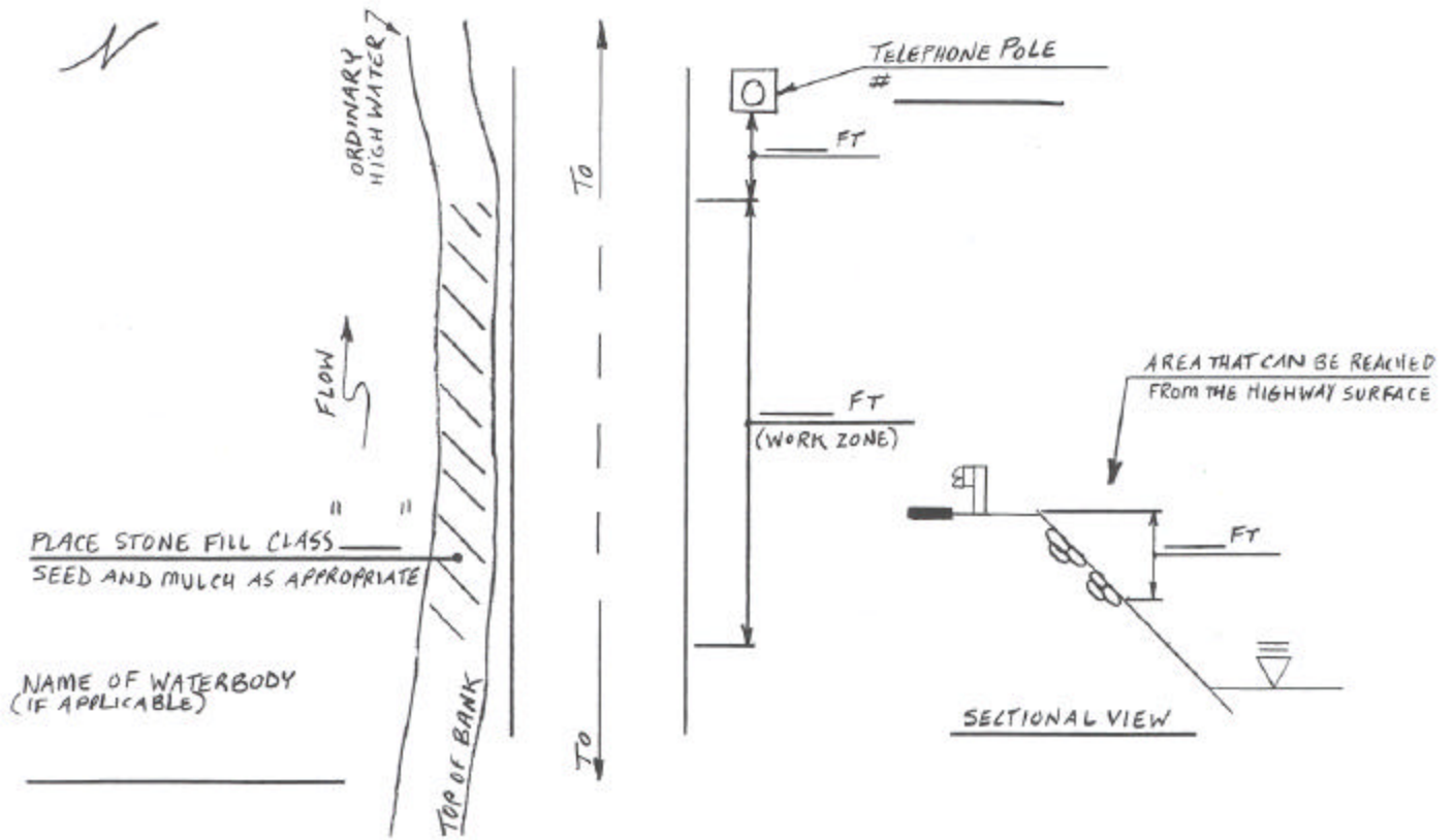
EMBANKMENT STABILIZATION
