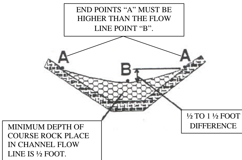
FRONT VIEW
