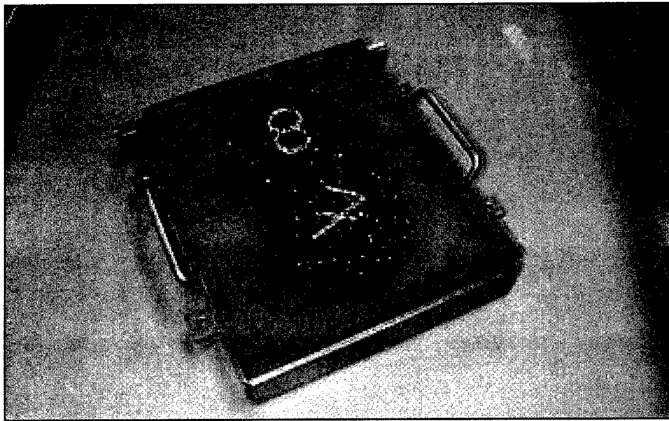
Figure 4 Test Specimen Configuration for the Hamburg Wheel-Tracking Device with Superpave Gyratory Compacted Specimens
