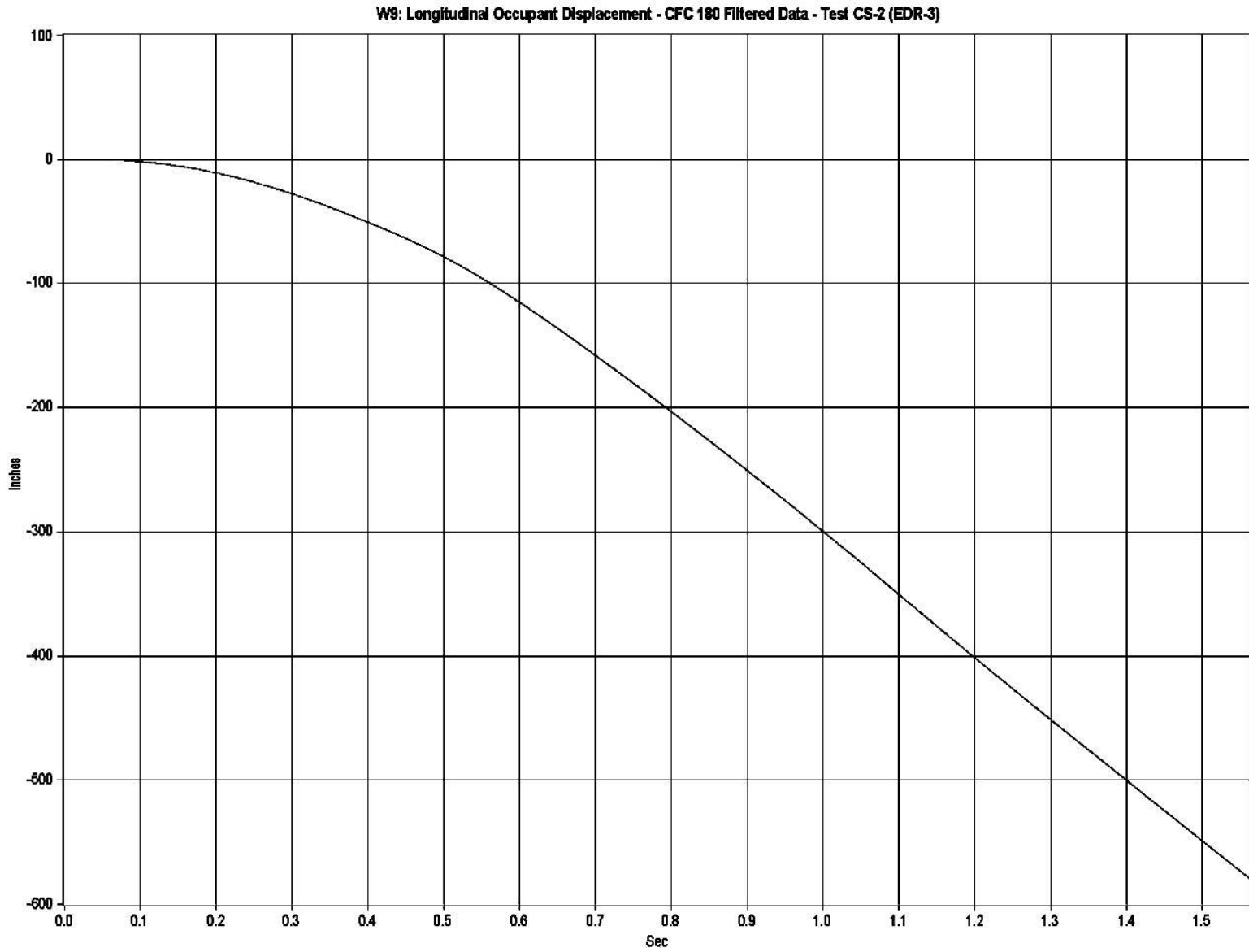
Figure D-3. Graph of Longitudinal Occupant Displacement, Test CS-2
