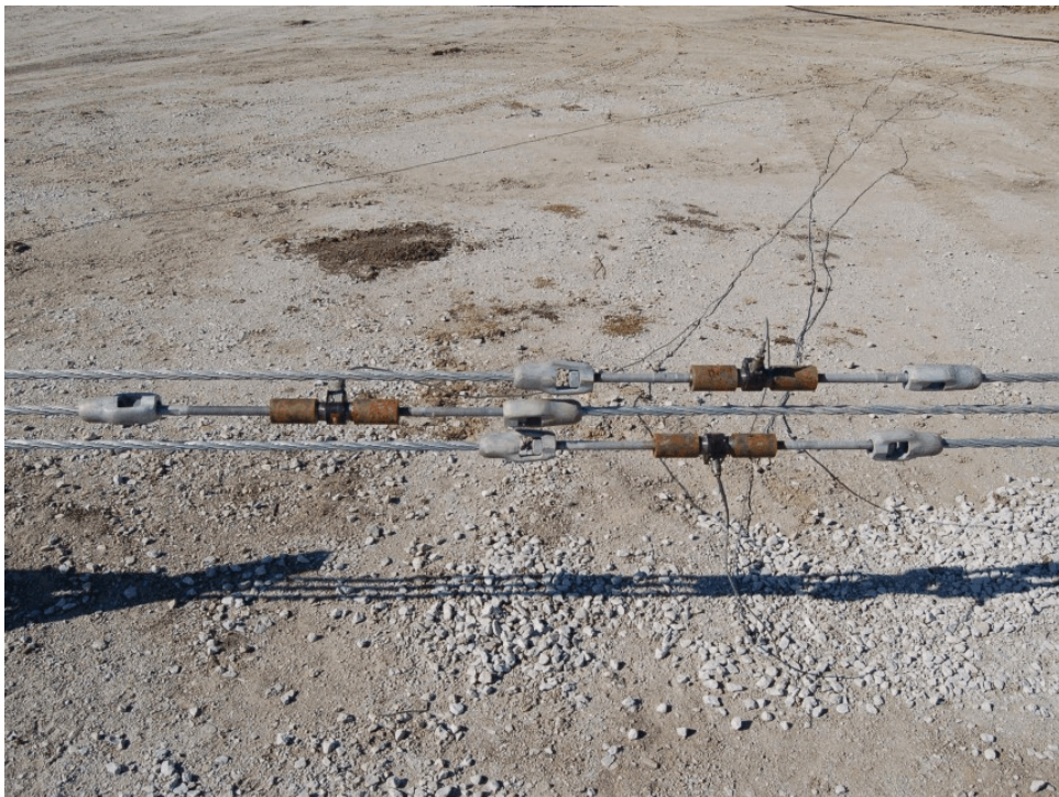
Figure 5. Upstream End Load Cell Positioning
