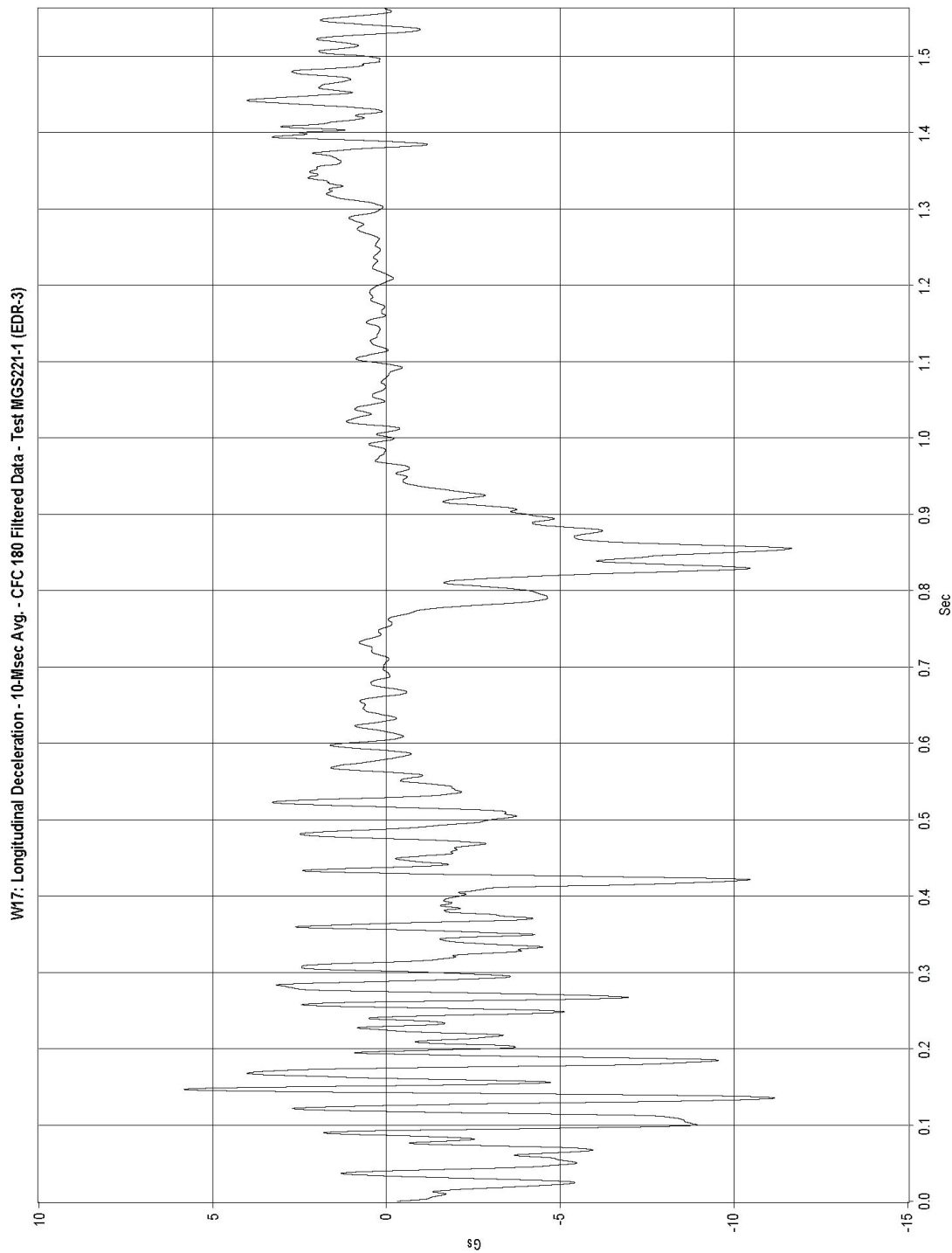
Figure F-1. Graph of Longitudinal Deceleration, Test MGS221-1
