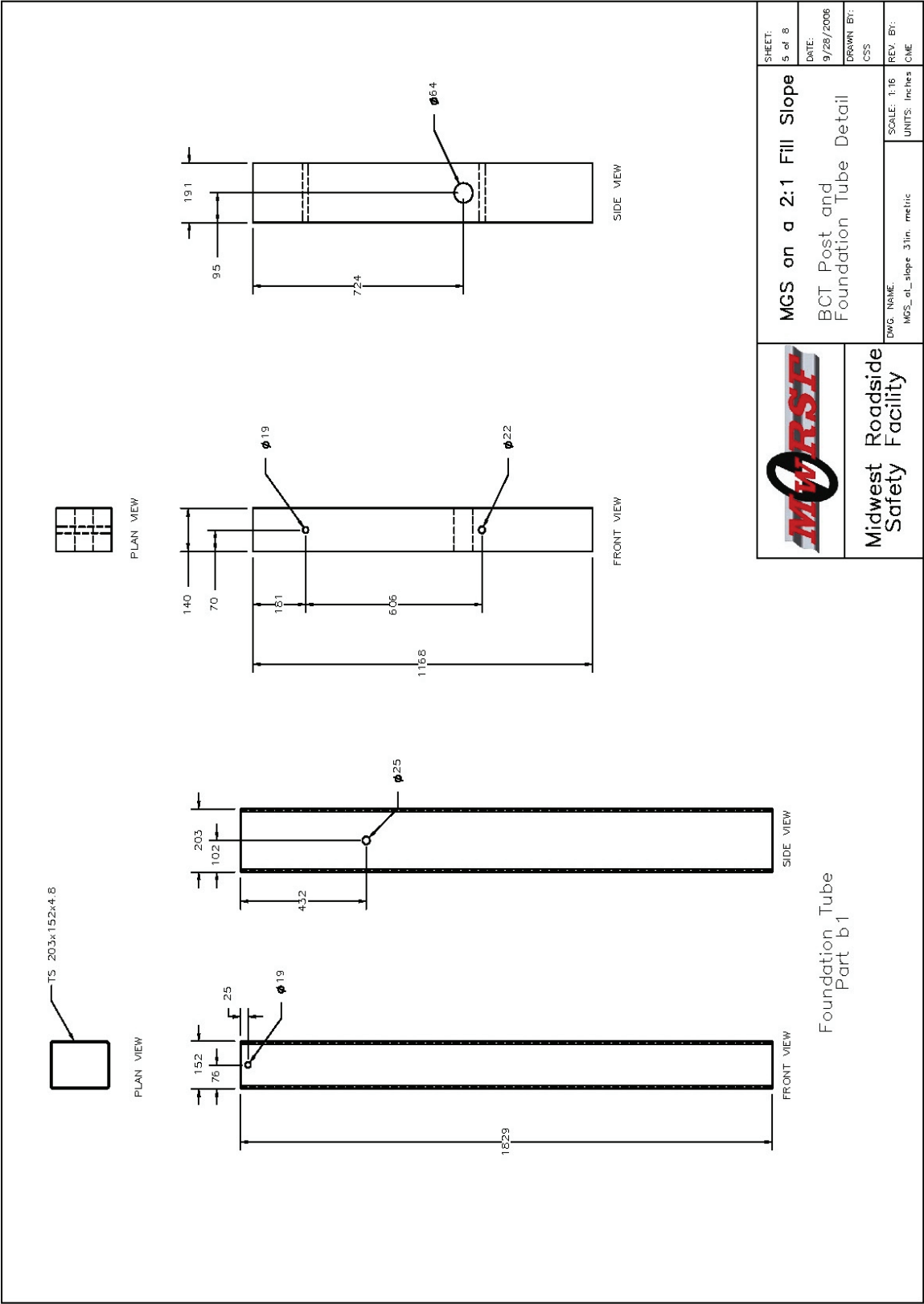
Figure G-5. Post and Foundation Tube Details, Test No. MGS221-2 (Metric)
