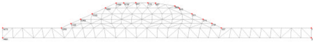
Fig. 5 Plot of the mesh with significant nodes
