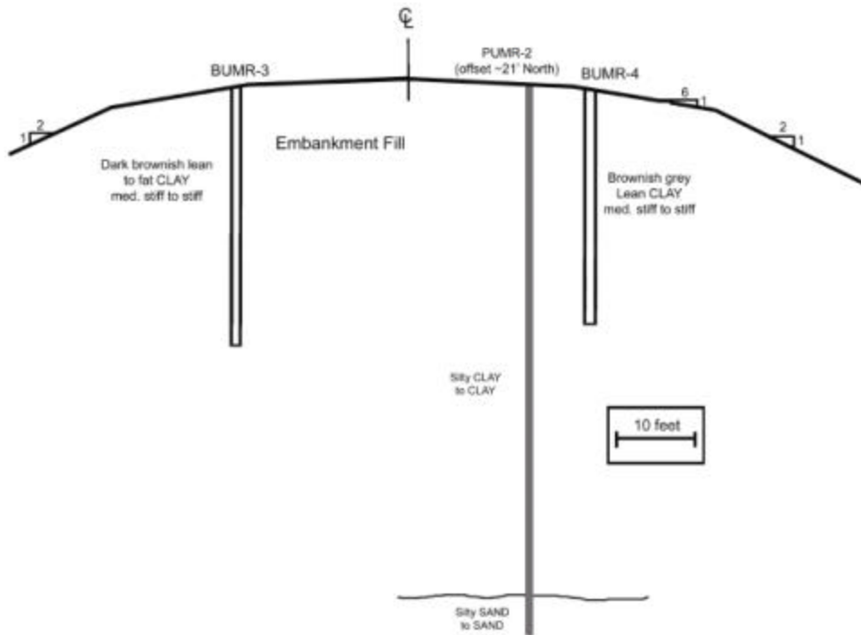
Cross-section A-A' (see figure 4.2 for plan view)
