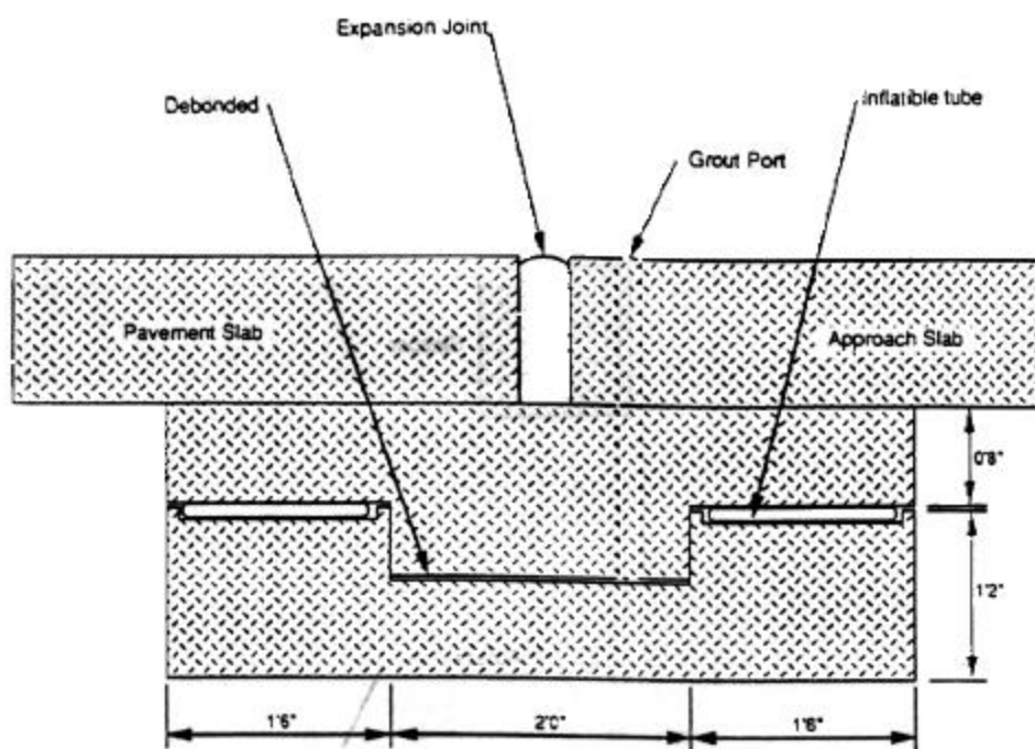
Figure A.16- Pneumatic Adjustable Sleeper, Tadros and Benak (1989).
