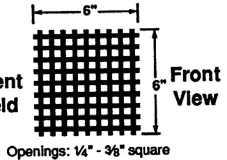
Figure 5.2. Design plans for precast concrete headwall with removable rodent screen (FHWA, 1992).
