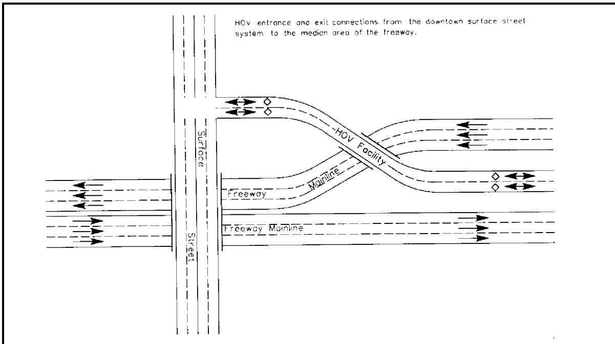
Figure 6-18. Terminal Flyover Connection to Surface Street System. (10)
