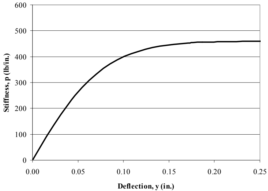
Figure 3.6. Example of a typical stiffness-deflection (p-y) curve.
