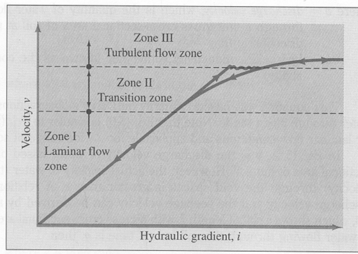
Figure 3. Flow Zones
