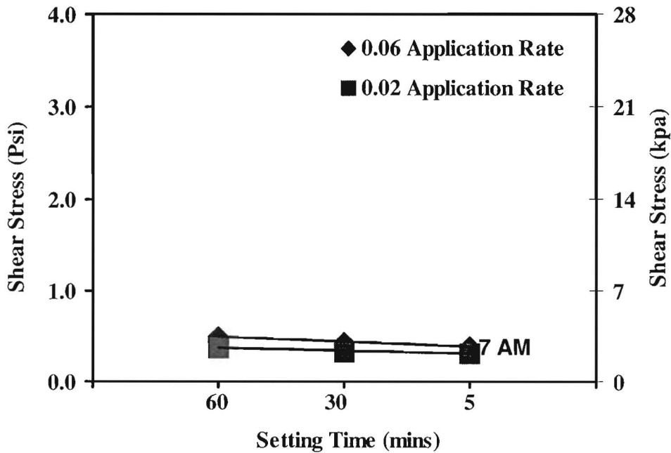
Figure 4.25 - ATACKER™ Parking Lot Test results for PG64-22 Tested at 7AM
