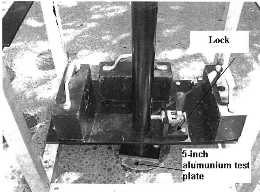
Figure 2.20 - ATACKER™ Field Test Set-Up
