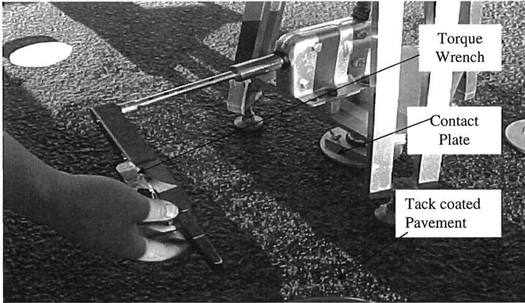
Figure 6.6 - Torque Wrench used during UPOD Testing
