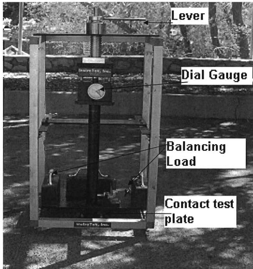
Figure 2.19 - ATACKER™ Test Set-Up
