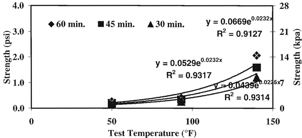
Figure 7.10 - UPOD Laboratory Test Results for SS-1h
