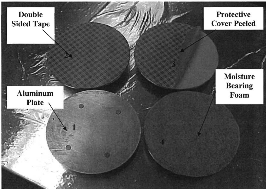
Figure 6.7 - Contact Test Plates for UPOD
