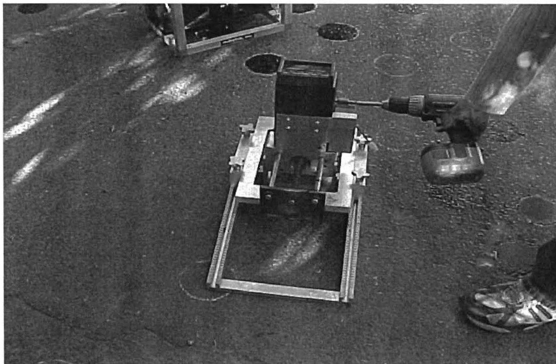
Figure 3.3 - Field Testing of Koch Materials Company Test Set-Up
