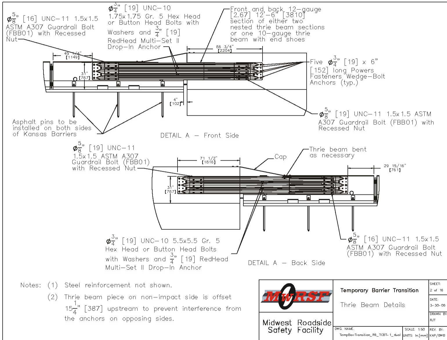
Figure 5. Thrie Beam Details, Test Nos. TCBT-1 and TCBT-2
