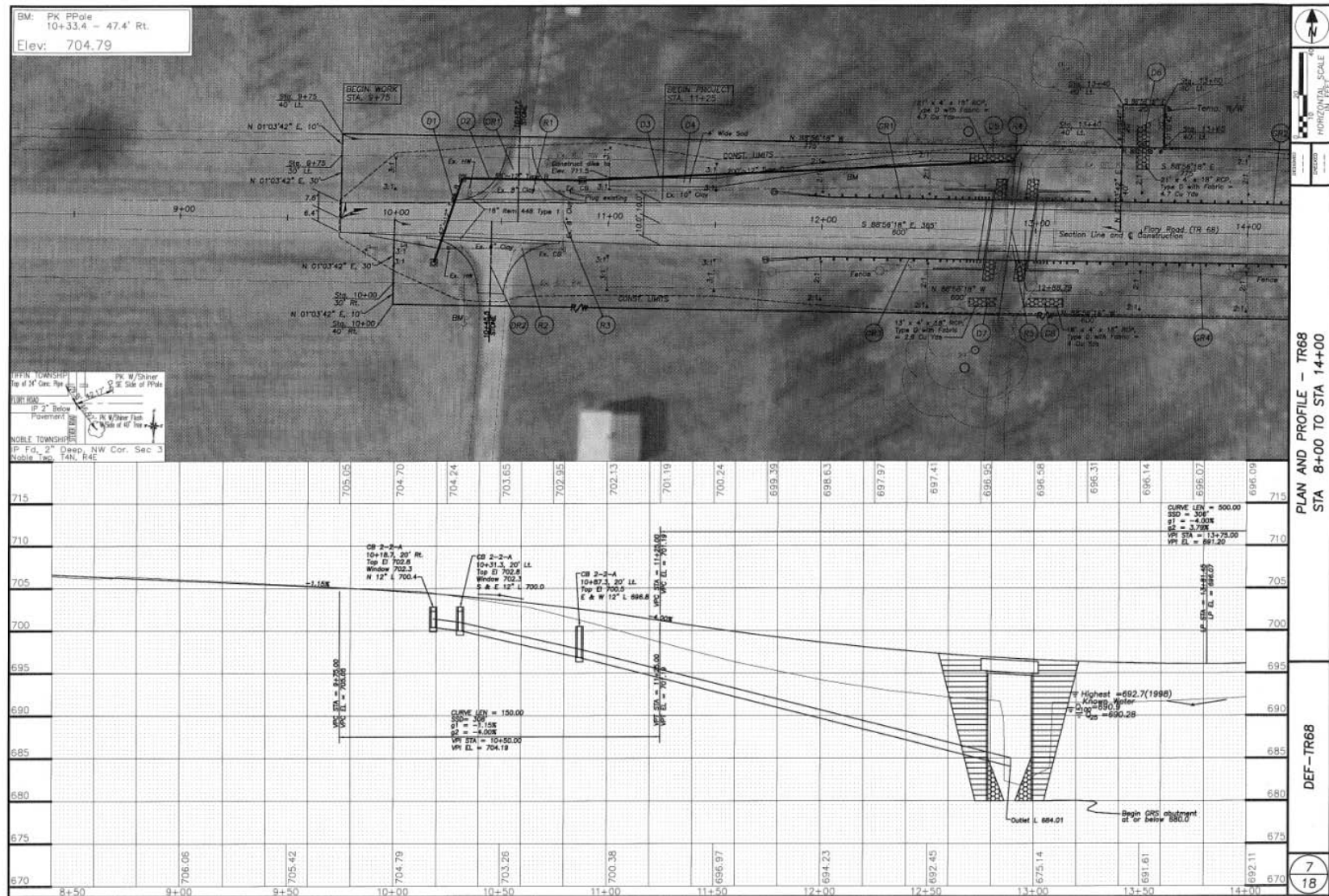
Figure 102. Illustration. Project plan and profile.
