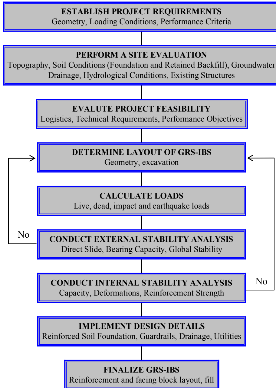
Figure 9. Chart. Steps for GRS-IBS design.
