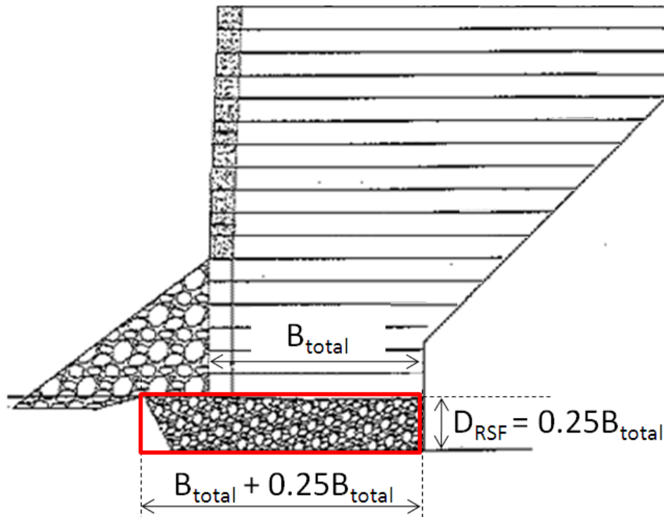
Figure 12. Illustration. RSF dimensions.
