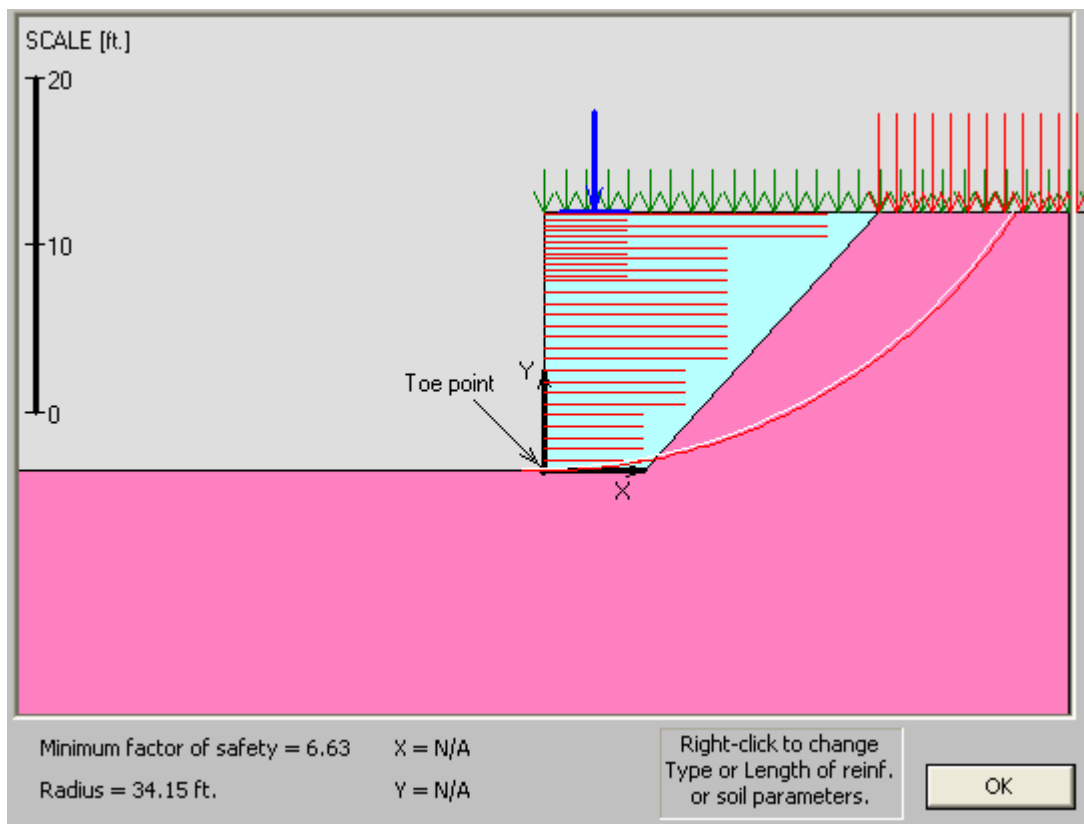
Figure 31. Screenshot. ReSSA results for global stability for Bowman Road Bridge.
