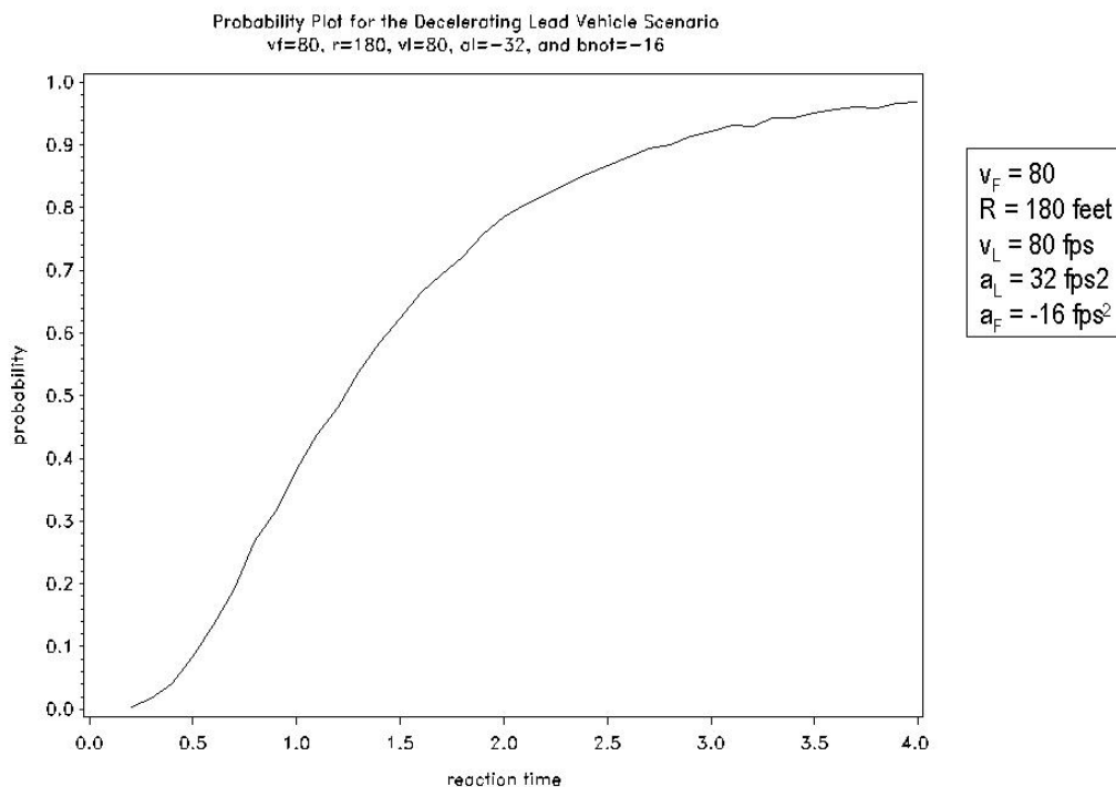
Figure 6-3. Analytical Model Developed for a Slice of the Lead Vehicle Decelerating 6-D Driving Conflict Space
