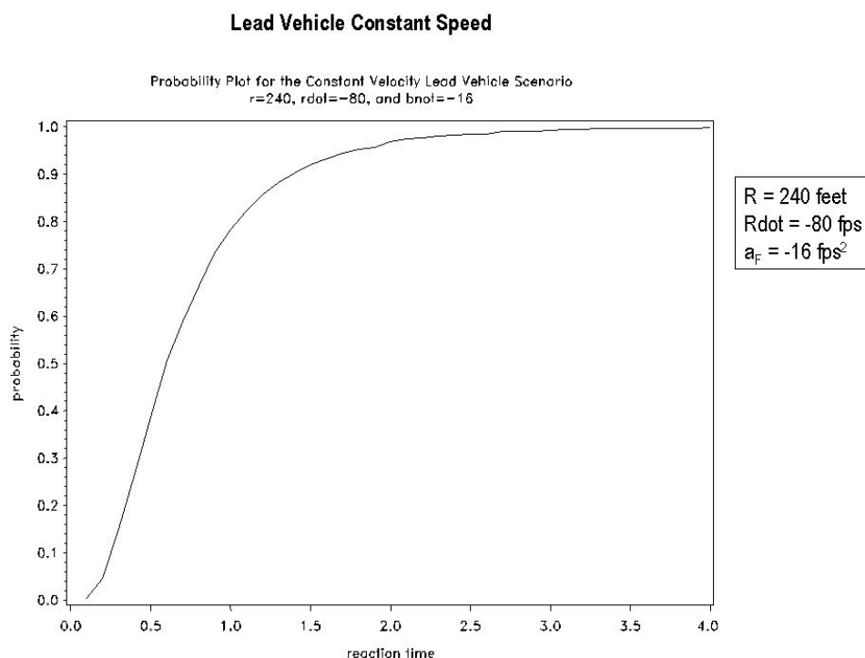
Figure 6-2. Analytical Model Developed for a Slice of the Lead Vehicle Stopped/Constant Speed Four-Dimensional Driving Conflict Space
