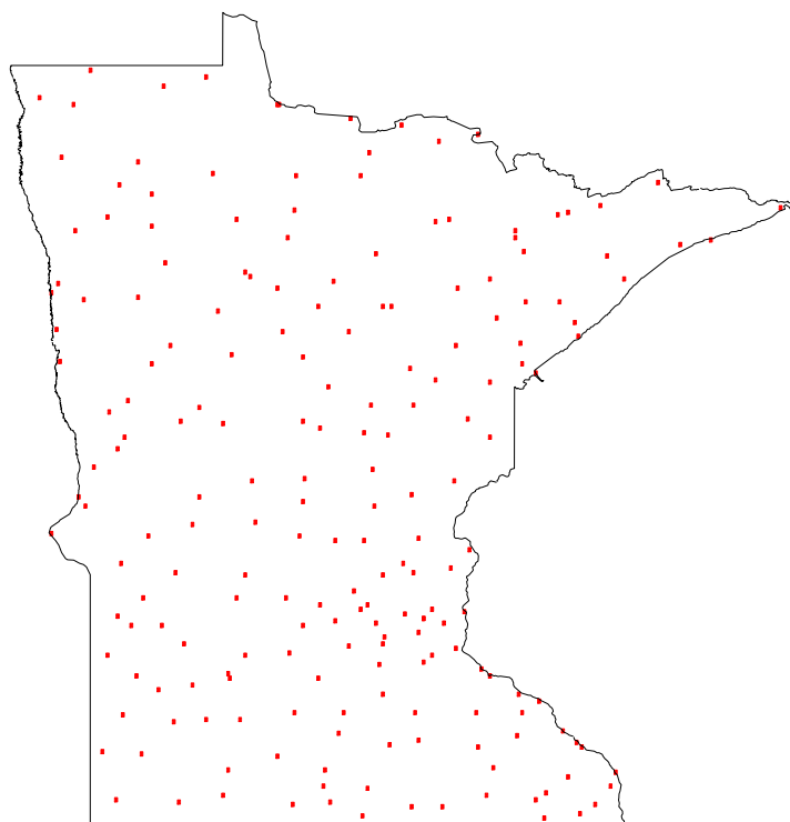
Figure 5-4. Minnesota Weather Stations
