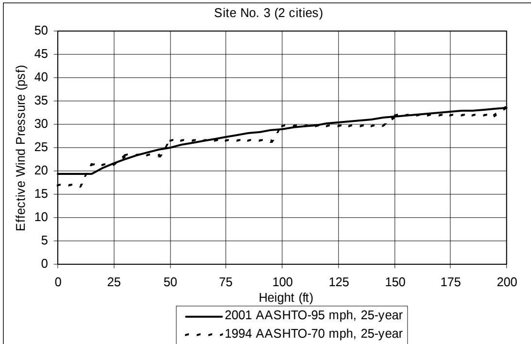
Figure B-12. Site no. 3: effective wind pressure
