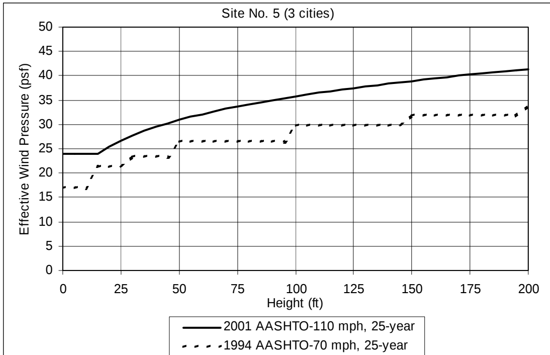
Figure B-16. Site no. 5: effective wind pressure
