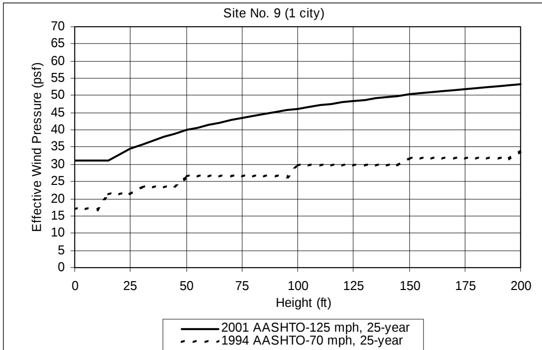
Figure B-24. Site no. 9: effective wind pressure
