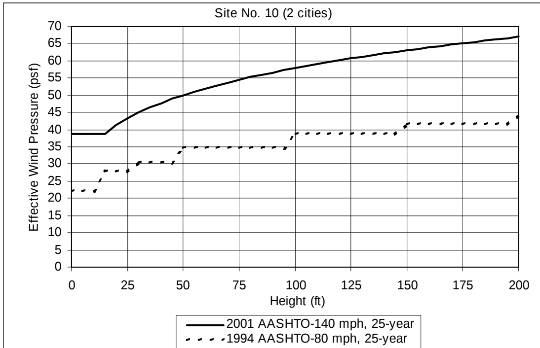
Figure B-26. Site no. 10: effective wind pressure
