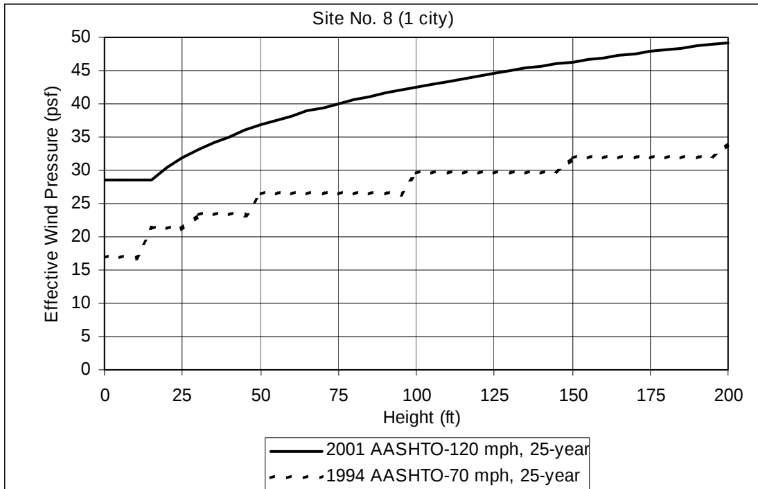
Figure B-22. Site no. 8: effective wind pressure
