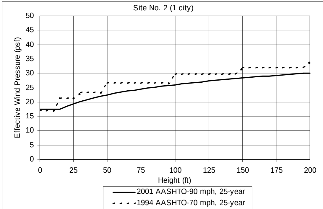
Figure B-10. Site no. 2: effective wind pressure
