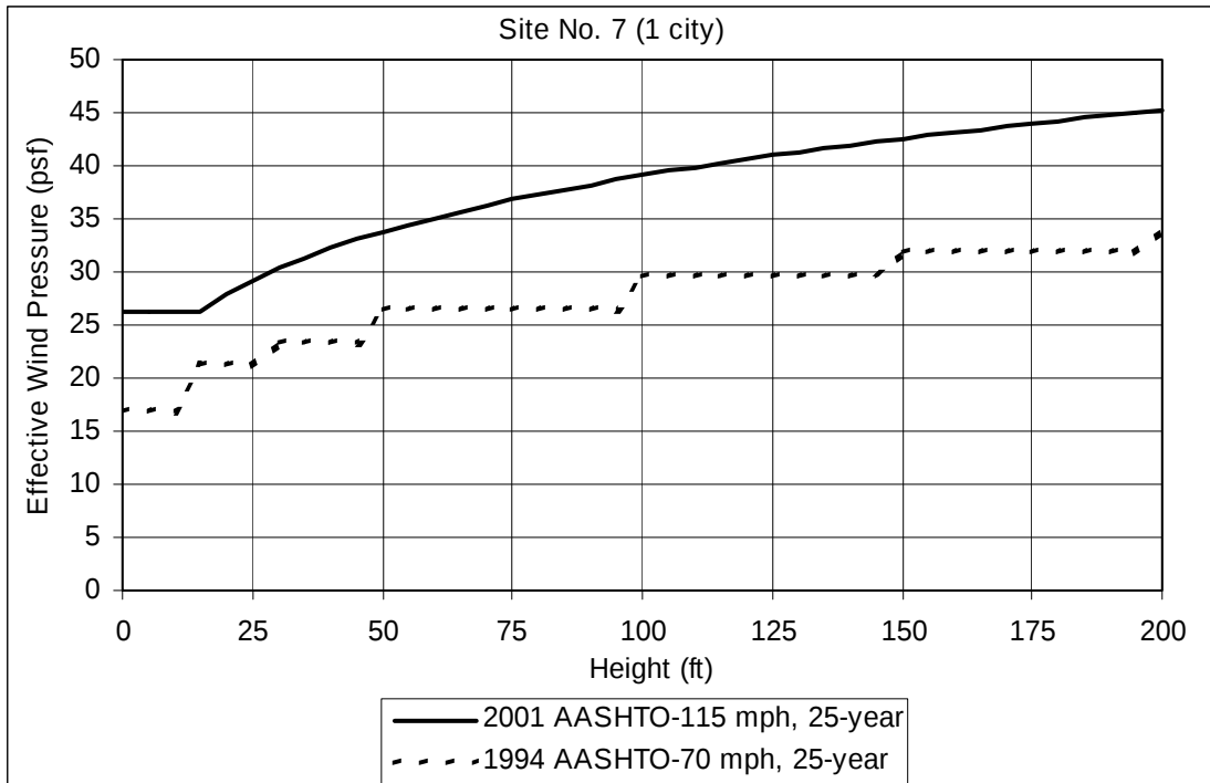
Figure B-20. Site no. 7: effective wind pressure
