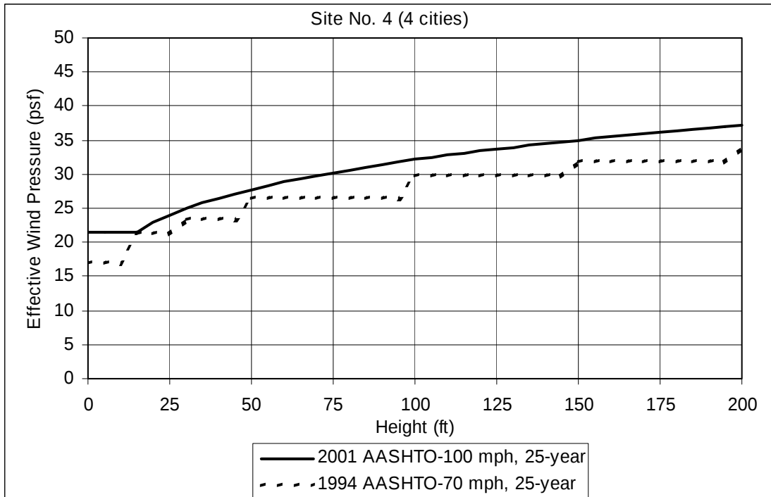
Figure B-14. Site no. 4: effective wind pressure
