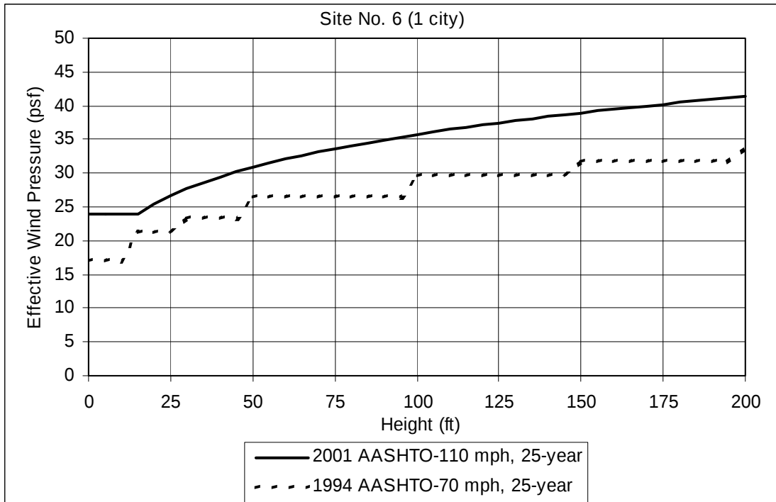
Figure B-17. Site no. 6: effective wind pressure
