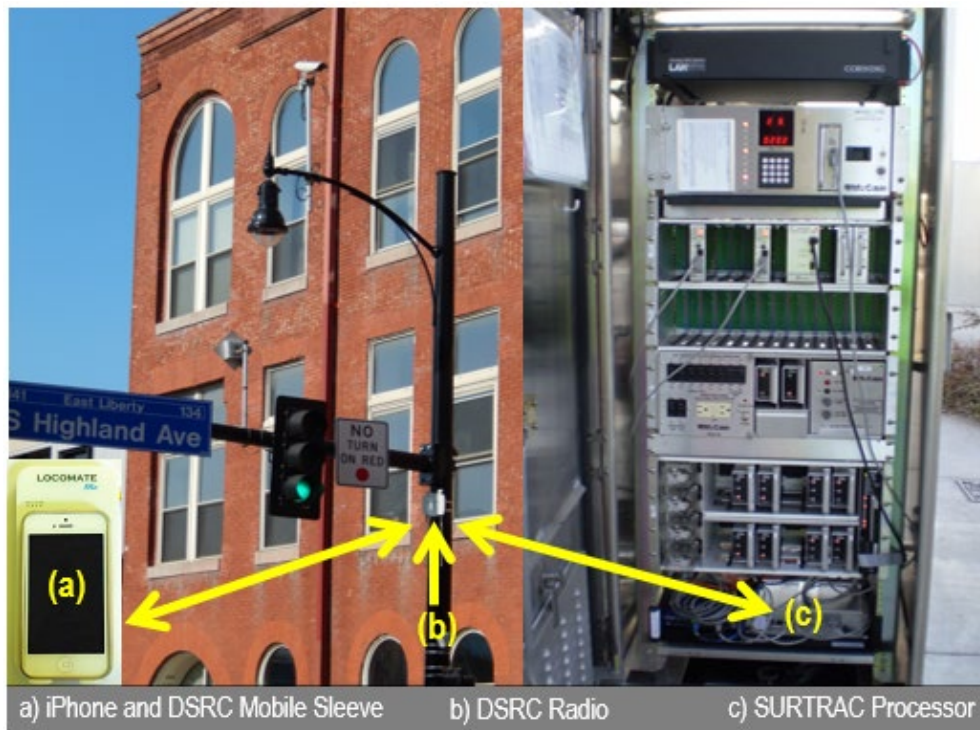
Figure 2-2: Schematic of Different Elements of the Safe Intersection Crossing Application
