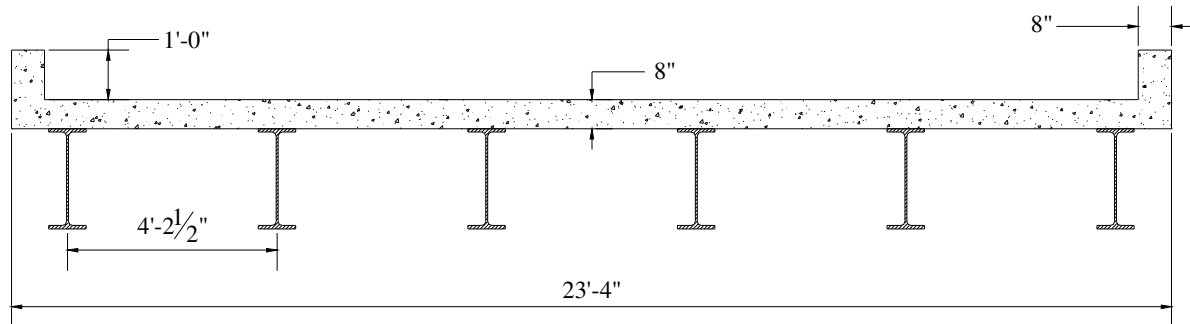
Figure 4.4. Cross Section of MCB Looking North.
