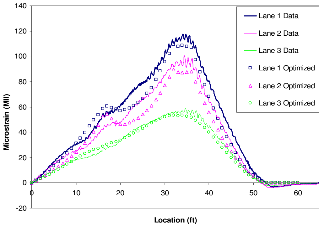
Figure 5.16. KCB1 Girder 2 Optimized Strain Comparison.
