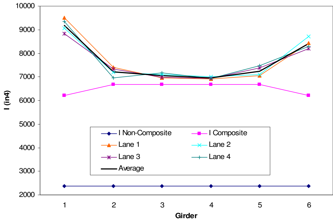
Figure 4.18. MCB Effective Moments of Inertia.
