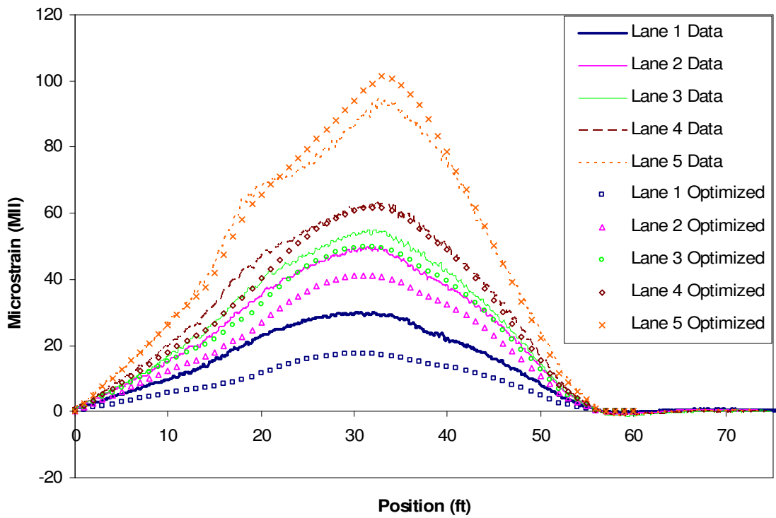
Figure 7.20. KCB2 Girder 5 Optimized Strain Comparison.
