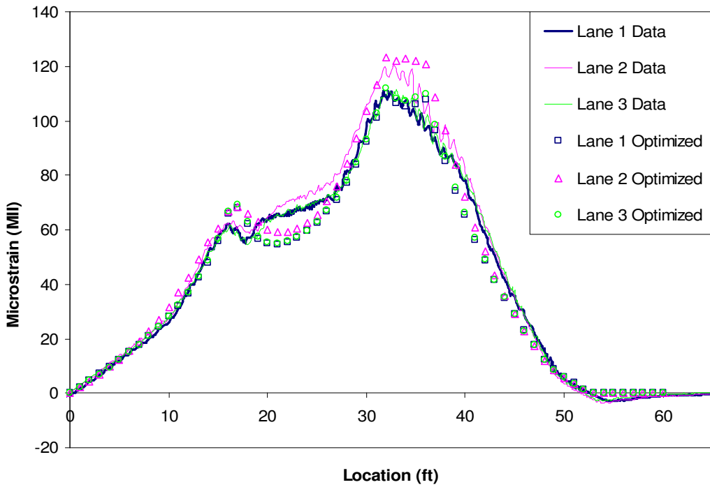
Figure 5.17. KCB1 Girder 3 Optimized Strain Comparison.
