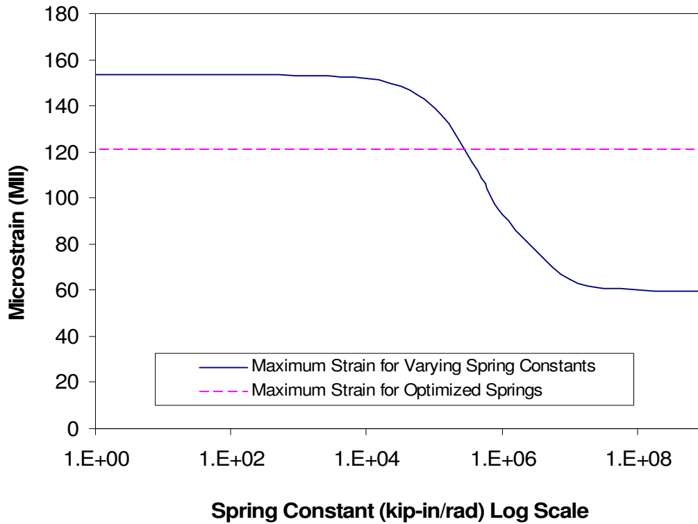
Figure 3.29. BCB Girder 1 Lane 1 Maximum Strain for Varying Spring Constants.
