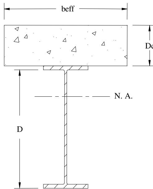
Figure 3.20. Effective Section.
