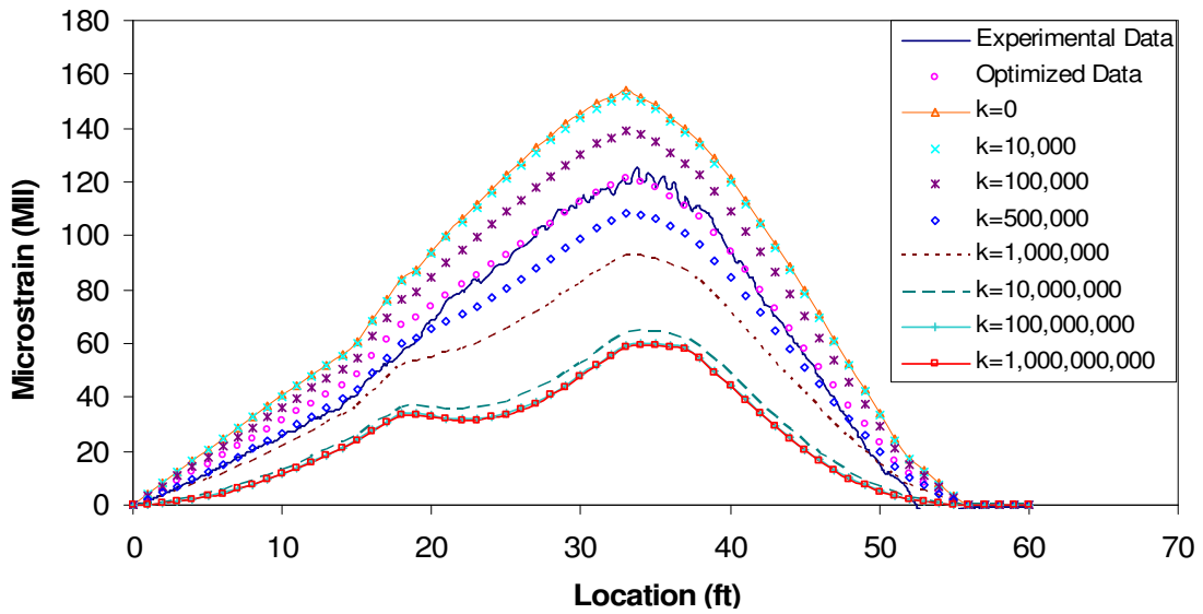
Figure 3.28. BCB Spring Constant Comparison for Lane 1 Girder 1.
