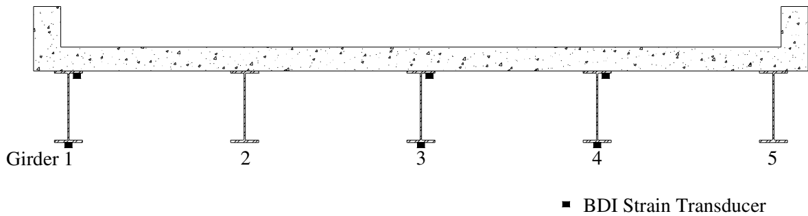
Figure 5.8. KCB1 North and South End Transducer Locations Looking North.
