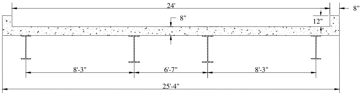
Figure 8.3. Cross Section of HCB Looking West.
