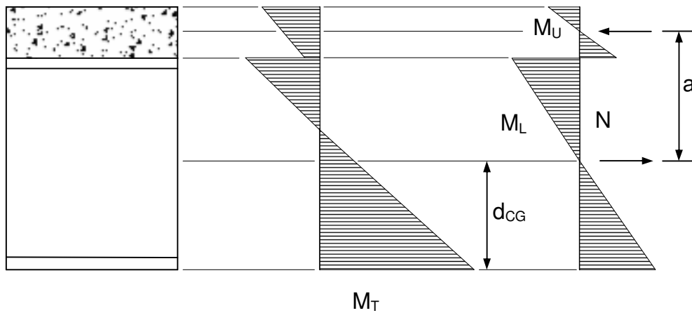
Figure 2.4. Girder - Concrete Stress Profile.
