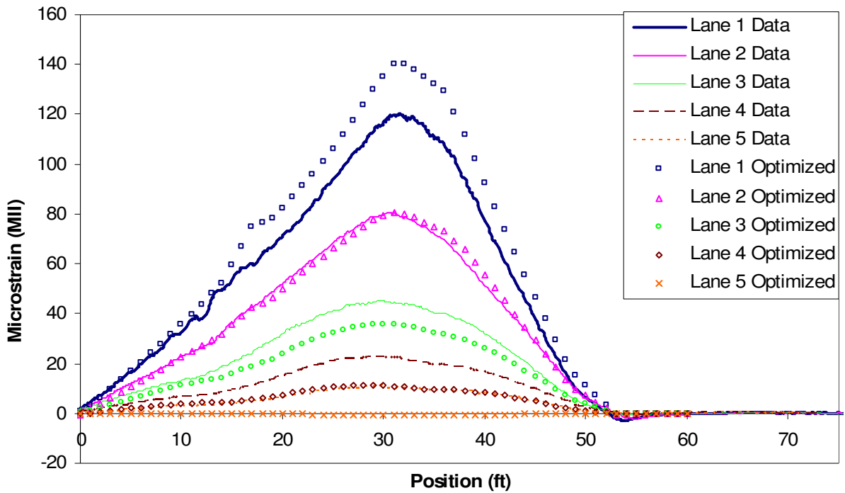
Figure 8.17. HCB Girder 1 Optimized Strain Comparison.
