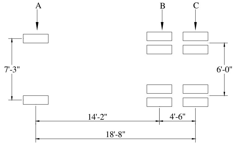
Figure 8.5. HCB Test Truck Dimensions
