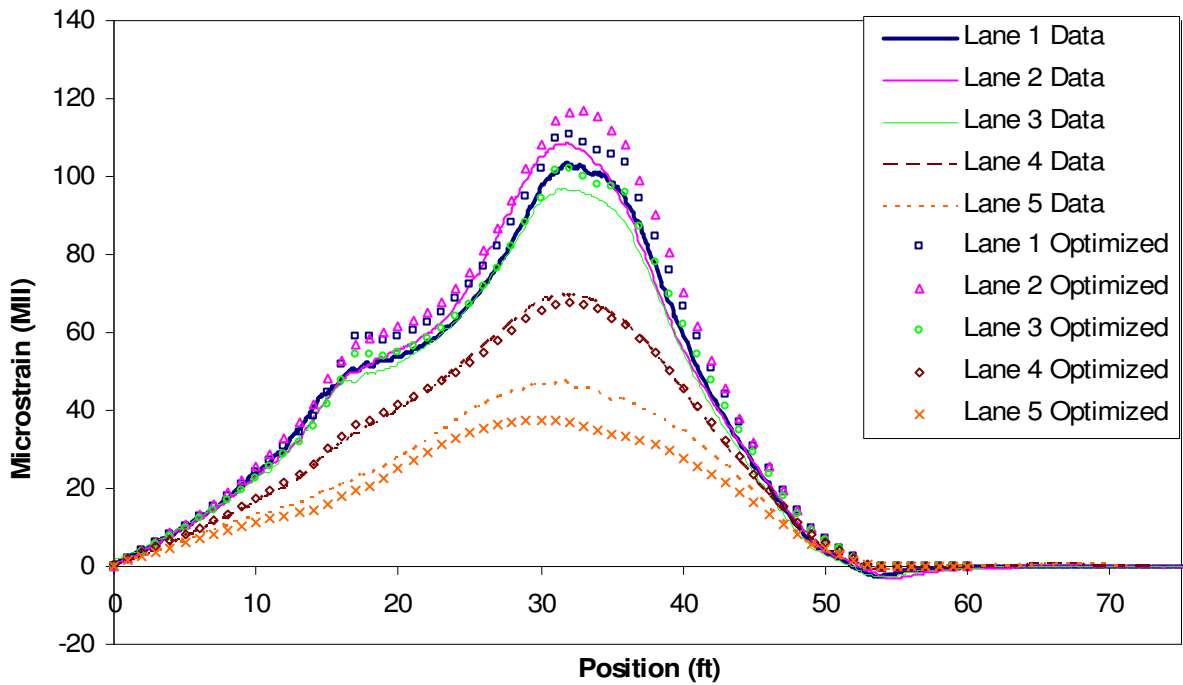
Figure 8.18. HCB Girder 2 Optimized Strain Comparison.
