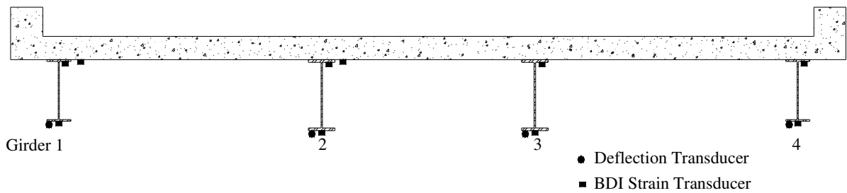
Figure 8.9. HCB Midspan Transducer Locations Looking West.
