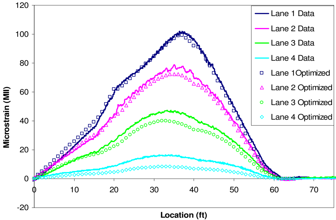
Figure 4.19. MCB Girder 1 Optimized Strain Comparison.
