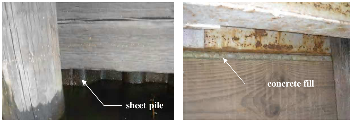
Figure 3.4. BCB Deterioration.
