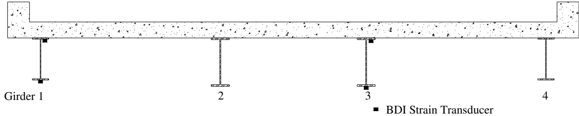
Figure 6.9. CCB South End Transducer Locations Looking North.
