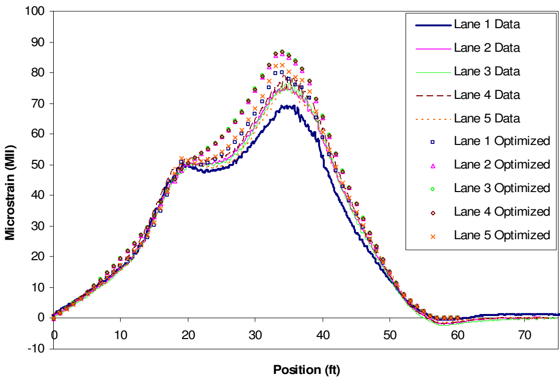
Figure 7.18. KCB2 Girder 3 Optimized Strain Comparison.
