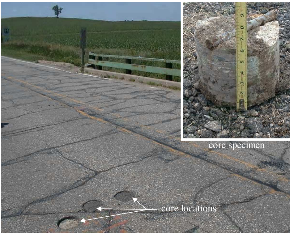
Figure 4.3. MCB Core Locations and Retrieved Core Specimen.
