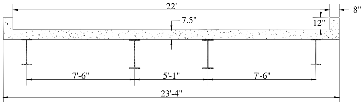
Figure 6.3. CCB Cross Section Looking North.
