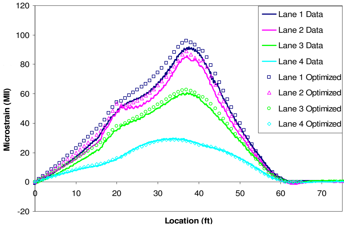
Figure 4.20. MCB Girder 2 Optimized Strain Comparison.
