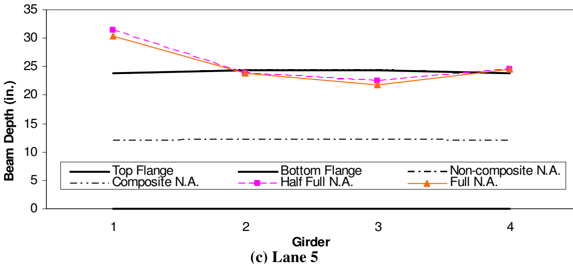
Figure 8.16.HCB Neutral Axis Locations.
