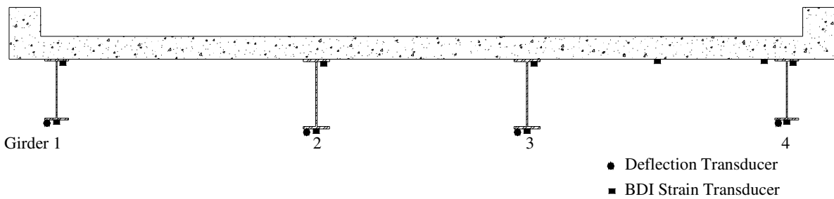
Figure 6.8. CCB Midspan Transducer Locations Looking North.
