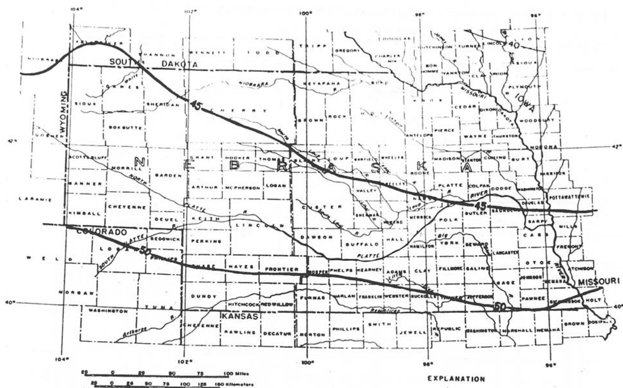
Figure 2.11: Normal daily March temperature, T_3 (Cordes and Hotchkiss, 1993)
