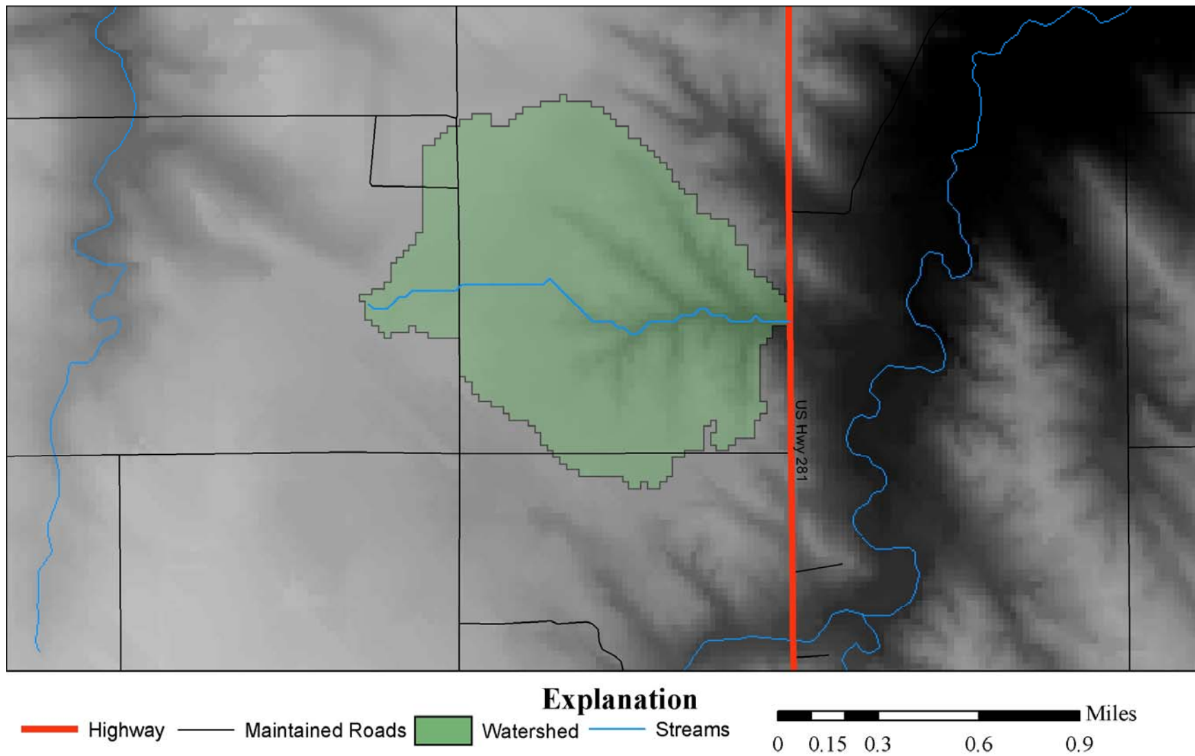
Figure 5.11: Site located north of O'Neill, Nebraska on U.S. Highway 281.
