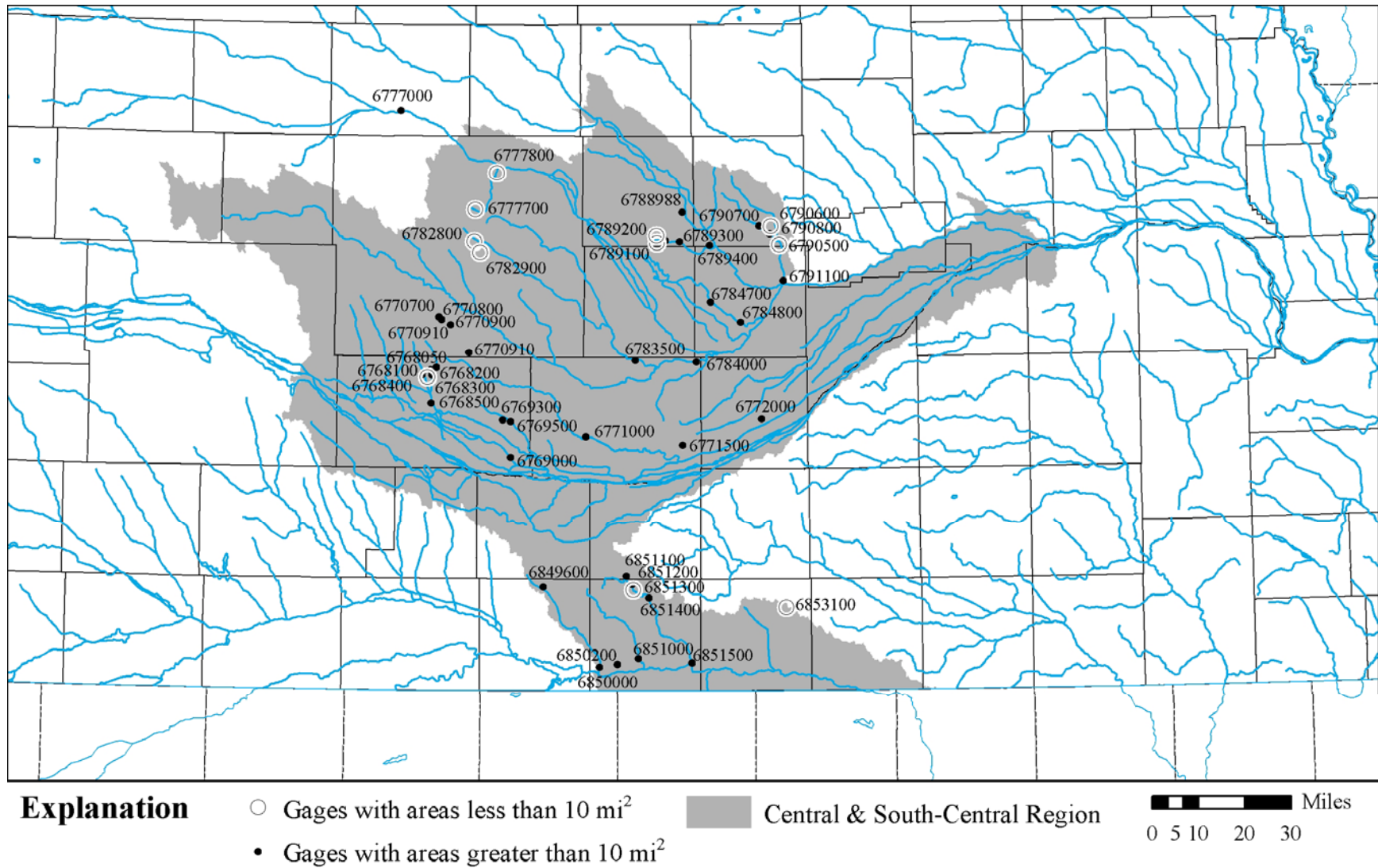
Figure 4.4: Location of streamflow gaging stations used in the Central and South Central regression analysis.
