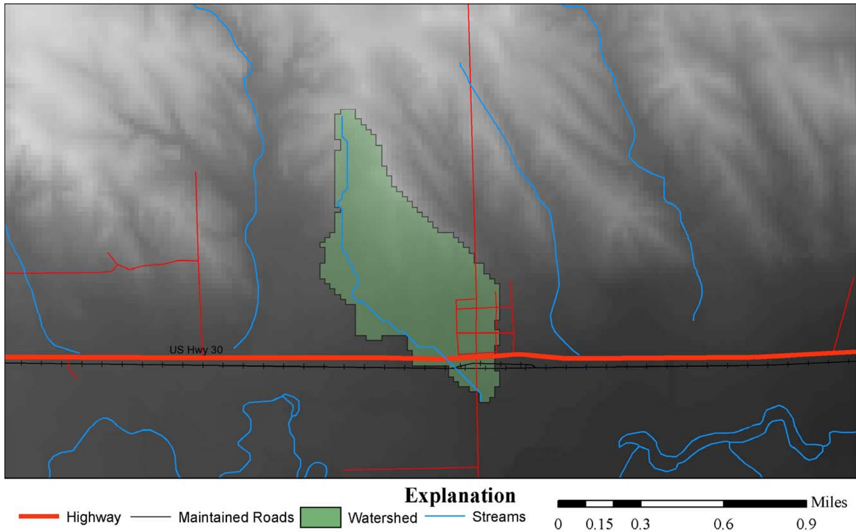
Figure 5.13: Site located at Sunol, Nebraska on U.S. Highway 30.
