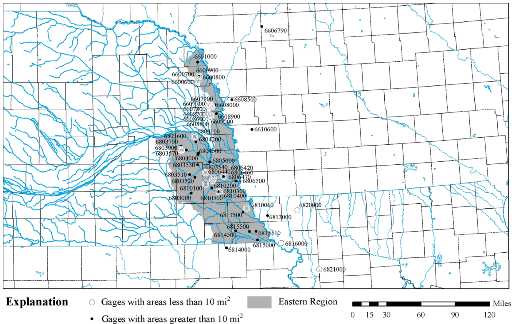
Figure 4.2: Location of streamflow gaging stations used in the Eastern regression analysis.
