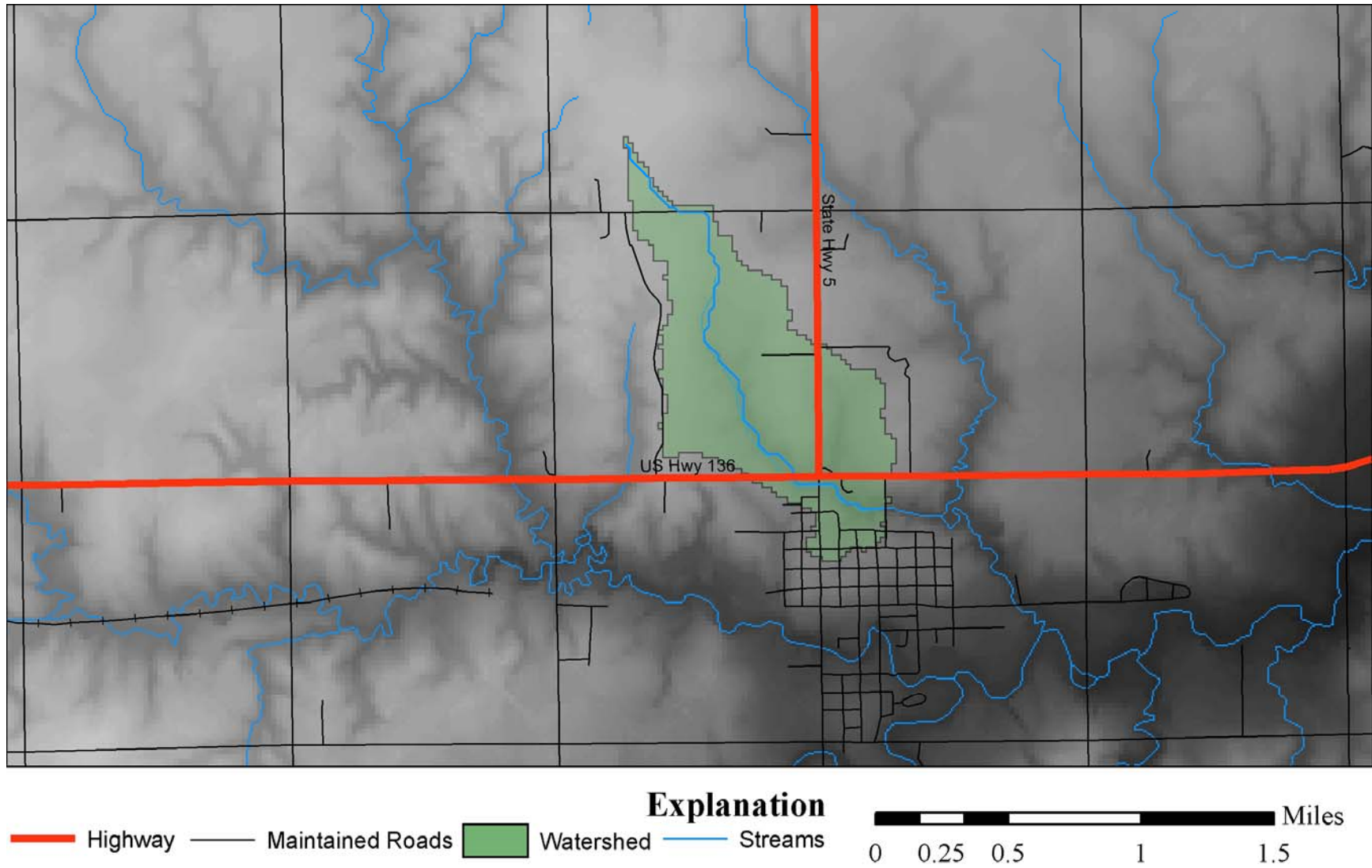
Figure 5.2: Drainage area upstream of a culvert located on U.S. Highway 136 in Deshler, Nebraska.
