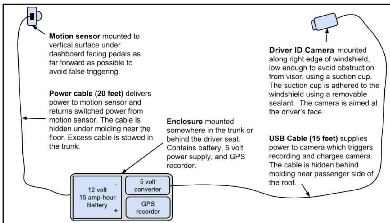
Figure 3. Vehicle Instrumentation.
