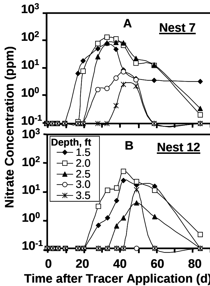
Figure 8.6. The nitrate concentrations detected during the study at various depths at nest 7 (A) and nest 12 (B). Nests 7 and 12 are located 7.3 ft (220 cm) and 10.7 ft (320 cm) from the tracer application spot, respectively.
