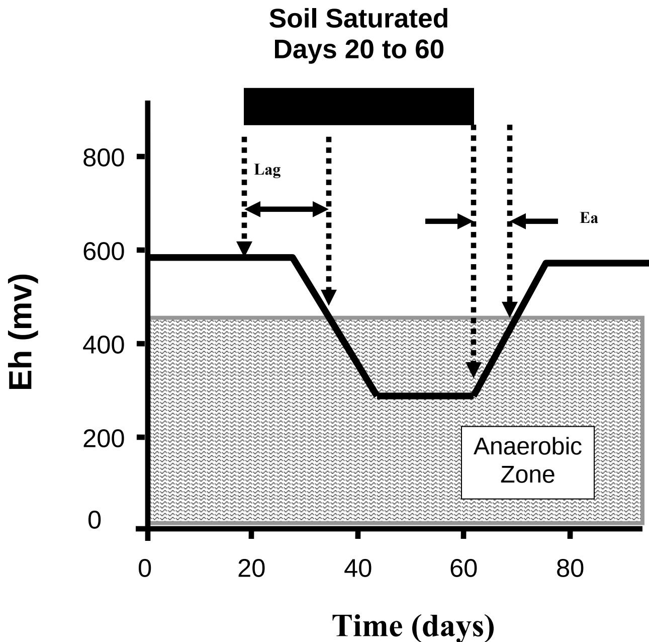
Figure 9.3. Illustration of how lag times (Lag) and extended anaerobic conditions were determined for Eh data from one depth in a soil plot. The Lag period was the time from the start of saturation to the beginning of anaerobic conditions as determined using Eq. 1. In this example, saturation began on day 20 and the Eh showed anaerobic conditions had developed on day 38, giving a Lag period of 18 days. Saturation ended on day 60 but the soil remained anaerobic until day 70, giving an extended anaerobic condition (Ea) of 10 days.
