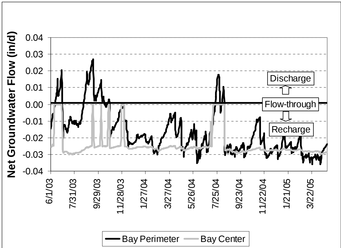
Figure 4.8. Simulated net groundwater flows for locations near the perimeter and near the center of Tatum Millpond Bay.
