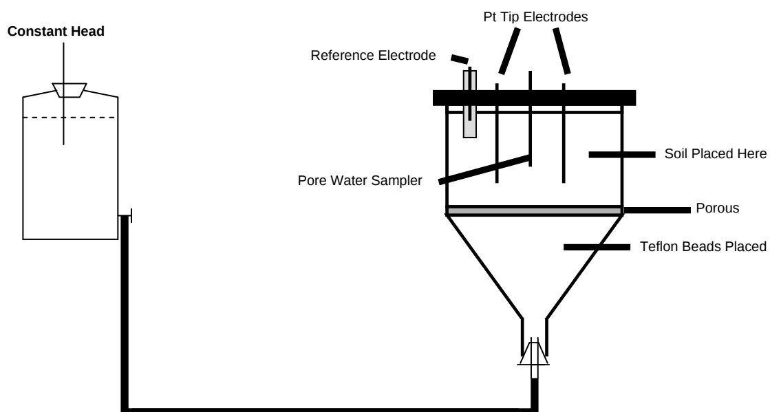
Figure 10.1: Redox incubation system depicting buchner funnel on right with Pt tip electrodes, reference electrode, pore water sampler and salt bridge. Soil was packed above the porous plate and teflon beads were placed below to minimize the amount of water during incubation. A constant head reservoir (left) was used to saturate columns from the bottom upward.
