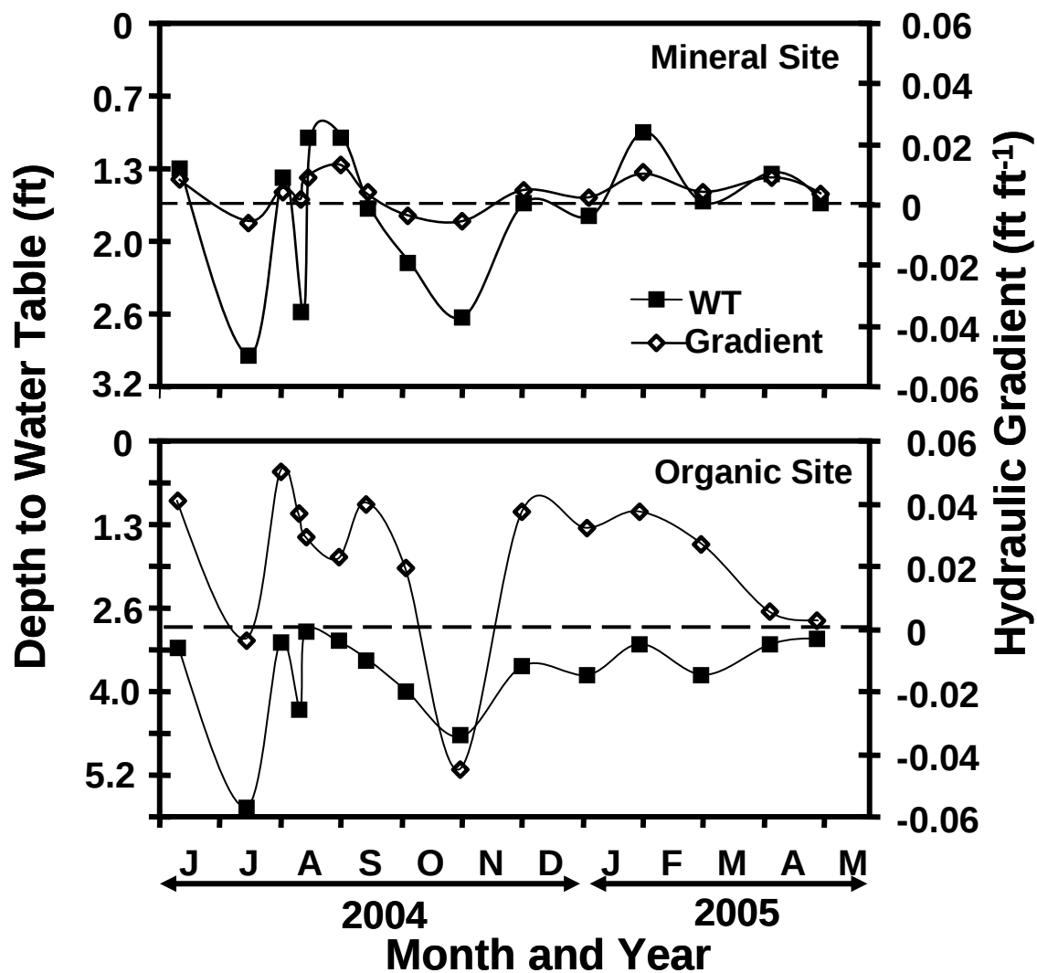
Figure 7.4. Depth to the water table and the subsurface hydraulic gradient computed for the axis that is perpendicular to the ditch. By convention, a positive hydraulic gradient value means that gradient is towards the ditch and a negative value indicates that it is going away from the ditch.
