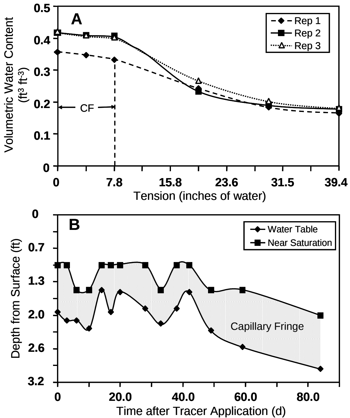
Figure 8.2. Soil water characteristic curves for three intact soil cores from the 1.5 to 2.0 ft layer (A), and depth to water table and the upper boundary of the near-saturated zone (measured using TDR) during the study (B). The 1.5 to 2.0 ft depth interval was mainly in the CF for most of the study period.
