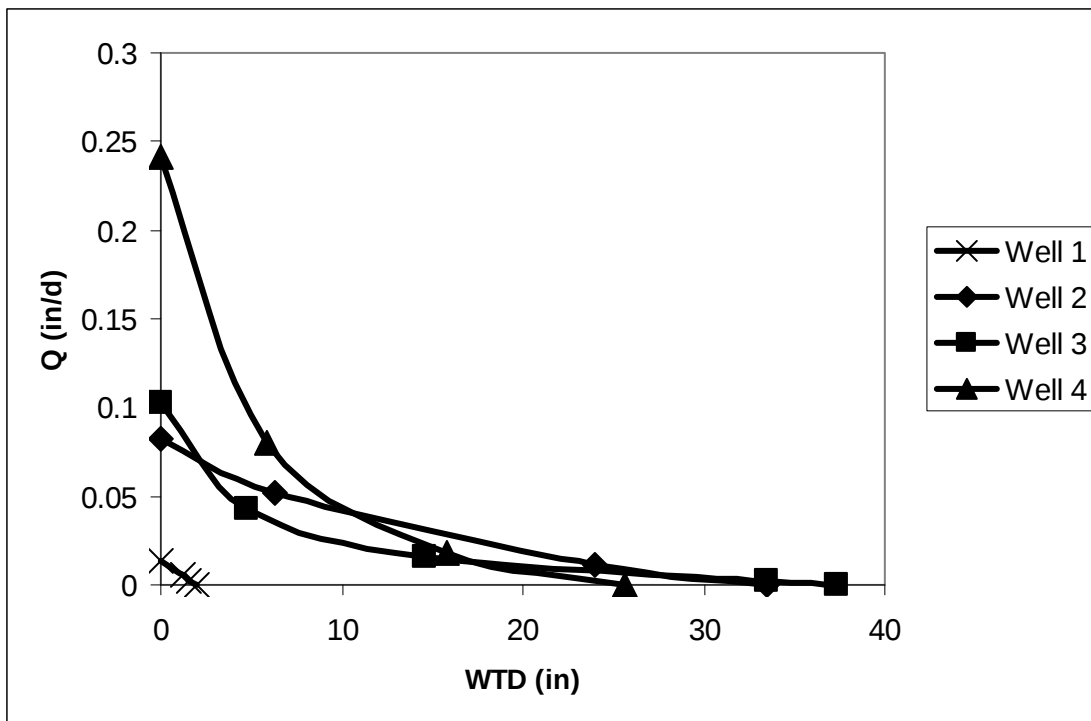
Figure 4.6. Relationship between drainage rate and water table depth for the four well locations in Charlie Long Millpond Bay as determined in the DRAINMOD model calibration process.
