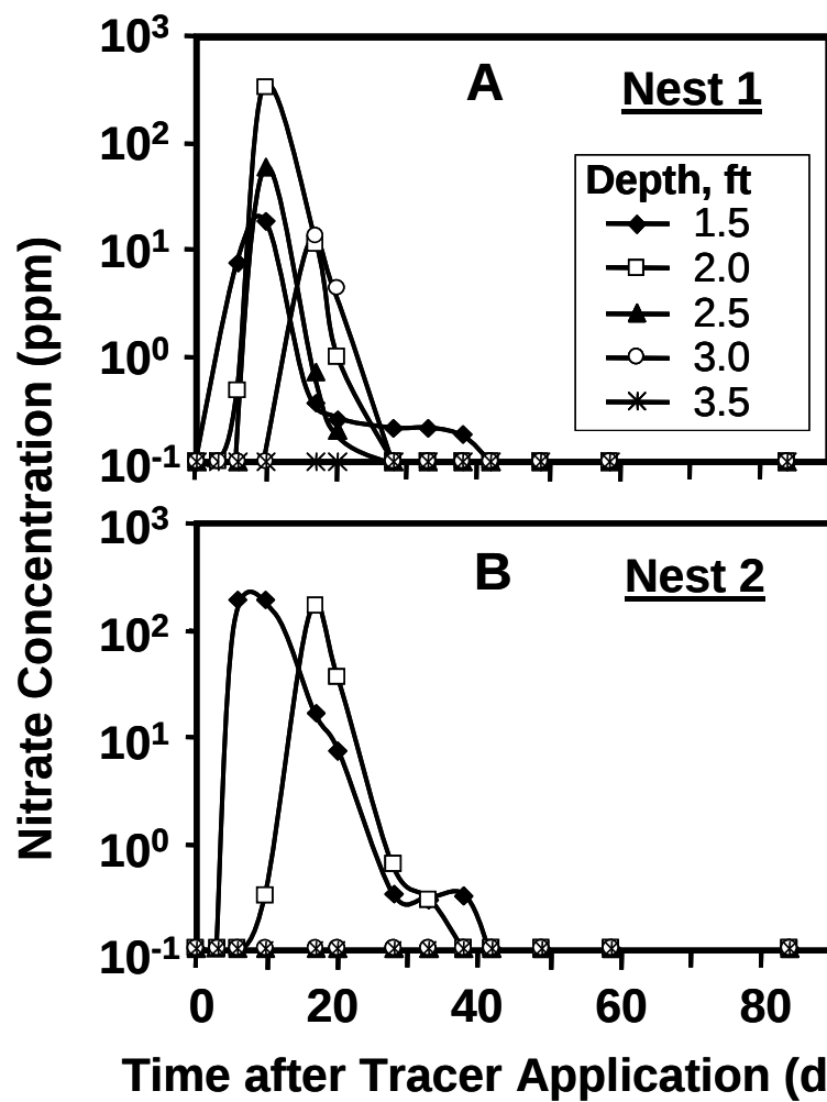
Figure 8.4. The nitrate concentrations detected at various depths at 2 ft (60 cm) horizontal distance from the tracer application spot in nests 1 (A) and 2 (B) during the study.
