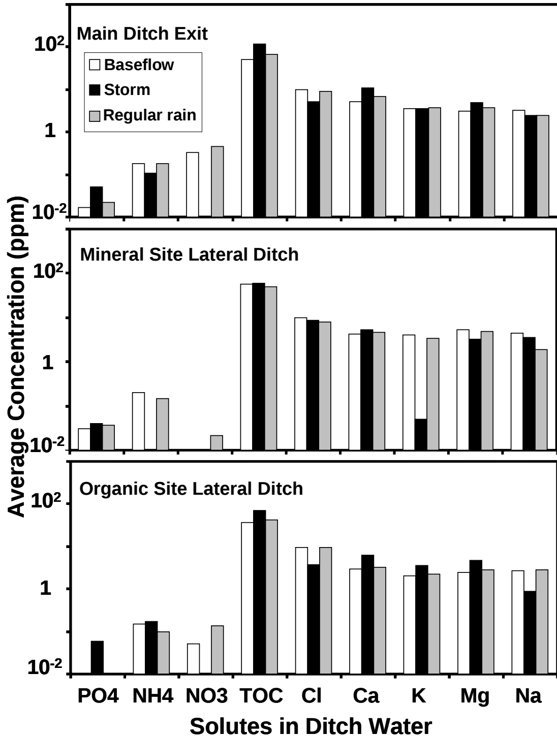
Figure 7.6. Average concentrations of different solutes monitored at the main ditch exit, side ditch at the mineral site, and side ditch at the organic site for base flow condition, days following a regular rain event, and days following a major storm event.
