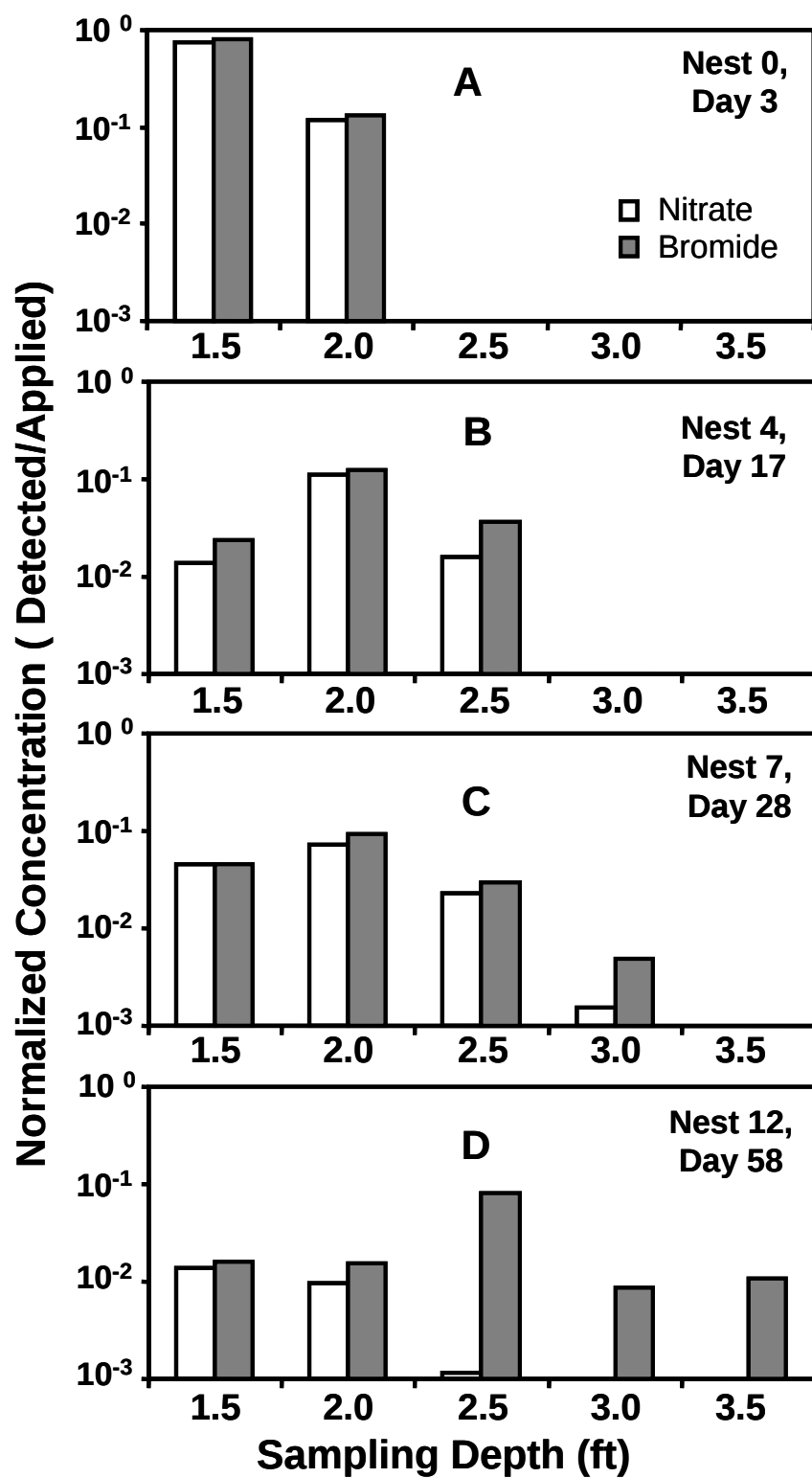
Figure 8.7. Normalized concentration of nitrate and bromide detected at various depths as the tracer plume moved through nest 0, 4, 7 and 12 located 0.67, 4.0, 7.3 and 10.7 ft, respectively, from the tracer application.
