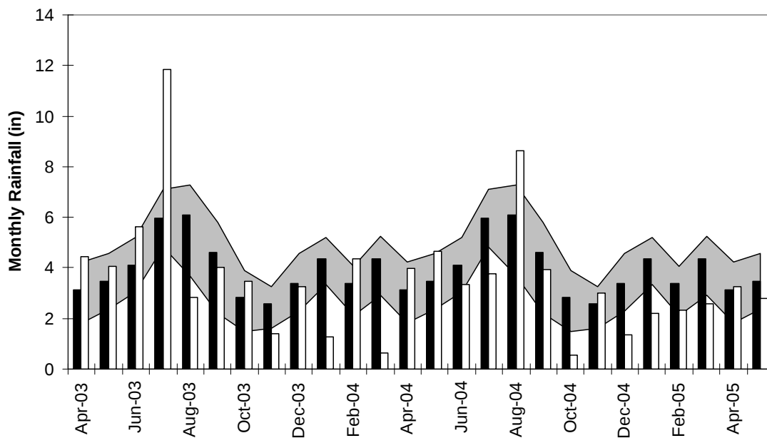
Figure 4.3. Monthly rainfall during the 2-yr calibration period. Black bars are the long-term average monthly rainfall amounts. White bars are monthly rainfall amounts measured at Charlie Long Millpond Bay. Gray area represents the range in normal rainfall amounts between the 30 th and 70 th percentile probability of occurrence.
