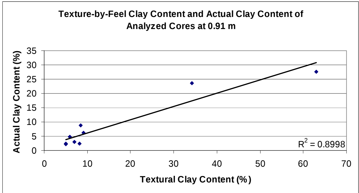
Fig. 6.10. Comparison of core clay content from the particle size analyses versus that estimated by the texture-by-feel method for the 3-ft (0.91-m) depth increment. The 3-ft (0.91-m) increment was chosen because there was a strong relationship between measured clay content and the texture-by-feel clay content of the analyzed cores. Clay content for the texture-by-feel method was estimated as the mean clay content of each textural class.
