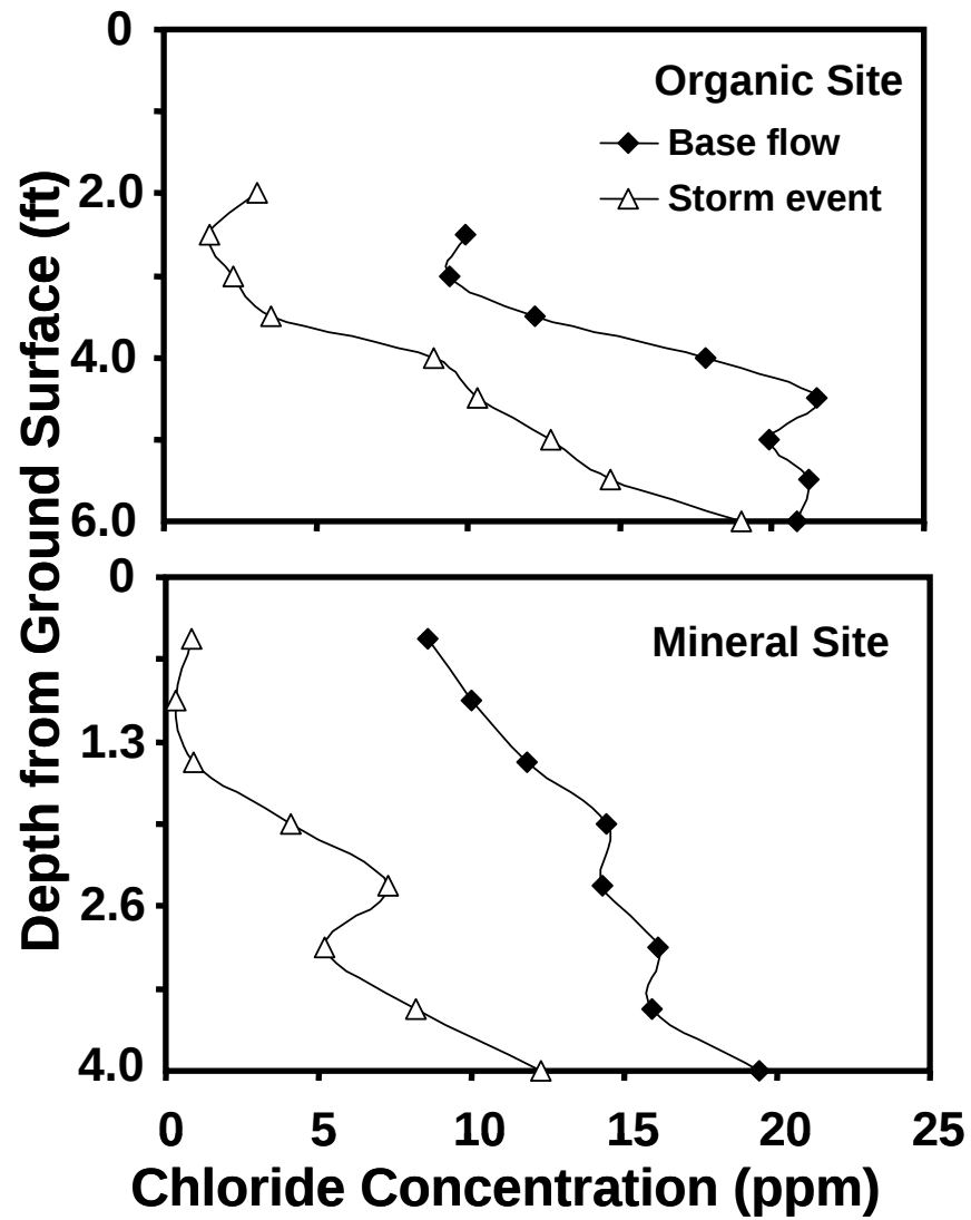
Figure 7.9. Soil solution chloride profile for sampling dates that represented base flow conditions and the day following the storm event at the organic and mineral soil sites.
