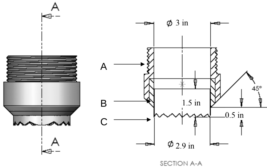
Figure 2.2. Drawing and relevant dimensions of the sampler cutting head. Components are: A) a 3 in diam. male threaded adapter, B) a 3 in diam. section of PVC pipe glued into (A), C) a 3 in diam. hole-saw with arbor end removed.
