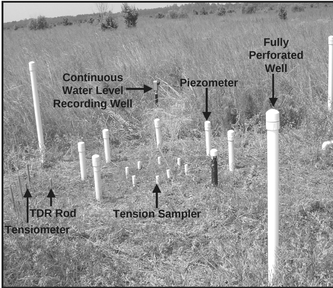
Figure 7.2. Photograph of the monitoring set-up.
