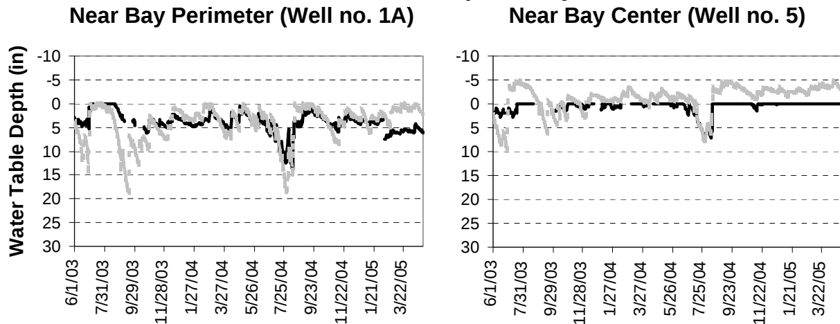
Figure 4.7. Measured (black solid line) and simulated (gray dotted line) water table depths at selected well locations in the study sites. Zero water table depth is at the land surface, positive depths below the land surface, and negative depths above the land surface. Field measured water table depths above the land surface during ponding events were not recorded and are shown as zero water table depths.
