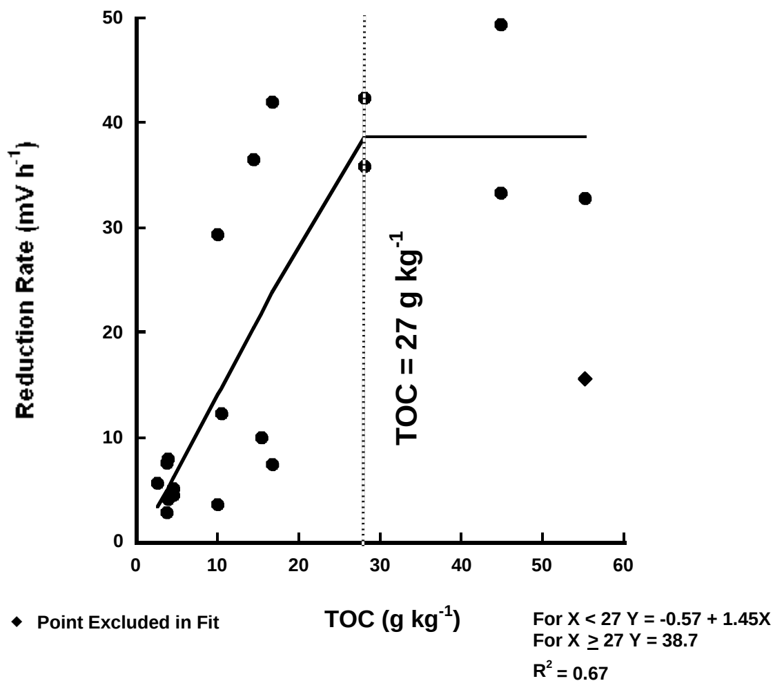
Figure 10.4: Total organic carbon (TOC) concentration in relation to reduction rate. A linear plateau model shows increasing reduction rate with increasing TOC up until TOC = 2.7 % (TOC = 27 \text{g kg}^{-1} ). One outlying point, pictured as a diamond, was excluded from this fit.
