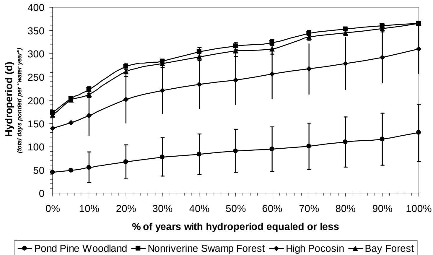
Fig. 5.2. Hydroperiod (total days ponded per water year) frequency curves for each plant community over the 40 yr simulation. Data shown for each plant community are averages among the various locations simulated. Error bars represent one standard error above and below the mean.
