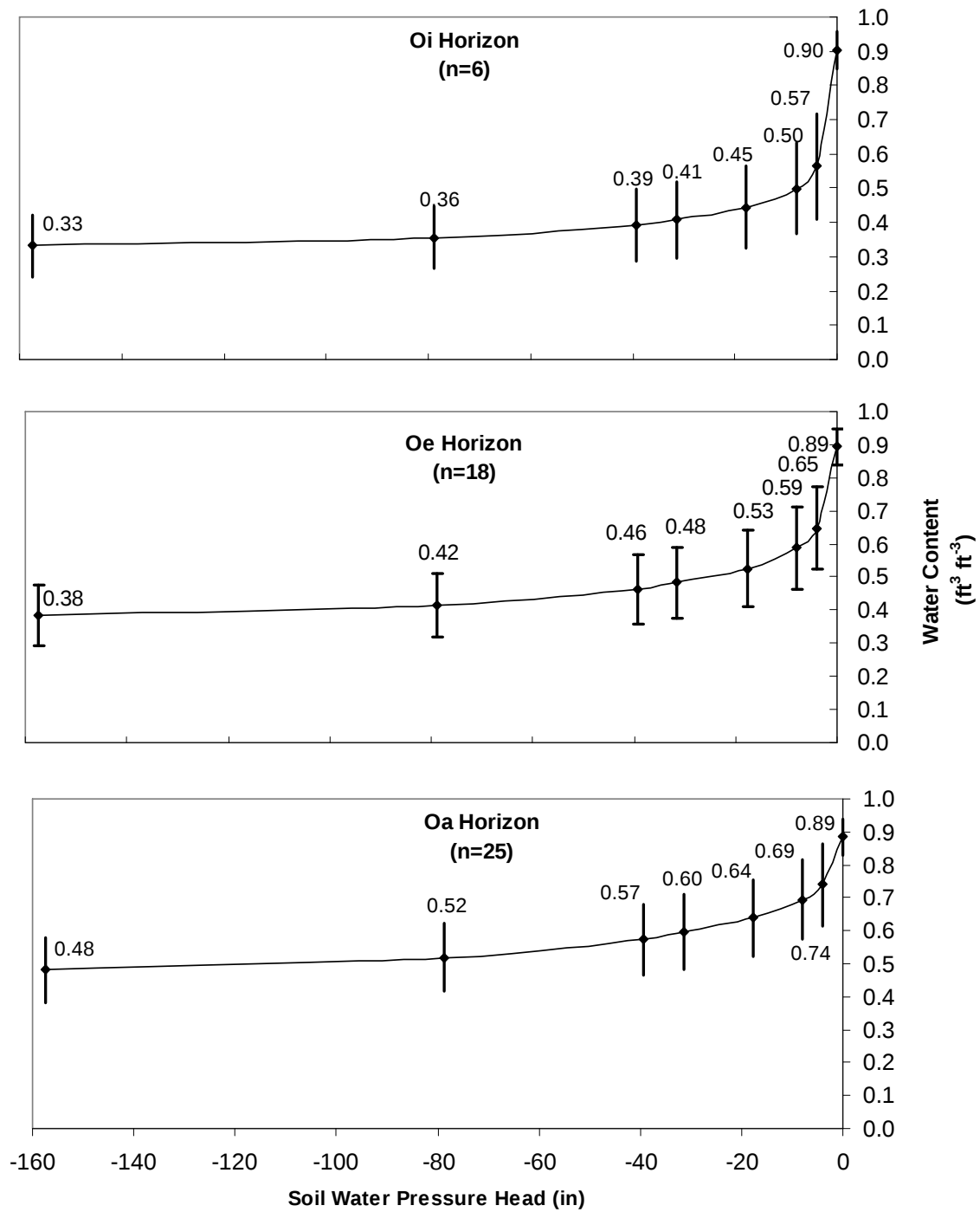
Figure 3.2. Mean soil water characteristic curves for Oi, Oe, and Oa horizons of the organic soils. Numbers are the average water contents at that soil water pressure. Error bars show one standard deviation around the mean.
