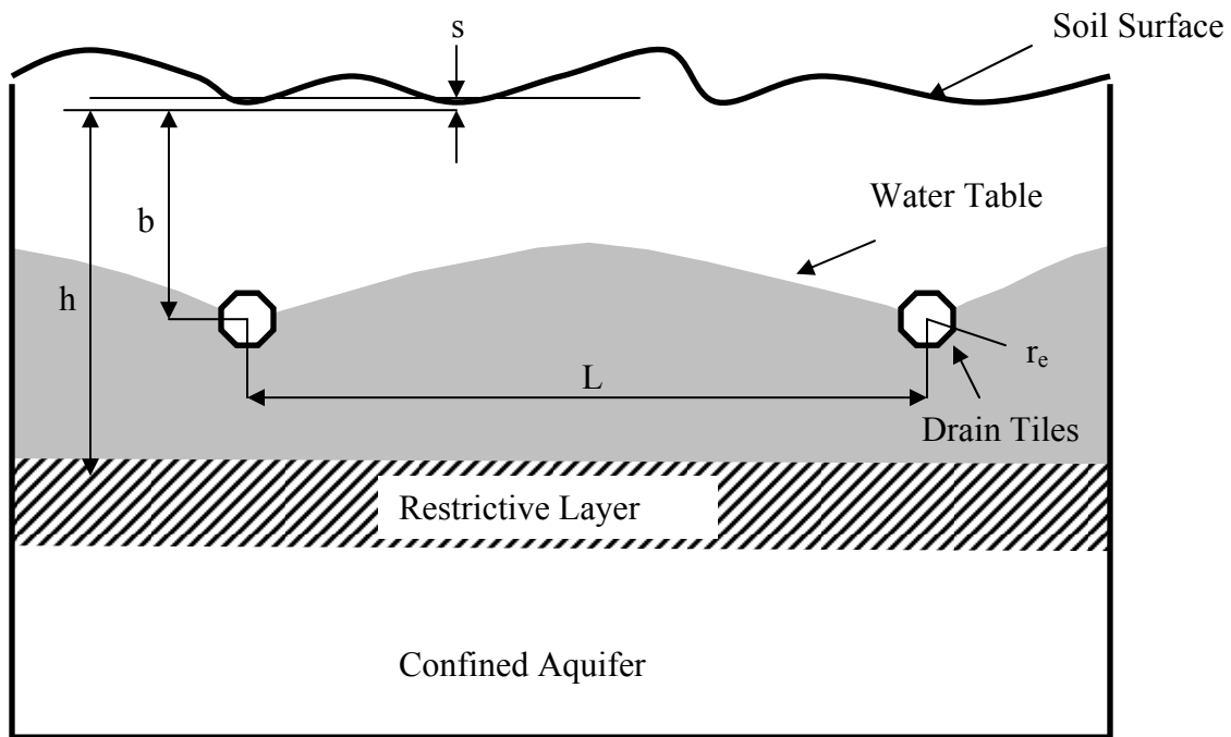
Figure 4.1. Schematic diagram of the drainage system simulated by DRAINMOD. Dimensions include the drain depth, b , drain spacing, L , depth to restrictive layer, h , effective radius of drains, r_e , and surface storage, s .
