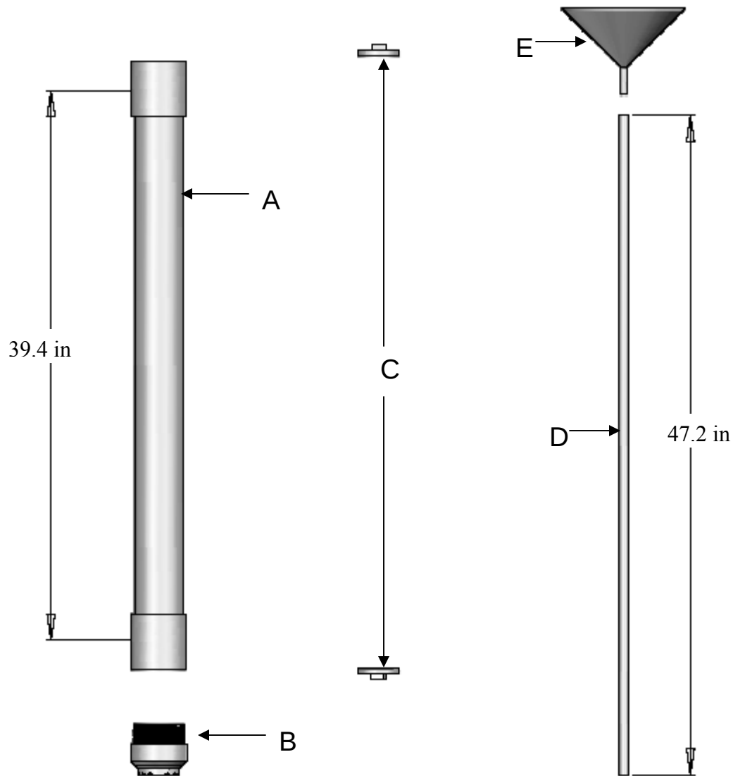
Figure 2.1. Schematic diagram of the core sampler. Components are: A) a 39.4 in (100 cm) long 3 in diam. schedule 40 PVC pipe with female threaded adapters on each end, B) a sampler cutting head, C) two 3 in. diam. male threaded PVC caps, D) a 47.2 in (120 cm) long, 0.5 in diam. galvanized pipe, and E) a plastic funnel.
