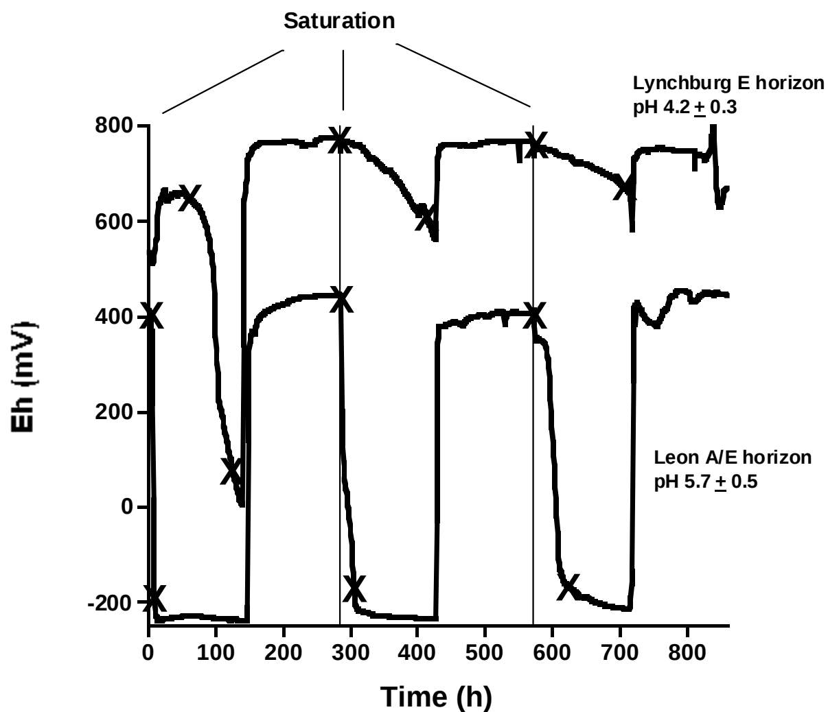
Figure 10.2: Three reduction-oxidation cycles of one replication of two different soil samples: the Lynchburg E horizon, and the Leon A/E horizon. The Y axis and the black vertical lines denote times where the water level was raised to saturate soils. “X” represents the endpoints of data used in the linear regression used to determine reduction rate.
