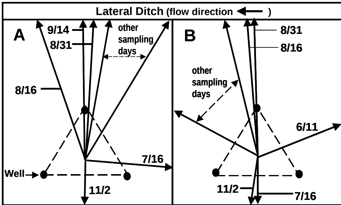
Figure 7.5. Relative direction of the subsurface lateral hydraulic gradient at the organic (A) and mineral (B) soil sites determined using the three-point technique.
