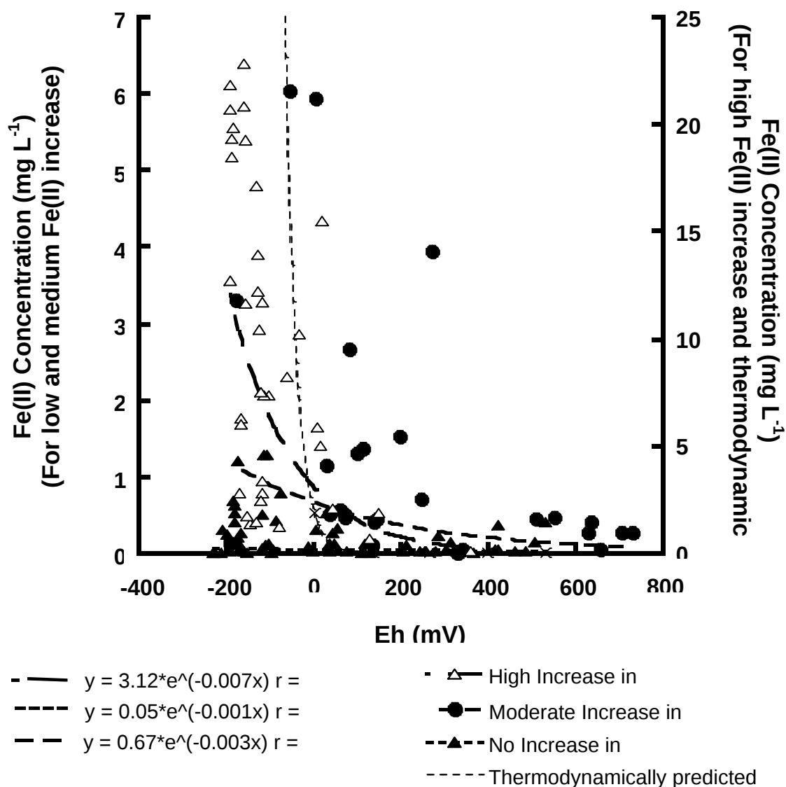
Figure 10.5: Dissolved Fe(II) ( \text{mg L}^{-1} ) vs. Eh for redox incubations. Three groups were denoted: those with high increases in Fe(II) (Pantego A and B horizons, Goldsboro A horizon, and Rains A horizon – right Y axis), those with moderate increases in Fe(II), (Rains E and B horizons, Lynchburg E horizon – left Y axis), and those with no increase in Fe(II), (remaining soils – left Y axis). The smooth curve corresponds to the thermodynamically predicted rate of Fe(II) dissolution from goethite, (right y axis).
