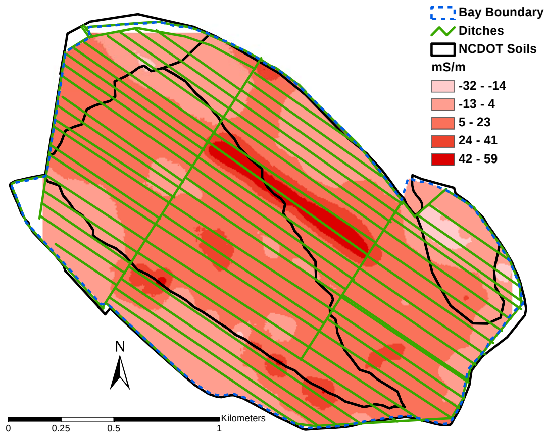
Fig. 6.5. Kriged December 2000 GEM-300 3.03 kHz. horizontal dipole orientation EC_a . One km equals 0.62 mi.
