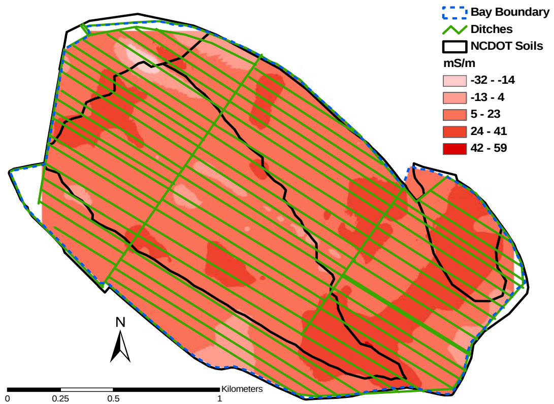
Fig. 6.6. Kriged December 2000 GEM-300 9.81 kHz. vertical dipole orientation EC_a . One km equals 0.62 mi.
