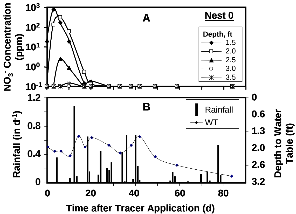
Figure 8.3. The nitrate concentrations detected at various depths at 0.7 ft (20 cm) horizontal distance from the tracer application spot in nest 0 (A), and rainfall data and measured water table during the study (B).
