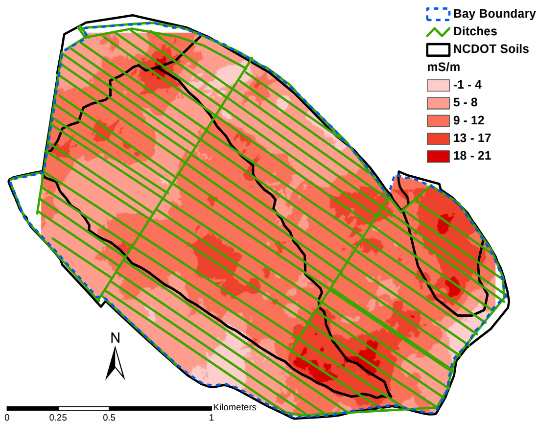
Fig. 6.4. Kriged December 2000 EM38 vertical dipole orientation EC_a . One km equals 0.62 mi.
