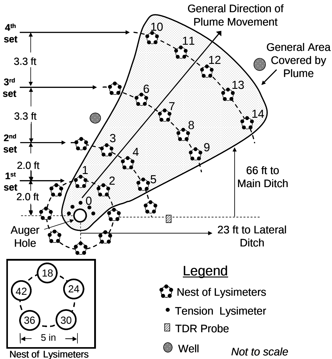
Figure 8.1. Schematic diagram of the plan view of the locations of the lysimeter nests, wells, and time domain reflectometry (TDR) probe in the experimental area. The inset shows the position of the tension lysimeters in a nest with porous cups at 1.5, 2.0, 2.5, 3.0 and 3.5 ft from the surface.
