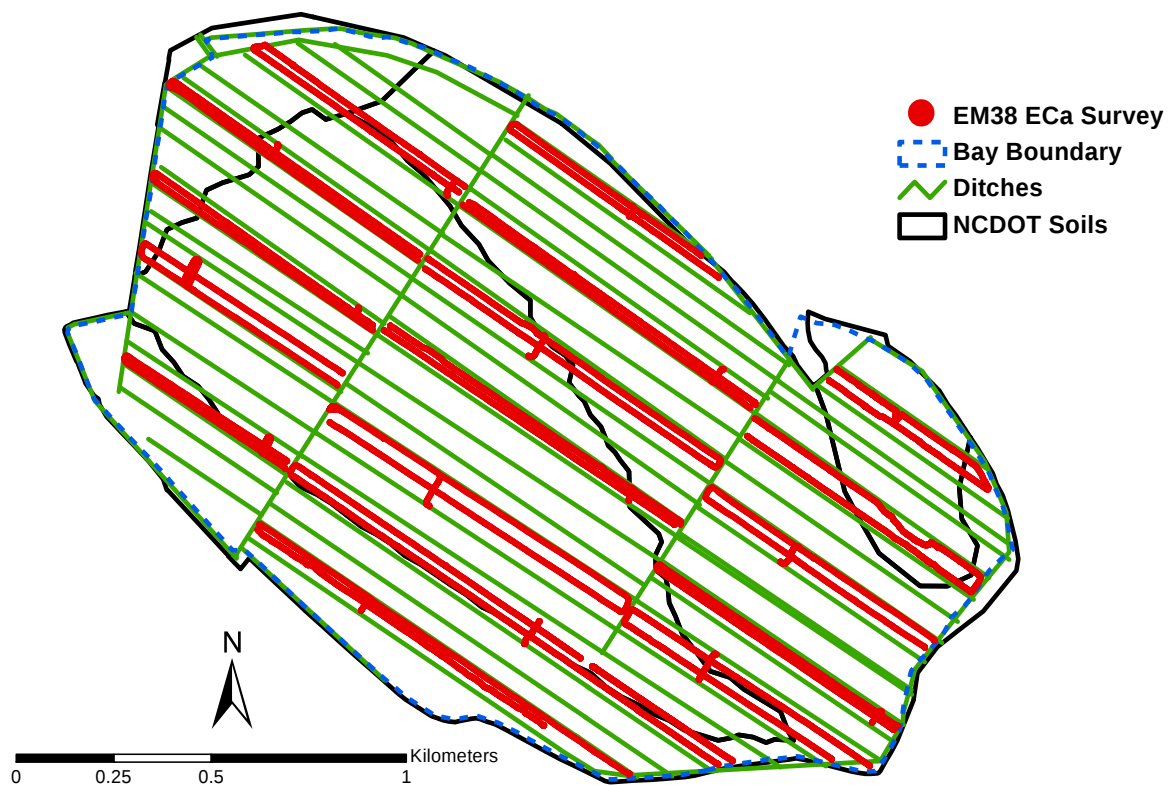
Fig. 6.3. Overall initial December 2000 EM38 EC a survey at Juniper Bay. The measurements were recorded on a continuous basis (1-s intervals). There were approximately 23,000 measurement locations. Overall initial December 2000 GEM-300 EC a survey at Juniper Bay was along the same transect lines. The measurements were recorded on a point basis. There were approximately 1,200 measurement locations. One km equals 0.62 mi.
