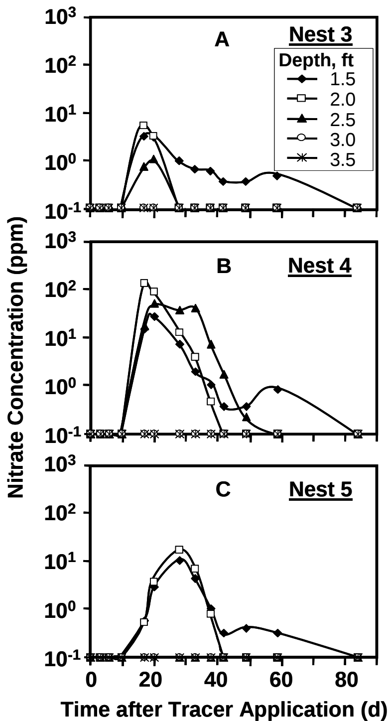
Figure 8.5. The nitrate concentrations detected at various depths at 4 ft (120 cm) horizontal distance from the tracer application spot in nests 3 (A), 4 (B) and 5 (C) during the study.
