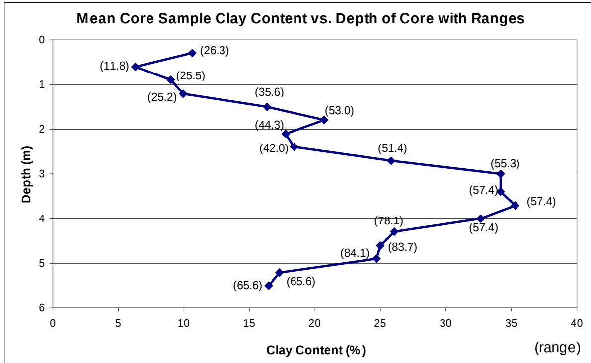
Fig. 6.8. Mean core clay content at each depth increment for the analyzed cores with ranges of clay content for each depth. One meter is 3.28 ft.
