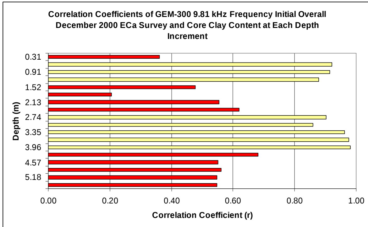
Fig. 6.7. Correlations (Pearson correlation coefficient, r ) between soil apparent conductivity ( EC_a ) from GEM-300 9.81 kHz vertical frequency from the initial overall December 2000 EC_a survey and core clay content displayed at each depth increment. The labels of the depth increments are the bottom of the profile increments. The light bars indicate significant correlations ( p \leq 0.05 ) and dark bars indicate those that were not significant.
