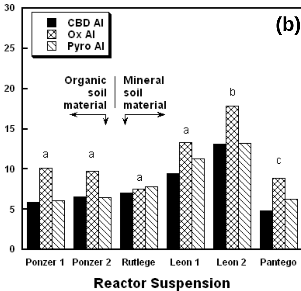
Figure 11.1b. Extractable forms of Al ( \text{mg kg}^{-1} ) in the < 0.002'' solids used in stirred reactor incubation studies. Extractions performed on separate samples. CBD = citrate bicarbonate dithionite.
