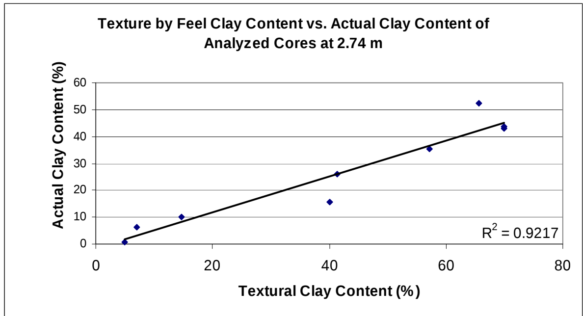
Fig. 6.11. Comparison of core clay content from the particle size analyses versus that estimated by the texture-by-feel method for the 9-ft (2.74-m) depth increment. The 9-ft (2.74-m) increment was chosen because there was a strong relationship between measured clay content and the textural clay content of the analyzed cores. Clay content for the texture-by-feel method was estimated as the mean clay content of each textural class.
