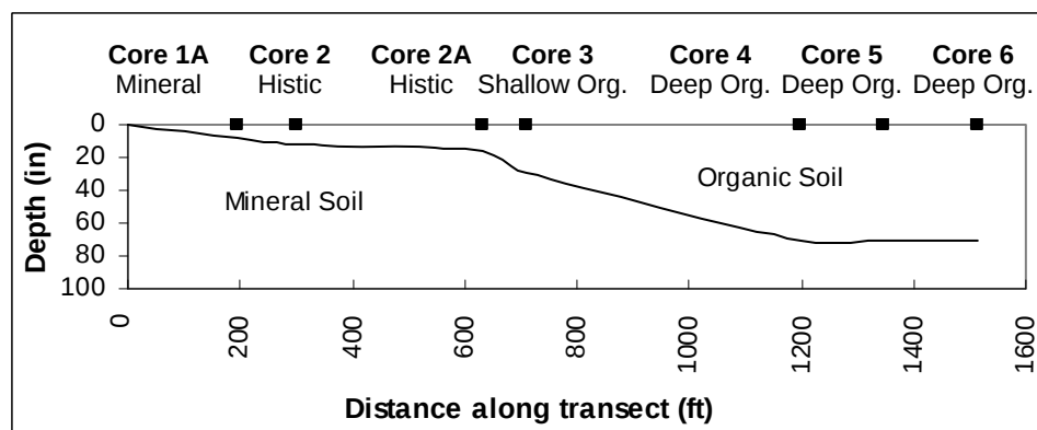
Figure 3.1. Approximate depths of organic soil layers and location of sampling plots along each bay transect. Relative surface elevations along transects are not represented.
