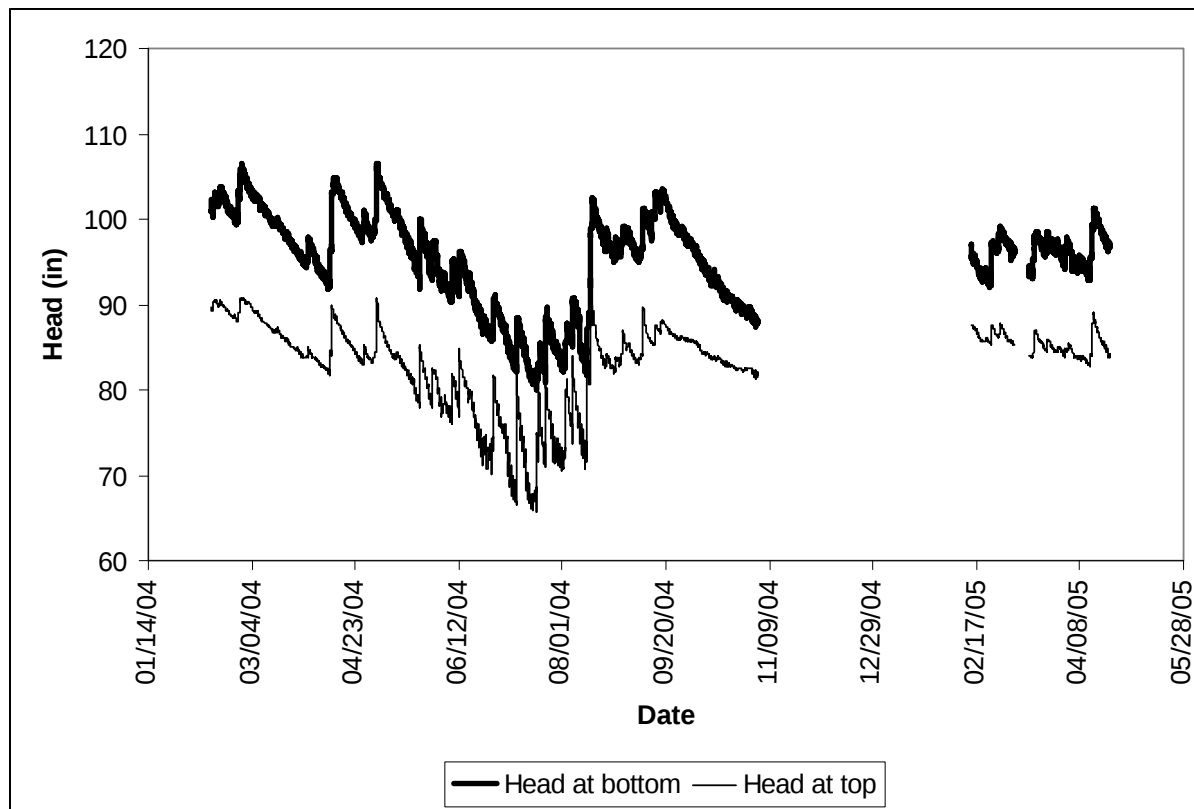
Figure 4.4. Hydraulic heads above and below restrictive layer in Charlie Long Millpond Bay near well no. 2.
