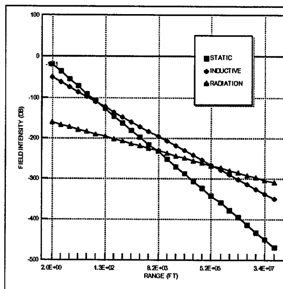
Figure: 4 Relative field intensity
