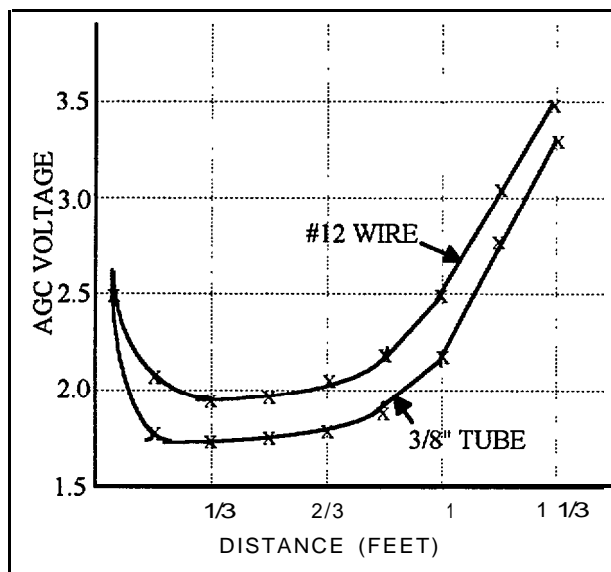
Figure: 13 Receiver AGC versus range
