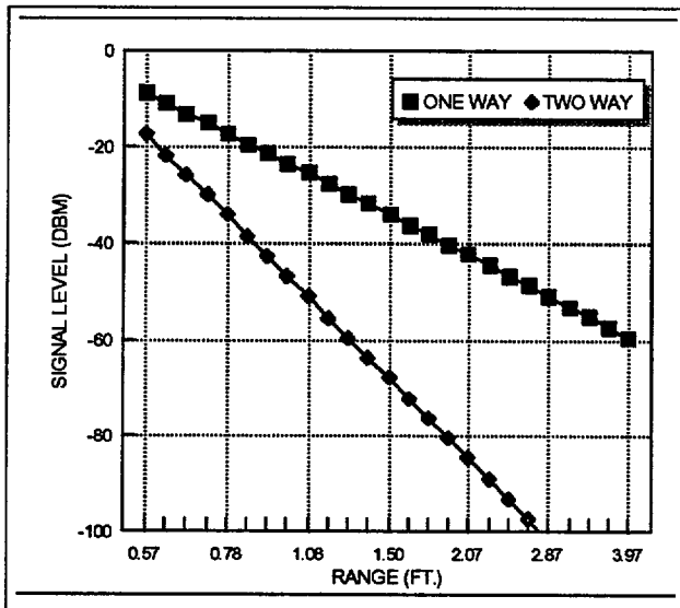
Figure: 9 Range sensitivity
