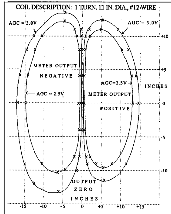
Figure: 7 Footprint diagram
