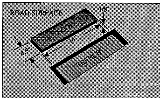
Figure: 14 Loop installation
