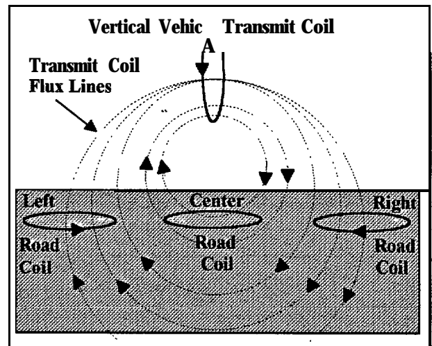
Figure: 2 Vehicle to road link
