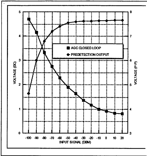
FIGURE 8 Receiver Sensitivity
