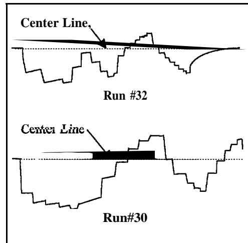
Figure: 12 Road test data
