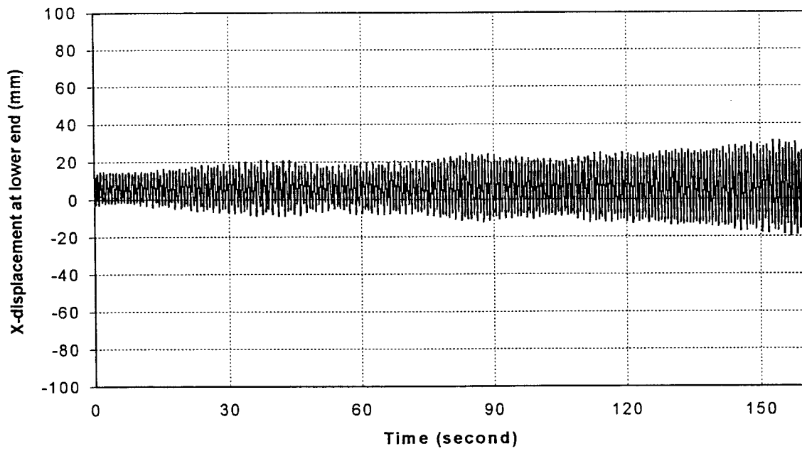
Figure 51a: Lower end X-motion, time history of Setup 2C at U=32 m/s.
