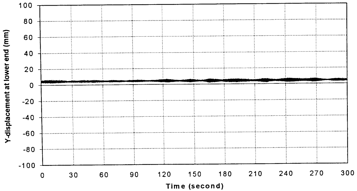
Figure 56c: Lower end Y-motion, time history of Setup 1B at U=24 m/s.
