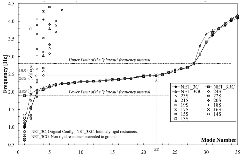
Figure 88: Comparative analysis of network vibration characteristics and individual-cable behavior; Fred Hartman Bridge; NET_3C, original configuration; NET_3RC, infinitely rigid restrainers; NET_3CG, spring connectors extended to ground (Restr. 2,3).
