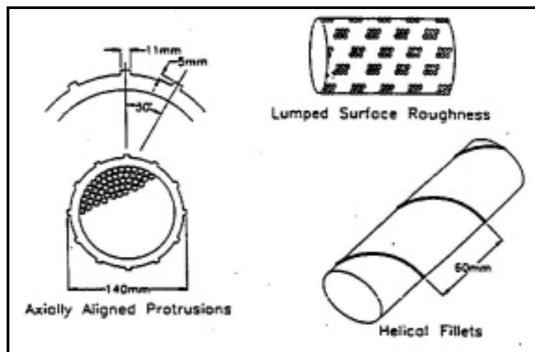
Figure 18: Types of cable surface treatments.
