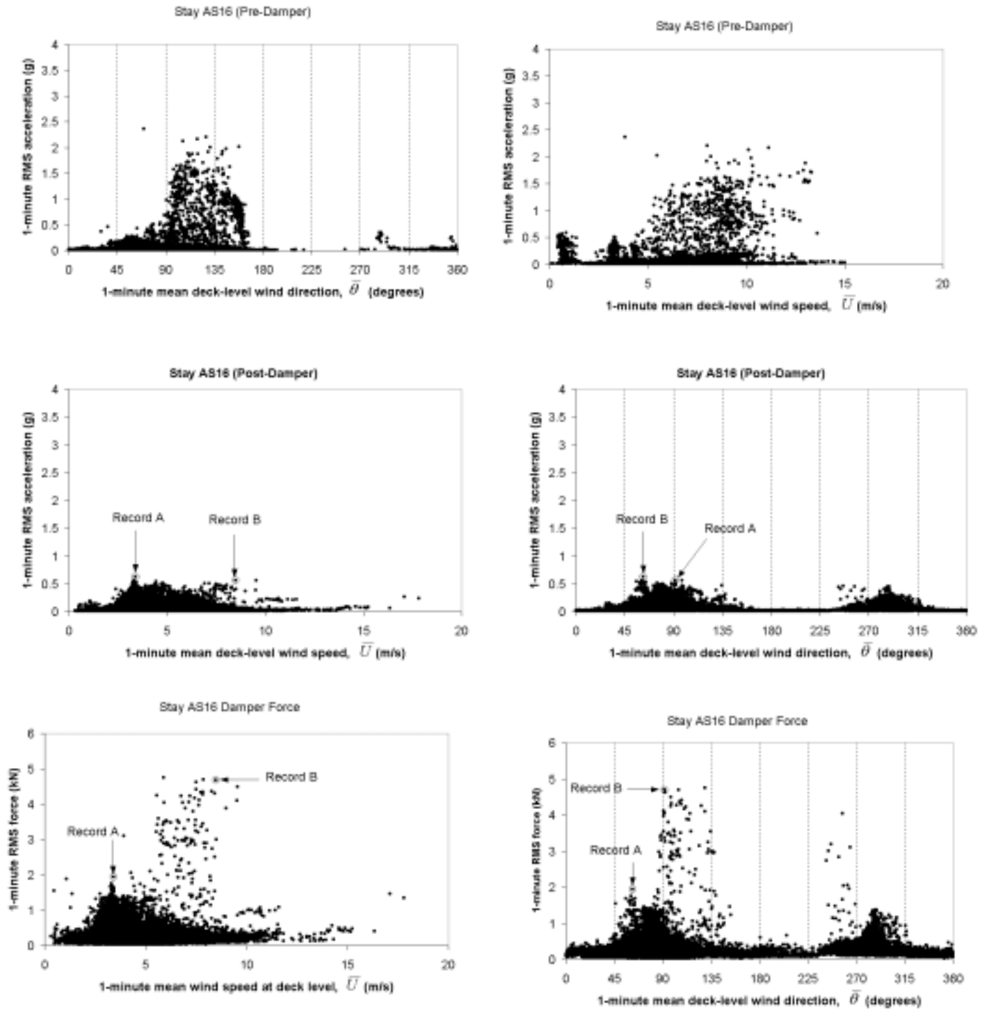
Figure 95: Stay vibration and damper force characteristics; Stay A16.
