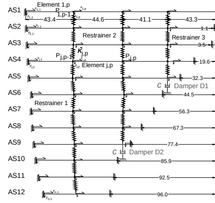
Figure 92b: Equivalent model.
