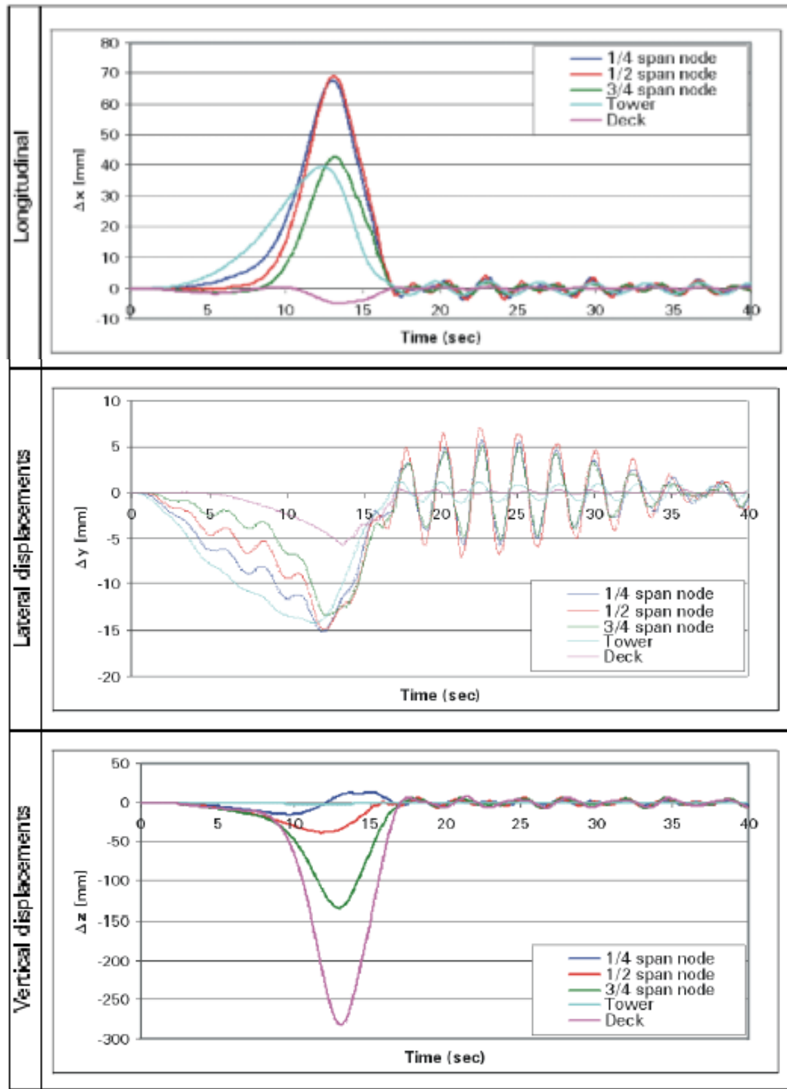
Figure 136: Global Coordinate Displacements of Cable M26 Nodes [mm] vs. Time. Train speed 80 km/hr.
