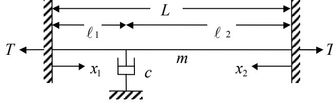
Figure 77: Taut cable with a linear damper.
