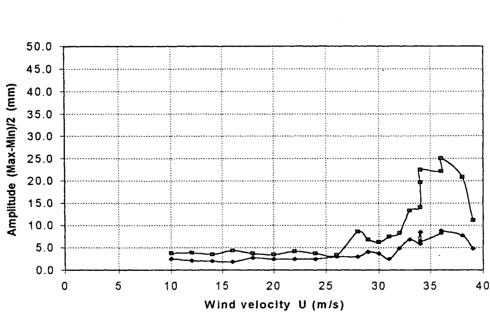
Figure 65: Wind-induced response of inclined dry cable. (Set-up 1C, smooth surface, low damping)
