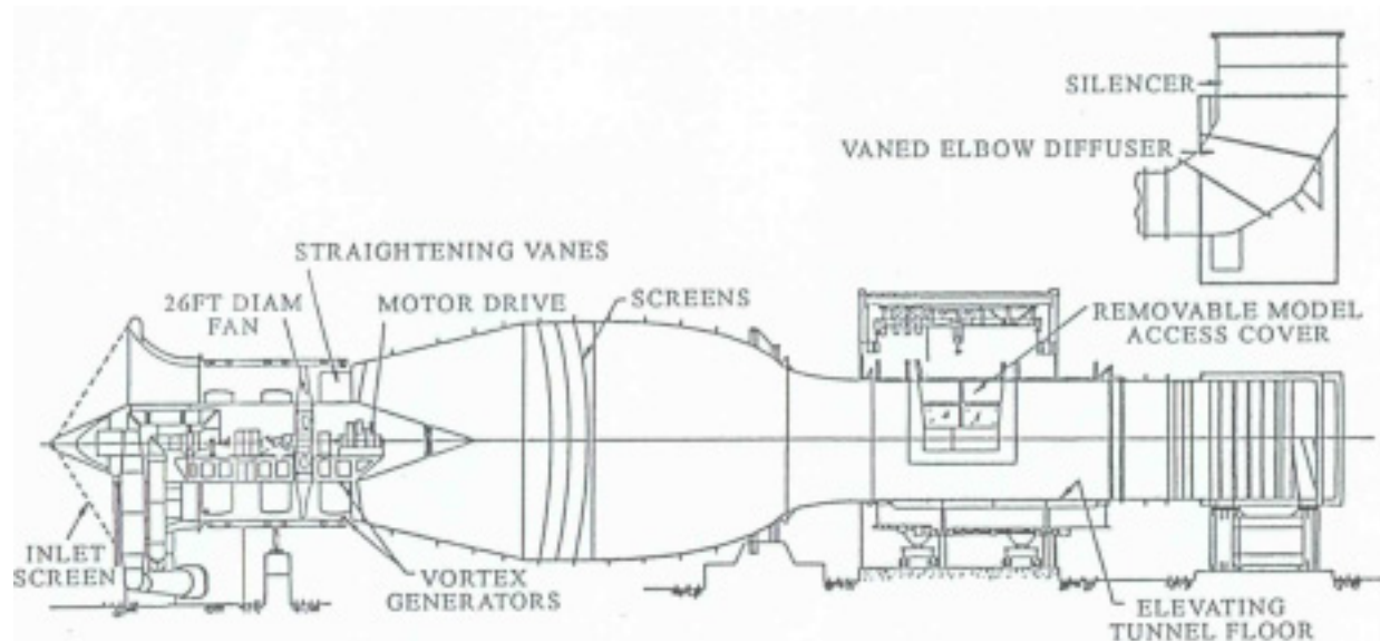
Figure 39: Longitudinal section of the “Propulsion” wind tunnel.
