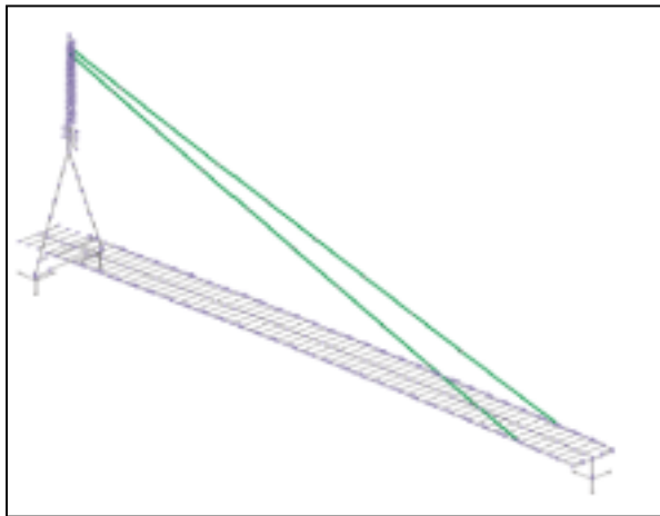
Figure 122: Cable M26 discretization - 10-segment model. View: Isometric. Only cables M26 are shown. Other cables not shown for clarity.
