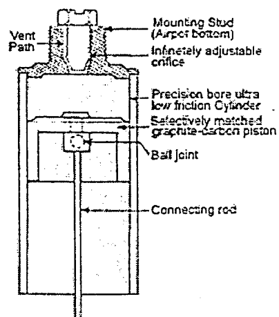
Figure 43: Cross-section of airpot damper.
