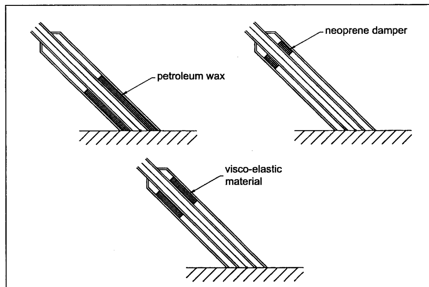
Figure 36: Material damping.
