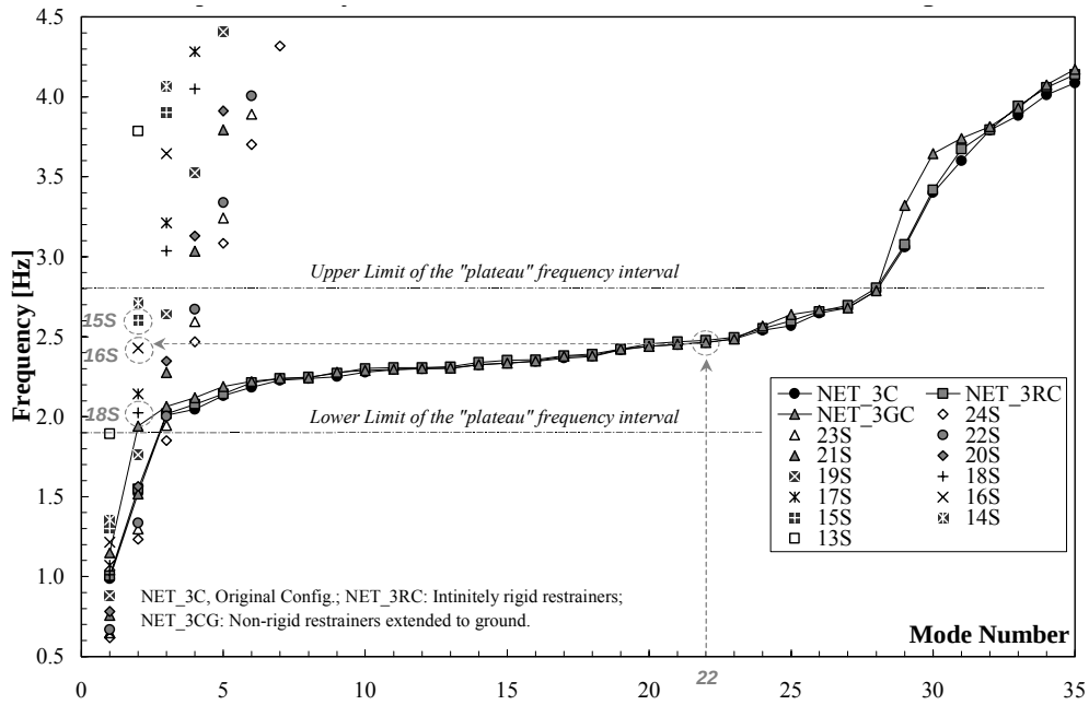
Figure 16: Comparative analysis of network vibration characteristics and individual-cable behavior; Fred Hartman Bridge.
