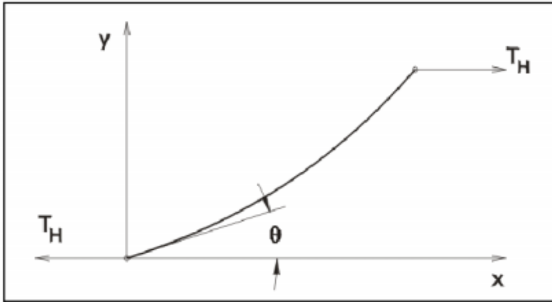
Figure 119: Cable catenary.
