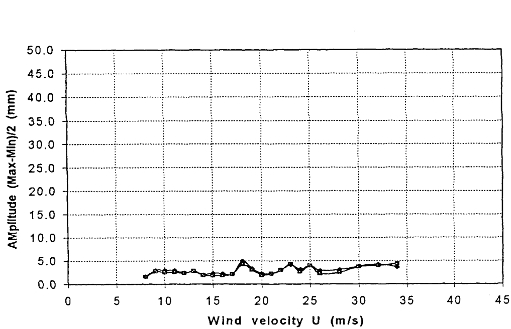
Figure 67: Wind-induced response of inclined dry cable. (Set-up 3B, smooth surface, low damping)
