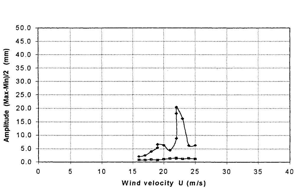
Figure 66: Wind-induced response of inclined dry cable. (Set-up 3A, smooth surface, low damping)
