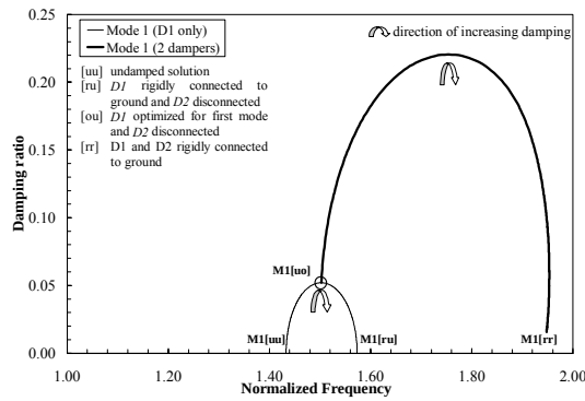
Figure 93a: Frequency solutions (1st mode) for the damped cable network (“A”-line).
