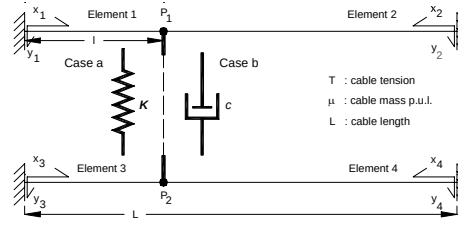
Figure 90: Twin cable with variable position connector.
