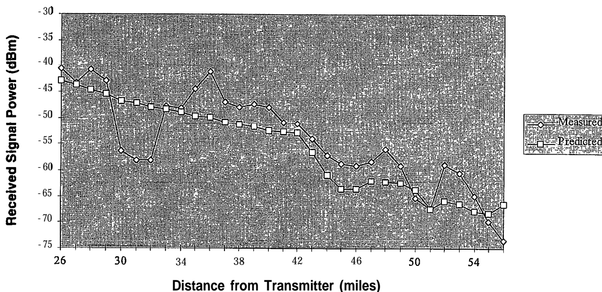
Figure D- 1. Measured and predicted mean received signal power for north-bound path (along Interstate 25).
