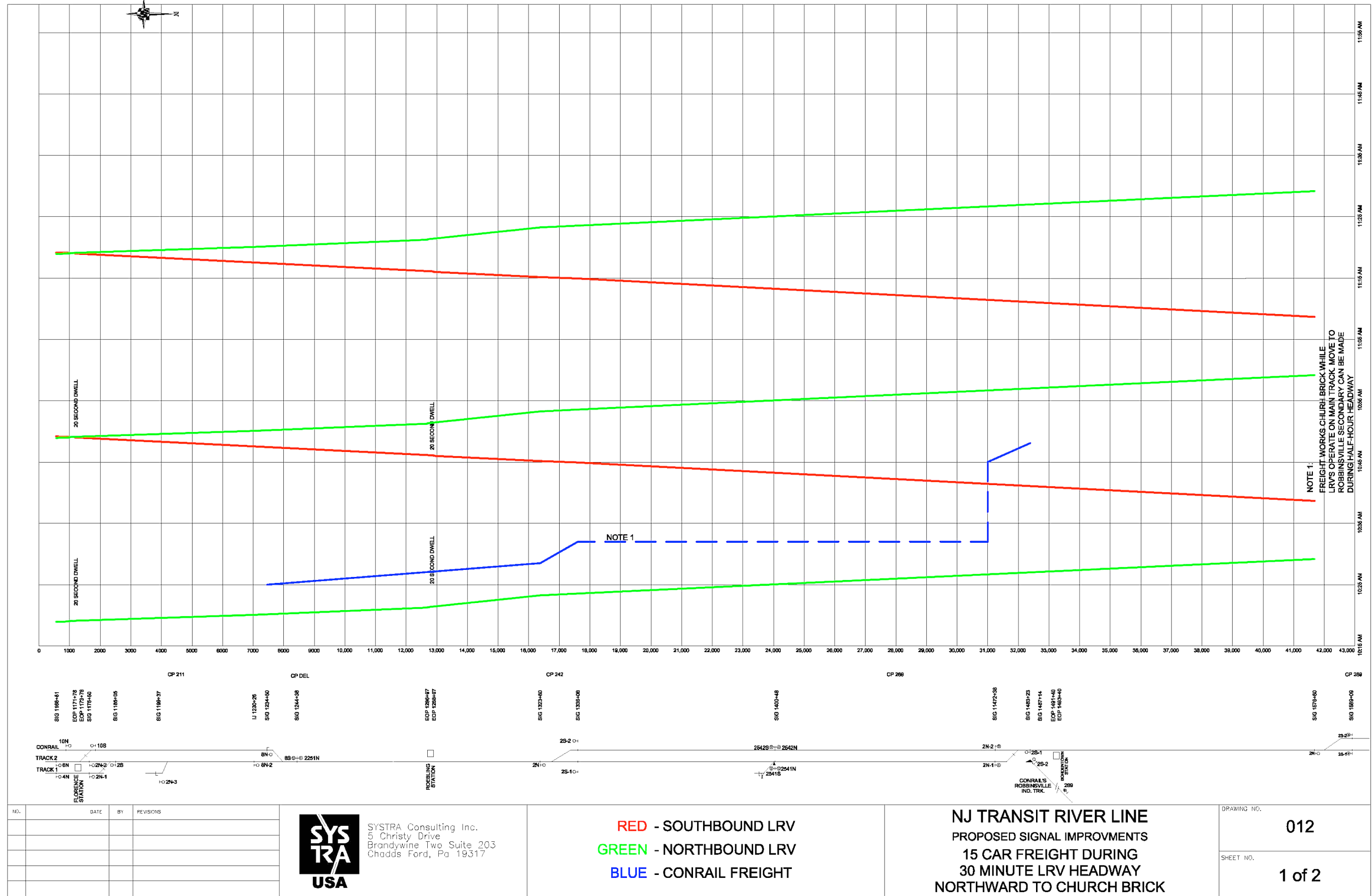
Figure 36 Existing Signal Plans and Proposed Signal and Train Operations Design Plans for the River LINE, Burlington Division, Drawing No. 12
