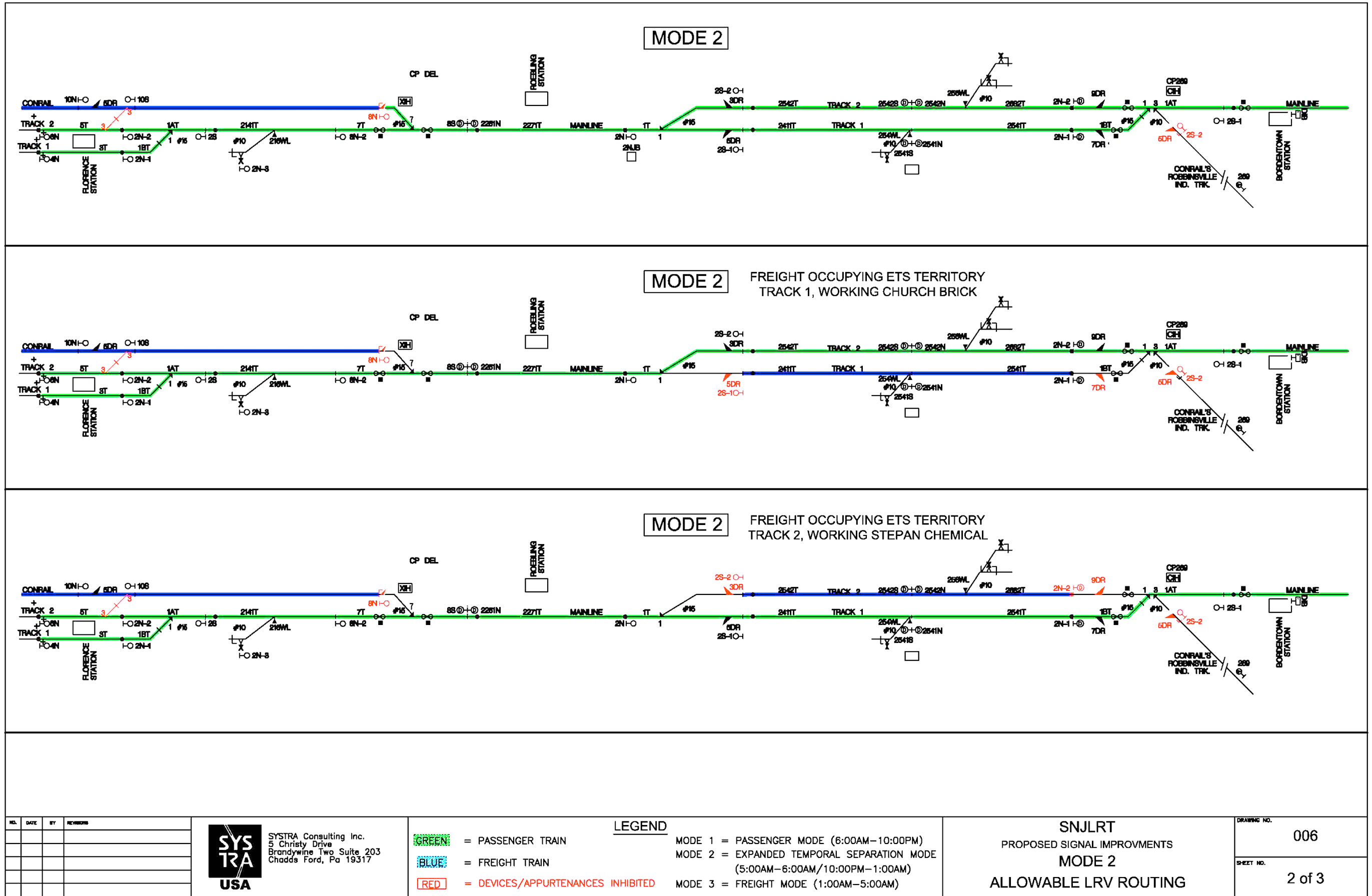
Figure 30 Existing Signal Plans and Proposed Signal and Train Operations Design Plans for the River LINE, Burlington Division, Drawing No. 6
