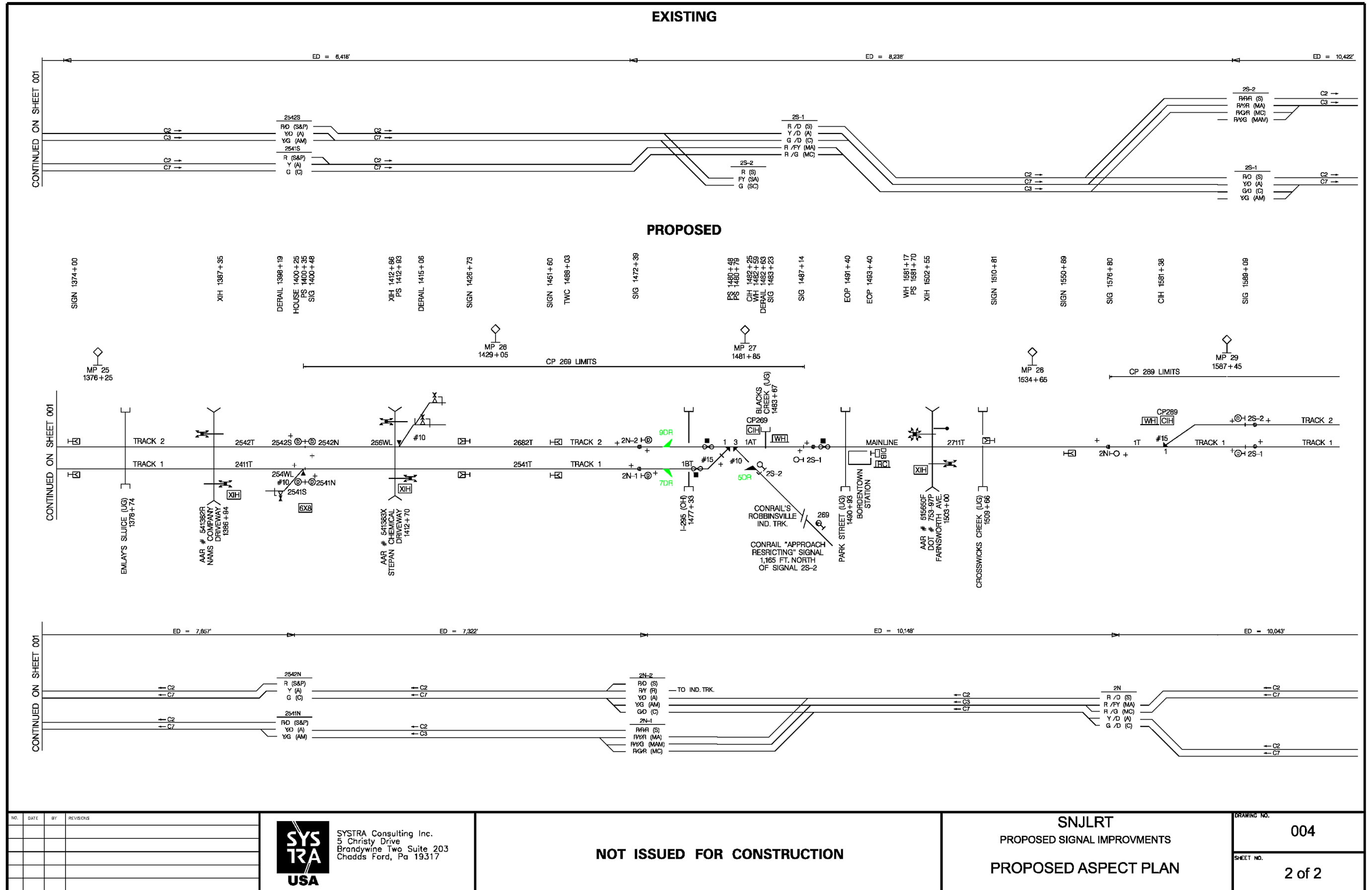
Figure 28 Existing Signal Plans and Proposed Signal and Train Operations Design Plans for the River LINE, Burlington Division, Drawing No. 4
