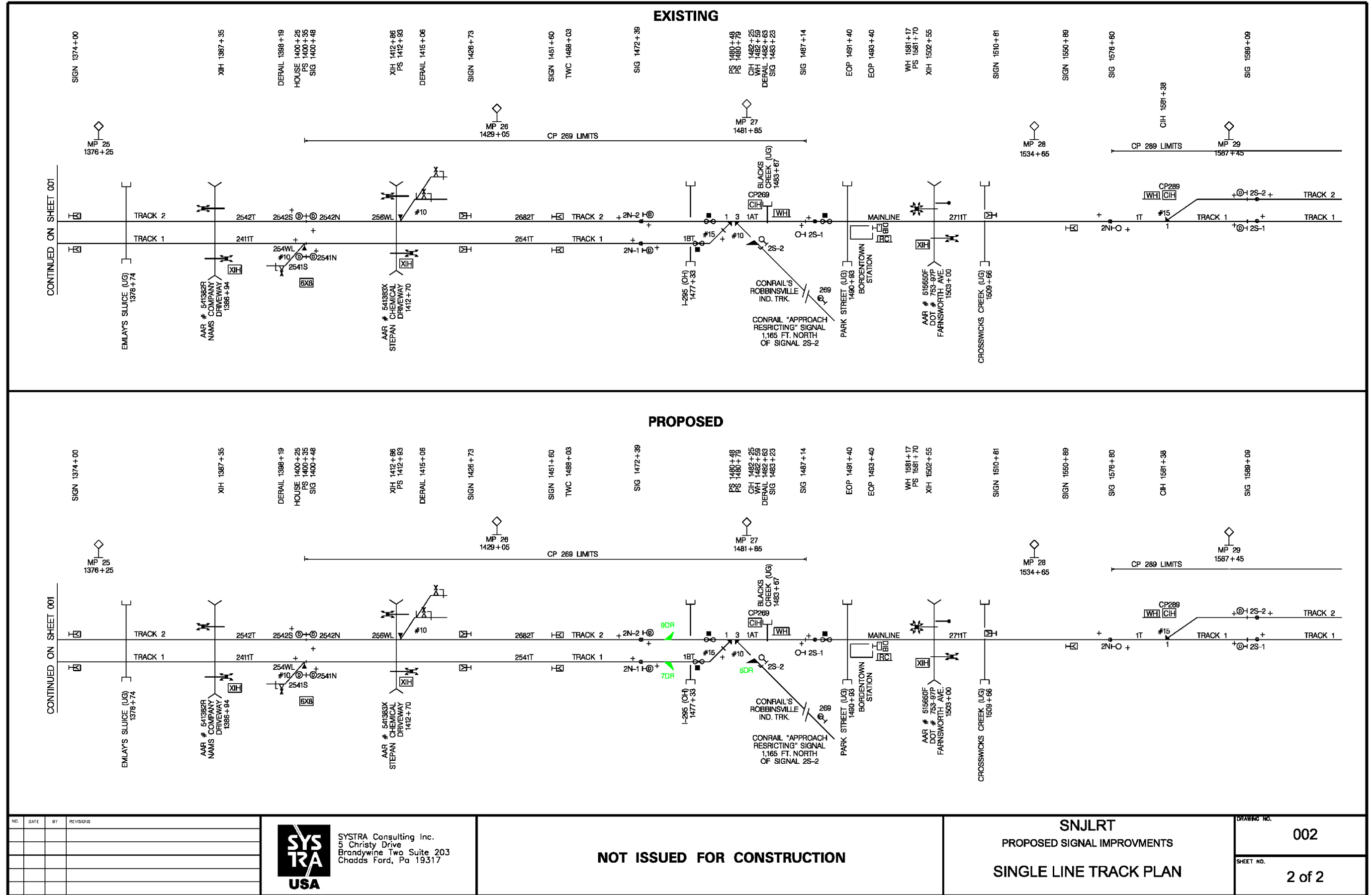
Figure 26 Existing Signal Plans and Proposed Signal and Train Operations Design Plans for the River LINE, Burlington Division, Drawing No. 2
