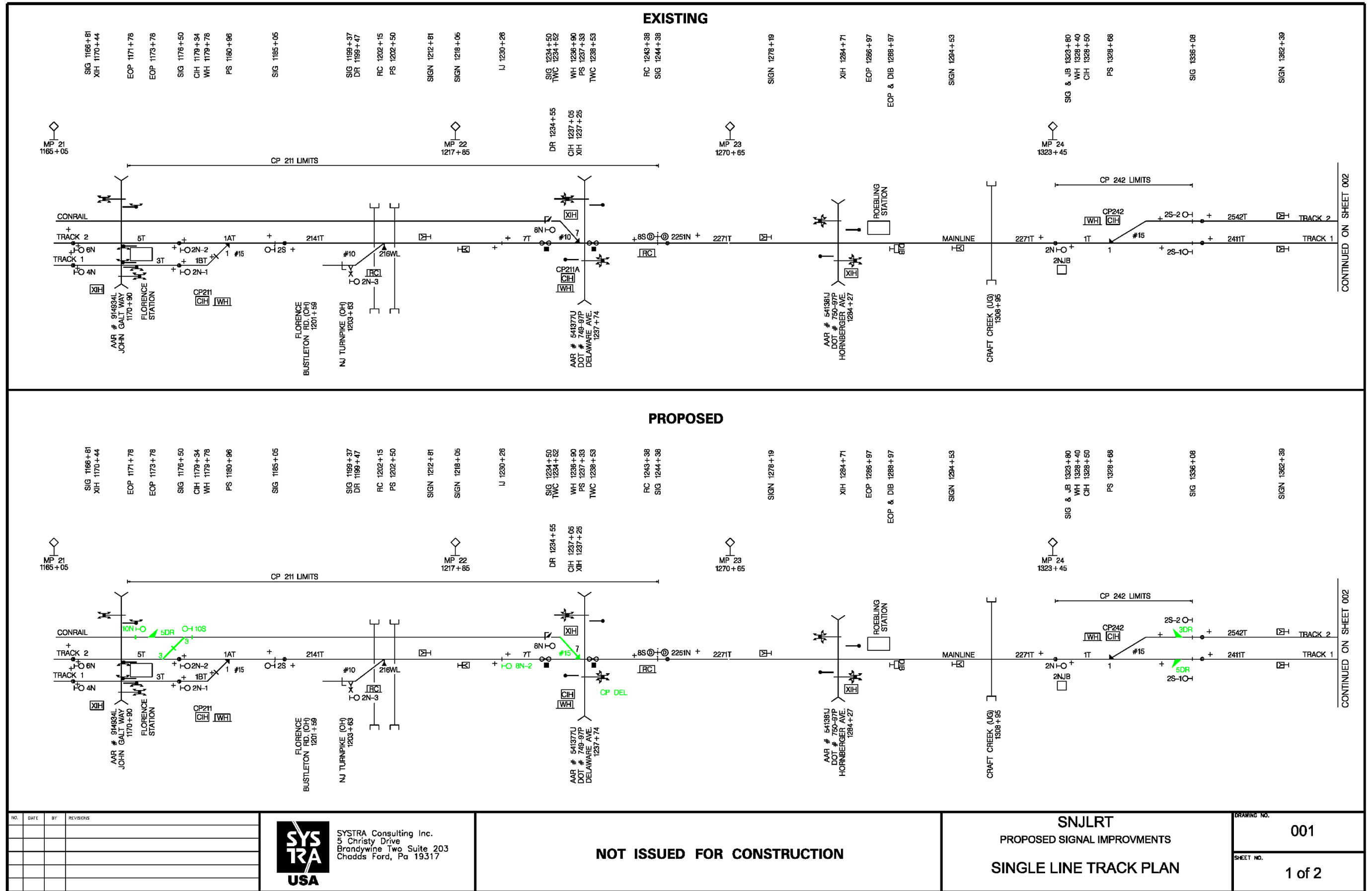
Figure 25 Existing Signal Plans and Proposed Signal and Train Operations Design Plans for the River LINE, Burlington Division, Drawing No. 1
