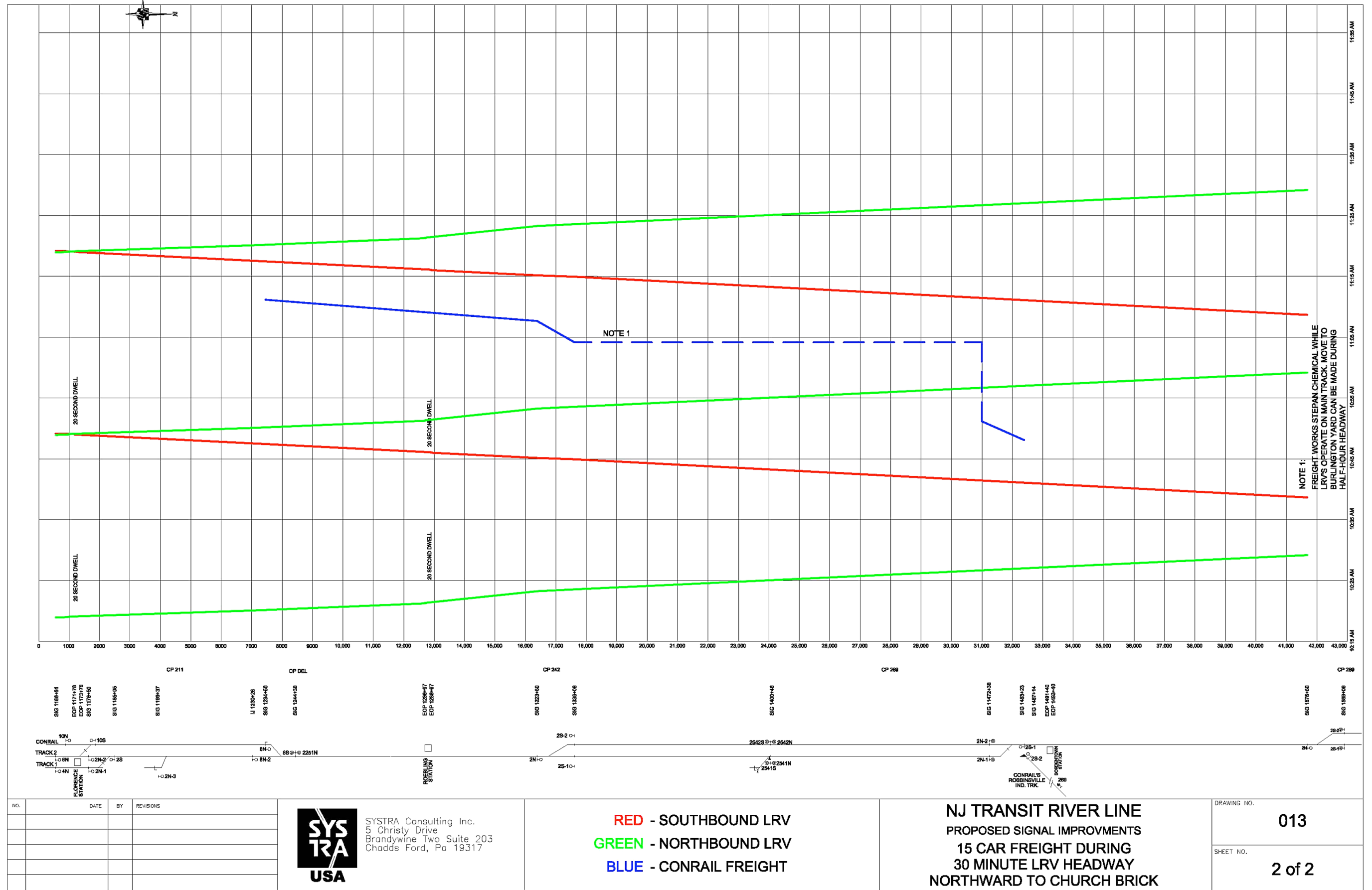
Figure 37 Existing Signal Plans and Proposed Signal and Train Operations Design Plans for the River LINE, Burlington Division, Drawing No. 13
