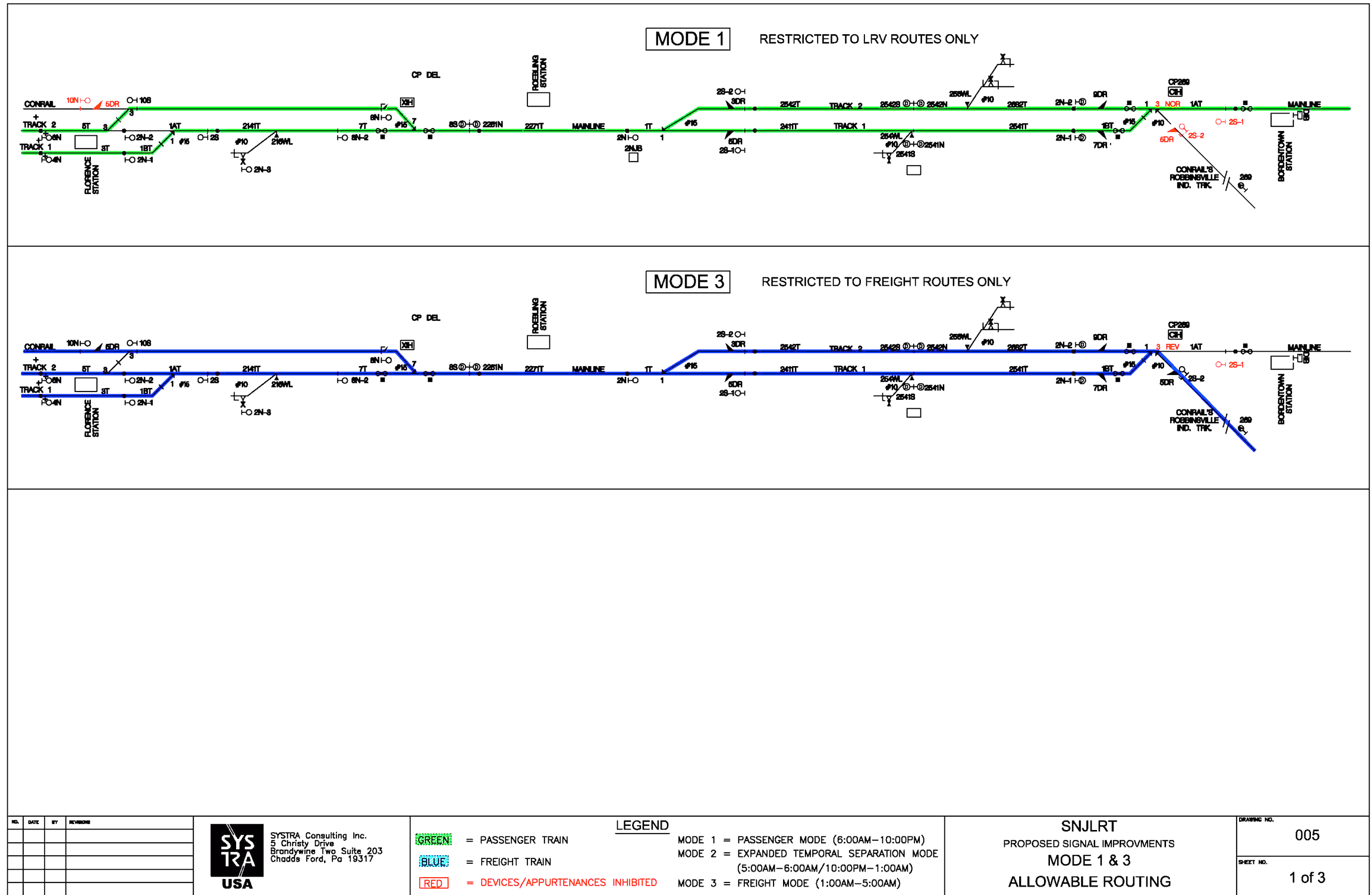
Figure 29 Existing Signal Plans and Proposed Signal and Train Operations Design Plans for the River LINE, Burlington Division, Drawing No. 5
