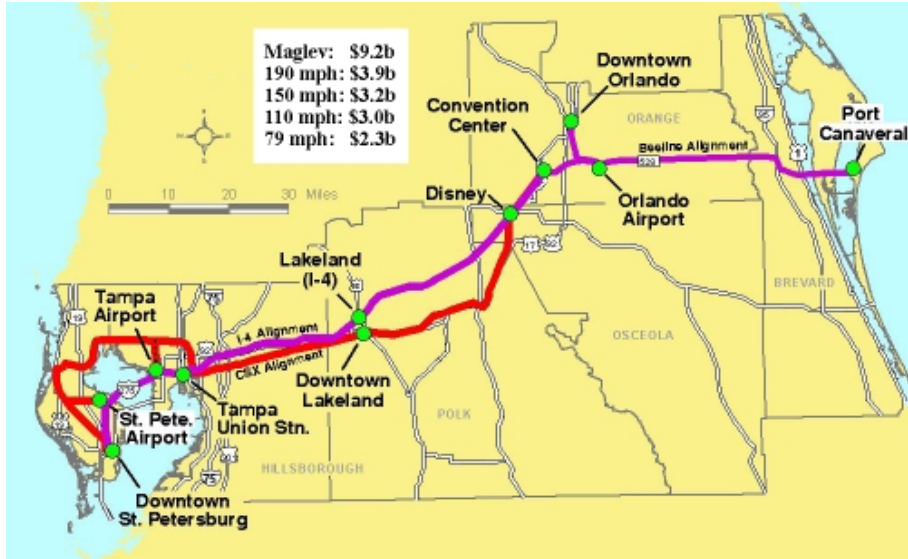
Figure 4: Route Alternative 1 -Full corridor from St. Petersburg to Port Canaveral. Could use I-4 or CSX right-of-way to Beeline. Provides direct connection between Disney, Orange County Convention Center, Downtown Orlando, and Orlando International Airport.
