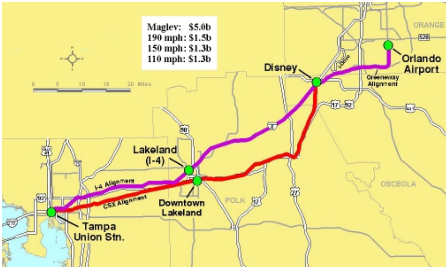
Figure 8: Route Alternative 5- Truncated Greenway alignment connecting Tampa to Orlando. Connections to Disney and Orlando International Airport only.
