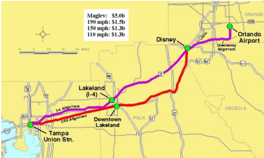
Figure 3.6: Route Alternative 5- Truncated Greenway alignment connecting Tampa to Orlando. Connections to Disney and Orlando International Airport only.
