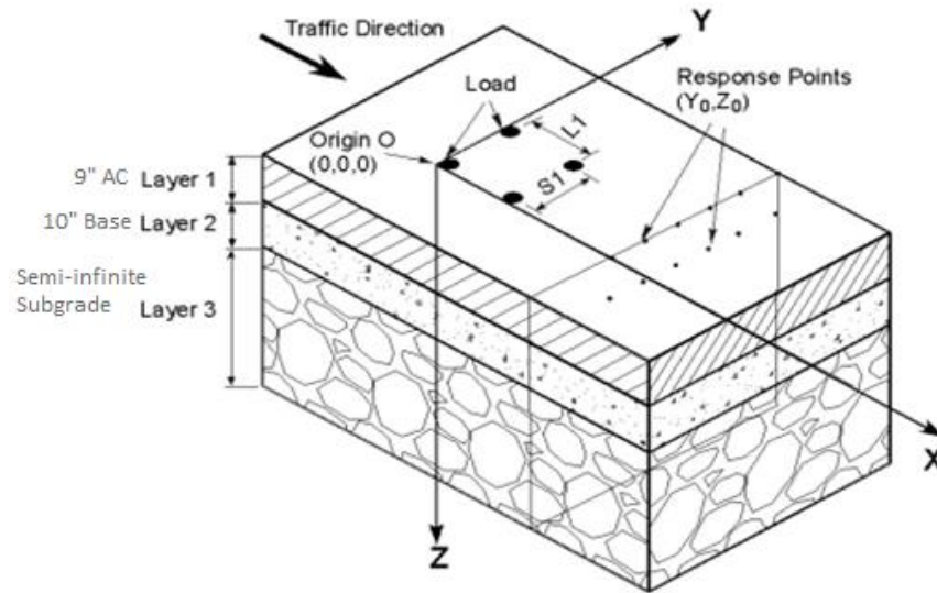
Figure 24. Picture. 3D schematic of the pavement structure in 3D-Move Analysis. (12)
