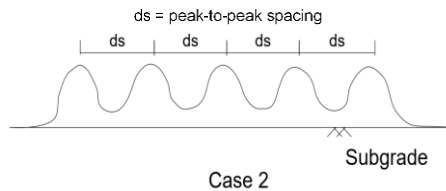
Figure 17. Illustration. \sigma_v distribution within pavement—case 2.
