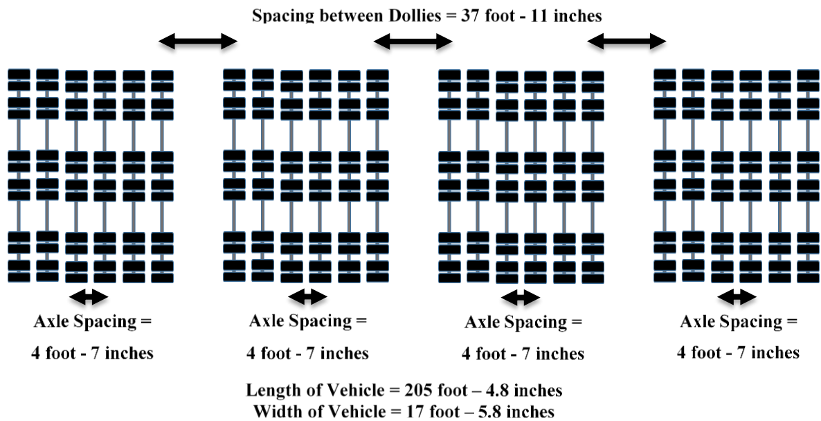
Figure 79. Illustration. Example configuration of a permitted SHL vehicle (LA-12T-16).
