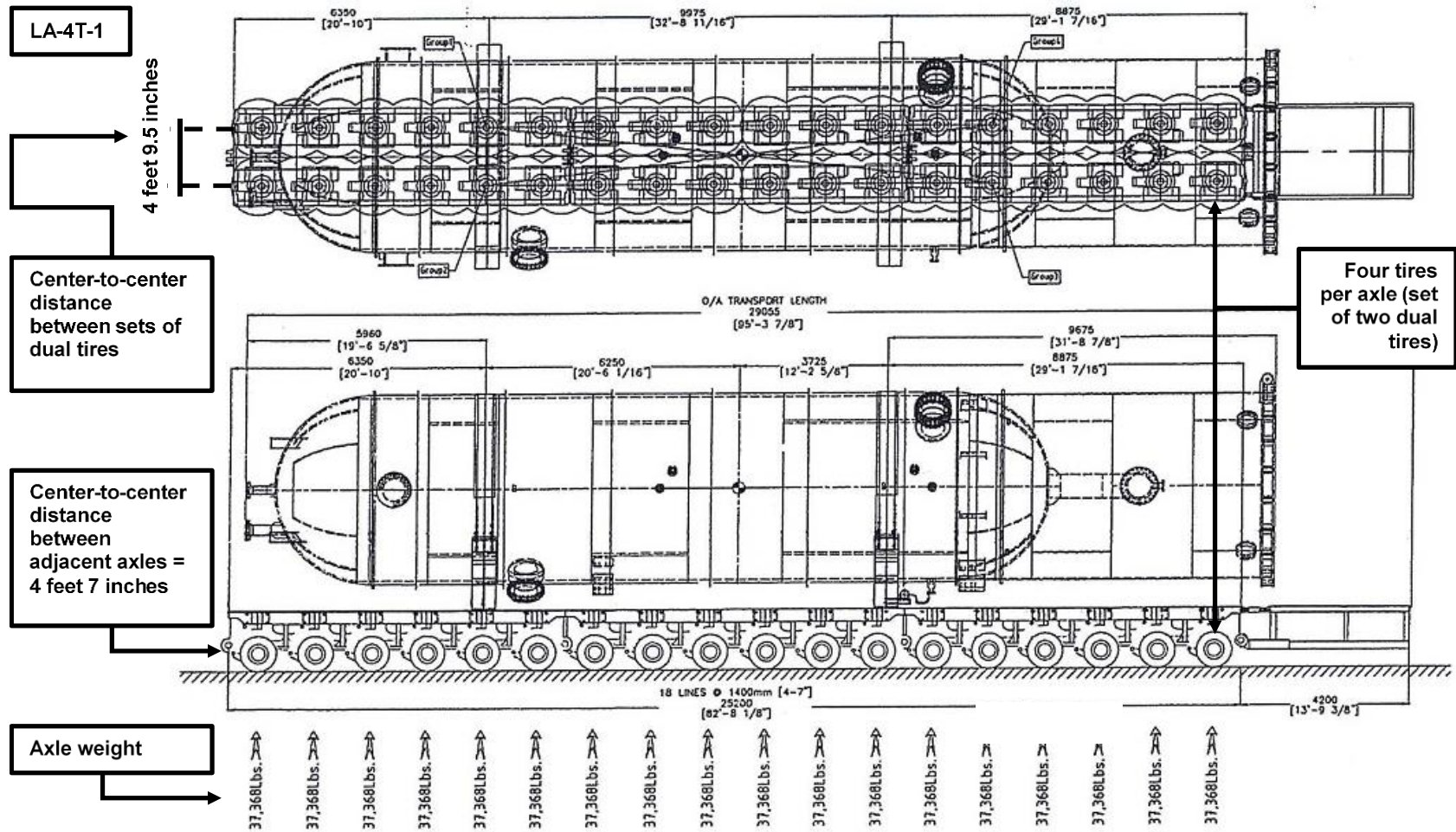
Figure 5. Picture. Example of relevant information from an SHL permit in Louisiana: transport configuration for D-943-004 (hot low-pressure separator) on 18 line axles.
