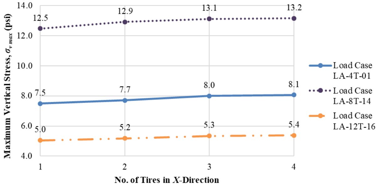
Figure 69. Chart. Change in \sigma_{v\ max} with added tires in x -direction (all SHL cases, 100 °F, PS 1).
