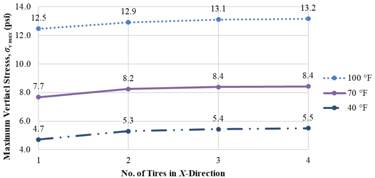
Figure 71. Chart. \sigma_{v\ max} change with tires in x -direction for three temperatures.
