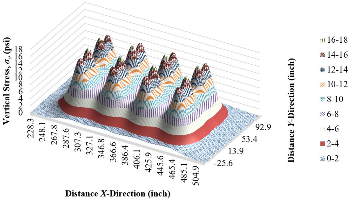
Figure 47. Chart. \sigma_v distribution on top of SG four by four tires (SHL case No. 2: LA-8T-14, 100 °F, PS 1)—3D view.
