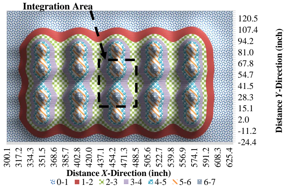
Figure 68. Chart. \sigma_v distribution on top of SG four by four tires (SHL case No. 3: LA-12T-16, 100 °F, PS 1)—top view.
