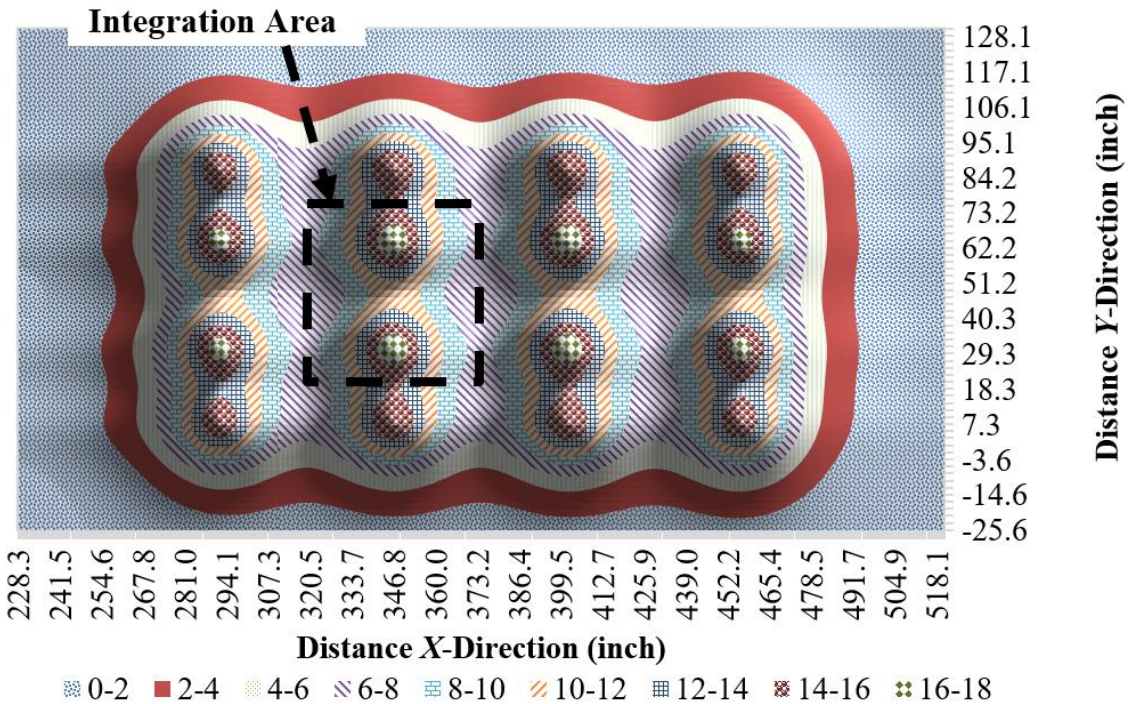
Figure 48. Chart. \sigma_v distribution on top of SG four by four tires (SHL case No. 2: LA-8T-14, 100 °F, PS 1)—top view.
