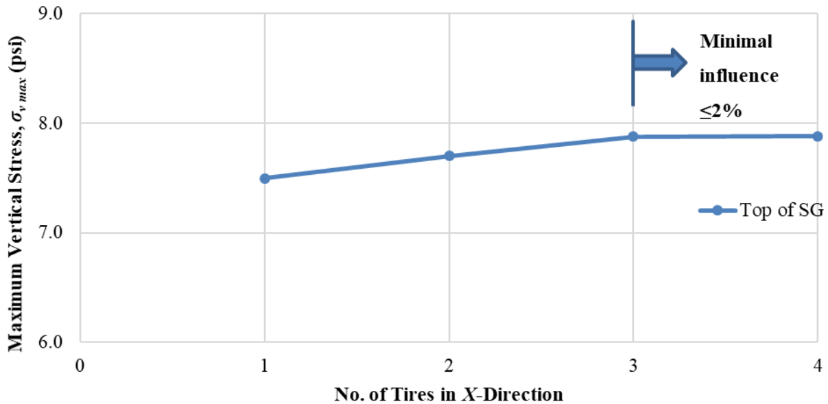
Figure 57. Chart. Change in \sigma_{v\ max} with added tires in x -direction (SHL case No. 1: LA-4T-1, 100 °F, PS 1).
