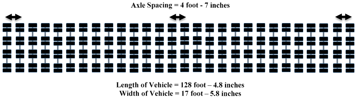
Figure 78. Illustration. Example configuration of a permitted SHL vehicle (LA-8T-14).
