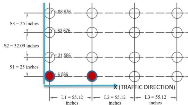
Figure 20. Illustration. Incremental tire-load approach—two tires (red-filled circles).
