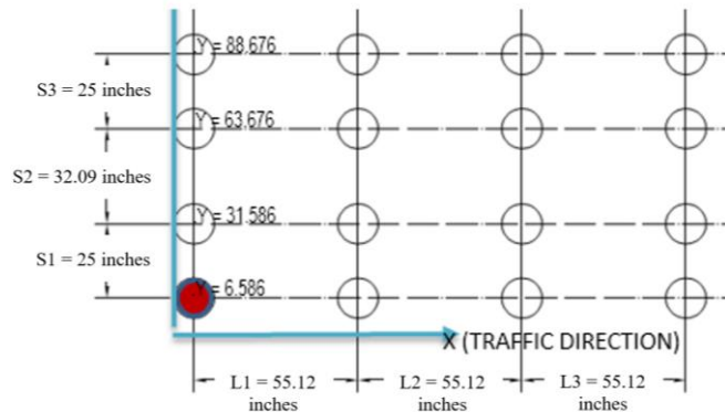
Figure 19. Illustration. Incremental tire-load approach—single tire (red-filled circle).
