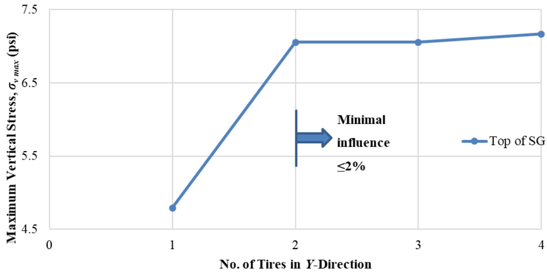
Figure 52. Chart. Change in \sigma_{v, max} with added tires in y-direction (SHL case No. 2: LA-8T-14, 100 °F, PS 3).
