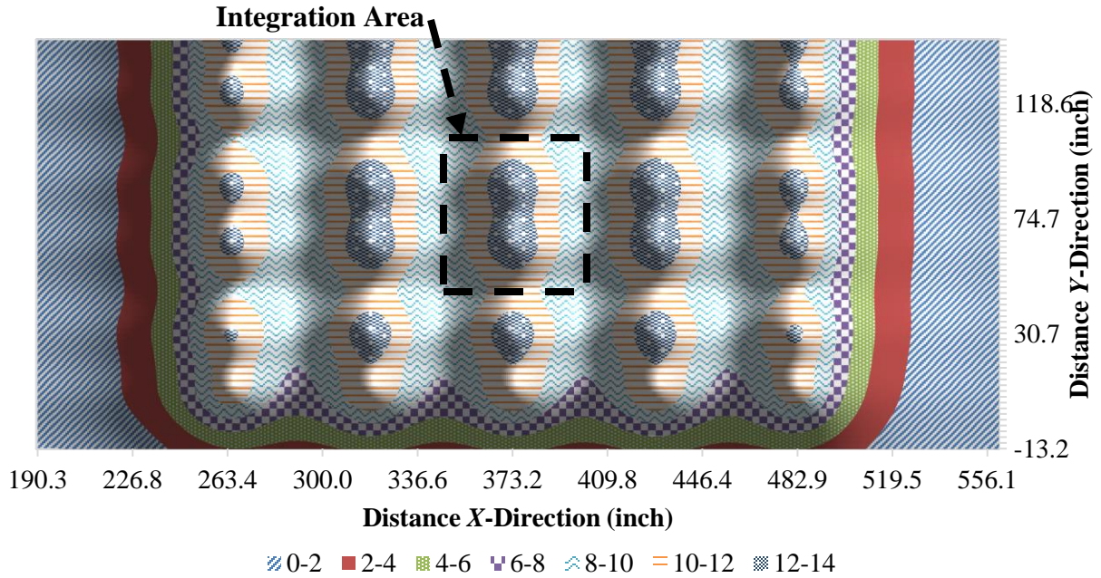
Figure 38. Chart. \sigma_v distribution on top of SG five by six tires (SHL case No. 2: LA-8T-14, 100 °F, PS 2)—top view.
