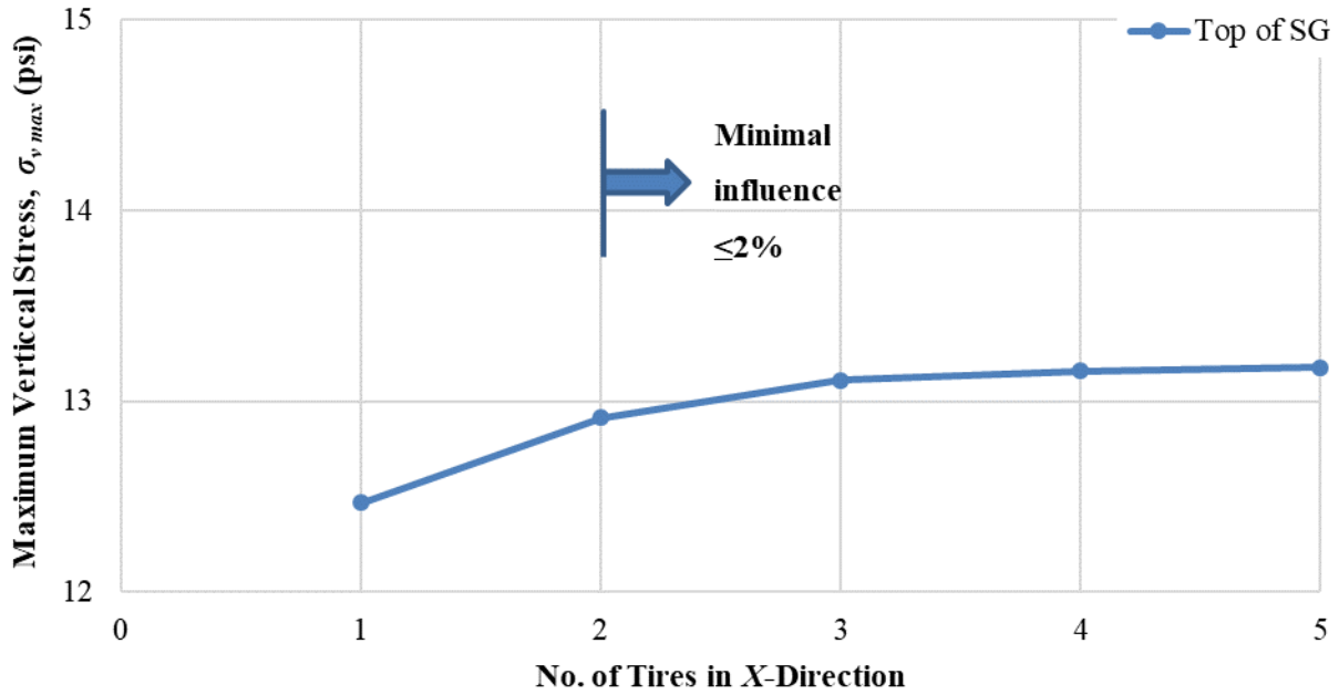
Figure 42. Chart. Change in \sigma_{v\ max} with added tires in x -direction (SHL case No. 2: LA-8T-14, 100 °F, PS 1).
