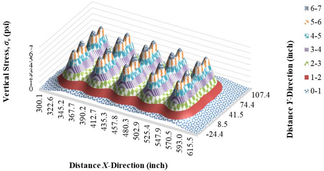
Figure 67. Chart. \sigma_v distribution on top of SG four by four tires (SHL case No. 3: LA-12T-16, 100 °F, PS 1)—3D view.
