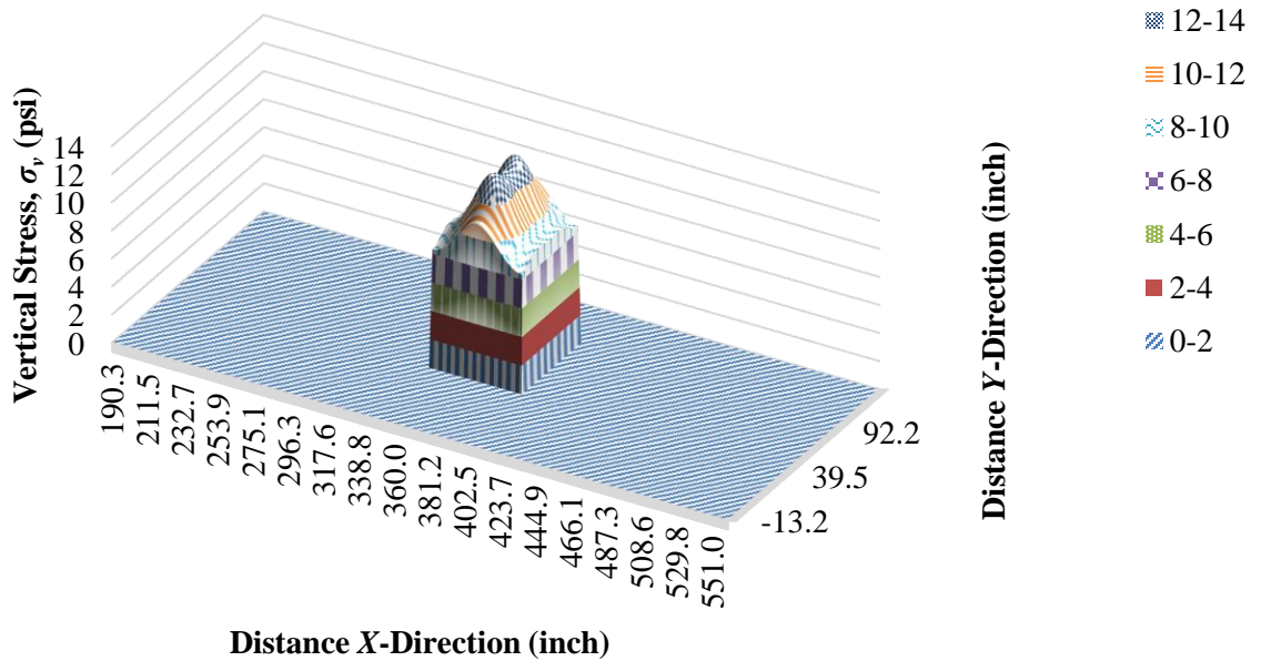
Figure 39. Chart. \sigma_v distribution at middle dual tires on top of SG (SHL case No. 2: LA-8T-14, 100 °F, PS 2)—3D view.
