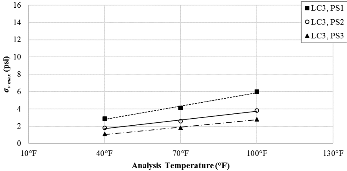
Figure 75. Chart. Change in \sigma_{v \max} with temperature for various pavement structures (SHL case No. 2: LA-8T-14).
