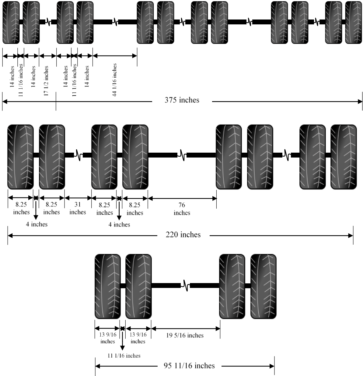
Figure 6. Illustration. Observed common tire configurations in Louisiana (not to scale).
