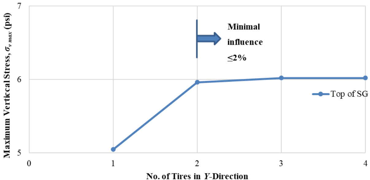
Figure 64. Chart. Change in \sigma_{v\ max} with added tires in y-direction (SHL case No. 3: LA-12T-16, 100 °F, PS 1).
