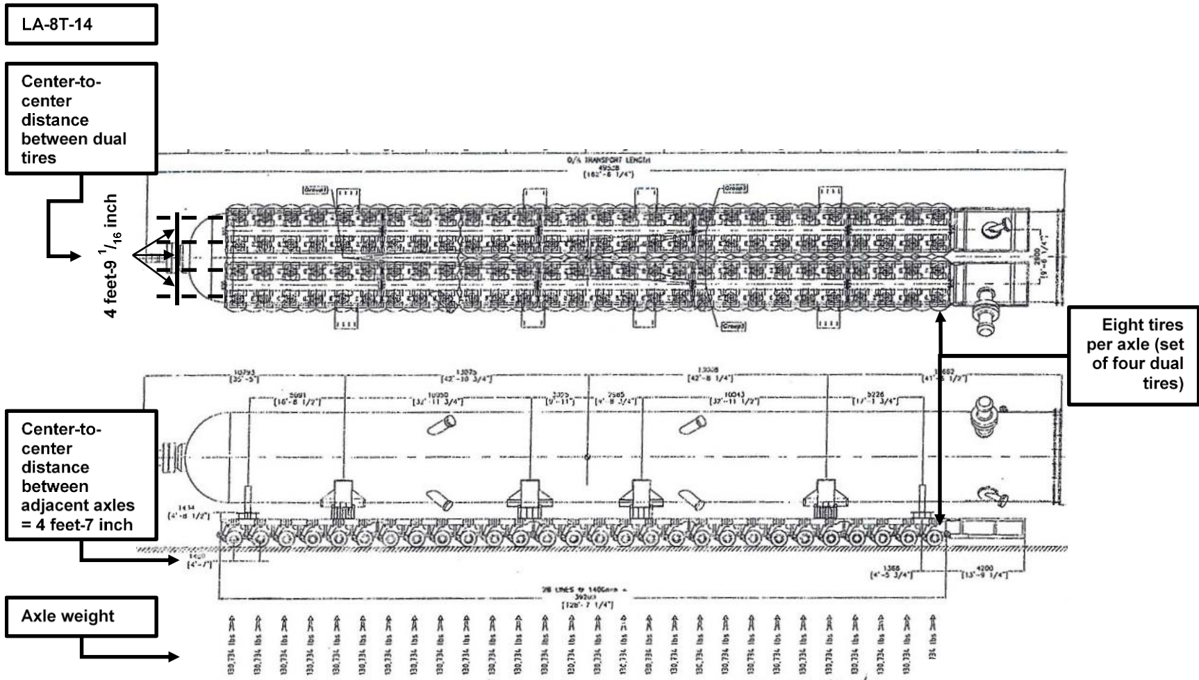
Figure 40. Picture. SHL-vehicle case analysis (reactors transport)—case No. 2: LA-8T-14.
