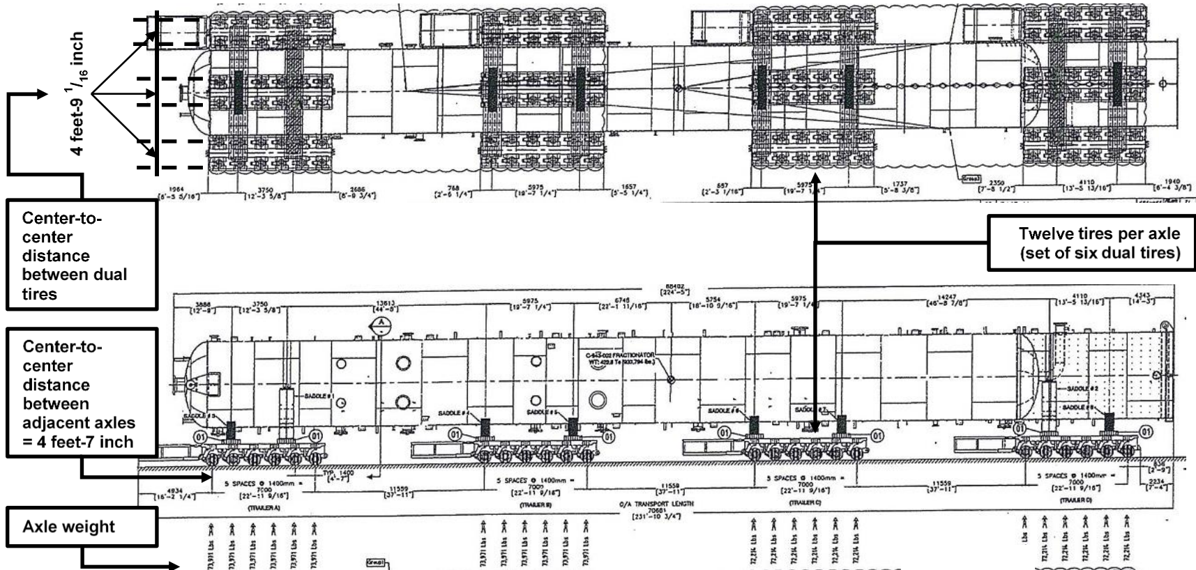
Figure 41. Picture. SHL-vehicle case analysis (C-943-002 fractionator)—case No. 3: LA-12T-16.
