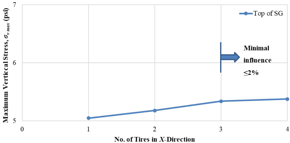
Figure 62. Chart. Change in \sigma_{v\ max} with added tires in x -direction (SHL case No. 3: LA-12T-16, 100 °F, PS 1).
