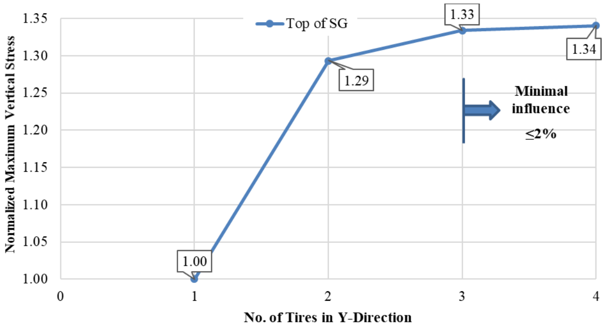
Figure 35. Chart. Normalized \sigma_{v \max} as a function of number of tires in y-direction (SHL case No. 2: LA-8T-14, 100 °F, PS2).
