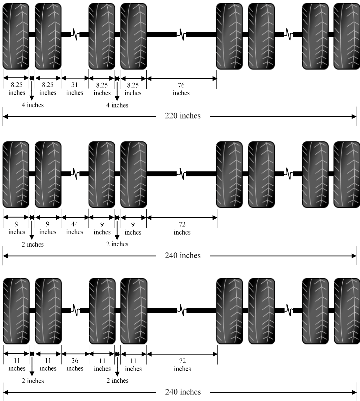
Figure 2. Illustration. Observed common tire configurations in Arizona (not to scale).
