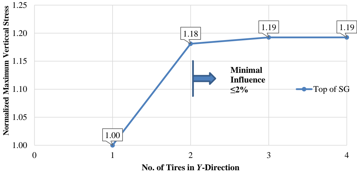
Figure 65. Chart. Change in normalized \sigma_{v\ max} with added tires in y-direction (SHL case No. 3: LA-12T-16, 100 °F, PS 1).
