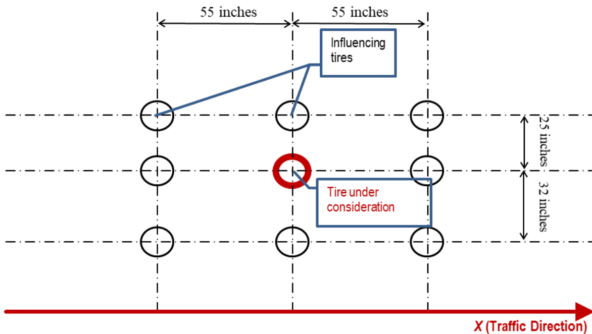
Figure 73. Chart. Representative nucleus of SHL axle configuration (70 °F, 40 °F).
