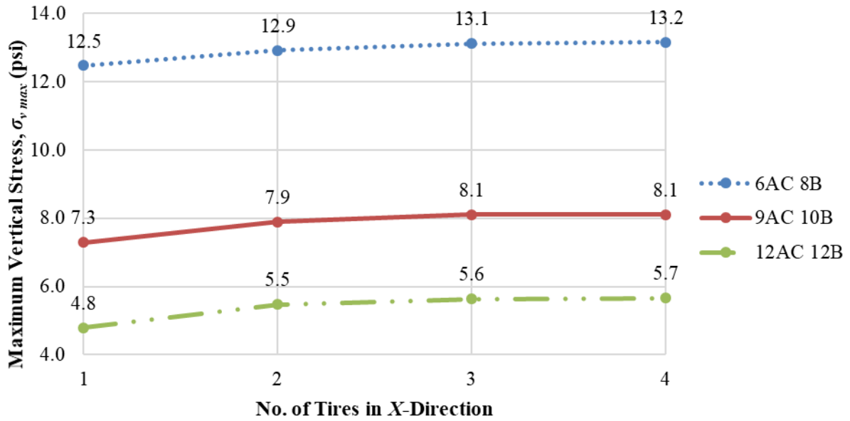
Figure 55. Chart. Change in \sigma_{v\ max} with added tires in x-direction (SHL case No. 2: LA-8T-14, 100 °F, all PSs).
