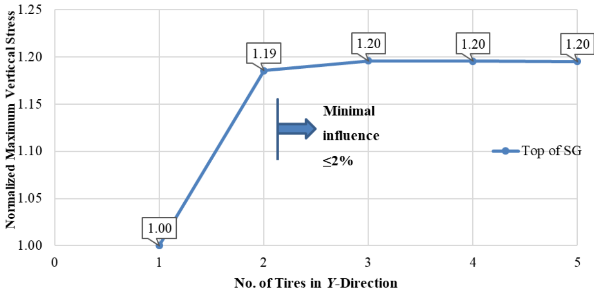
Figure 44. Chart. Change in \sigma_{v \max} with added tires in y-direction (SHL case No. 2: LA-8T-14, 100 °F, PS 1).
