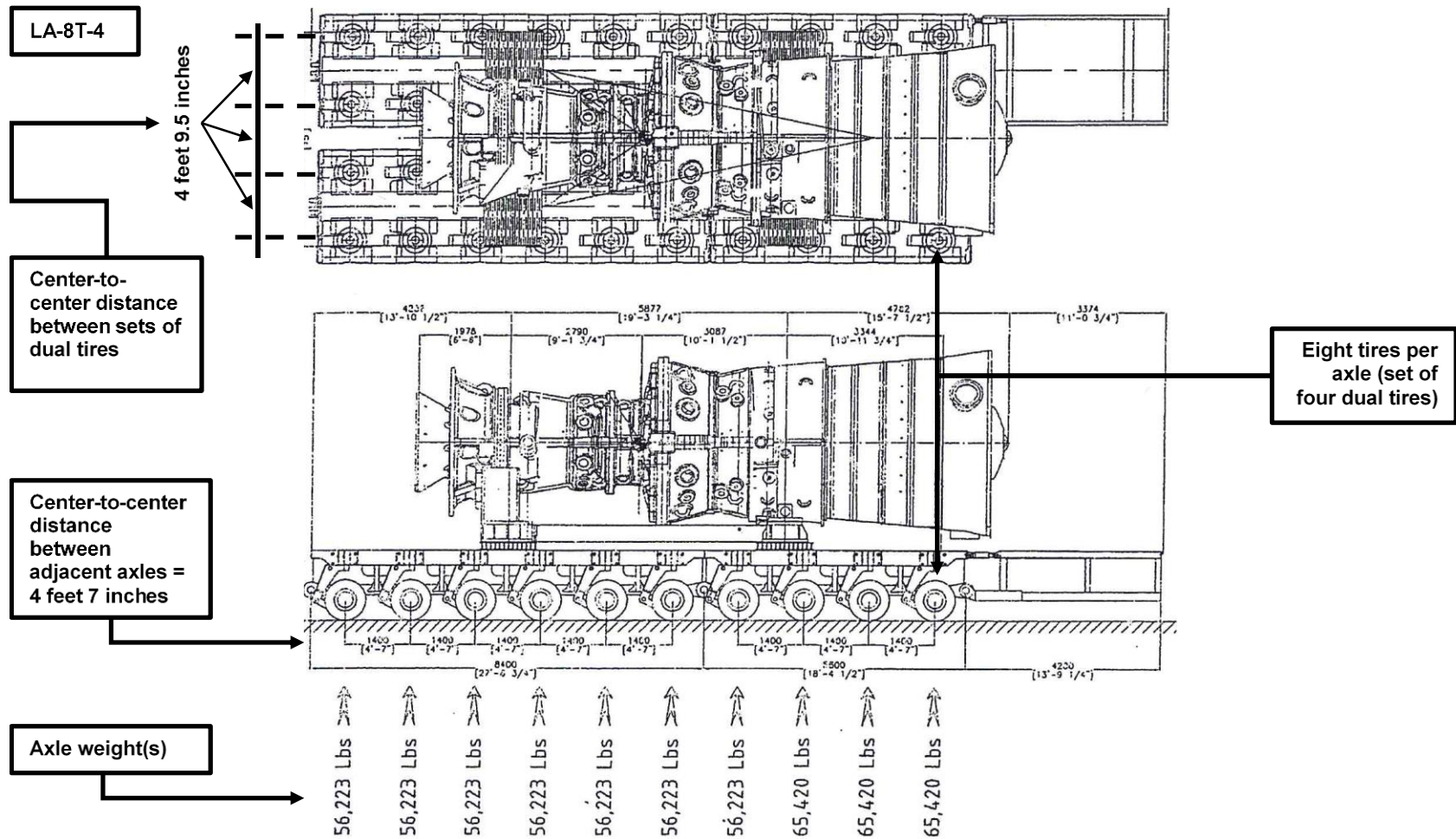
Figure 4. Picture. Example of relevant information from an SHL permit in Louisiana: transport configuration for gas-turbine package.
