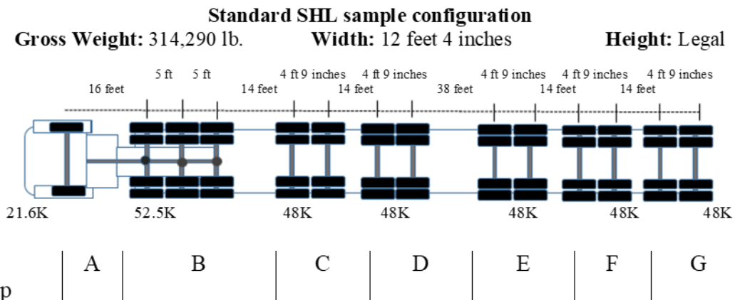
Figure 79. Illustration. Example configuration of a permitted SHL vehicle (LA-12T-16).
