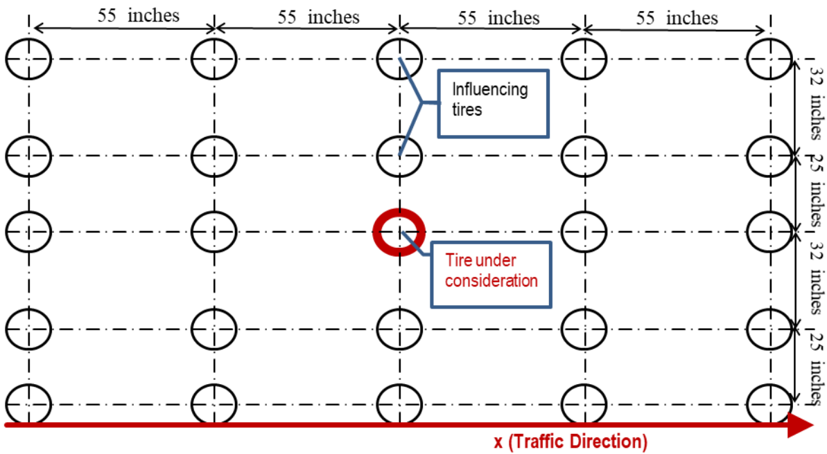
Figure 36. Chart. Representative nucleus (SHL case No. 2: LA-8T-14, 100 °F, PS 2).
