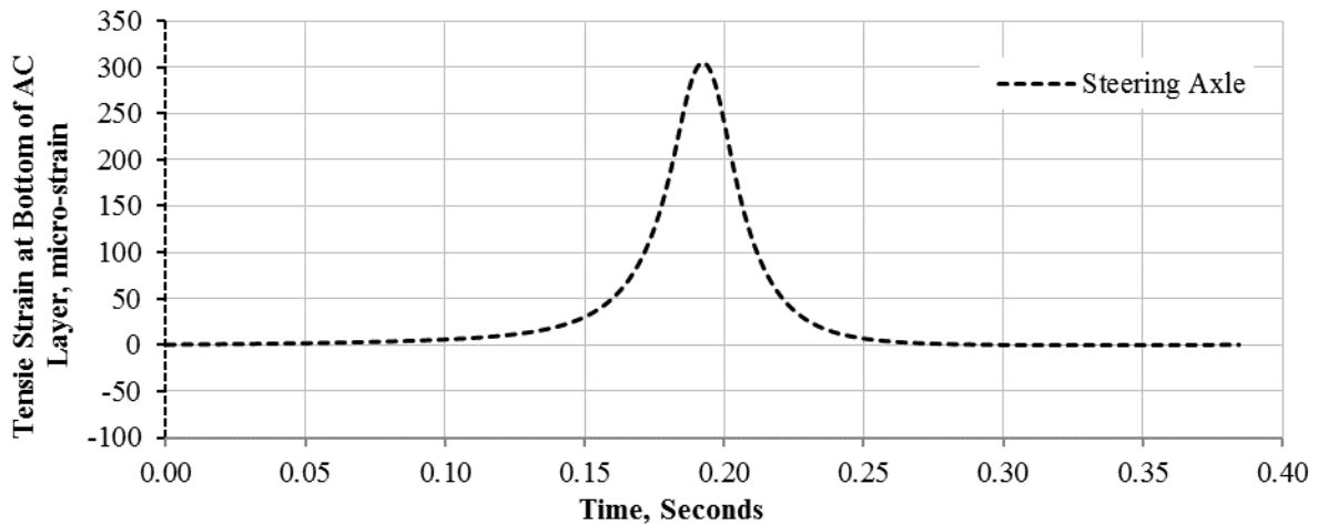
Figure 10. Graph. Tensile strain response history at the bottom of AC layer for axle group A (single axle).
