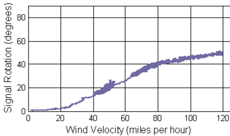
Figure A-10. Test 10: Pipe Hanger with 45° Signal and 45° Simulator Orientations
