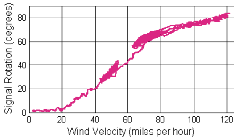
Figure A-24. Test 24: Pivotal Hanger with 90° Signal and 45° Simulator Orientations (Messenger on Front)
