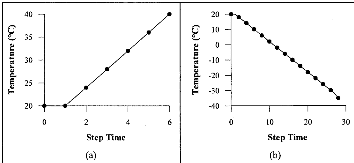
Figure 3.10. Amplitude curves for (a) positive and (b) negative temperature change
