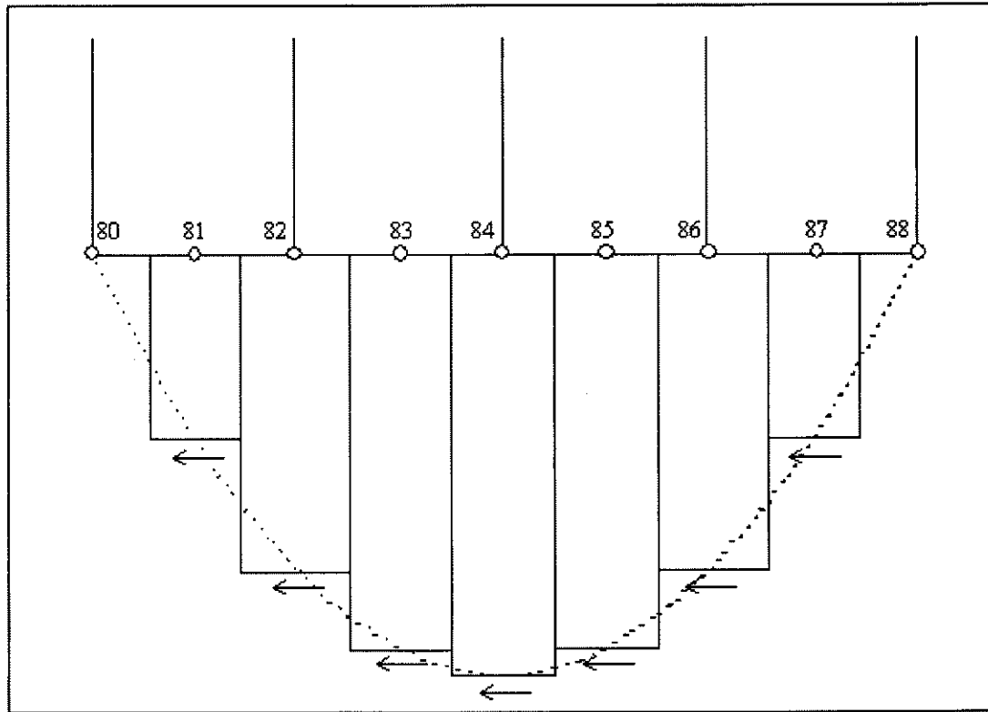
Figure 3.6. Distribution of equivalent reaction forces at pile toe
