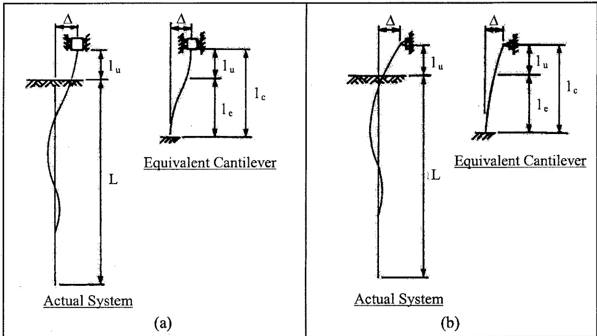
Figure 2.9. Equivalent cantilevers for: (a) fixed-head condition (b) pinned-head condition (Greimann et al., 1987)
