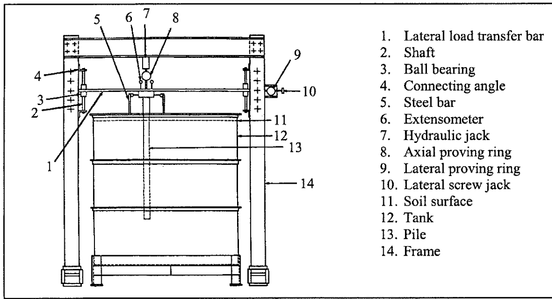
Figure 2.6. H-pile testing apparatus (after Amde et al, 1997)
