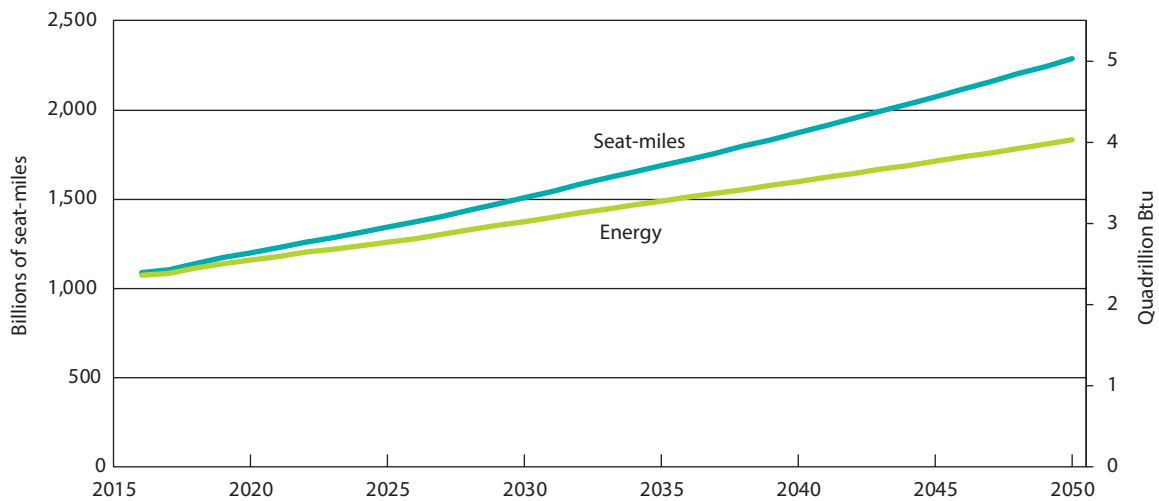
FIGURE 7-21 Air Transport Seat-Miles and Energy Use: 2015 Projected to 2050
