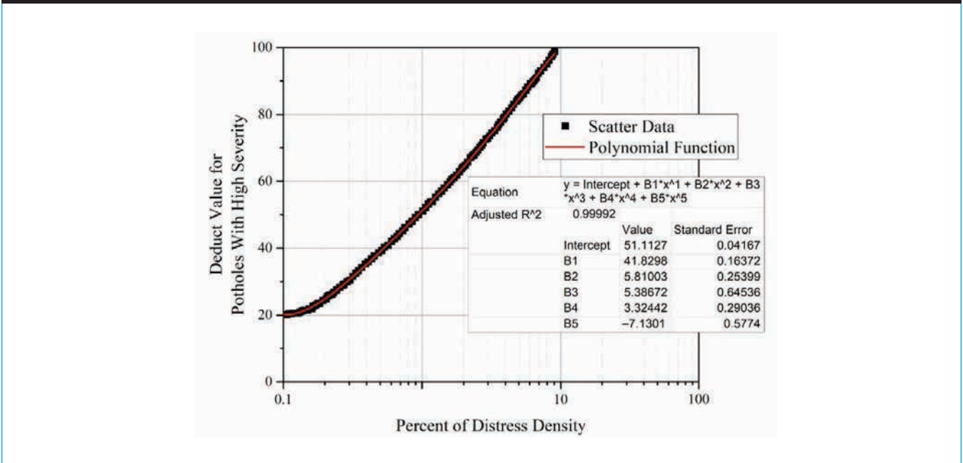
Figure 2. Graph. Fitting a polynomial to the ASTM deduct value curve highlighted in figure 1 and extracting the mathematical formula for potholes with a high severity (metric units).
