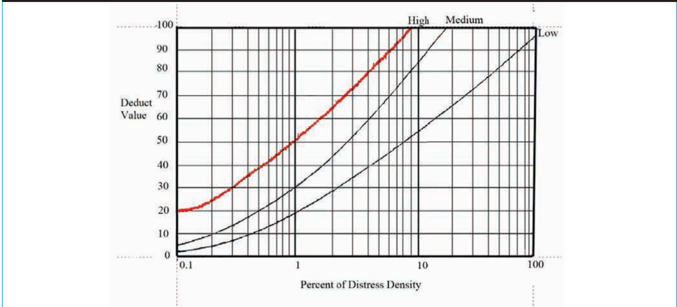
Figure 1. Graph. Digitized graph for calculation of deduct values for high-severity potholes (graph regenerated based on guidelines of ASTM D6433 - 07). (4)
