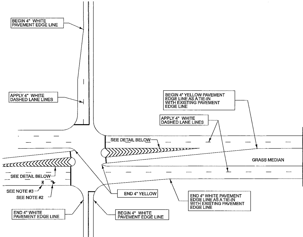
Figure 37. Illustration. SCDOT Standard Drawing 625-310-00 excerpts for turn lane installations (part 3).
