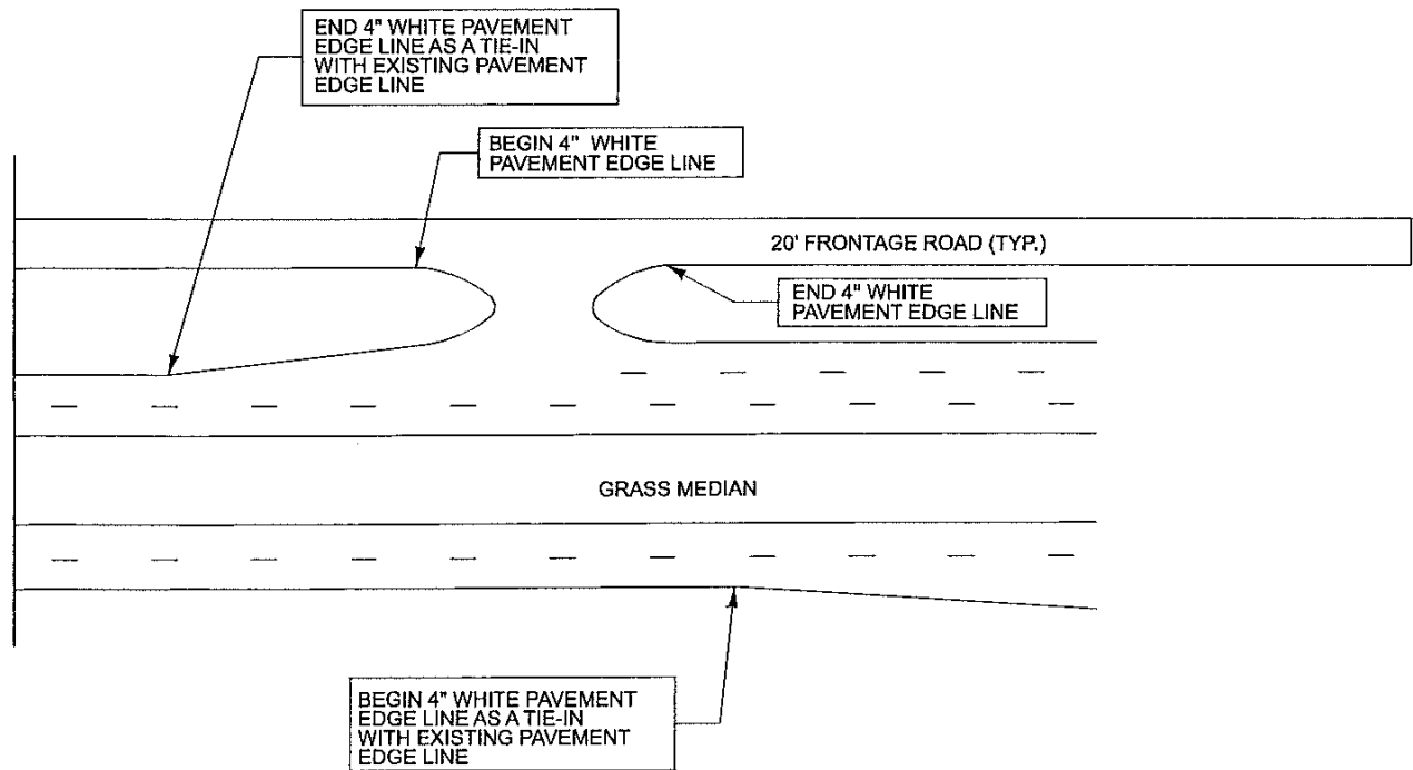
Figure 35. Illustration. SCDOT Standard Drawing 625-310-00 excerpts for turn lane installations (part 1).
