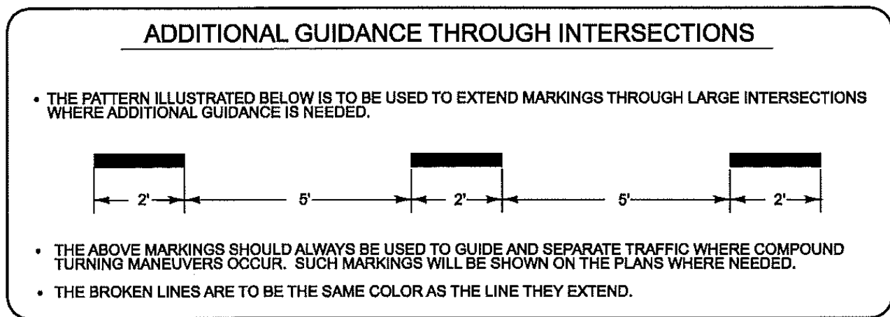
Figure 33. Illustration. SCDOT Standard Drawing 625-305-00 excerpt for guidance through intersections.
