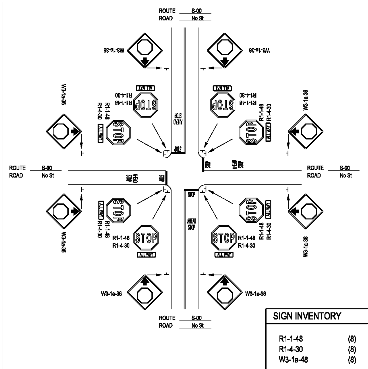
Figure 51. Illustration. SCDOT typical for a four-way stop controlled intersection.
