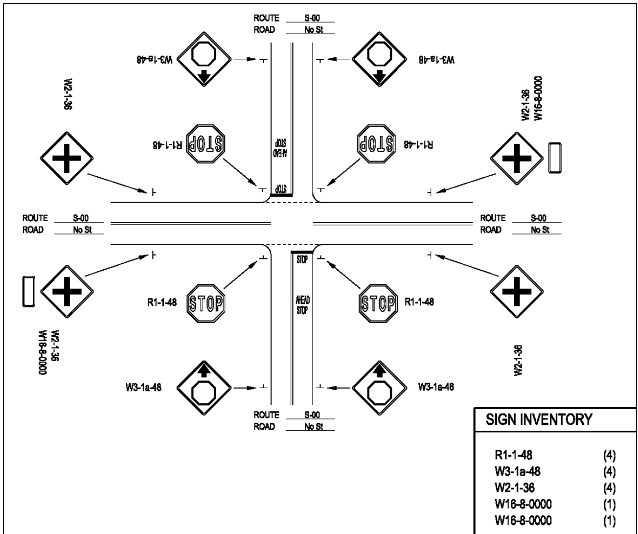
Figure 52. Illustration. SCDOT typical for a cross-type stop controlled intersection.
