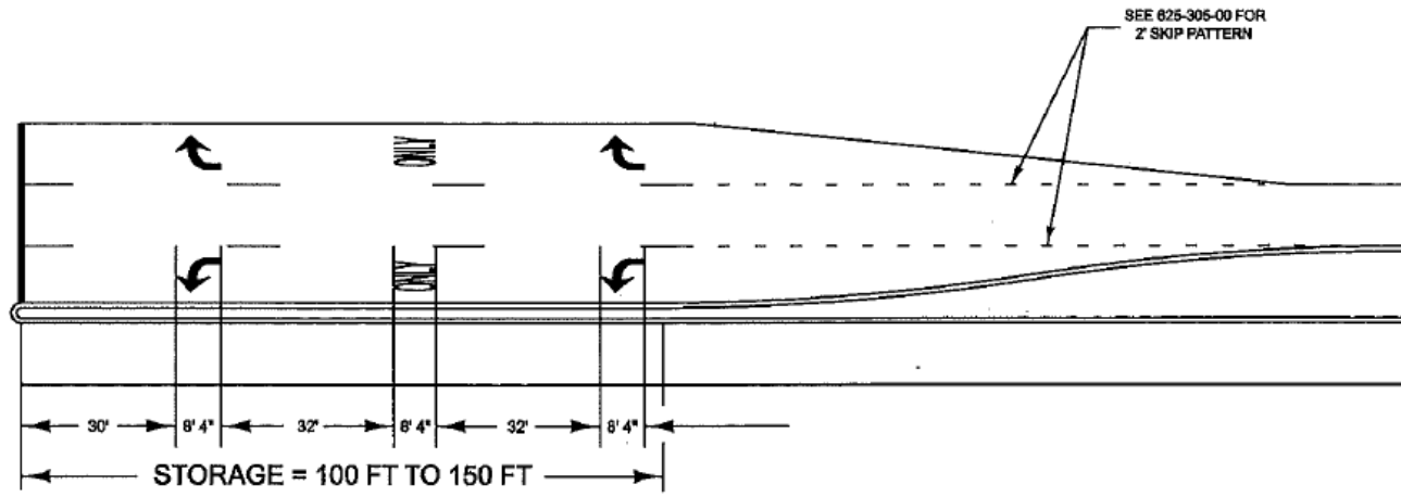
Figure 43. Illustration. SCDOT Standard Drawing 625-410-00 excerpt for right or left turn markings application.
