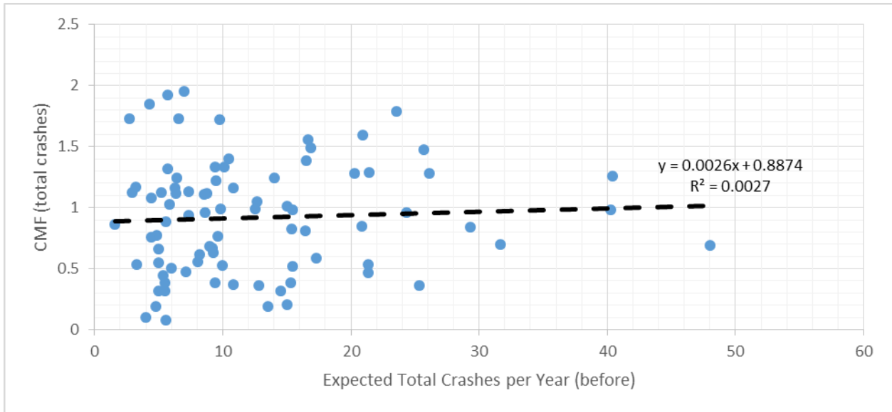
Figure 30. Chart. The relationship between CMF (total crashes) and expected total crashes during the before period.
