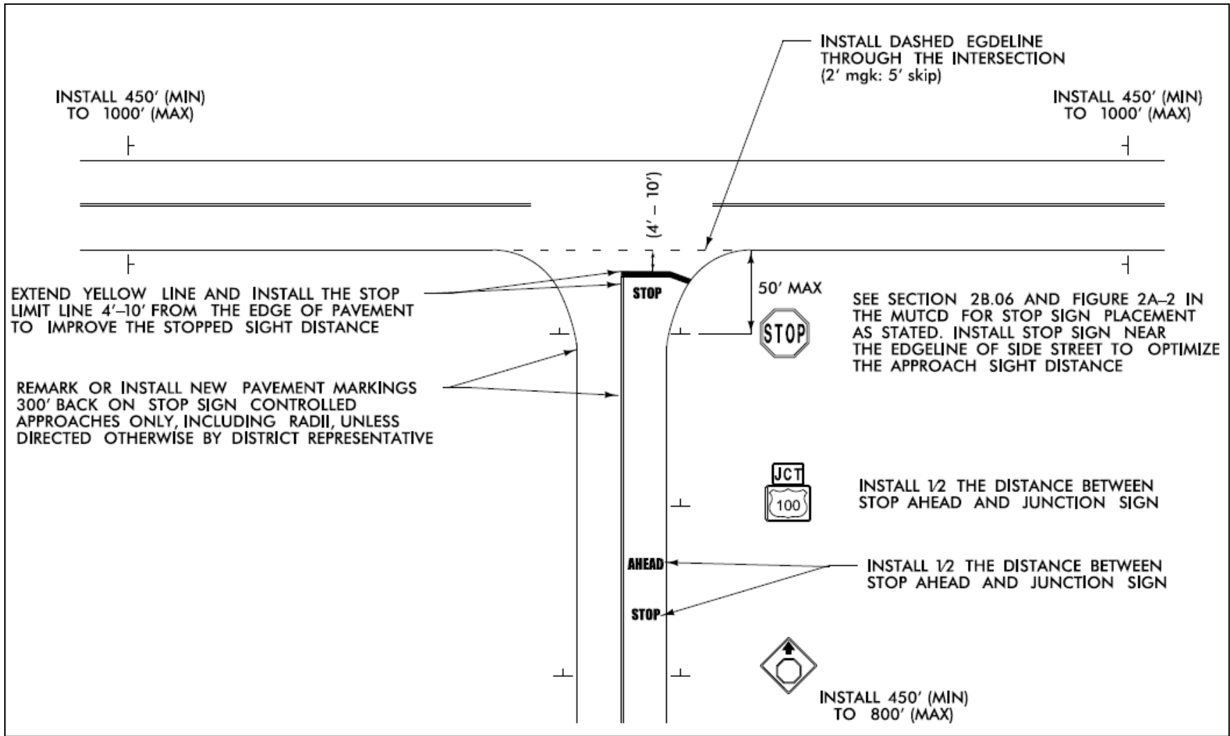
Figure 48. Illustration. SCDOT nonsignalized intersection design for pavement marking and sign installations.
