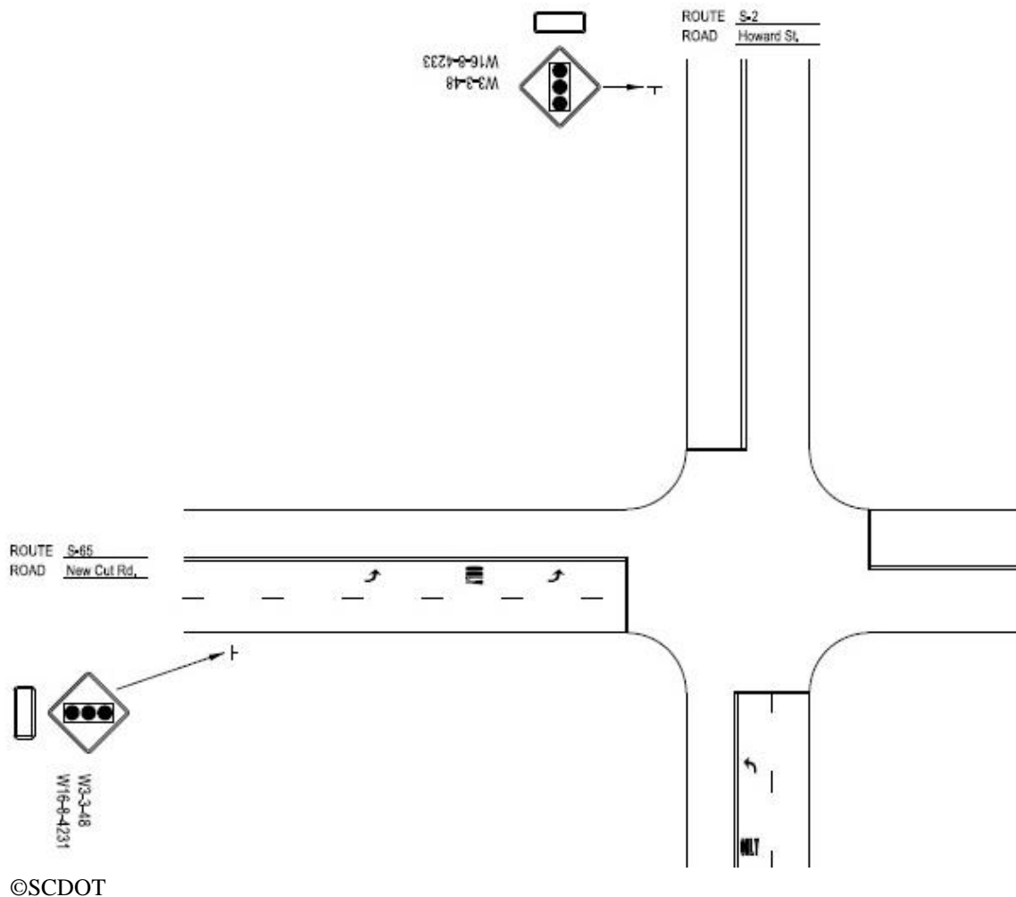
Figure 7. Illustration. Collecting the number of legs and verifying the number of lanes from the work plan.
