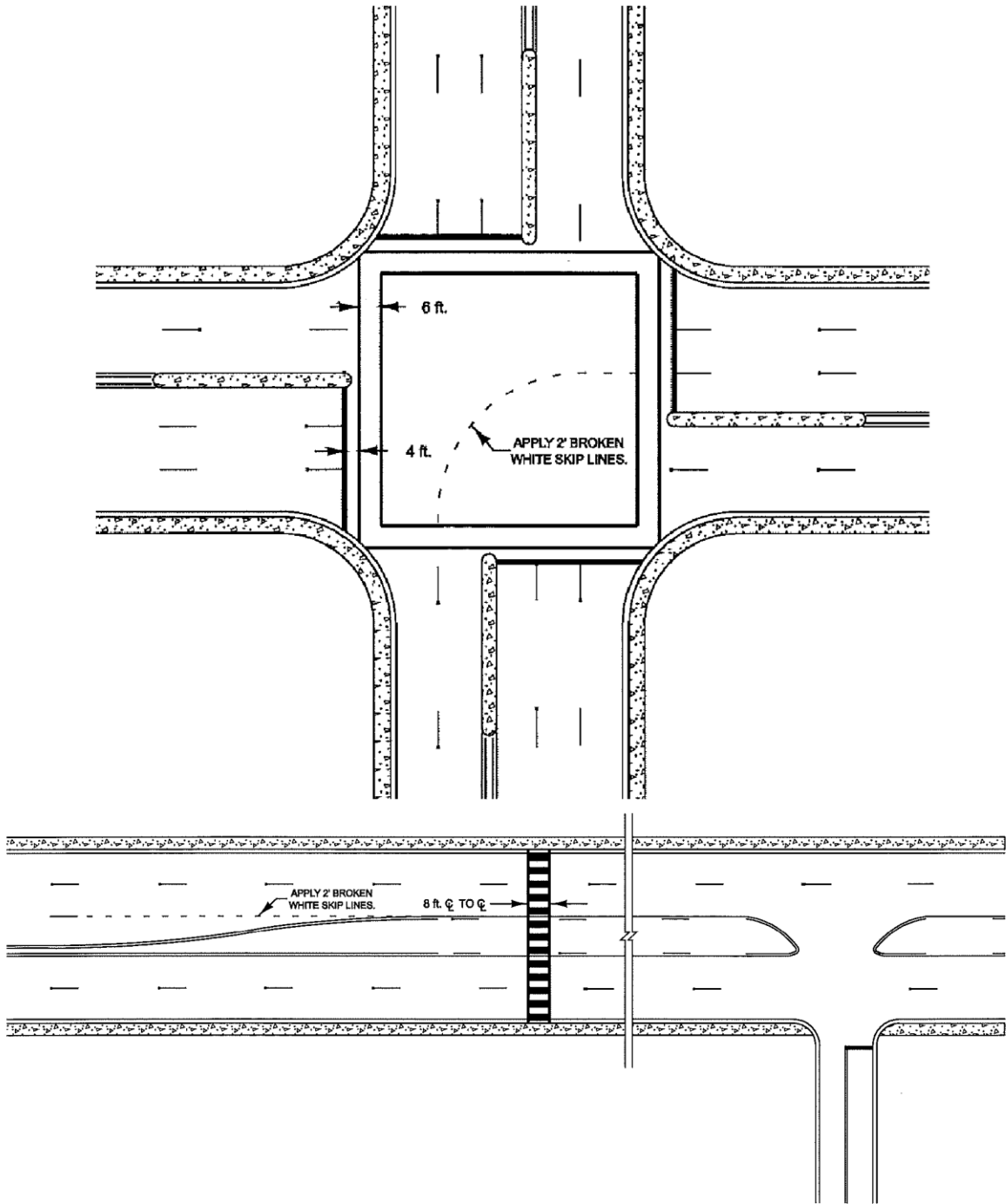
Figure 32. Illustration. SCDOT Standard Drawing 625-305-00 excerpts for application of markings at intersections.
