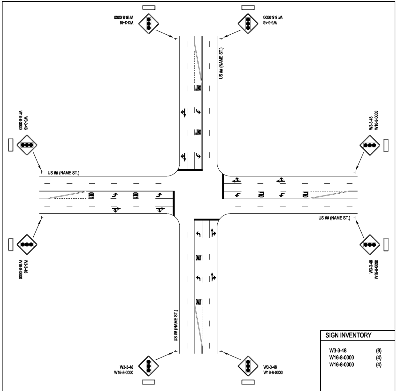
Figure 50. Illustration. SCDOT typical for a signalized intersection.
