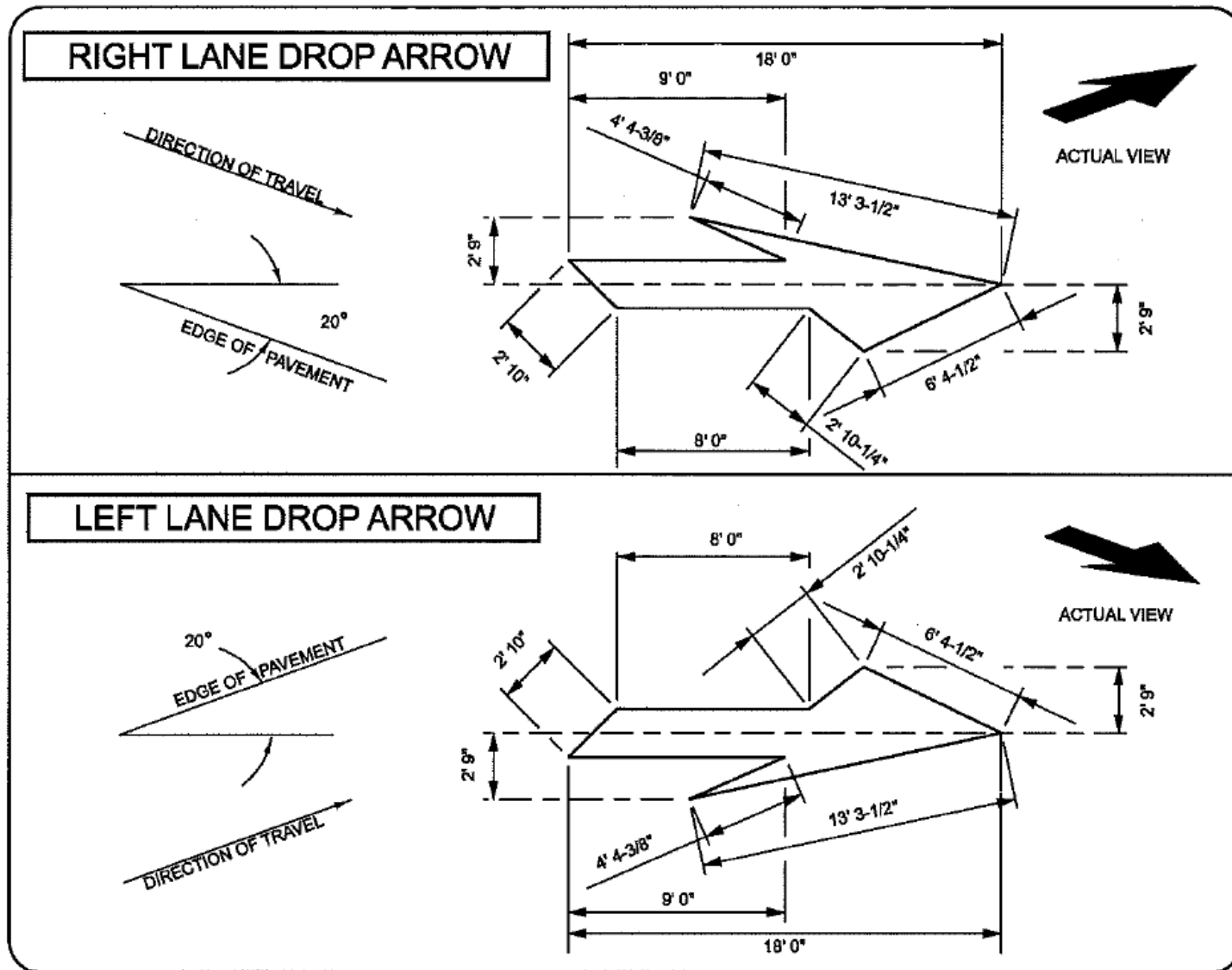
Figure 41. Illustration. SCDOT Standard Drawing 625-410-00 excerpt for right lane drop arrow and left lane drop arrow standard pavement marking.
