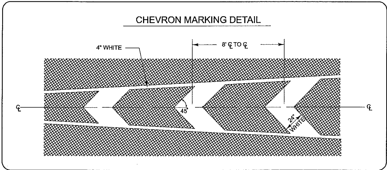
Figure 38. Illustration. SCDOT Standard Drawing 625-310-00 excerpts for chevron marking details.
