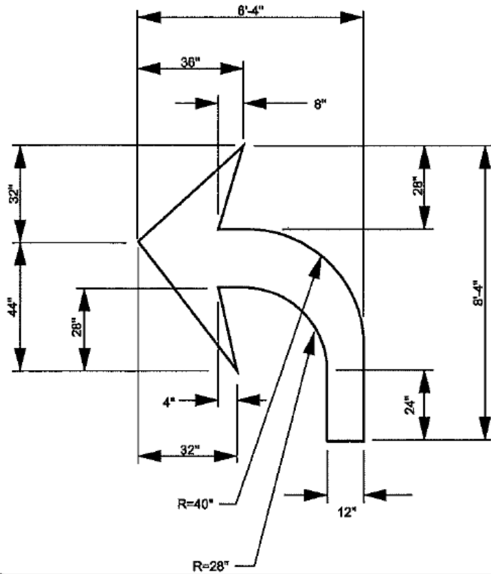
Figure 40. Illustration. SCDOT Standard Drawing 625-410-00 excerpt for right or left turn arrow and combination straight and left or right turn arrow standard pavement marking.
