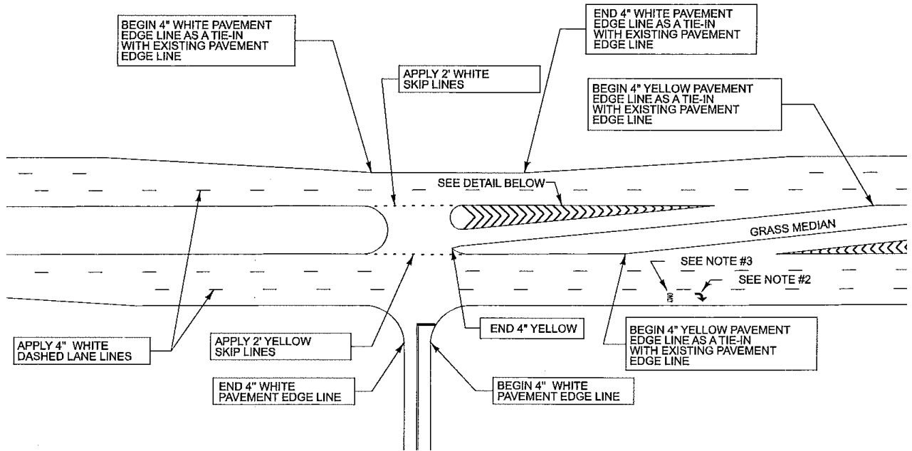
Figure 36. Illustration. SCDOT Standard Drawing 625-310-00 excerpts for turn lane installations (part 2).
