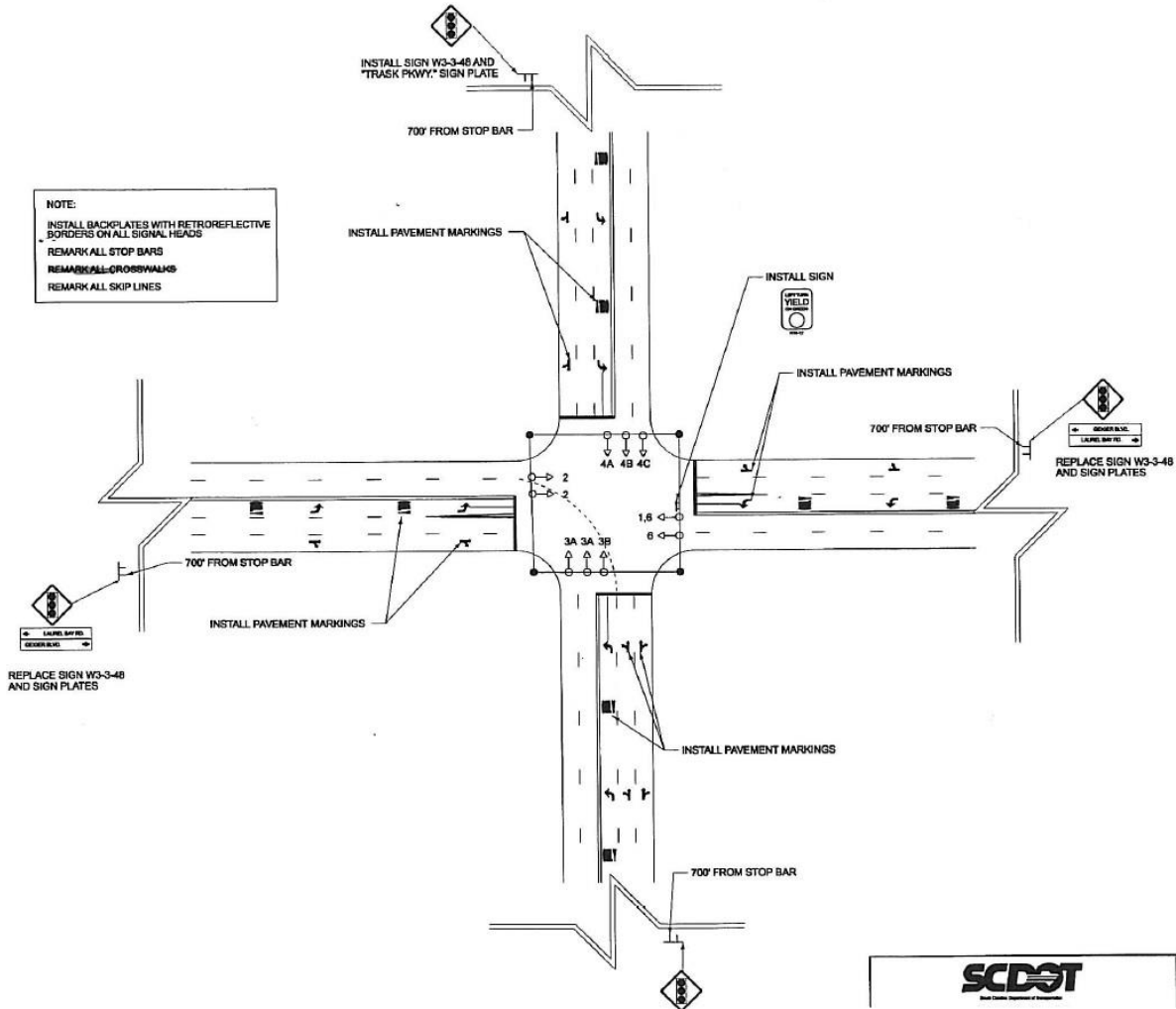
Figure 1. Illustration. Example of signalized intersection improvements.
