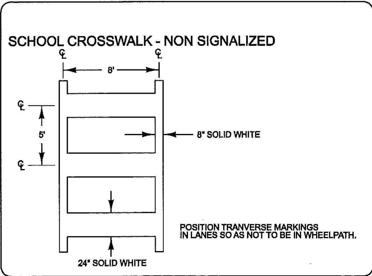
Figure 34. Illustration. SCDOT Standard Drawing 625-305-00 excerpts for crosswalk markings.
