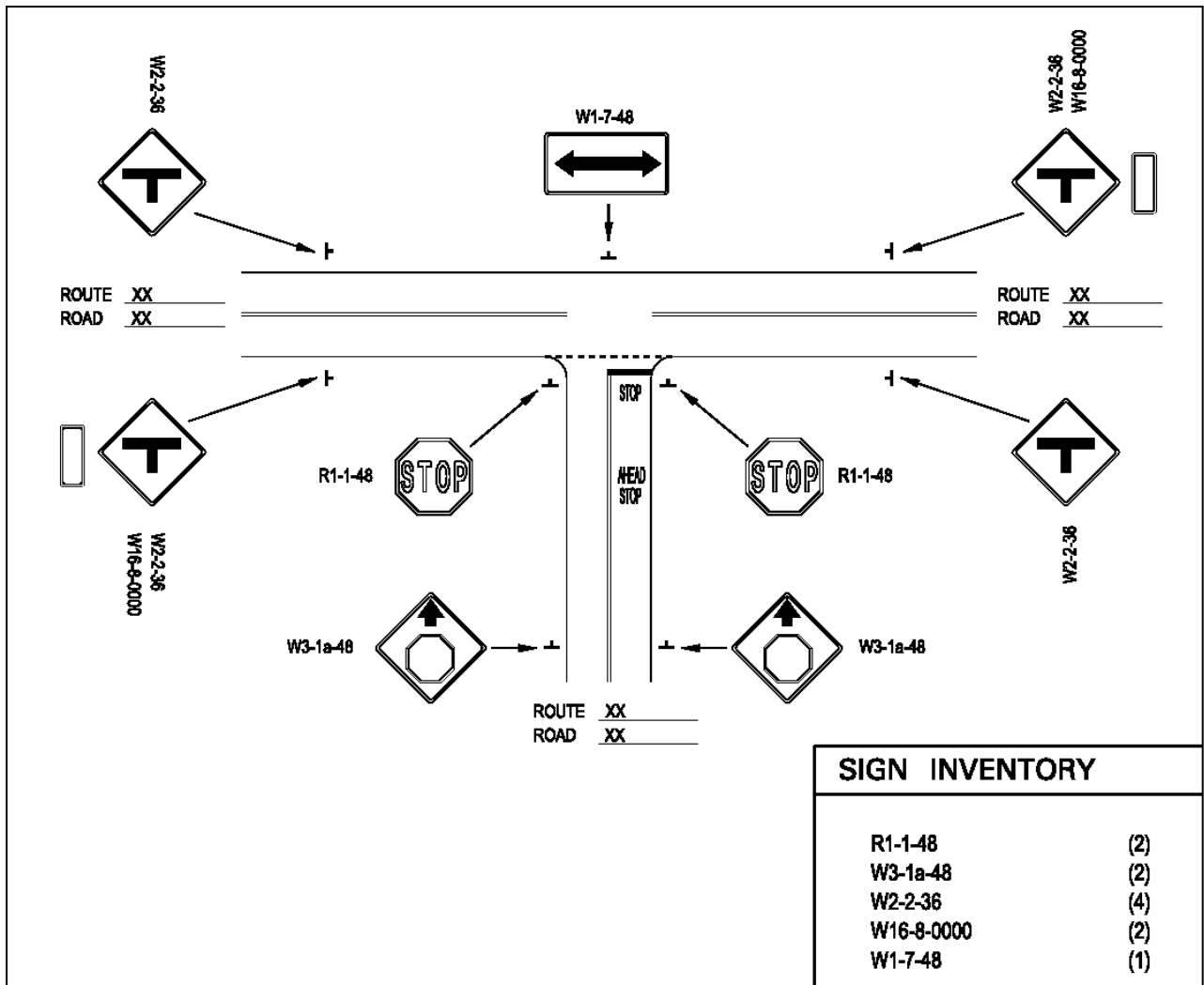
Figure 53. Illustration. SCDOT typical for a t-type stop controlled intersection.
