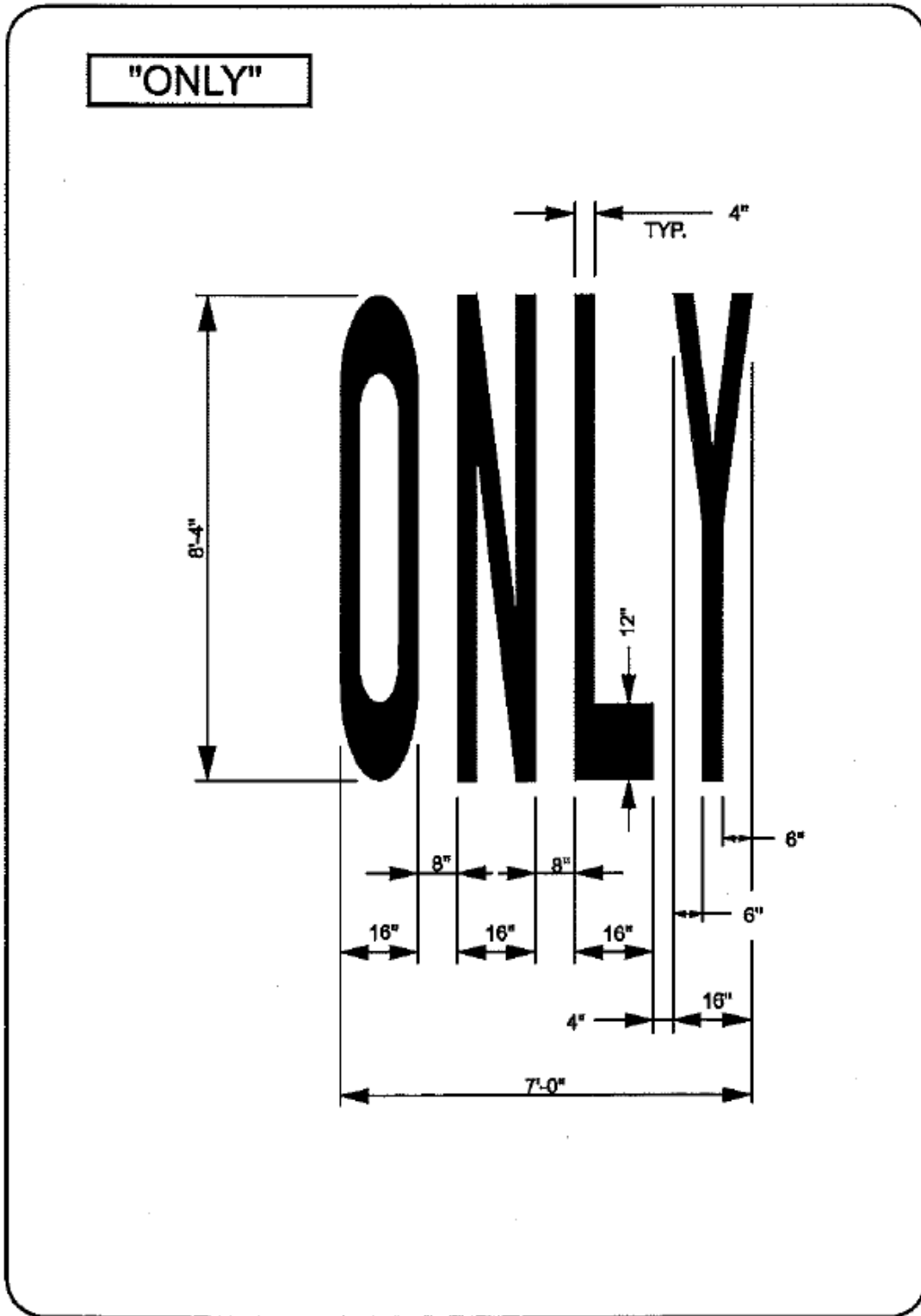
Figure 42. Illustration. SCDOT Standard Drawing 625-410-00 excerpt for "ONLY" standard pavement marking.
