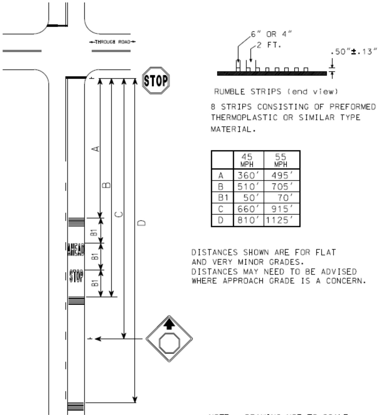
Figure 49. Illustration. SCDOT traffic engineering rumble strip typical.
