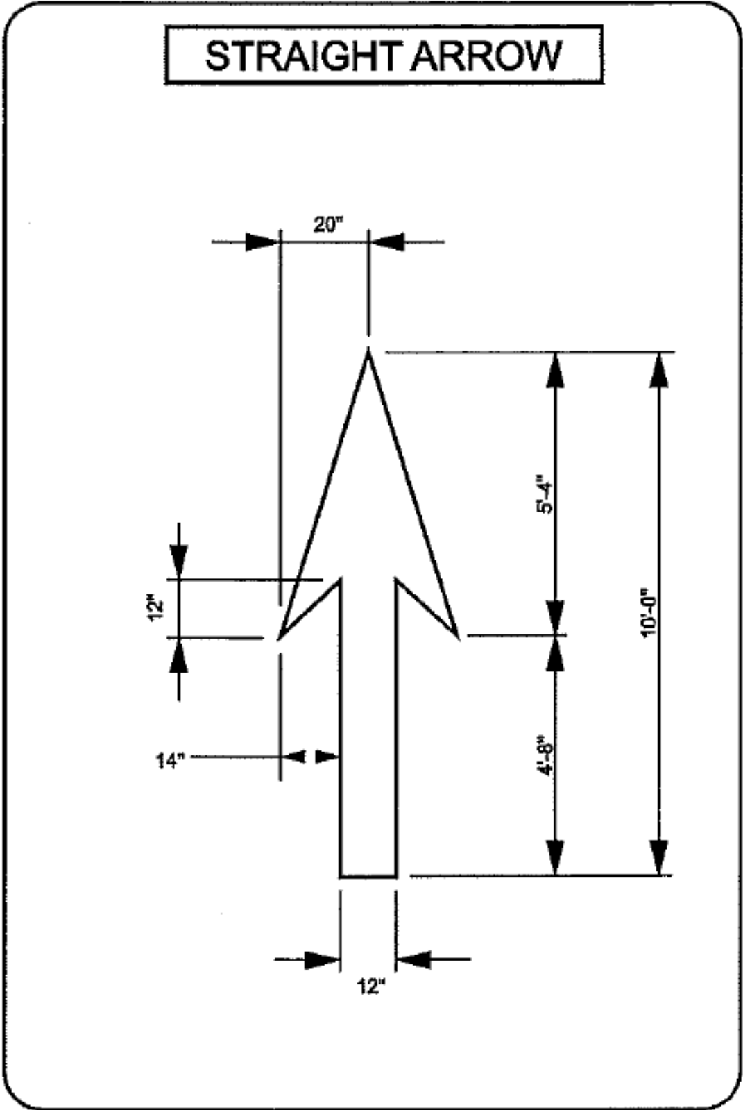
Figure 39. Illustration. SCDOT Standard Drawing 625-410-00 excerpt for straight arrow standard pavement marking.
