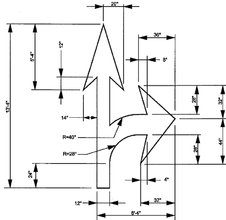
Figure 40. Illustration. SCDOT Standard Drawing 625-410-00 excerpt for right or left turn arrow and combination straight and left or right turn arrow standard pavement marking.
