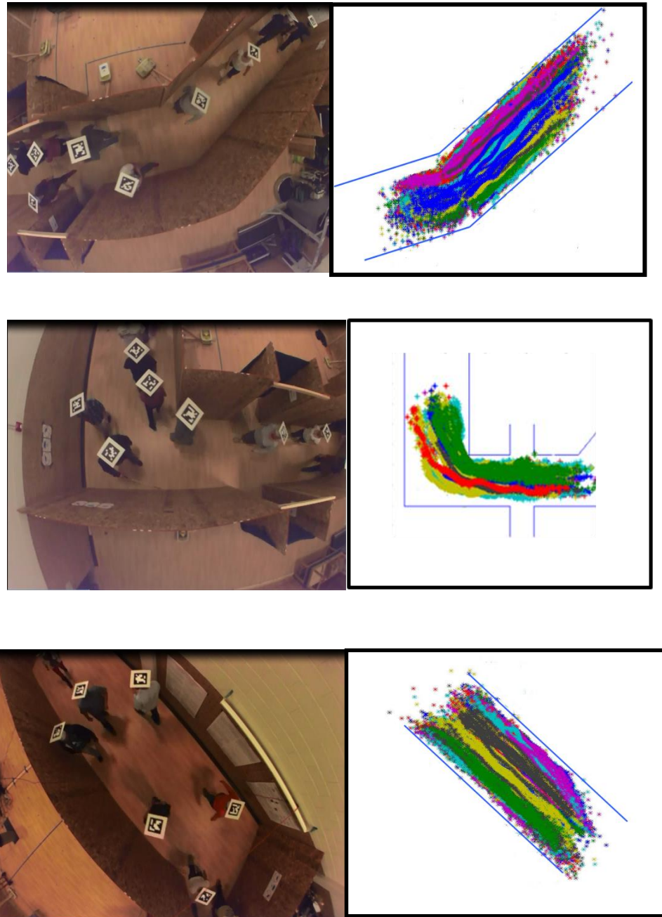
Figure 5. Tracking results.
