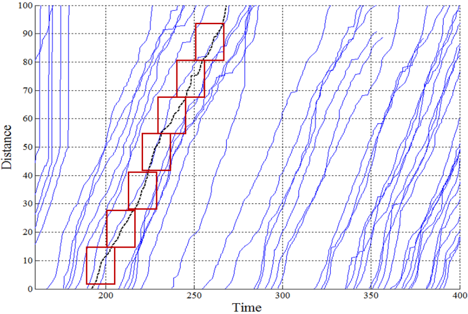
Figure 7. Time-space diagram for a surveyed participant.
