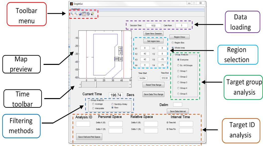
Figure 4. Snapshot of GUI.
